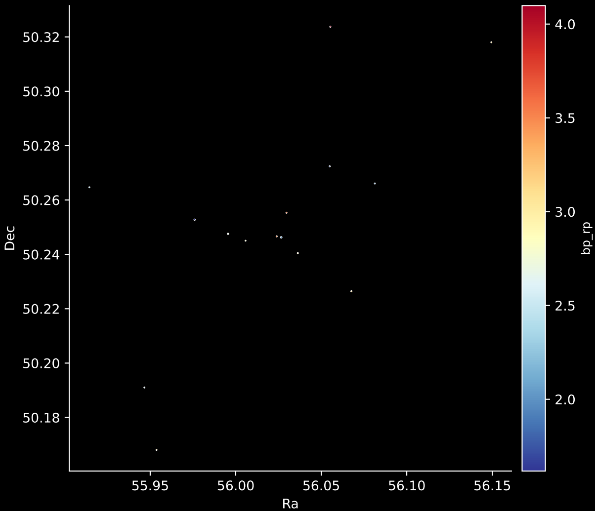
Gaia Cluster: [LDN_988e] Stars: 15
