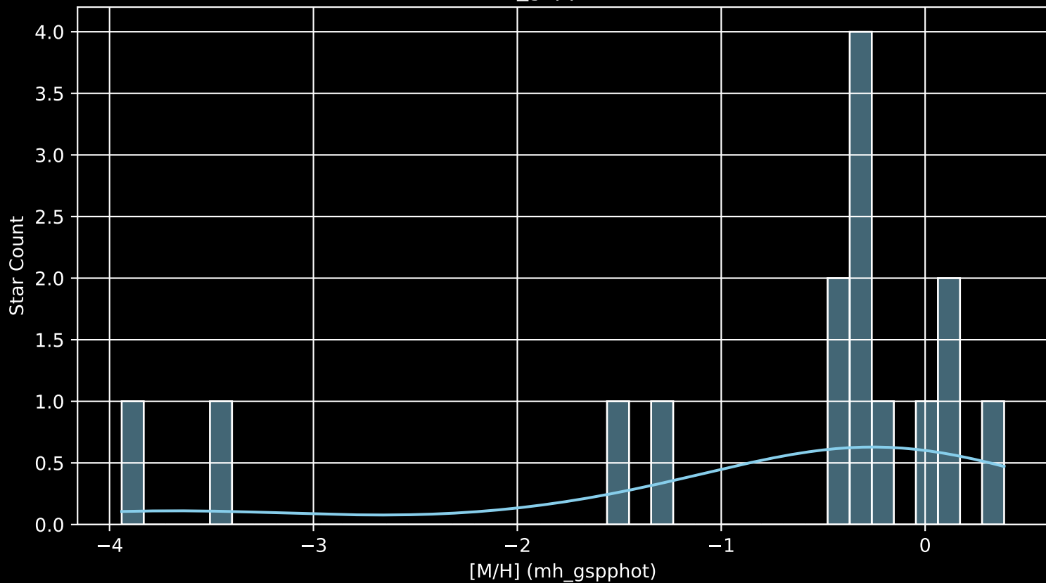
Gaia Cluster: [LDN_988e [M/H] (mh_gspphot) (n= 15)
