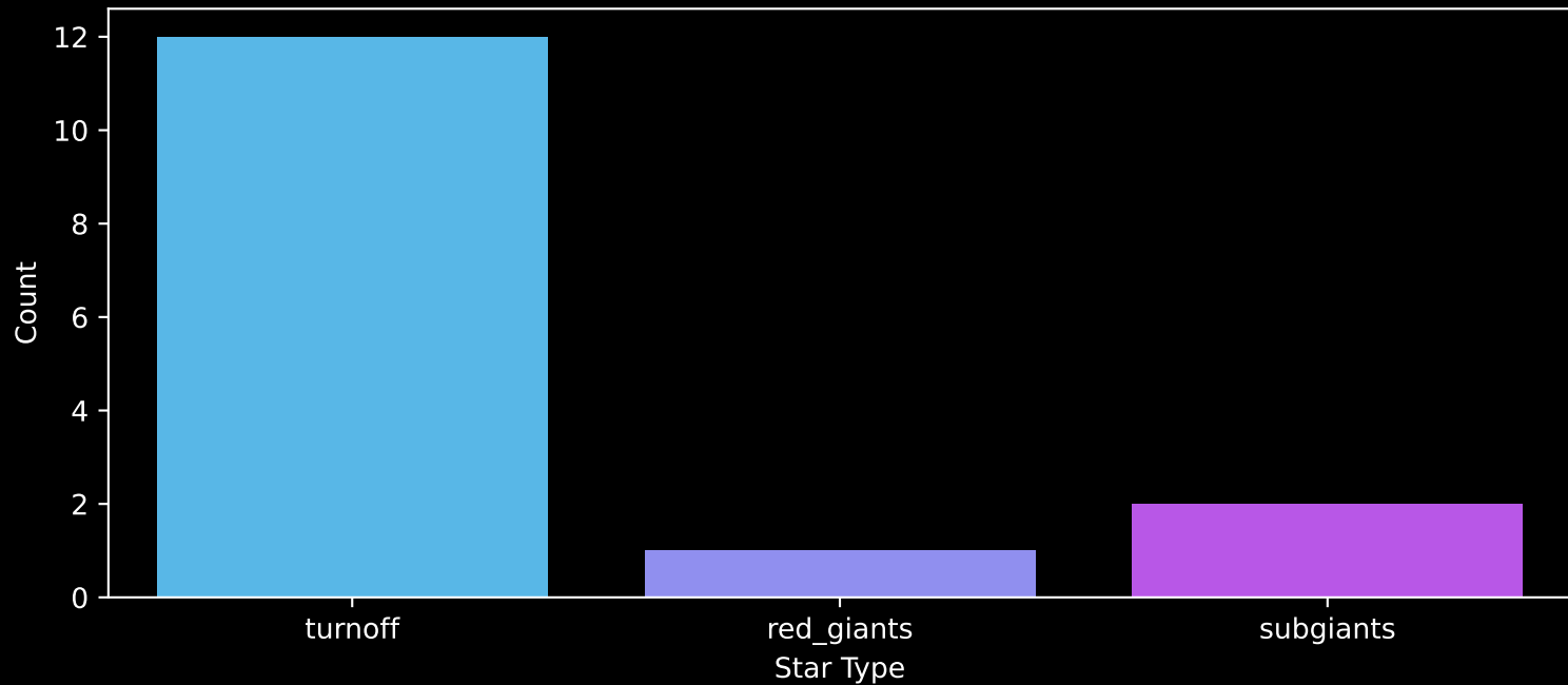
Gaia Cluster: [LDN_988e] Count plot of Star Type
