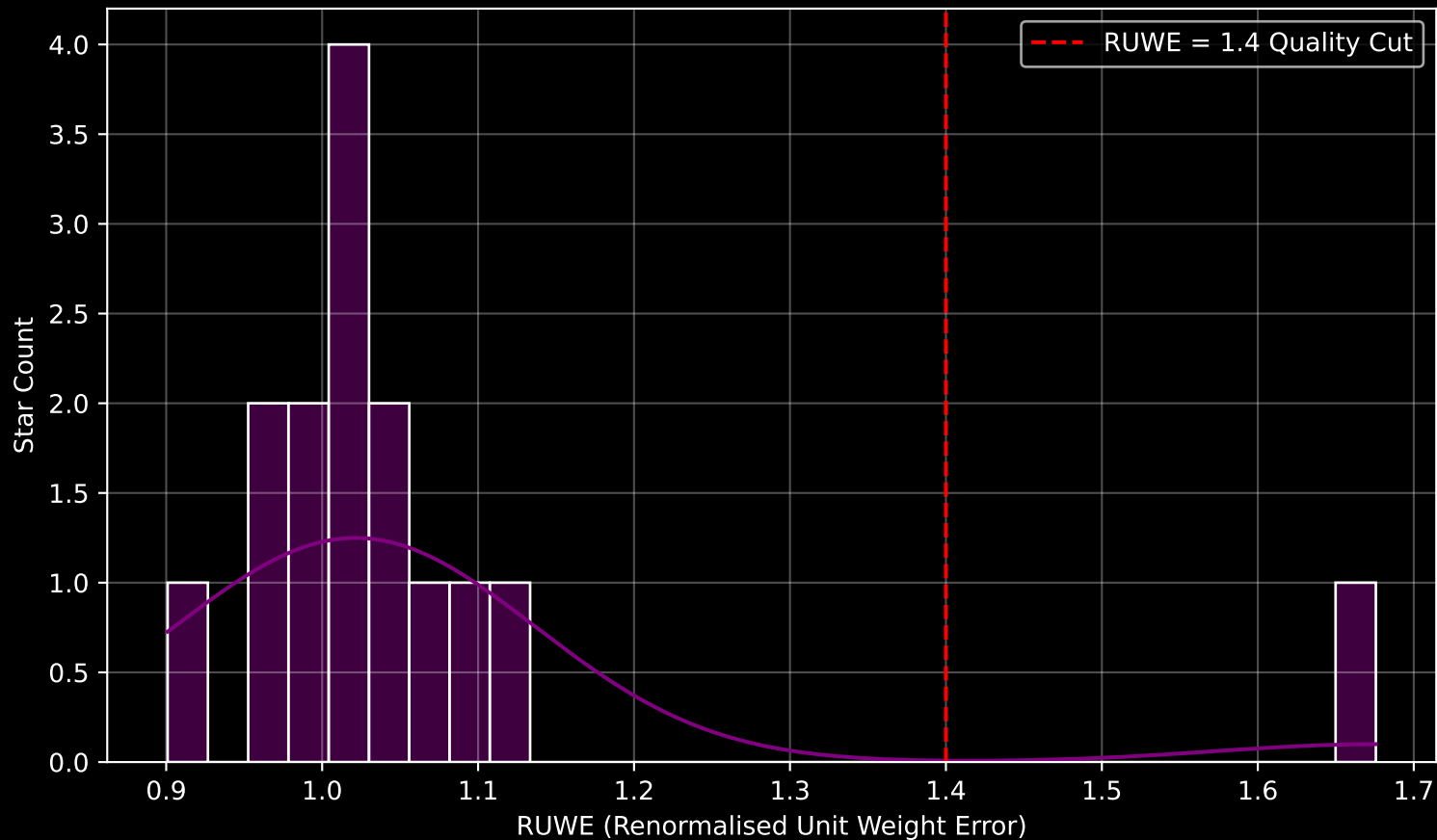
Gaia Cluster: [LDN_988e] RUWE Distribution (n= 15)
