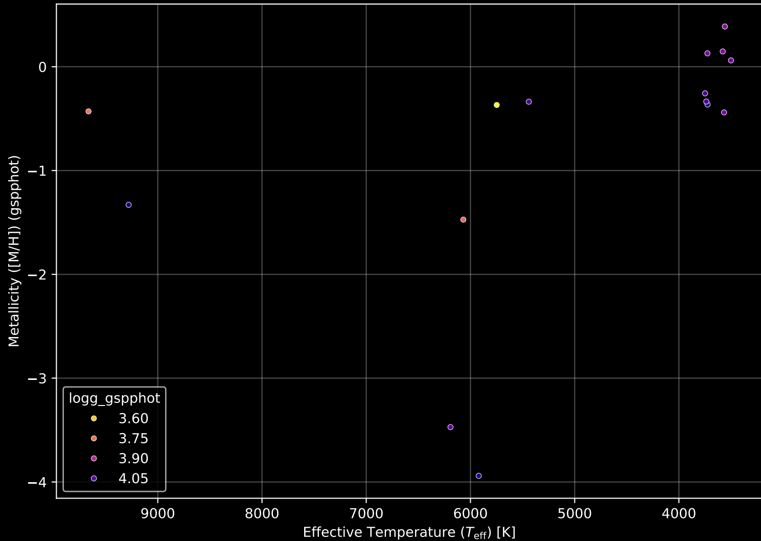
Gaia Cluster: [LDN_988e] Stellar Population Parameters (n= 15)
