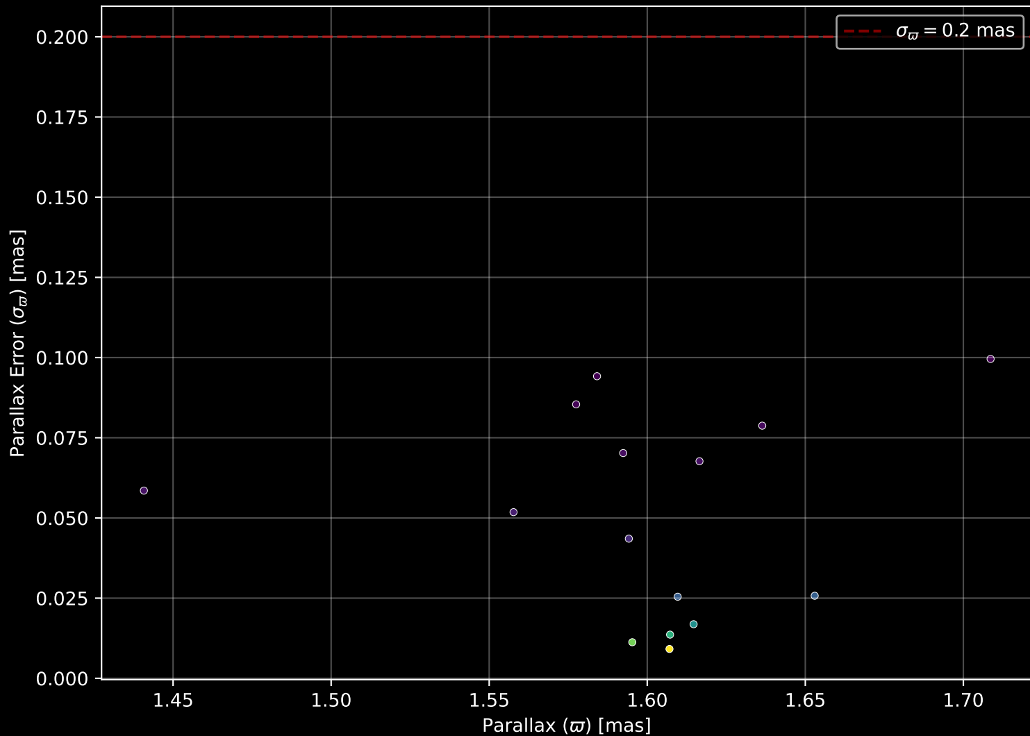
Gaia Cluster: [LDN_988e] Parallax Quality (n= 15)
