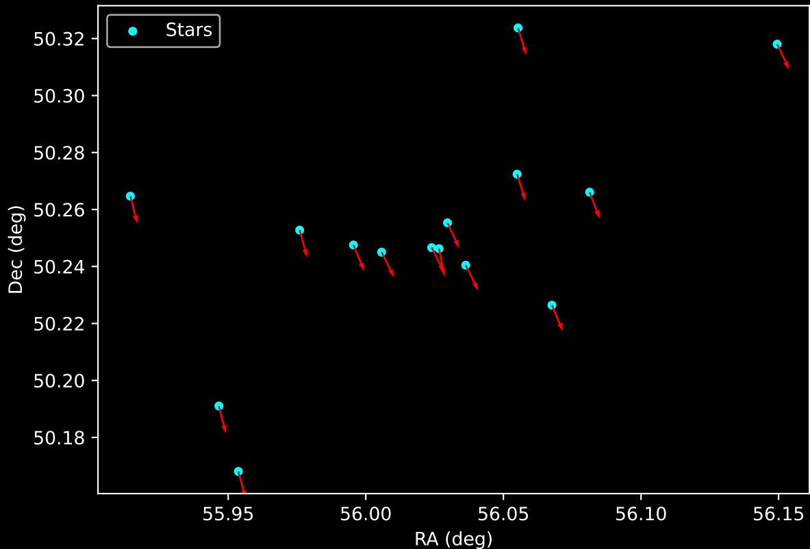
Gaia Cluster: [LDN_988e] Proper Motion Vectors for Gaia Star Field (n= 15)
