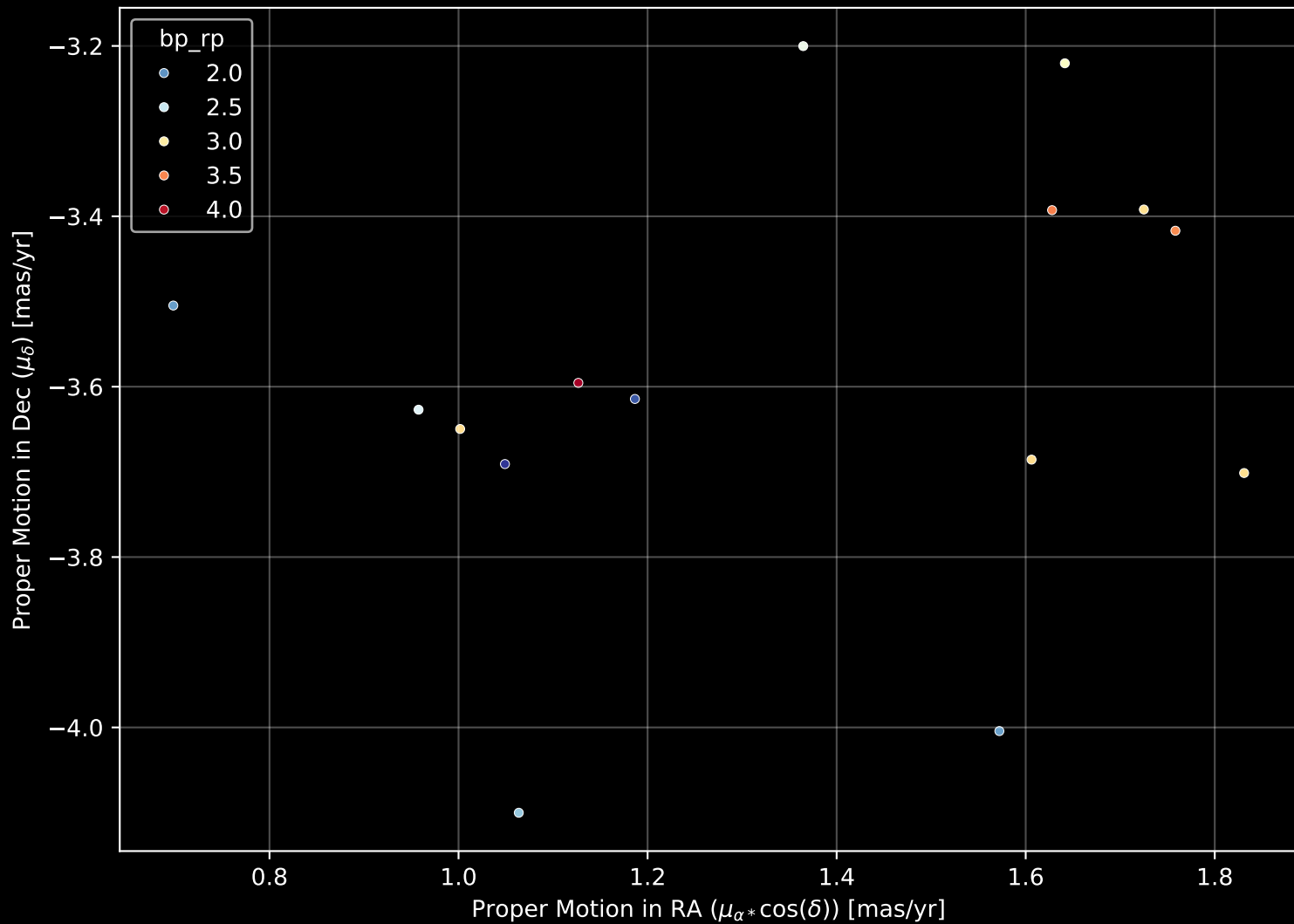
Gaia Cluster: [LDN_988e] Proper Motion Diagram (n= 15)
