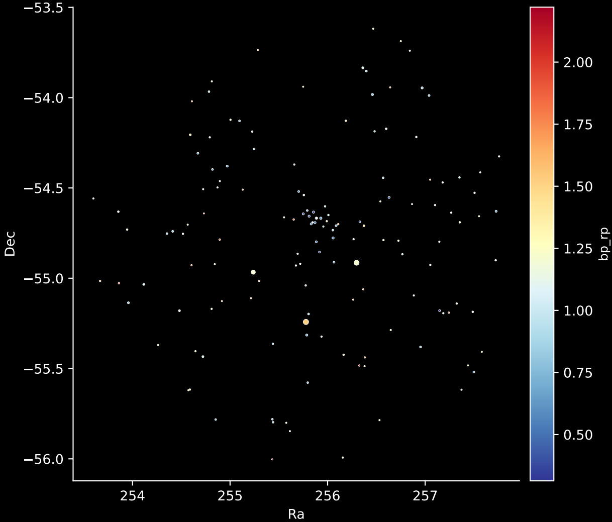
Gaia Cluster: [Loden_46] Stars: 144
