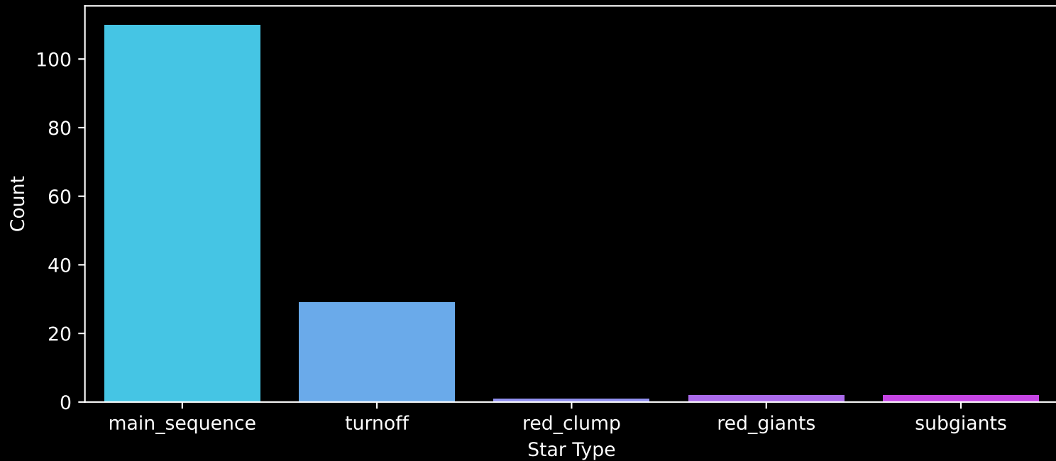
Gaia Cluster: [Loden_46] Count plot of Star Type
