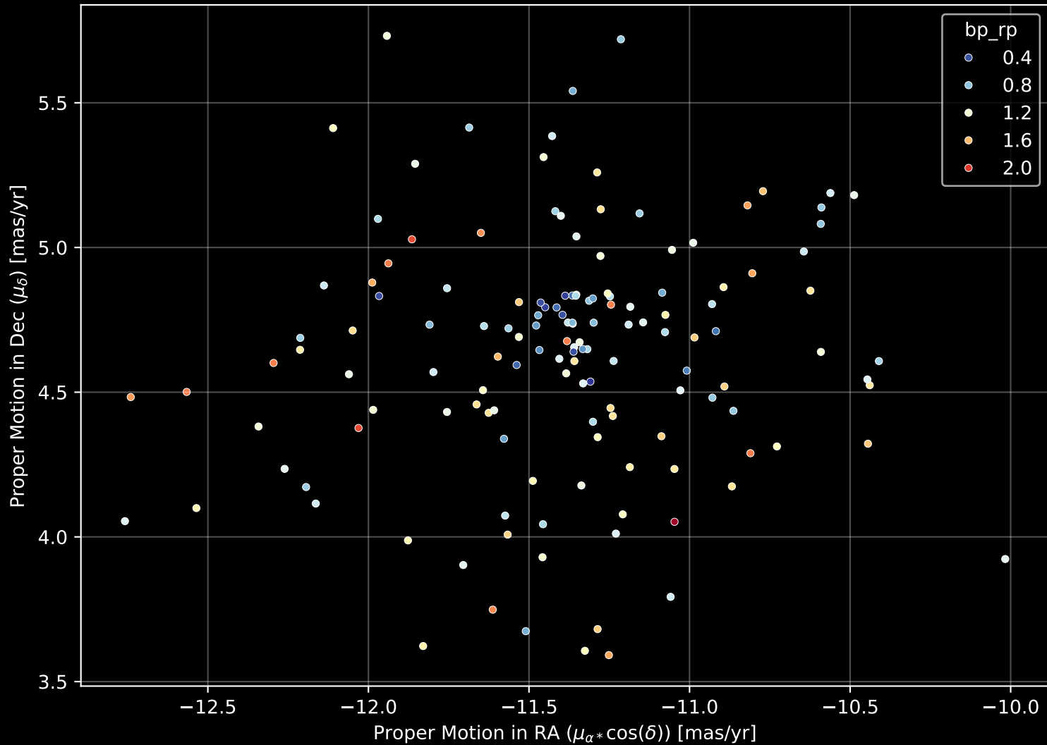
Gaia Cluster: [Loden_46] Proper Motion Diagram (n= 144)
