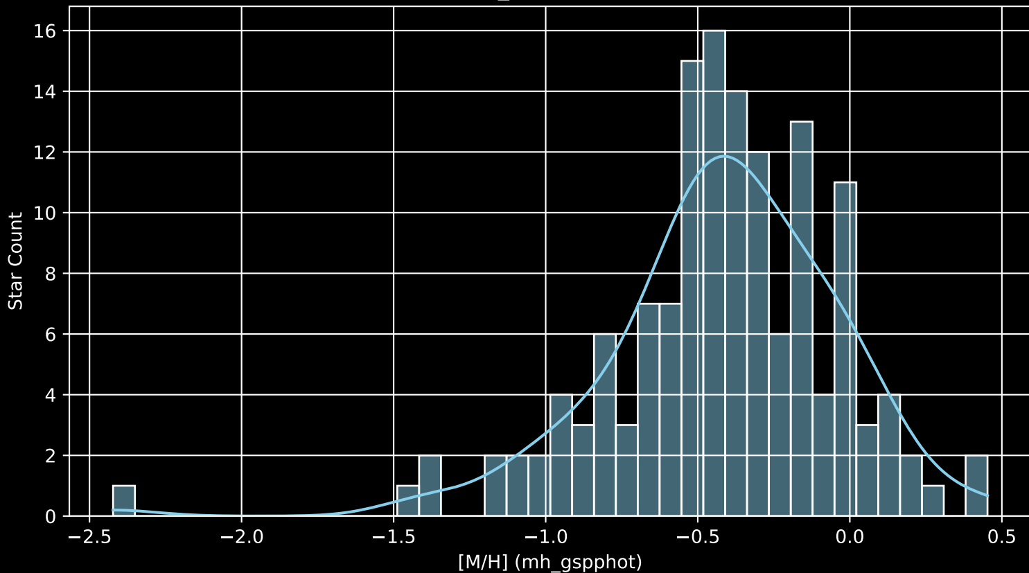
Gaia Cluster: [Loden_46 [M/H] (mh_gspphot) (n= 143)
