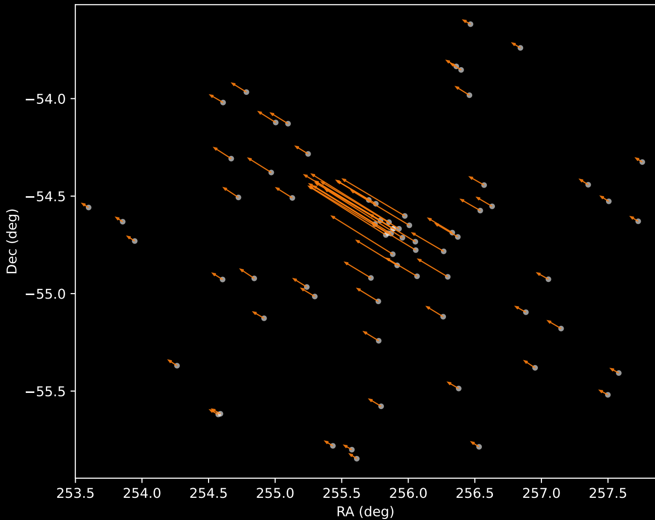
Gaia DR3 Cluster 2 Proper Motion Vectors (n=71)
