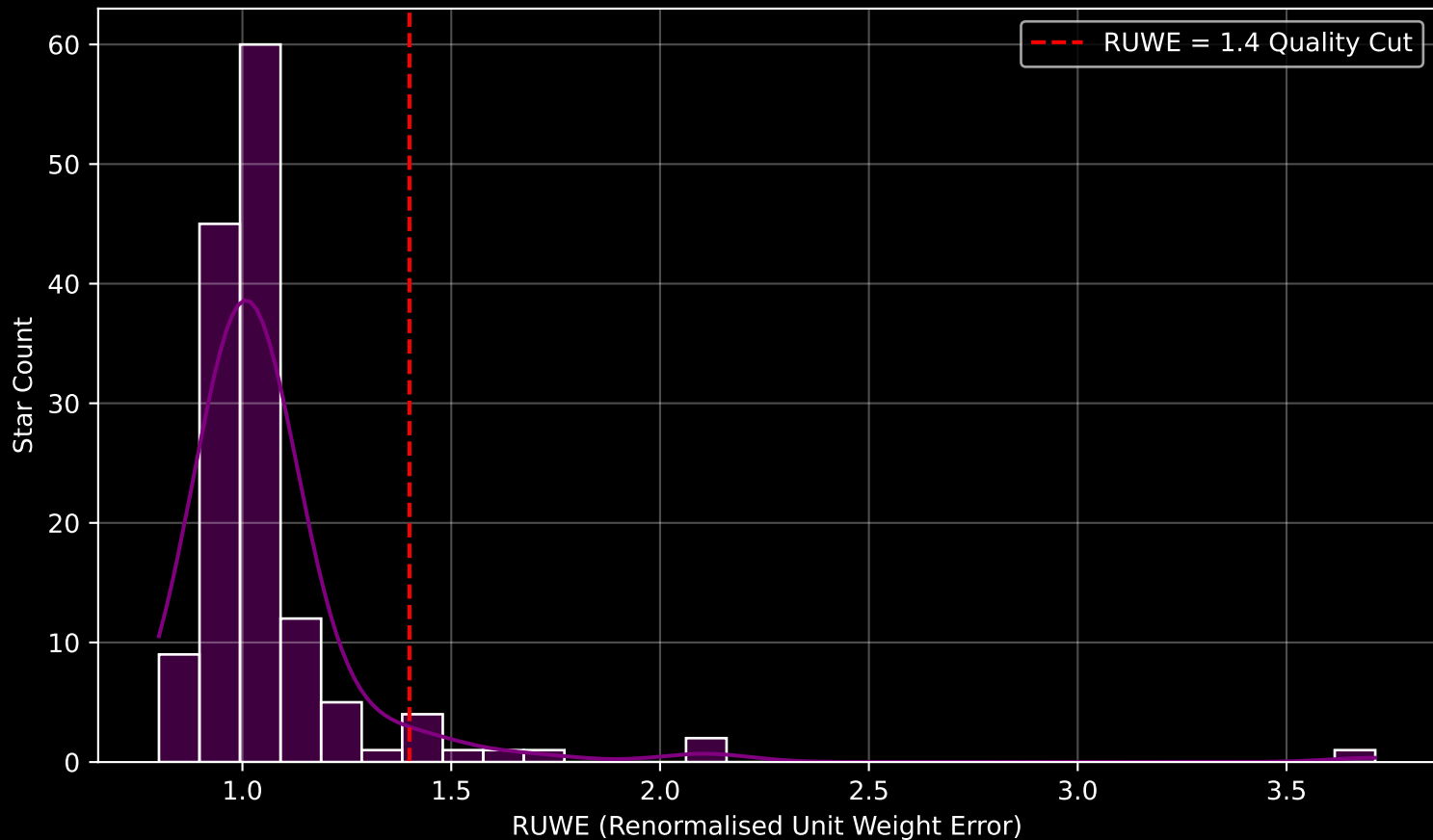
Gaia Cluster: [Loden_46] RUWE Distribution (n= 142)
