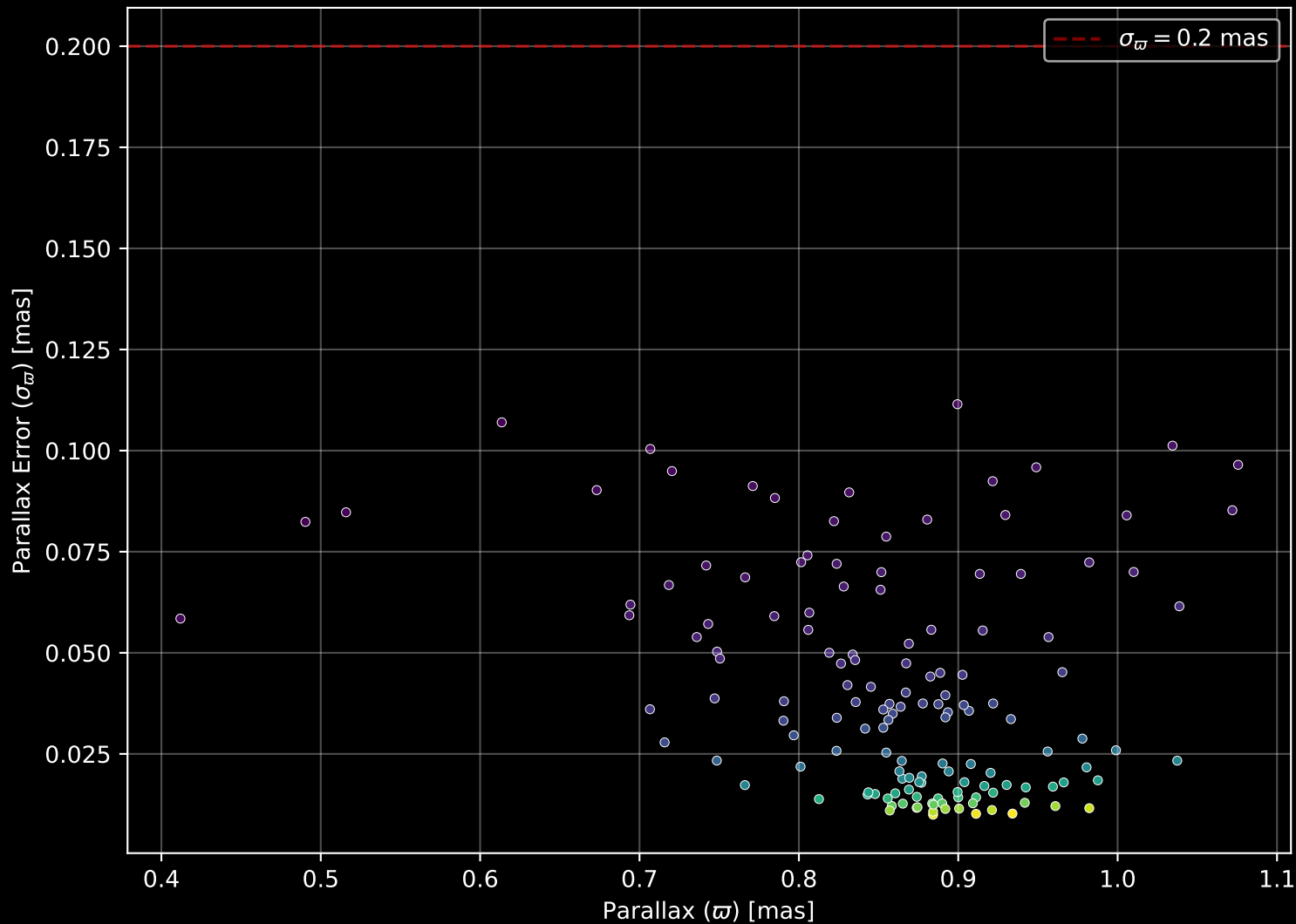
Gaia Cluster: [Loden_46] Parallax Quality (n= 144)
