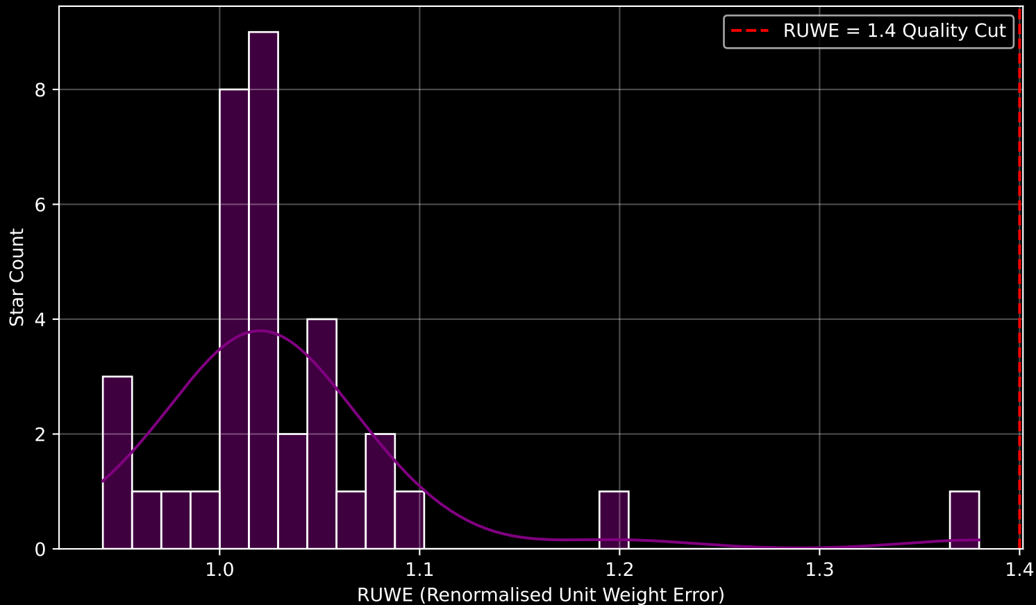
Gaia Cluster: [Lynga_1] RUWE Distribution (n= 35)
