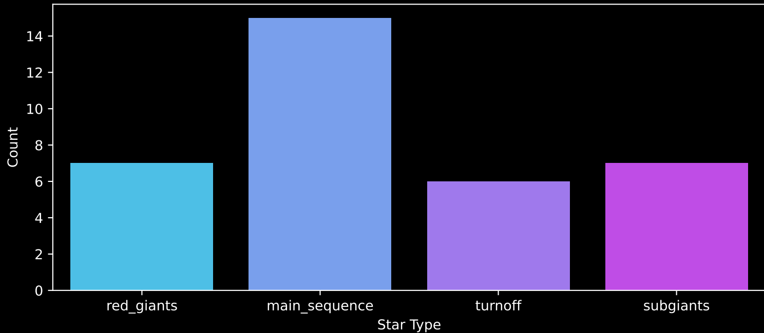
Gaia Cluster: [Lynga_1] Count plot of Star Type
