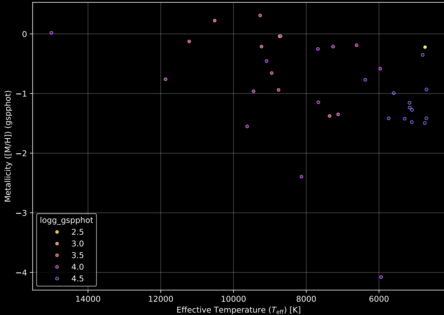
Gaia Cluster: [Lynga_1] Stellar Population Parameters (n= 35)
