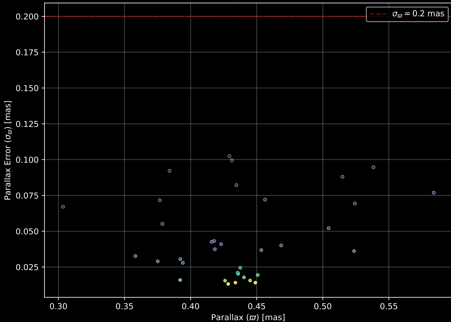
Gaia Cluster: [Lynga_1] Parallax Quality (n= 35)
