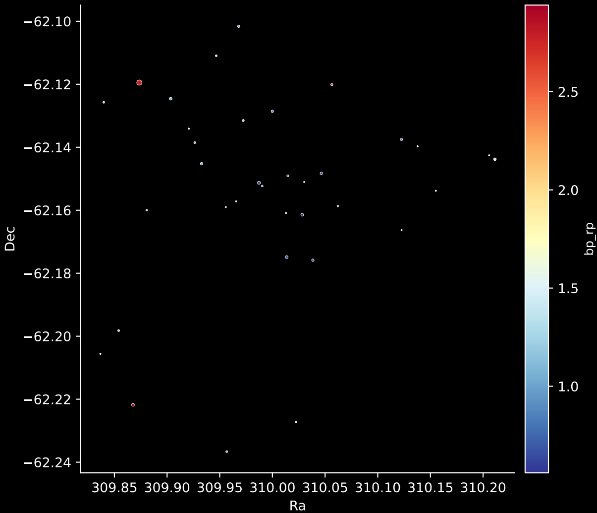
Gaia Cluster: [Lynga_1] Stars: 35
