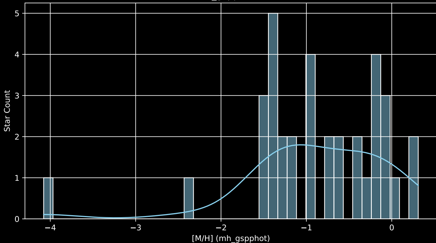
Gaia Cluster: [Lynga_1 [M/H] (mh_gspphot) (n= 35)
