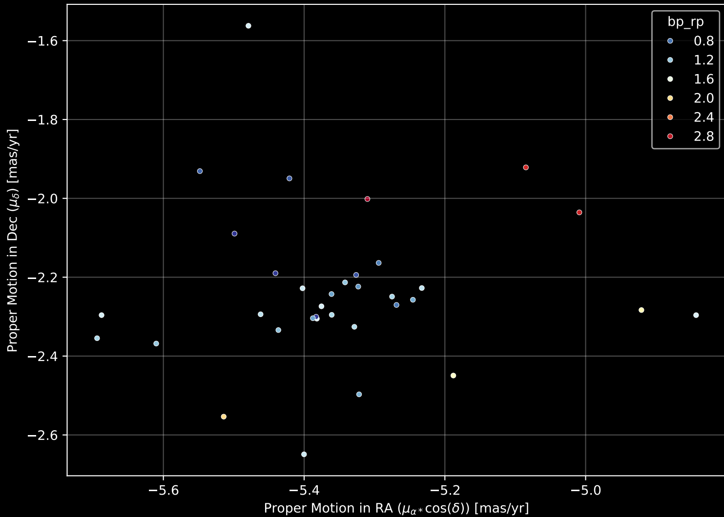
Gaia Cluster: [Lynga_1] Proper Motion Diagram (n= 35)
