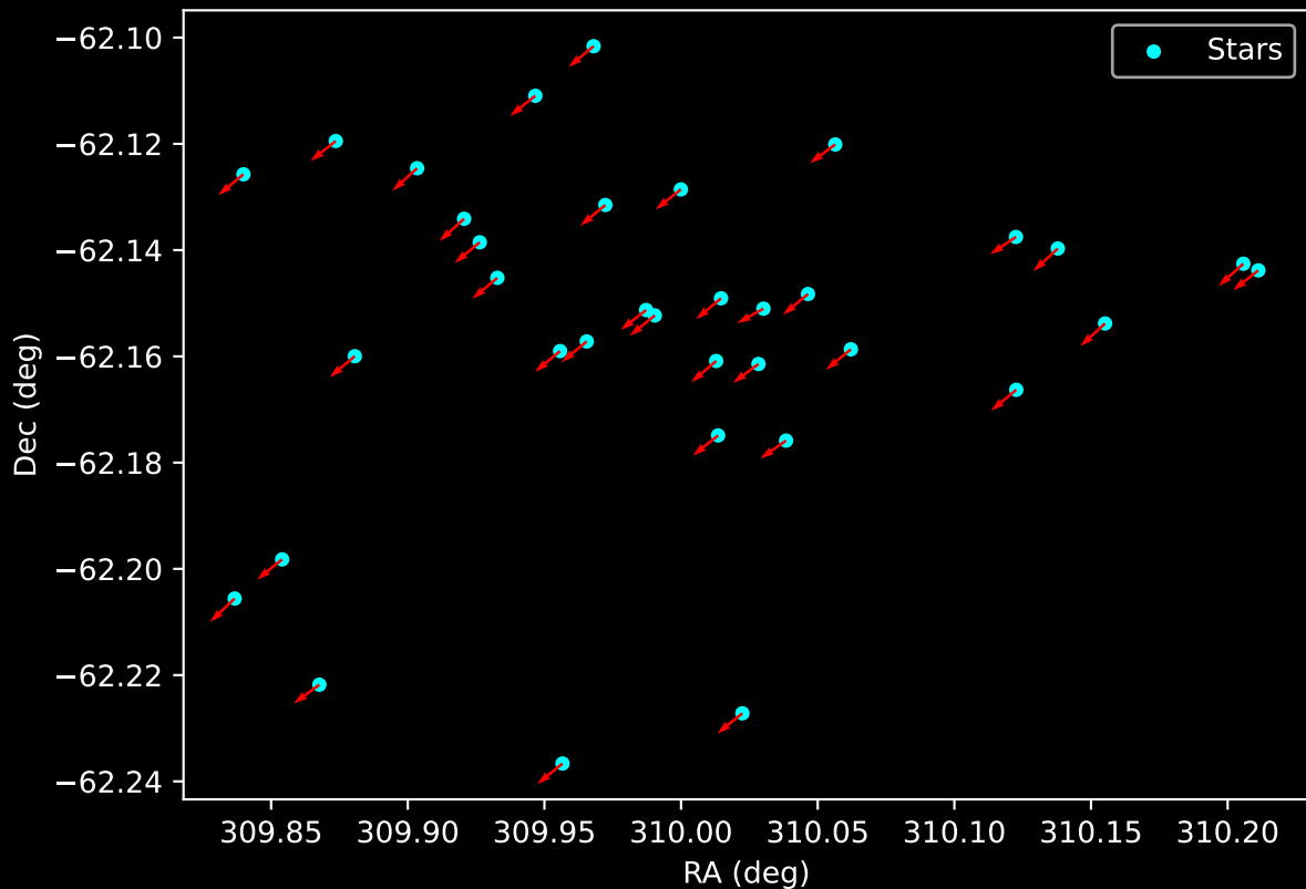
Gaia Cluster: [Lynga_1] Proper Motion Vectors for Gaia Star Field (n= 35)
