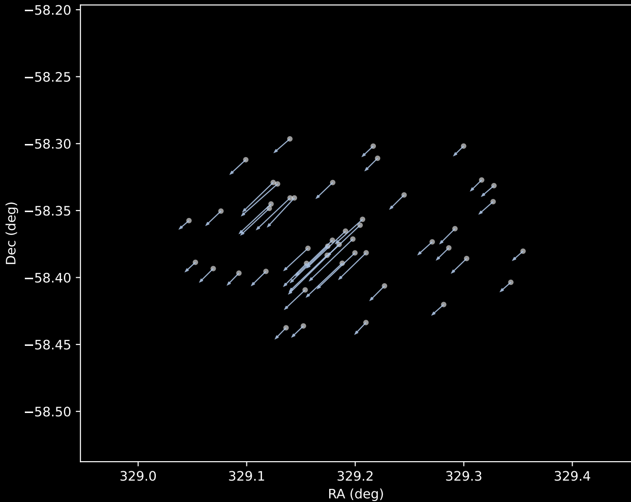
Gaia DR3 Cluster 1 Proper Motion Vectors (n=47)
