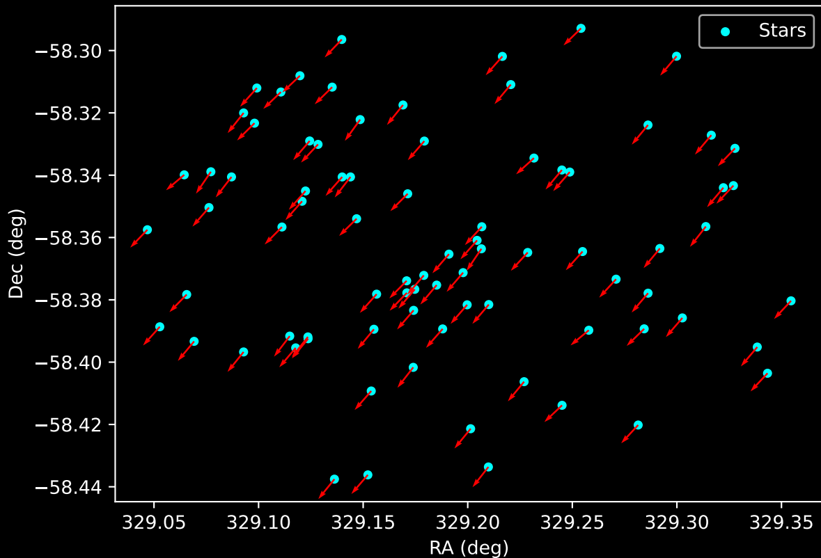
Gaia Cluster: [Lynga_3] Proper Motion Vectors for Gaia Star Field (n= 81)
