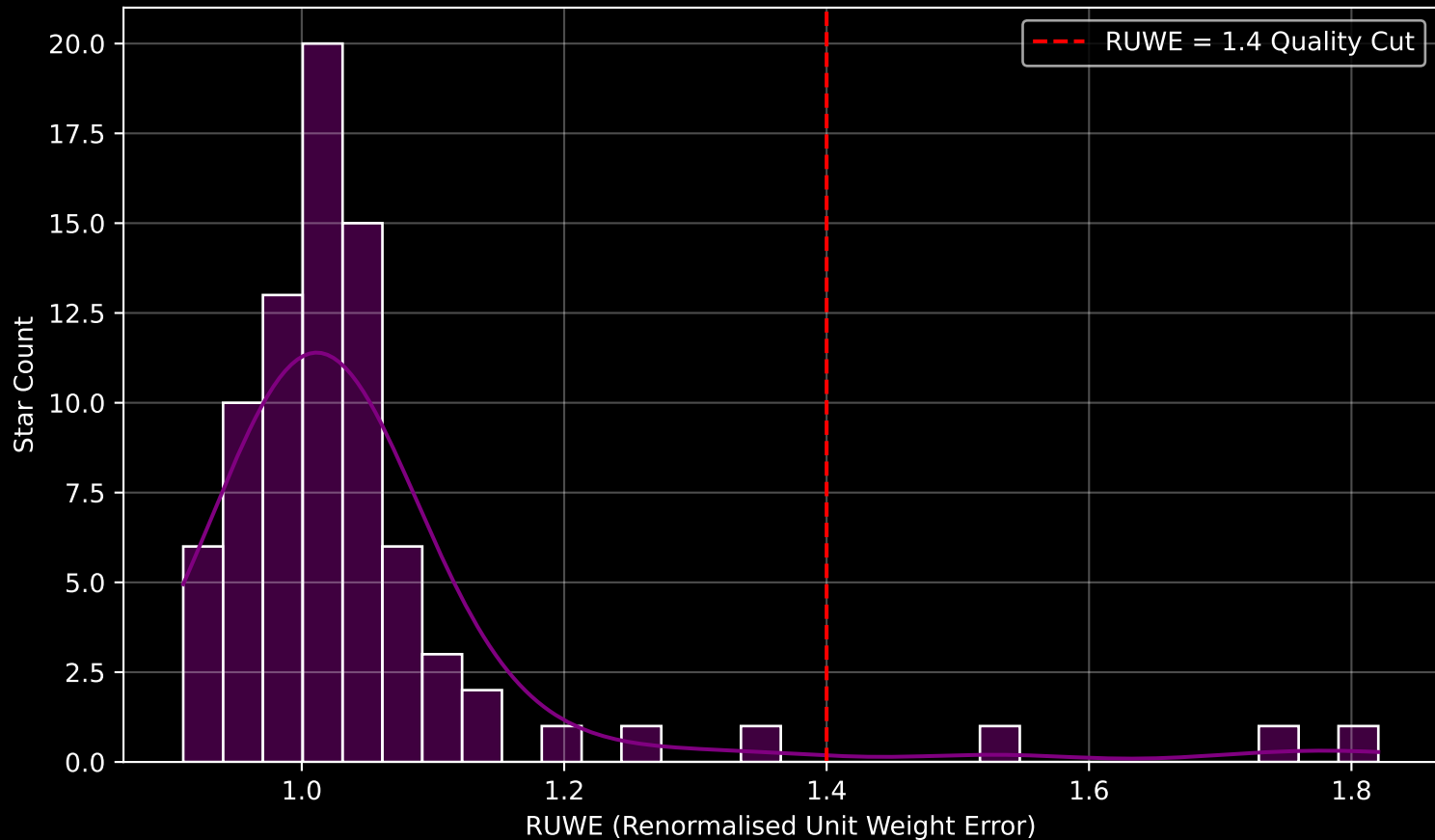
Gaia Cluster: [Lynga_3] RUWE Distribution (n= 81)
