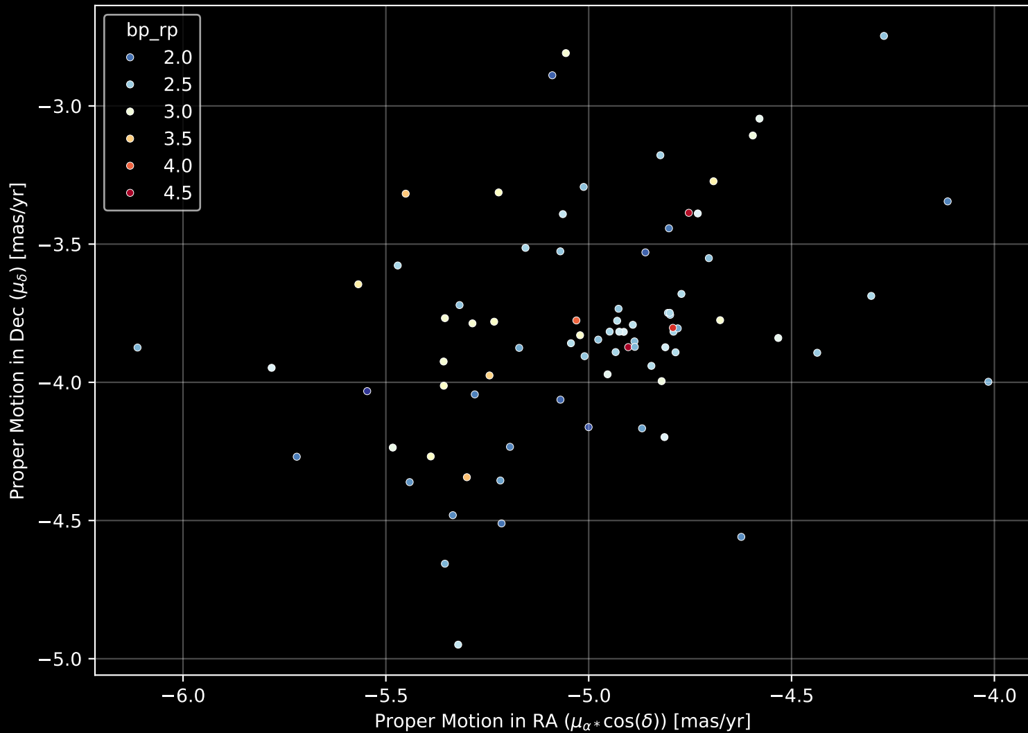
Gaia Cluster: [Lynga_3] Proper Motion Diagram (n= 81)
