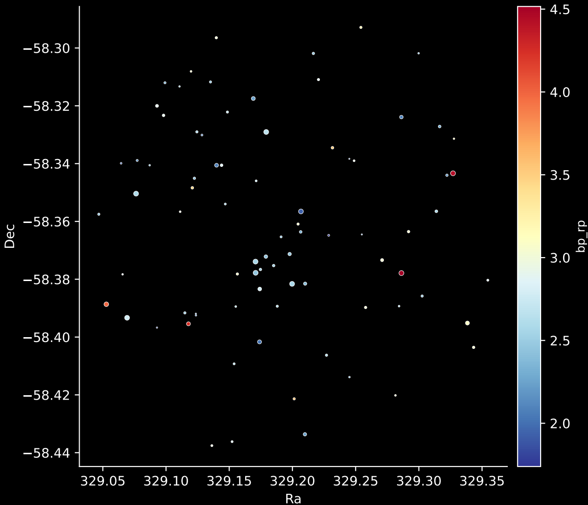
Gaia Cluster: [Lynga_3] Stars: 81
