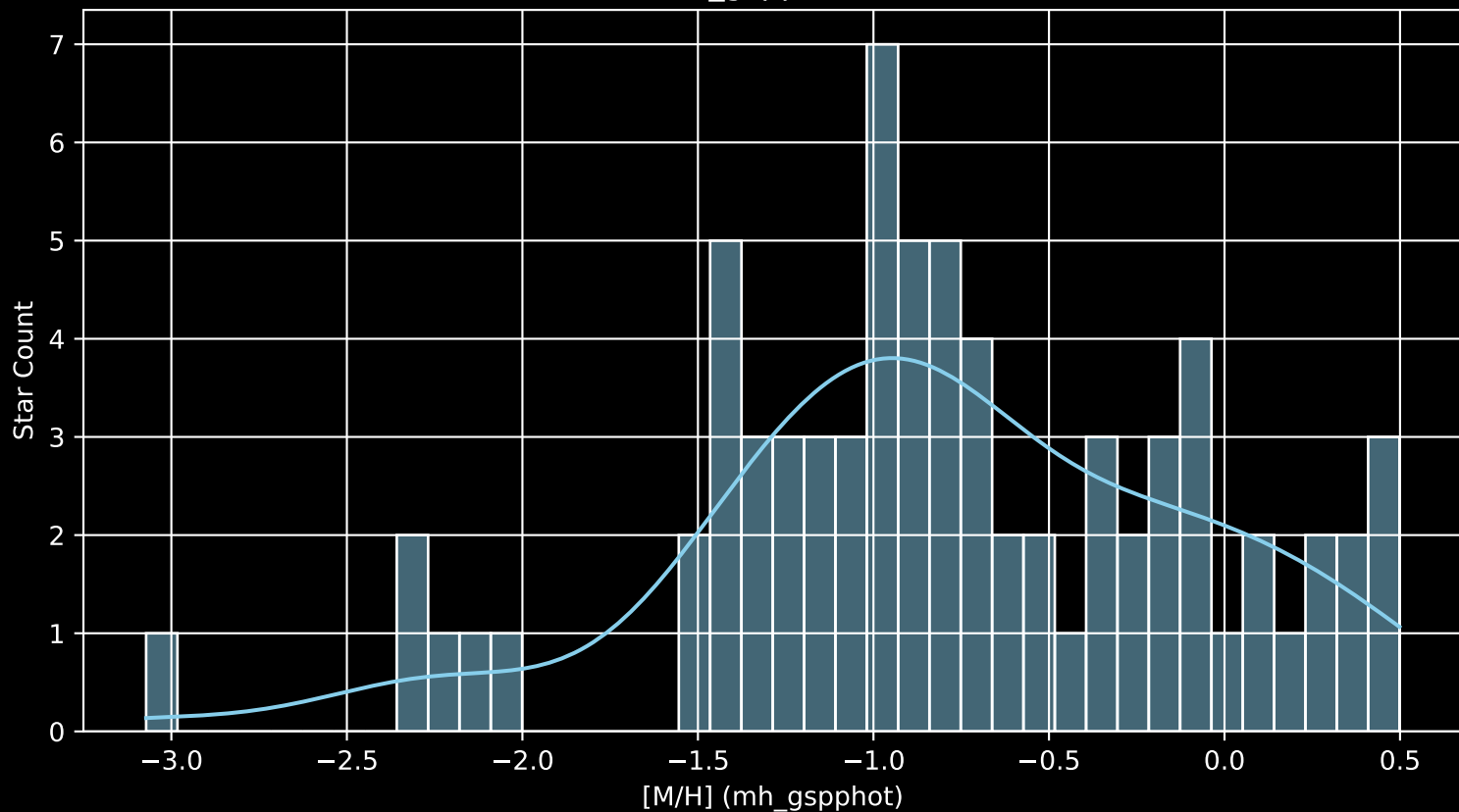
Gaia Cluster: [Lynga_3 [M/H] (mh_gspphot) (n= 74)
