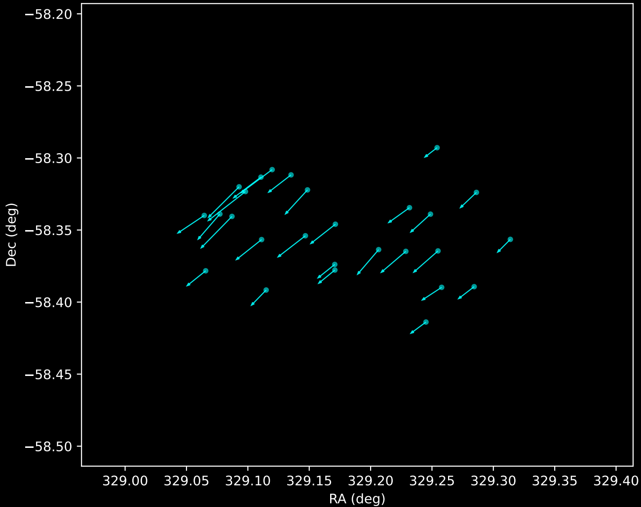
Gaia DR3 Noise Stream Proper Motion Vectors (n=27)
