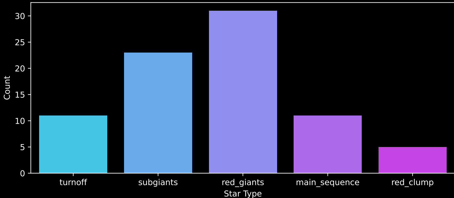
Gaia Cluster: [Lynga_3] Count plot of Star Type
