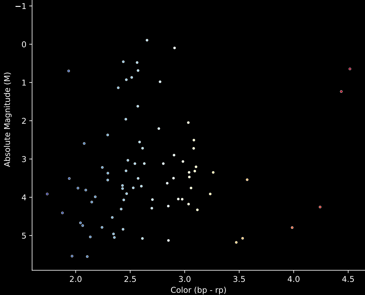
Gaia Cluster: [Lynga_3] Stars (n= 81) Hertzsprung-Russel Diagram
