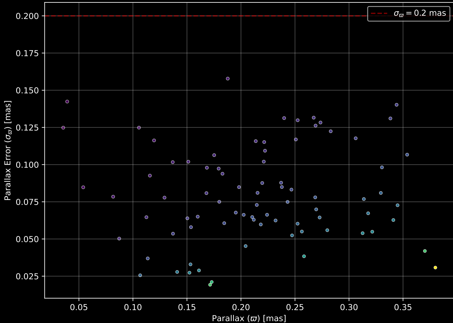
Gaia Cluster: [Lynga_3] Parallax Quality (n= 81)
