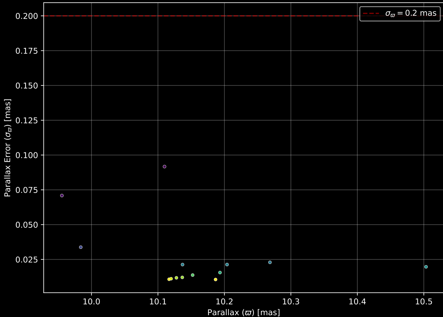
Gaia Cluster: [Mamajek_1] Parallax Quality (n= 14)
