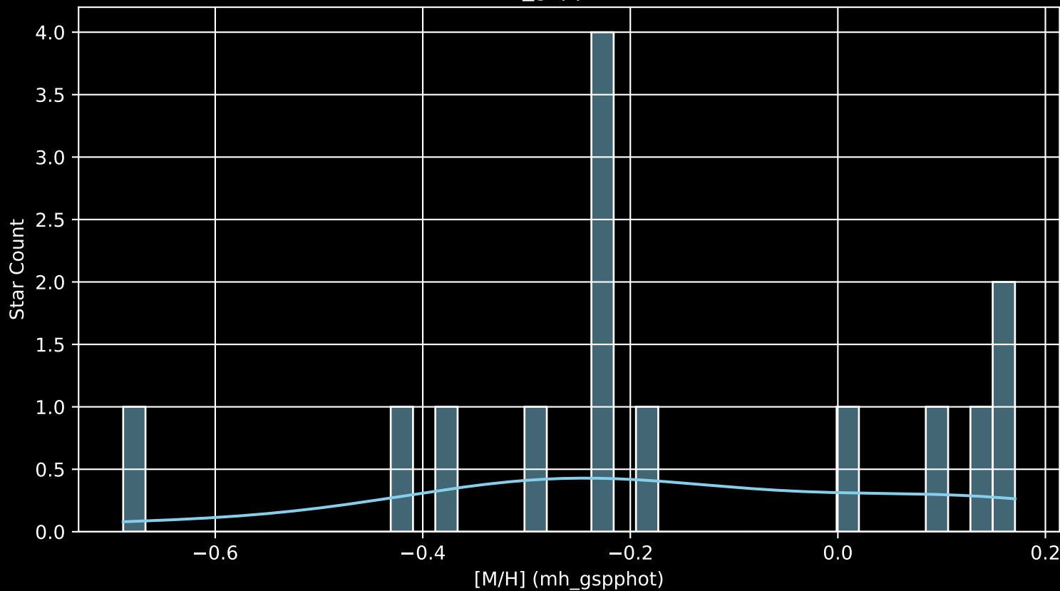
Gaia Cluster: [Mamajek_1 [M/H] (mh_gspphot) (n= 14)
