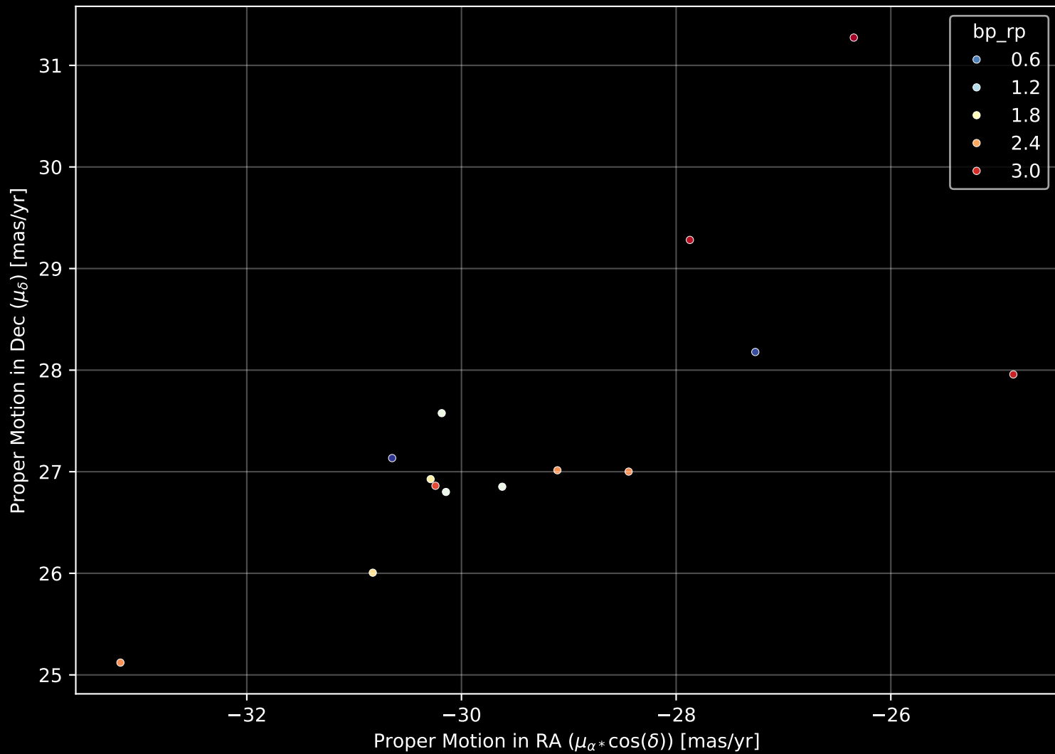
Gaia Cluster: [Mamajek_1] Proper Motion Diagram (n= 14)
