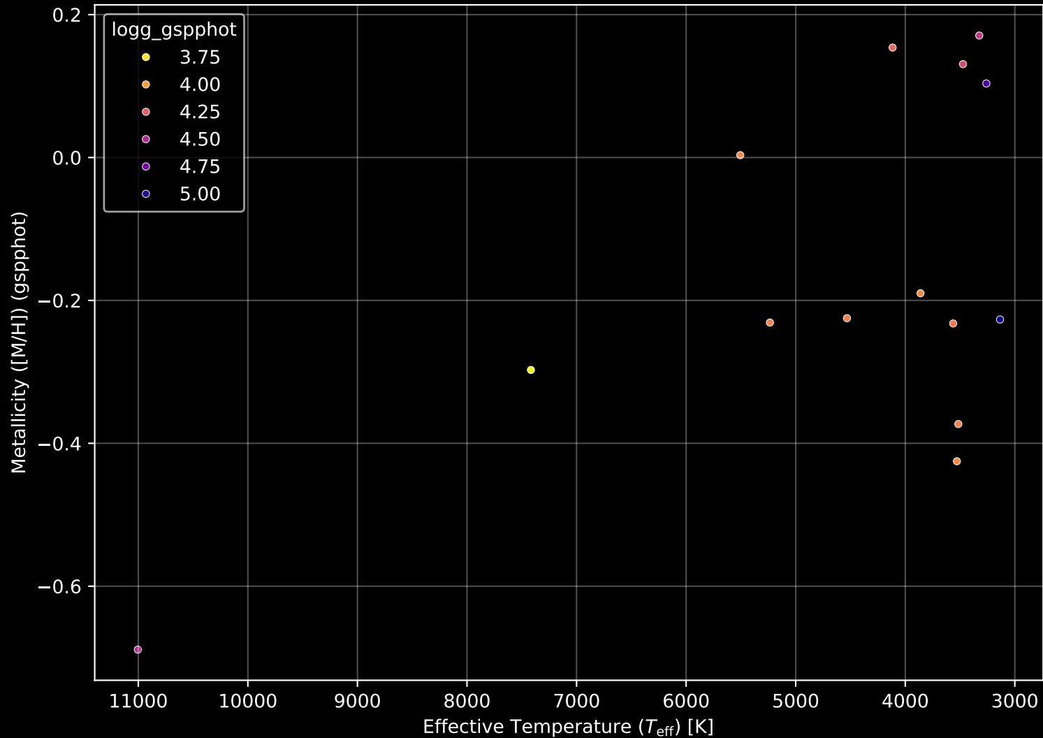
Gaia Cluster: [Mamajek_1] Stellar Population Parameters (n= 14)
