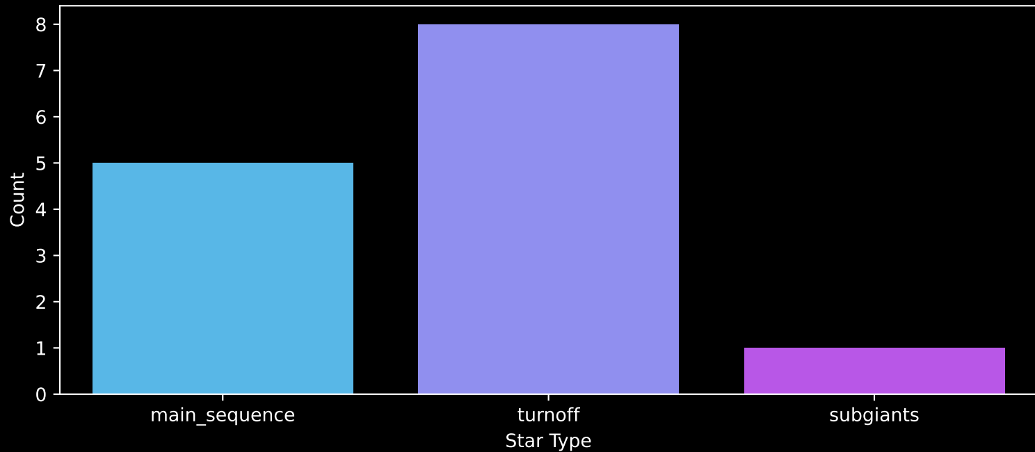
Gaia Cluster: [Mamajek_1] Count plot of Star Type
