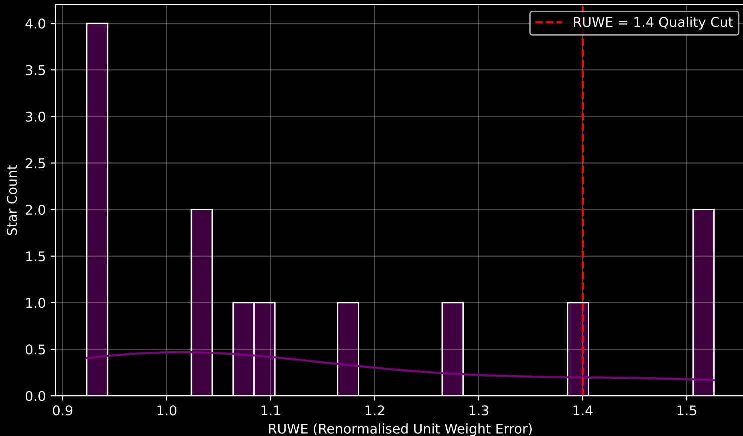
Gaia Cluster: [Mamajek_1] RUWE Distribution (n= 13)
