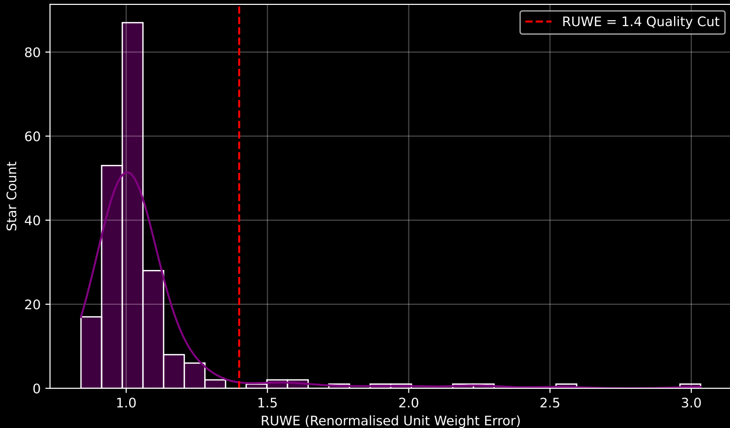
Gaia Cluster: [Mamajek_4] RUWE Distribution (n= 213)
