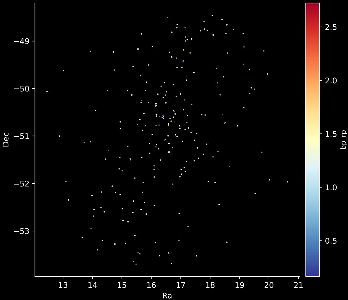
Gaia Cluster: [Mamajek_4] Stars: 215
