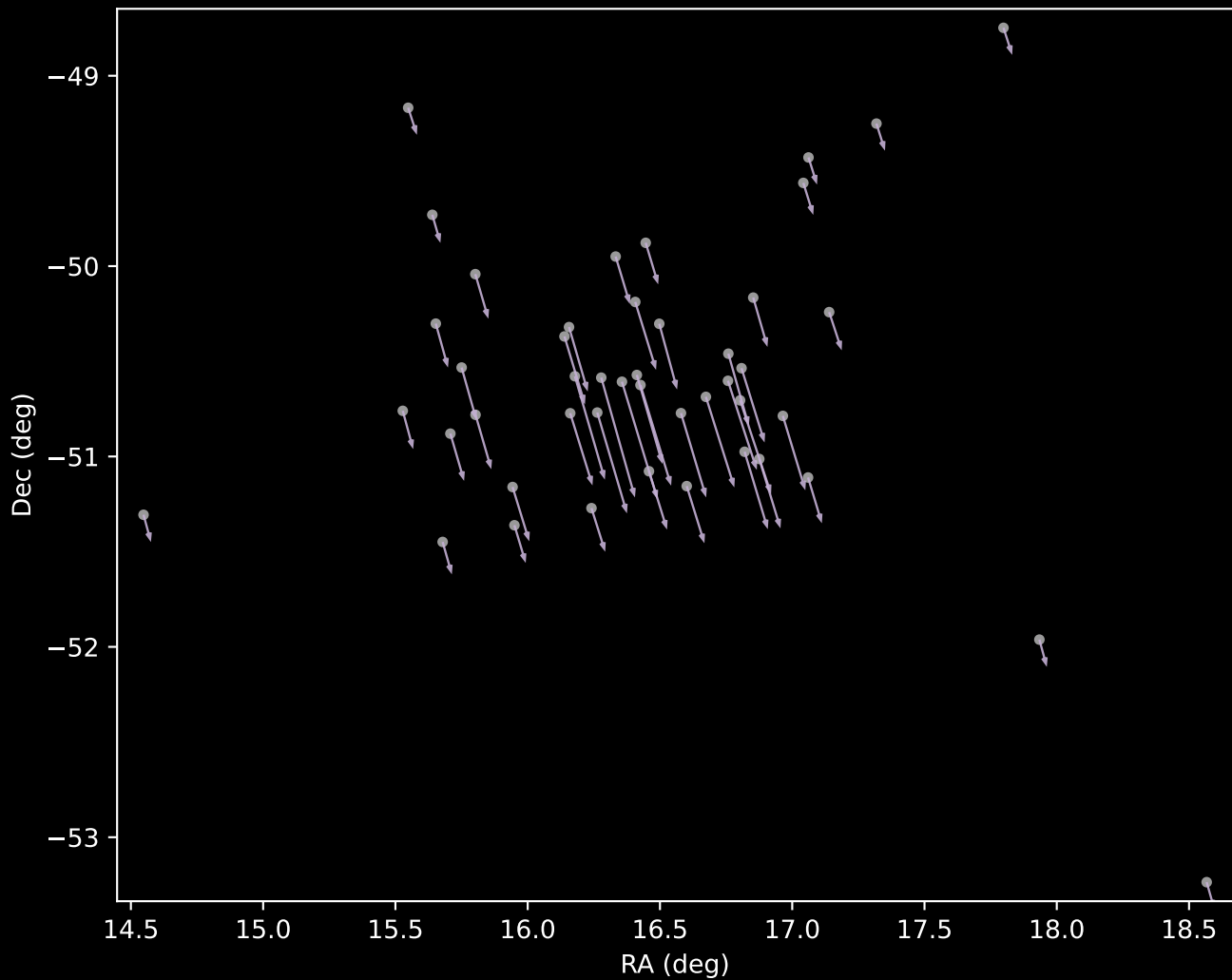
Gaia DR3 Cluster 9 Proper Motion Vectors (n=46)
