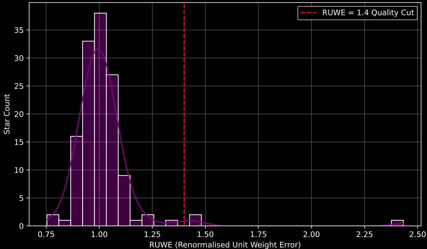
Gaia Cluster: [Markarian_38] RUWE Distribution (n= 133)
