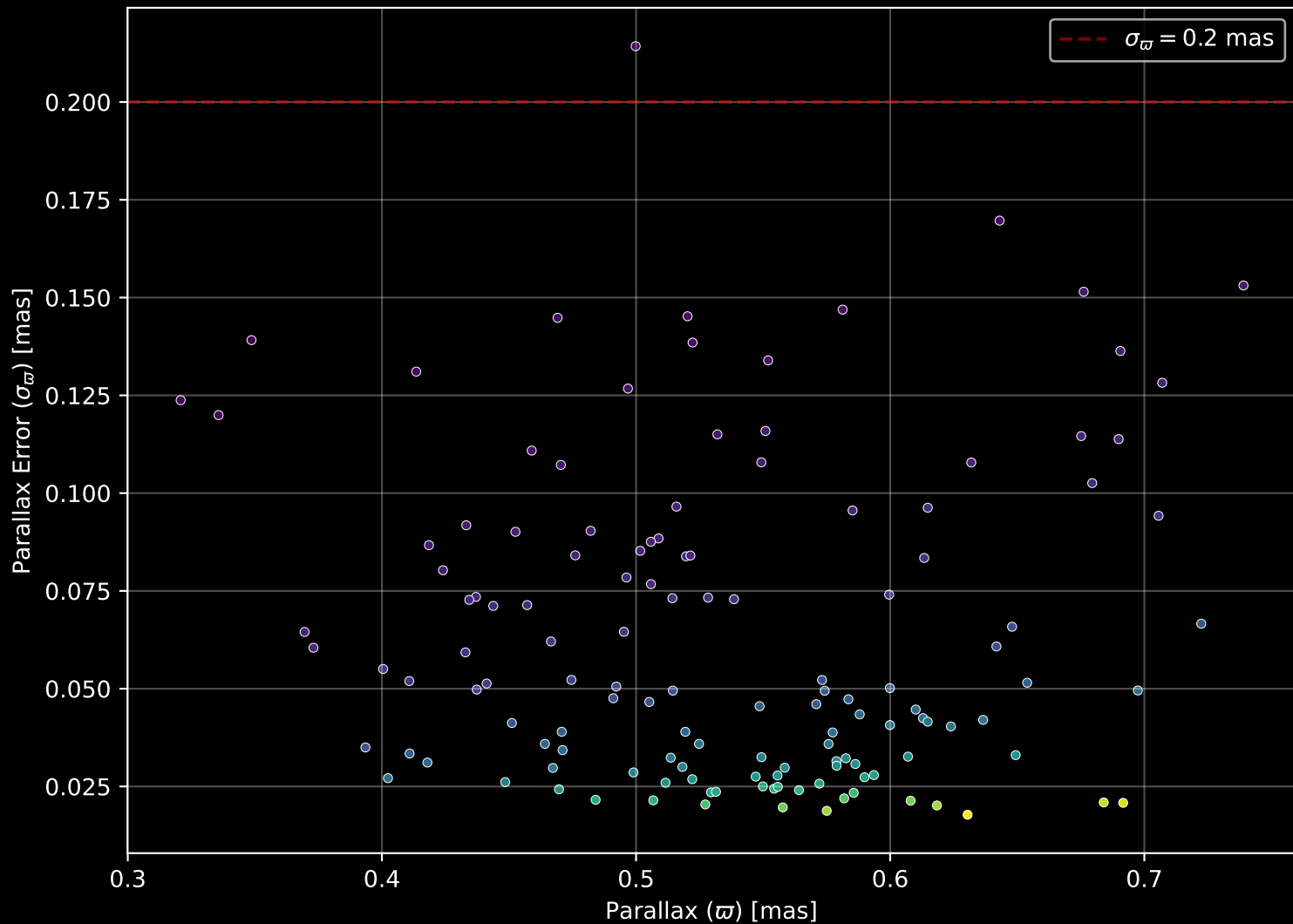
Gaia Cluster: [Markarian_38] Parallax Quality (n= 134)
