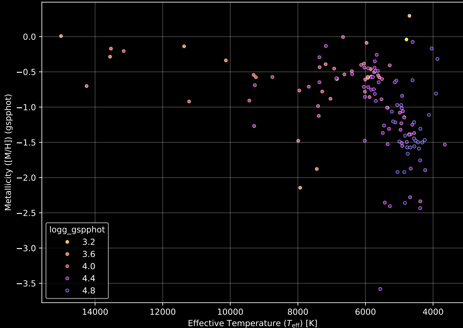
Gaia Cluster: [Markarian_38] Stellar Population Parameters (n= 134)
