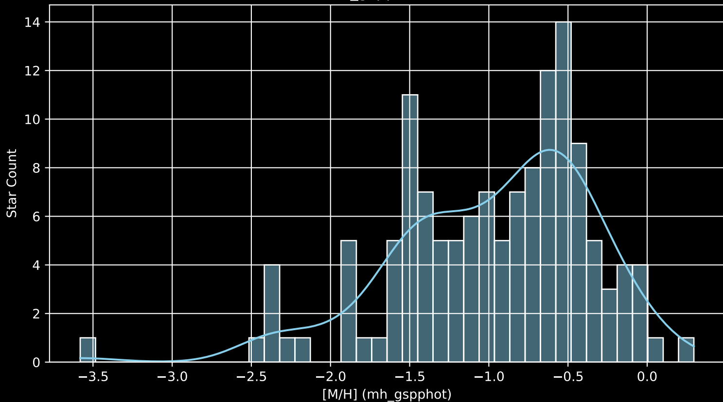
Gaia Cluster: [Markarian_38 [M/H] (mh_gspphot) (n= 134)
