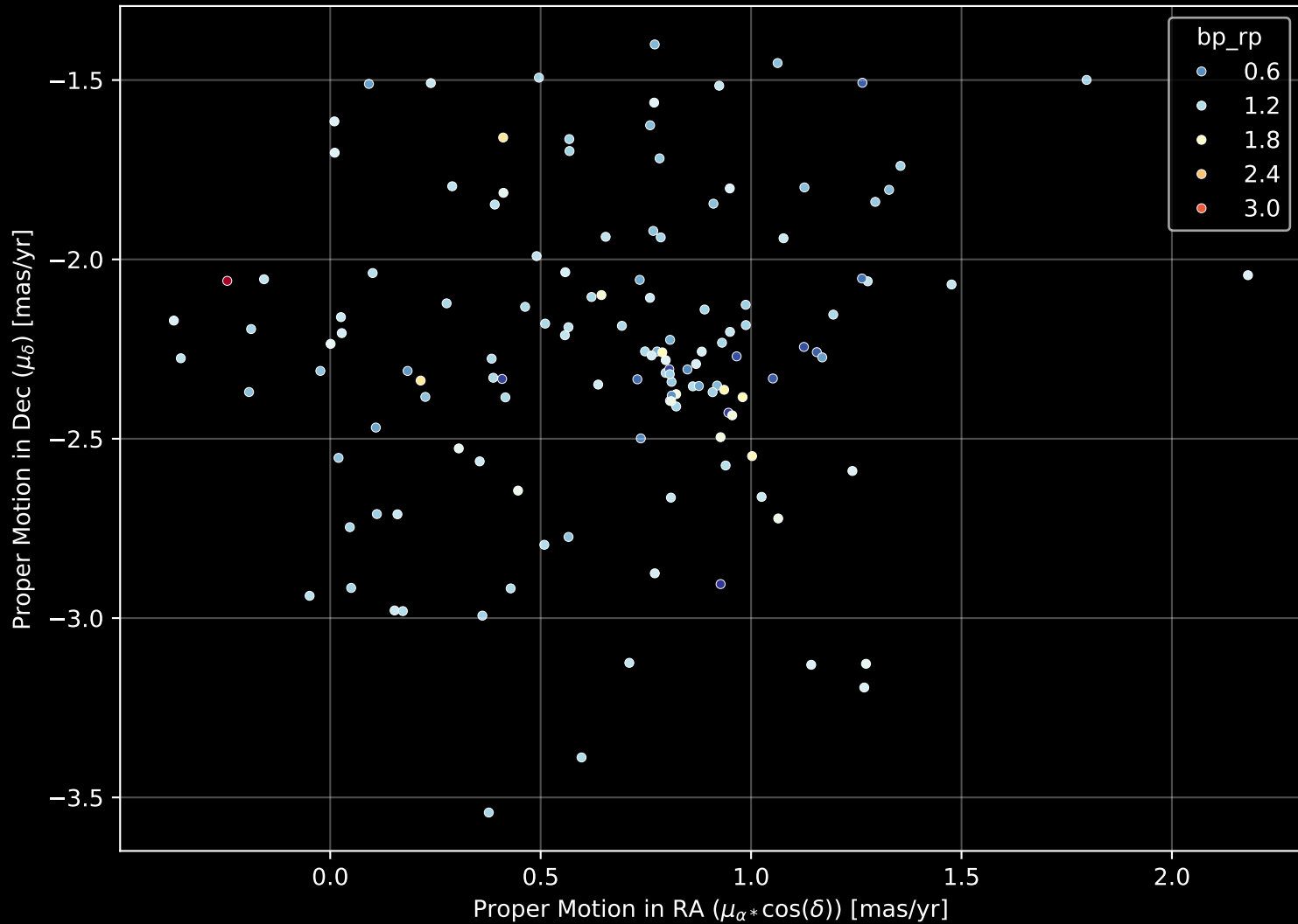
Gaia Cluster: [Markarian_38] Proper Motion Diagram (n= 134)
