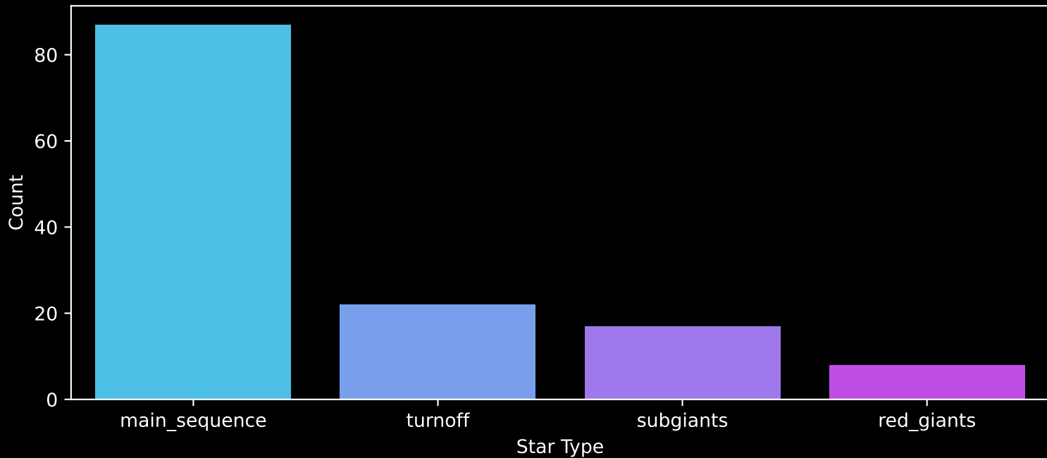
Gaia Cluster: [Markarian_38] Count plot of Star Type
