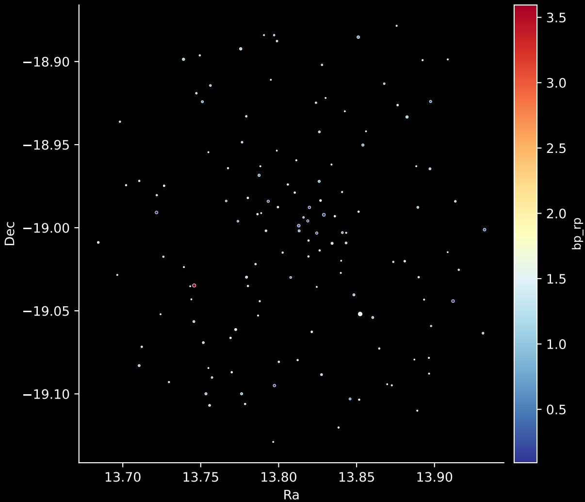
Gaia Cluster: [Markarian_38] Stars: 134
