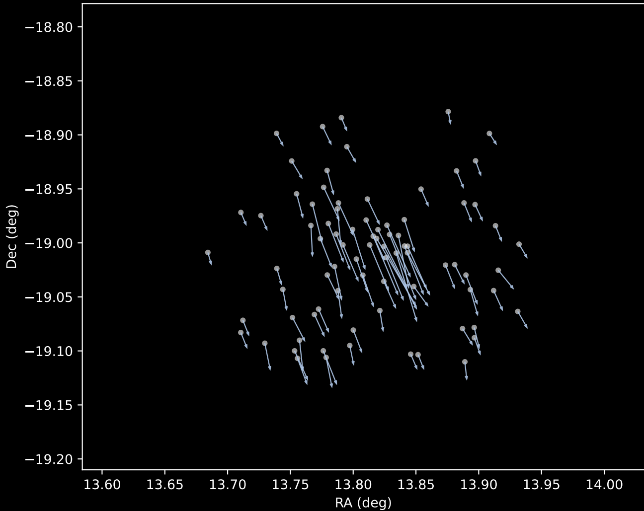
Gaia DR3 Cluster 1 Proper Motion Vectors (n=81)
