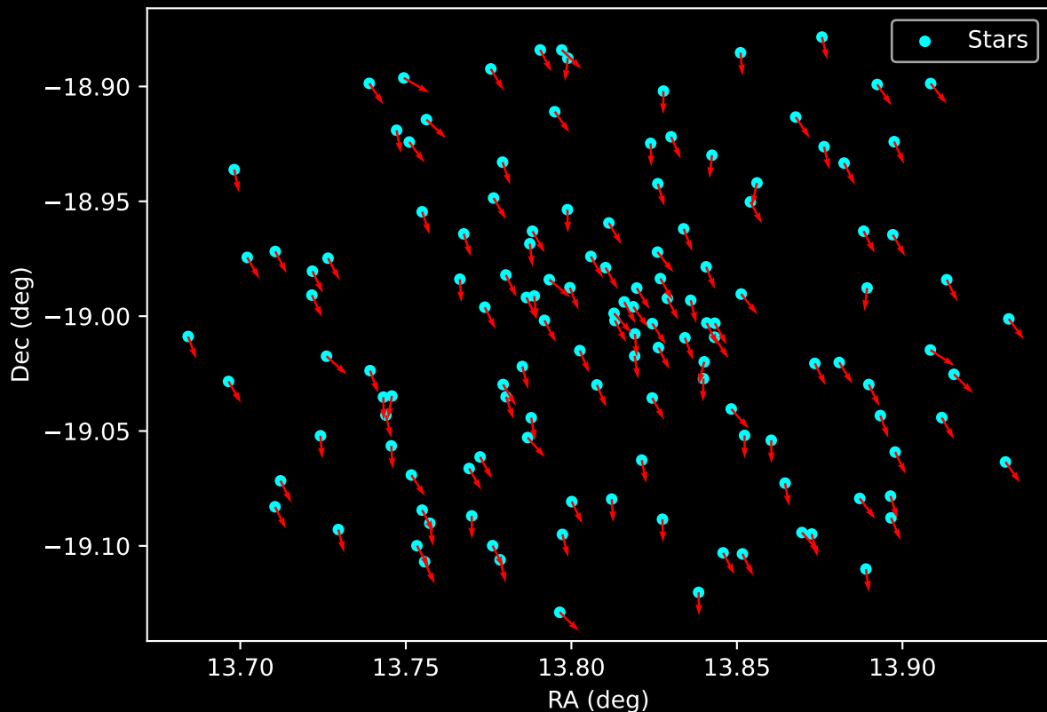
Gaia Cluster: [Markarian_38] Proper Motion Vectors for Gaia Star Field (n= 134)
