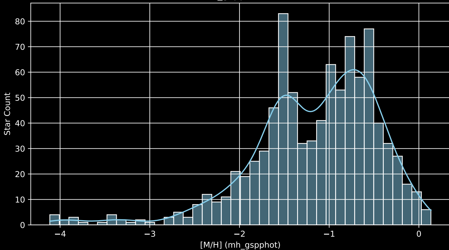
Gaia Cluster: [Melotte_101 [M/H] (mh_gspphot) (n= 912)
