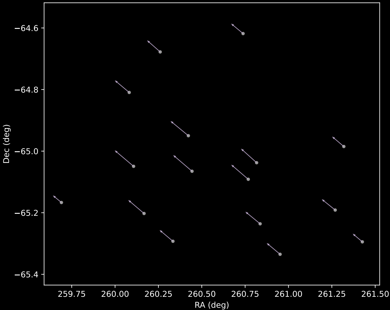
Gaia DR3 Cluster 9 Proper Motion Vectors (n=16)
