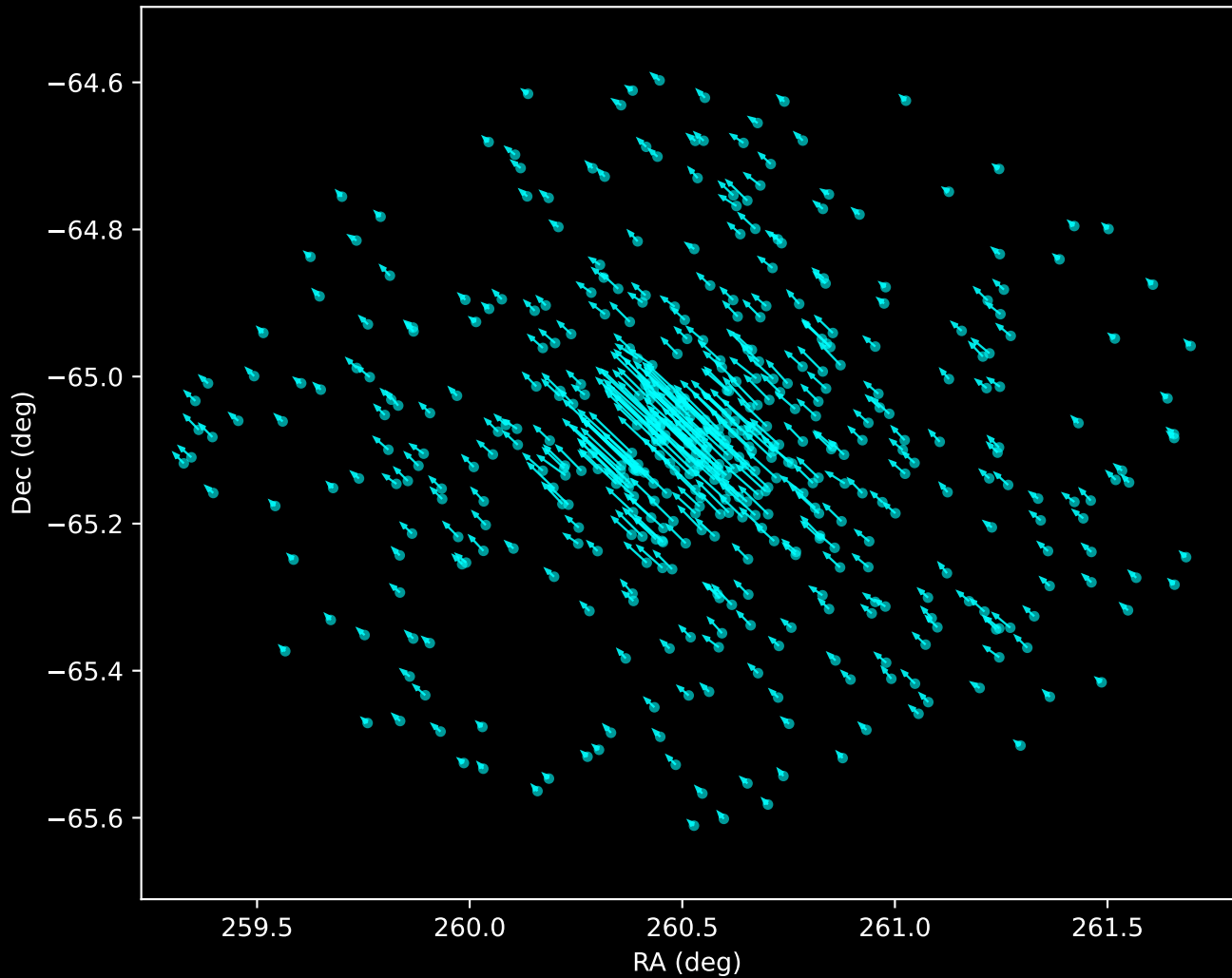
Gaia DR3 Noise Stream Proper Motion Vectors (n=461)
