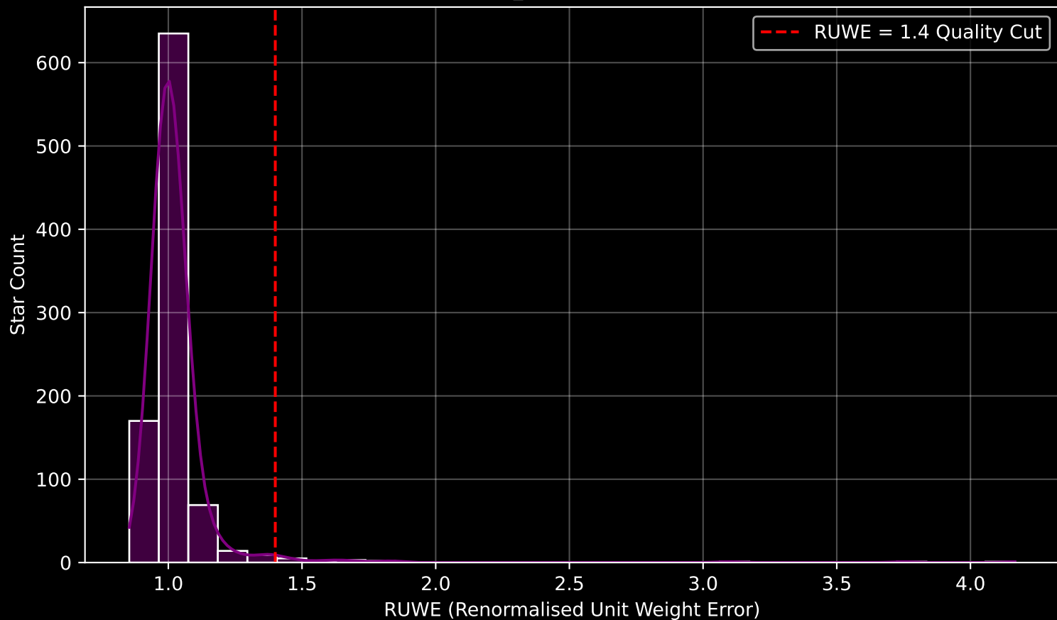
Gaia Cluster: [Melotte_101] RUWE Distribution (n= 912)
