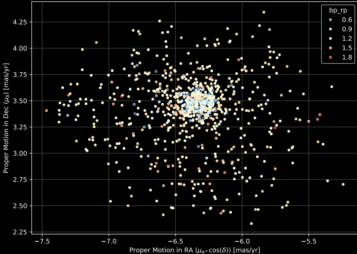
Gaia Cluster: [Melotte_101] Proper Motion Diagram (n= 912)
