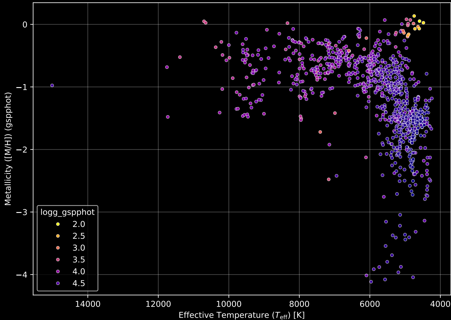
Gaia Cluster: [Melotte_101] Stellar Population Parameters (n= 912)
