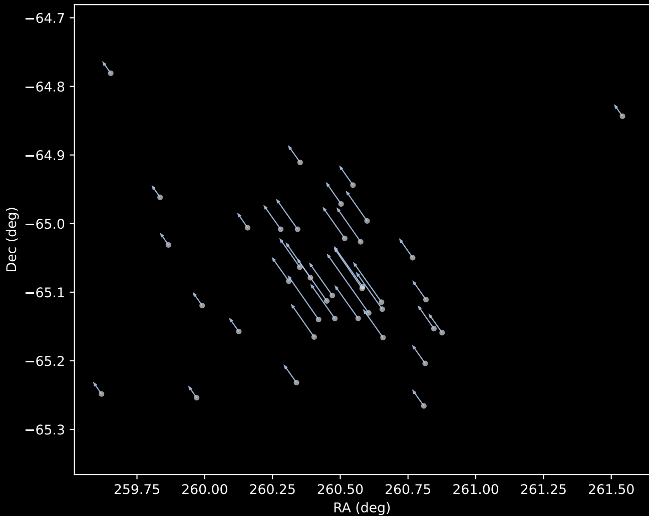
Gaia DR3 Cluster 41 Proper Motion Vectors (n=39)
