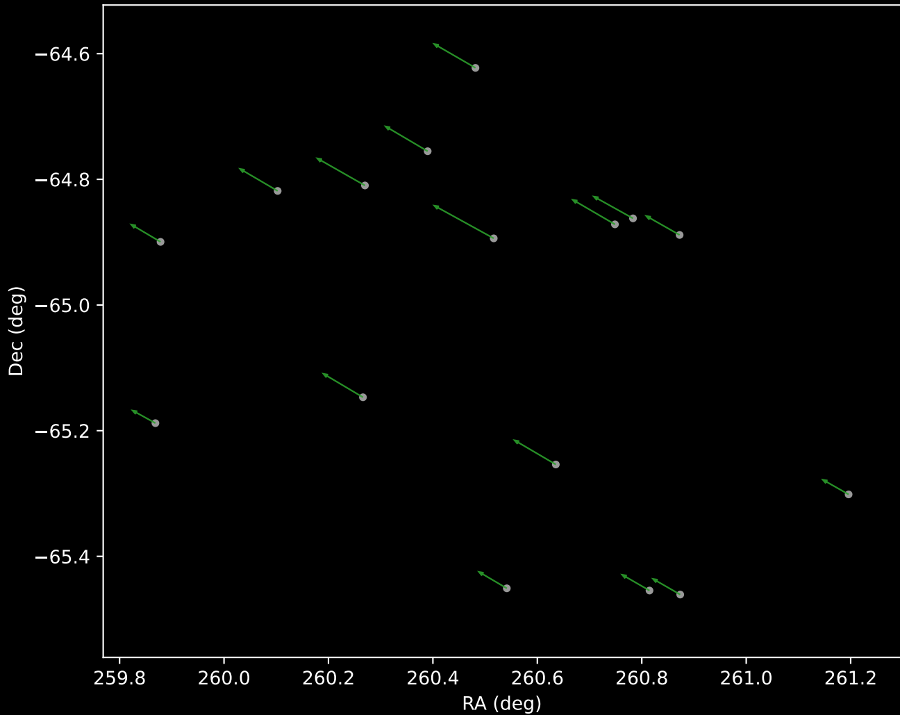
Gaia DR3 Cluster 4 Proper Motion Vectors (n=16)
