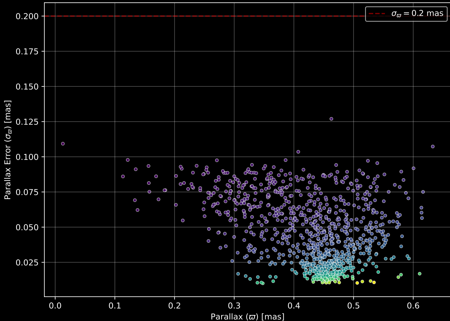
Gaia Cluster: [Melotte_101] Parallax Quality (n= 912)
