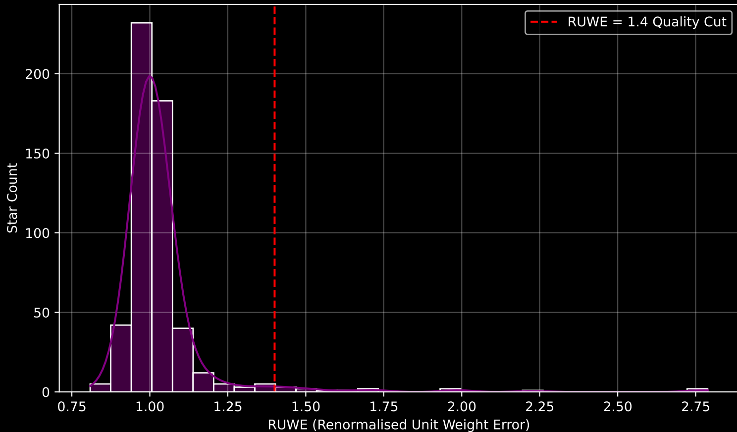
Gaia Cluster: [Melotte_105] RUWE Distribution (n= 541)
