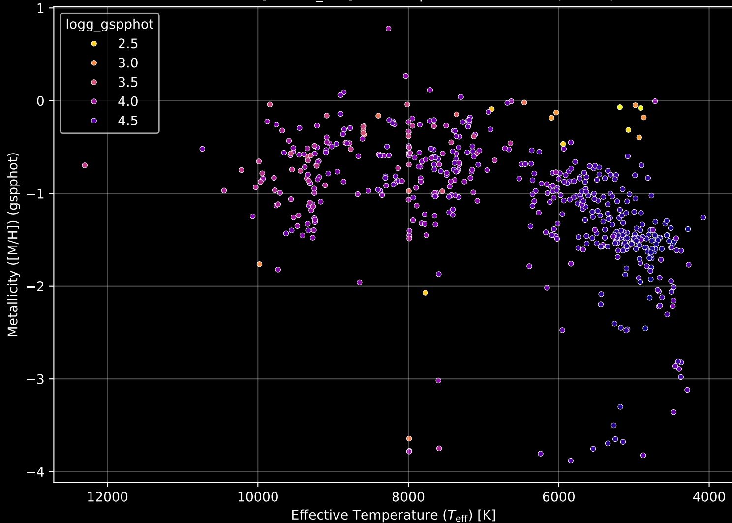
Gaia Cluster: [Melotte_105] Stellar Population Parameters (n= 542)
