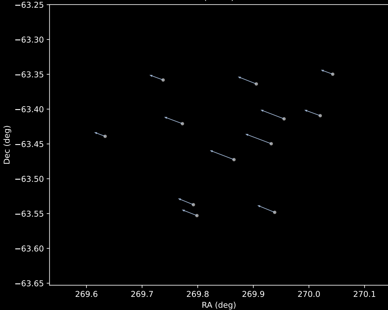
Gaia DR3 Cluster 1 Proper Motion Vectors (n=12)
