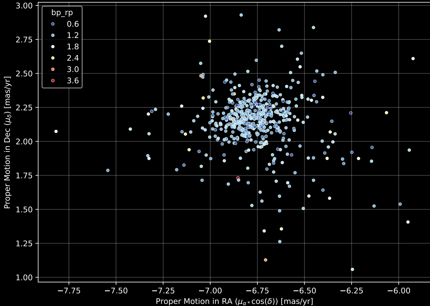
Gaia Cluster: [Melotte_105] Proper Motion Diagram (n= 542)
