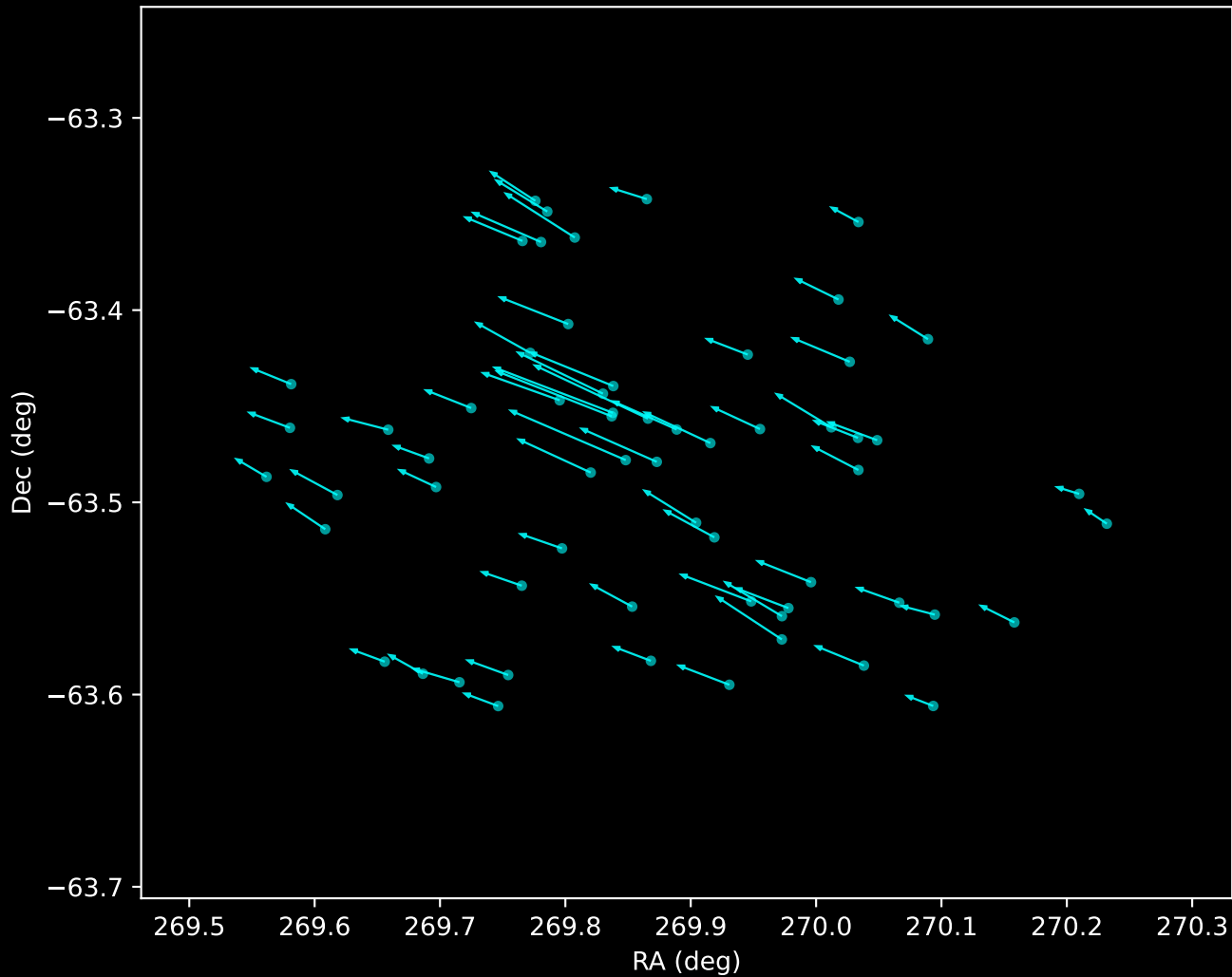
Gaia DR3 Noise Stream Proper Motion Vectors (n=62)
