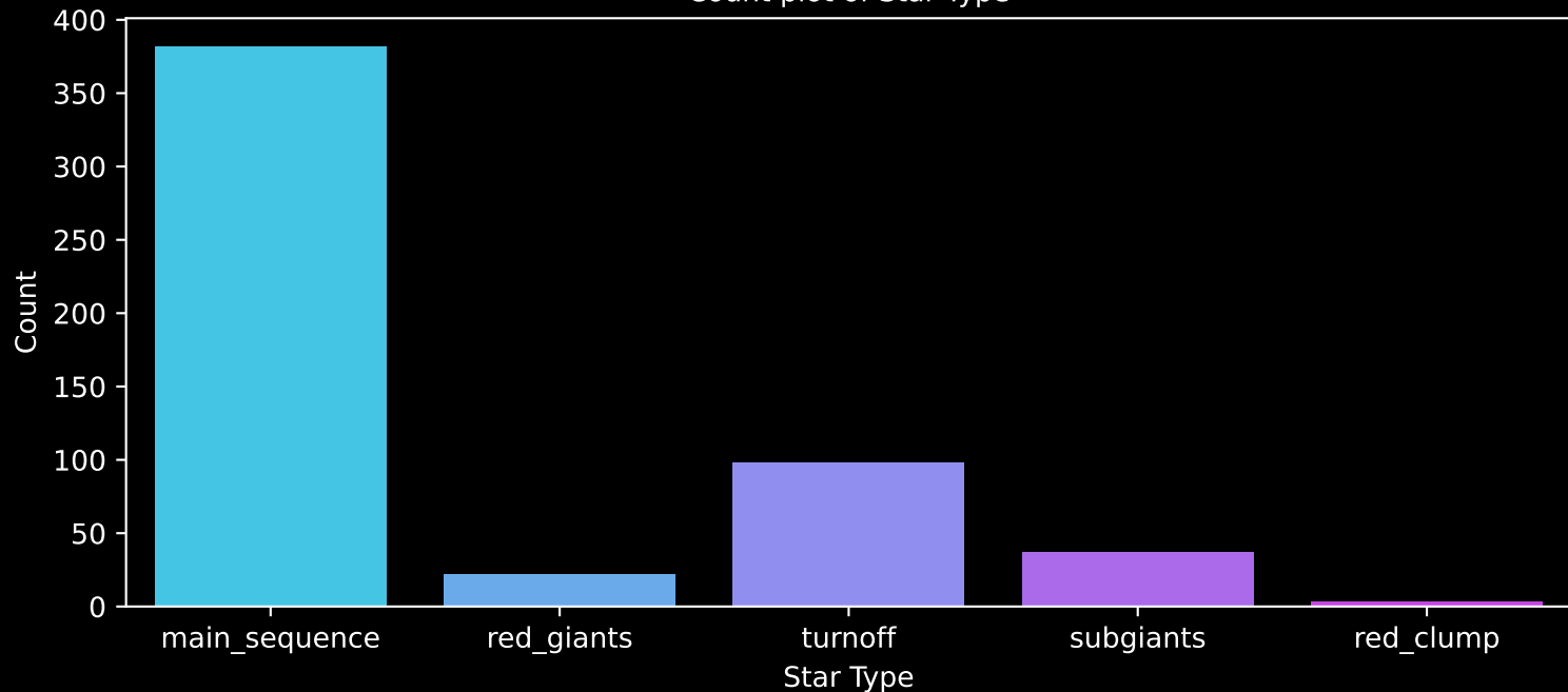
Gaia Cluster: [Melotte_105] Count plot of Star Type
