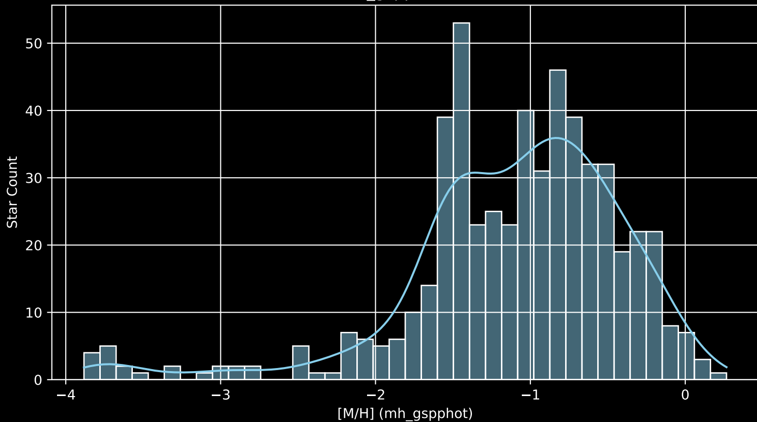
Gaia Cluster: [Melotte_105 [M/H] (mh_gspphot) (n= 541)
