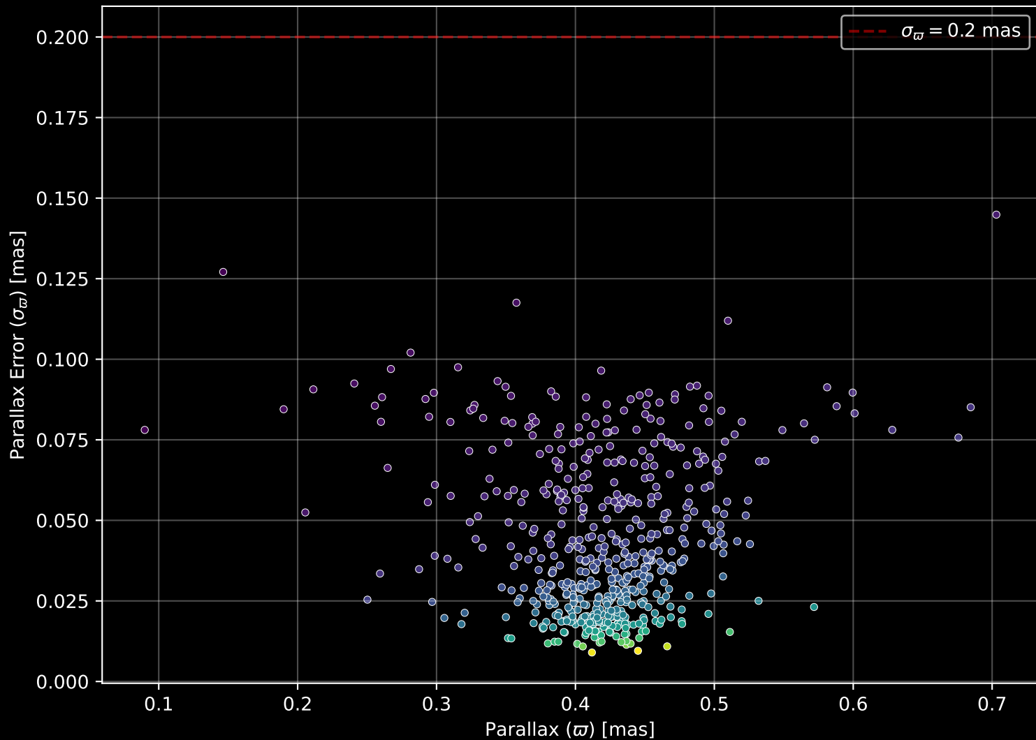
Gaia Cluster: [Melotte_105] Parallax Quality (n= 542)
