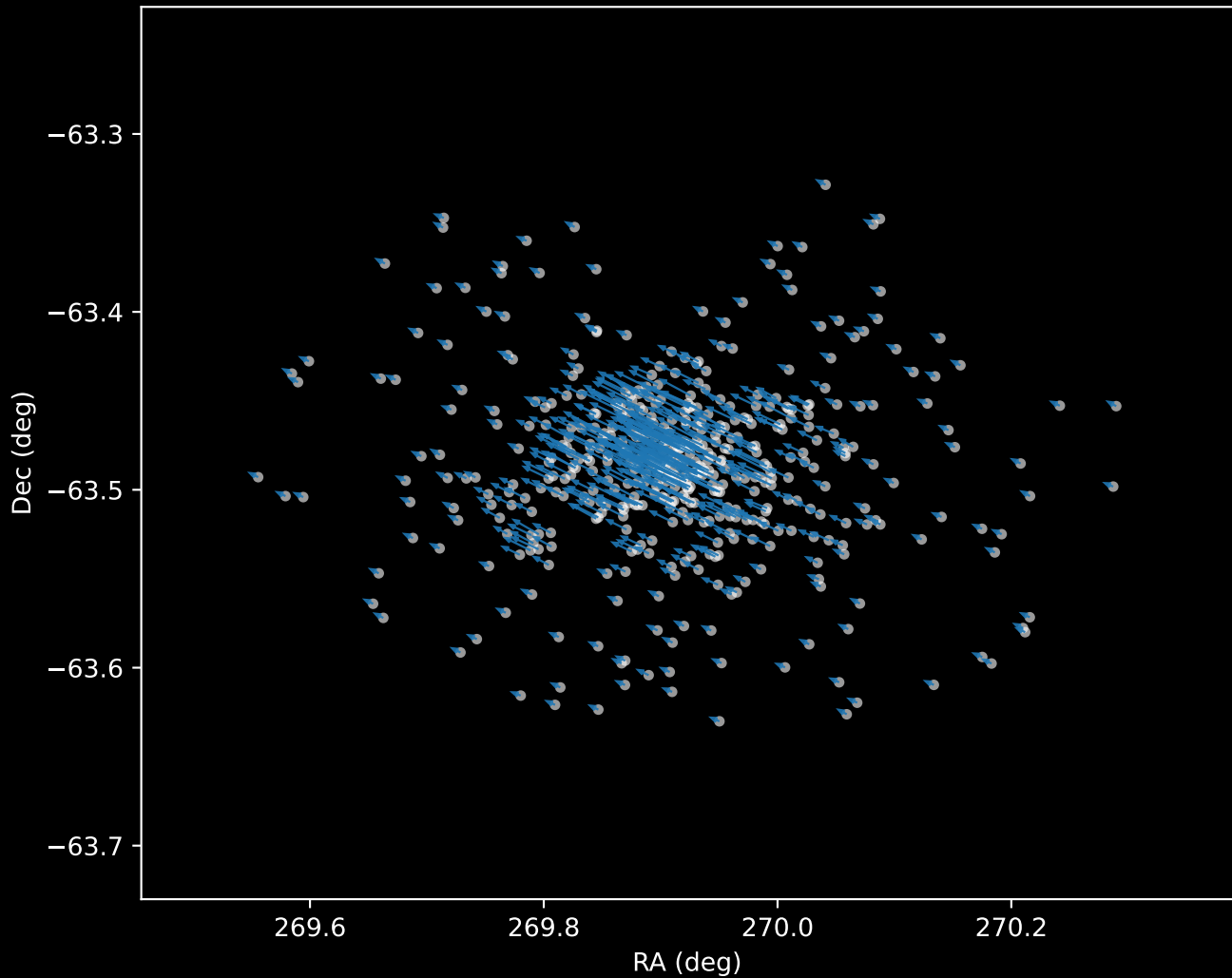
Gaia DR3 Cluster 0 Proper Motion Vectors (n=468)
