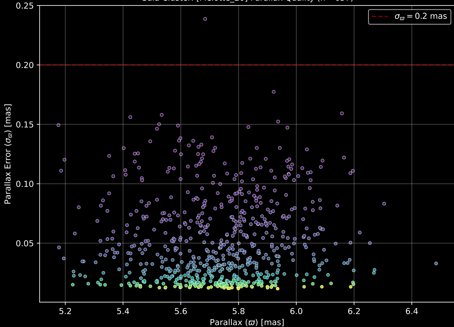
Gaia Cluster: [Melotte_20] Parallax Quality (n= 657)
