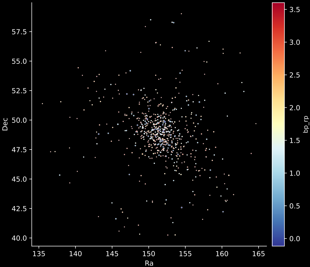
Gaia Cluster: [Melotte_20] Stars: 657
