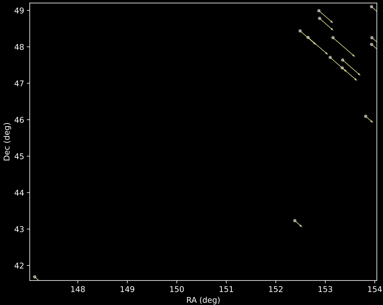
Gaia DR3 Cluster 17 Proper Motion Vectors (n=14)
