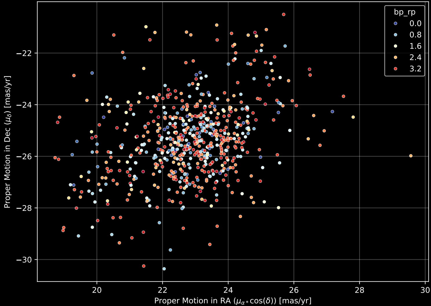
Gaia Cluster: [Melotte_20] Proper Motion Diagram (n= 657)
