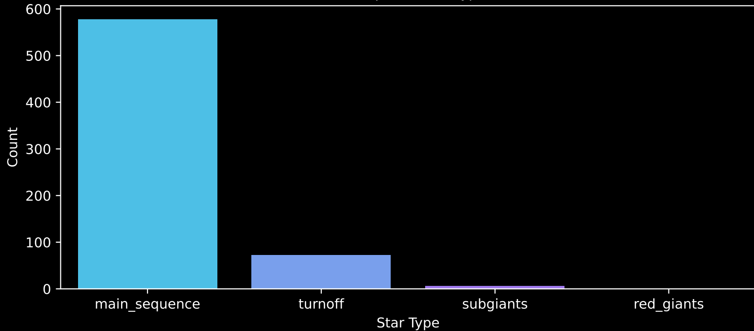
Gaia Cluster: [Melotte_20] Count plot of Star Type
