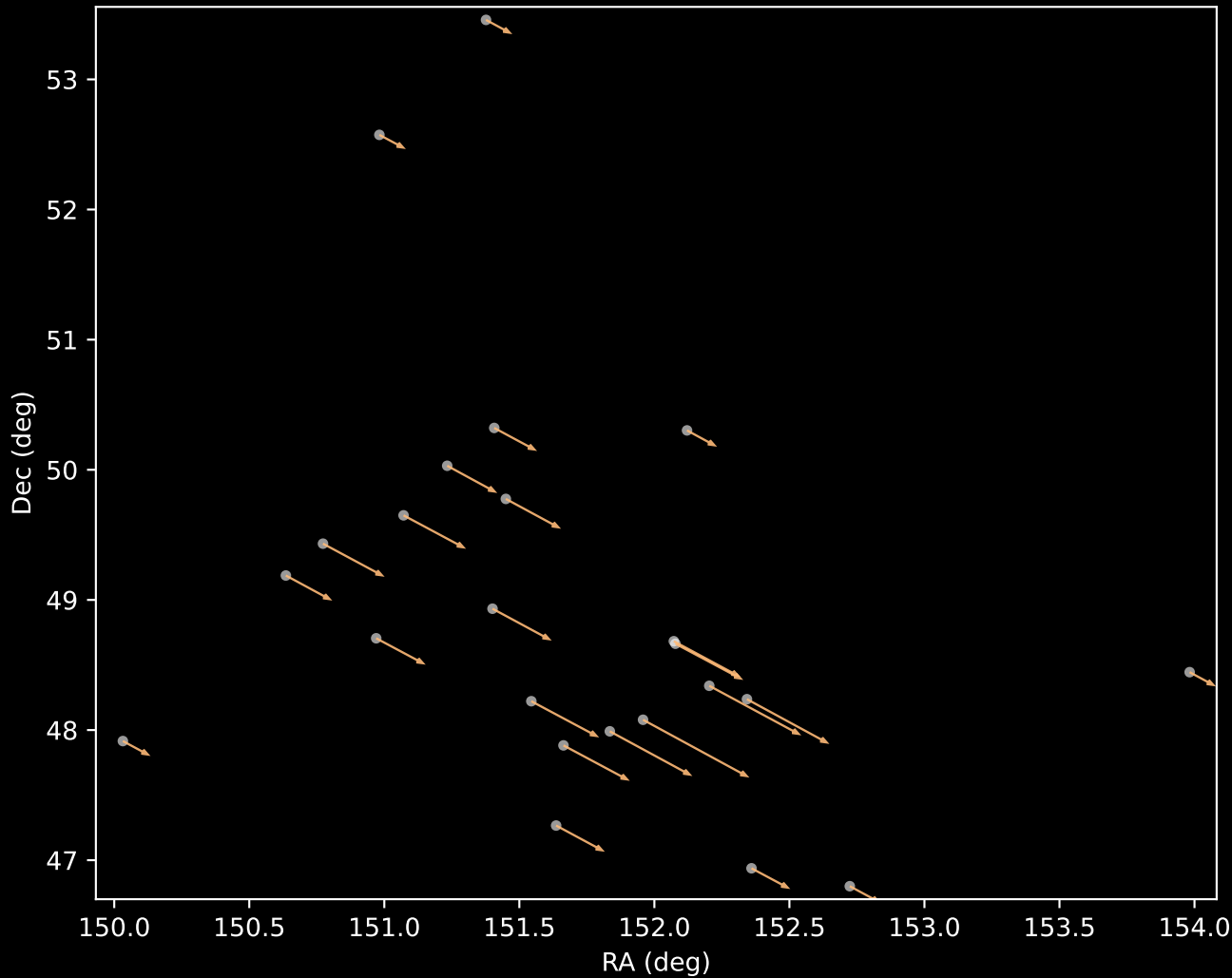
Gaia DR3 Cluster 23 Proper Motion Vectors (n=24)
