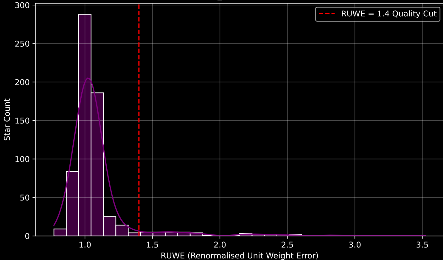
Gaia Cluster: [Melotte_20] RUWE Distribution (n= 652)
