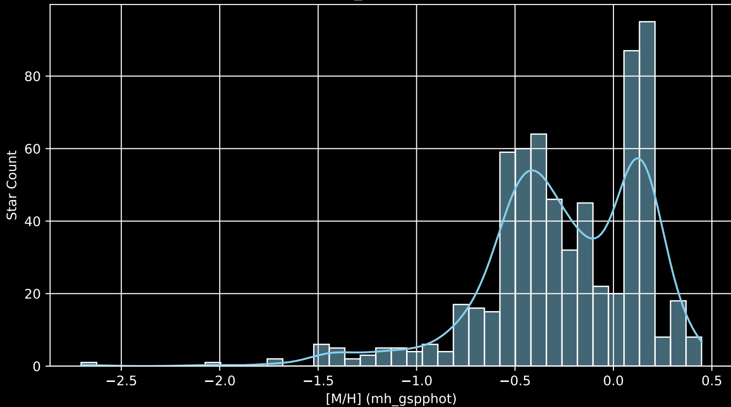
Gaia Cluster: [Melotte_20 [M/H] (mh_gspphot) (n= 656)
