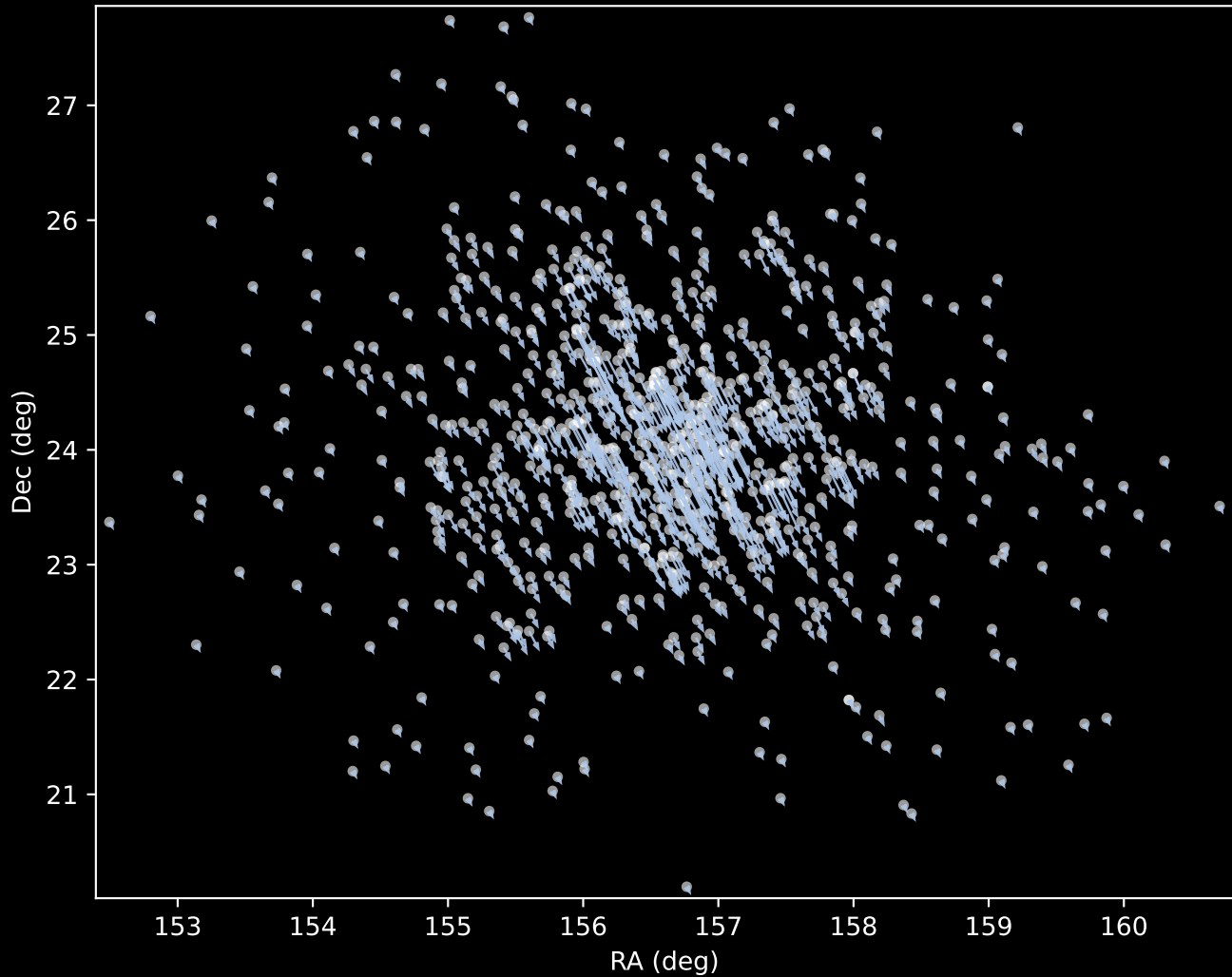
Gaia DR3 Cluster 1 Proper Motion Vectors (n=856)
