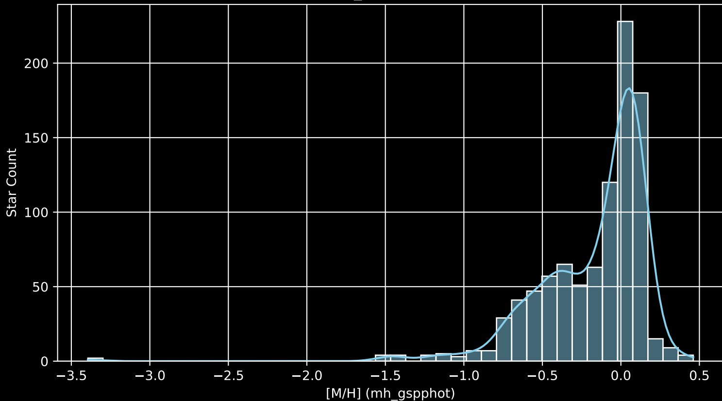
Gaia Cluster: [Melotte_22 [M/H] (mh_gspphot) (n= 945)
