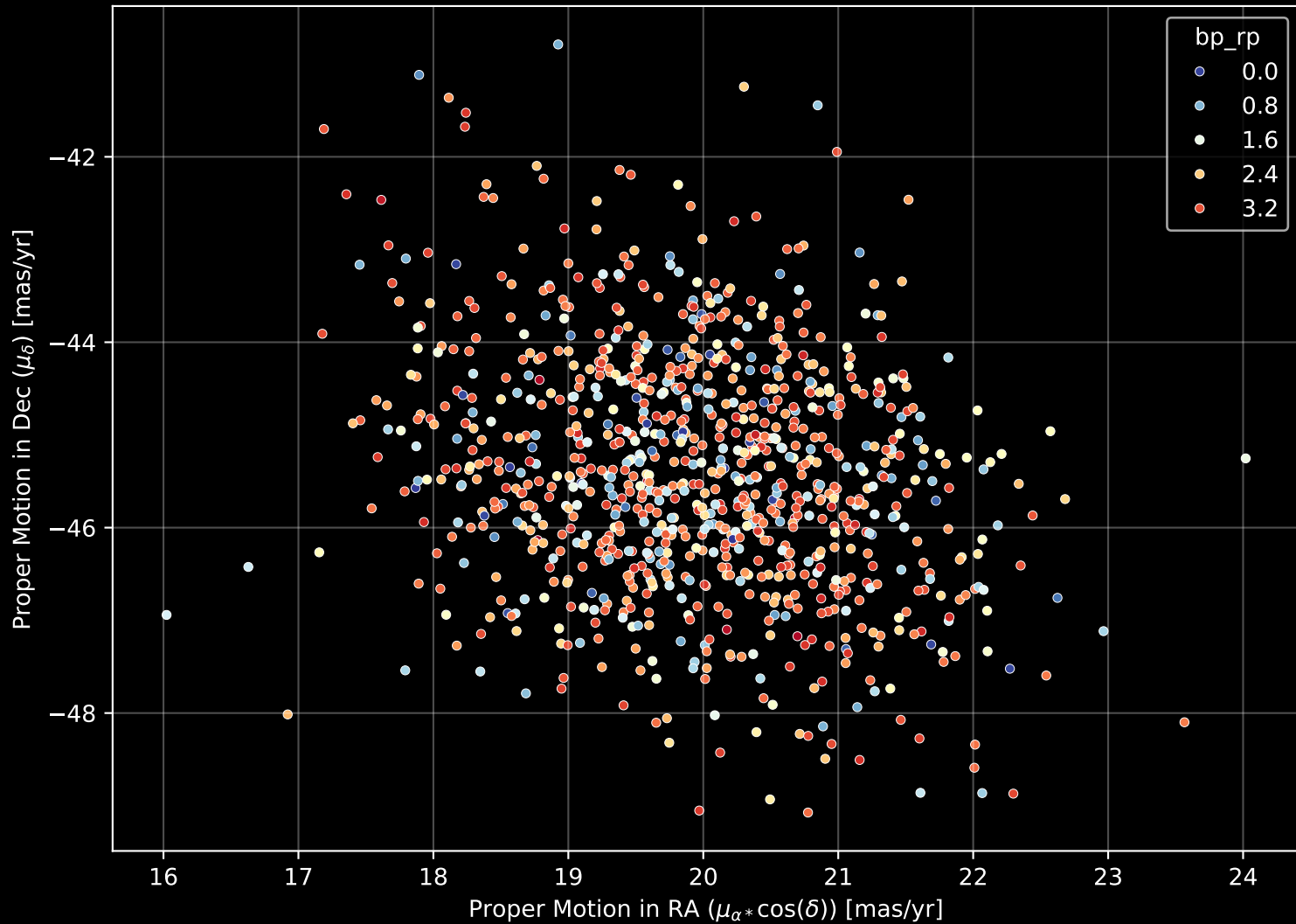
Gaia Cluster: [Melotte_22] Proper Motion Diagram (n= 947)
