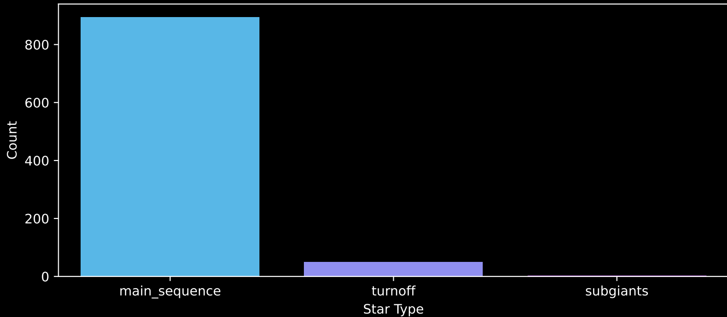
Gaia Cluster: [Melotte_22] Count plot of Star Type
