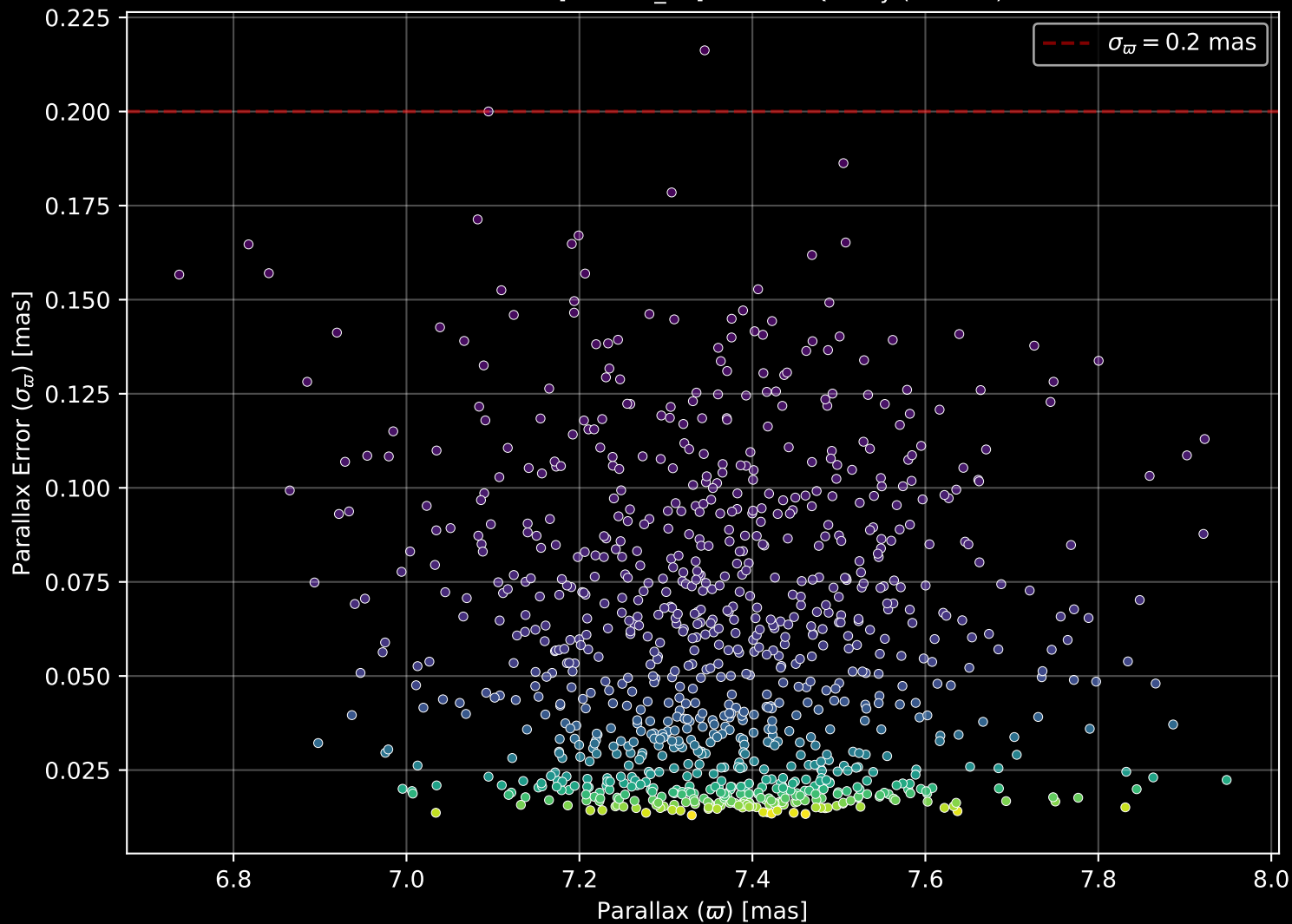
Gaia Cluster: [Melotte_22] Parallax Quality (n= 947)
