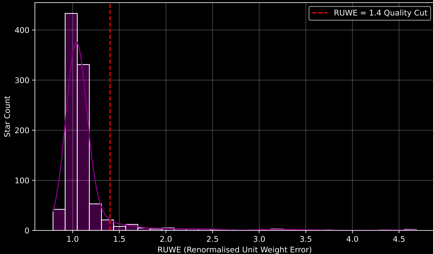
Gaia Cluster: [Melotte_22] RUWE Distribution (n= 938)
