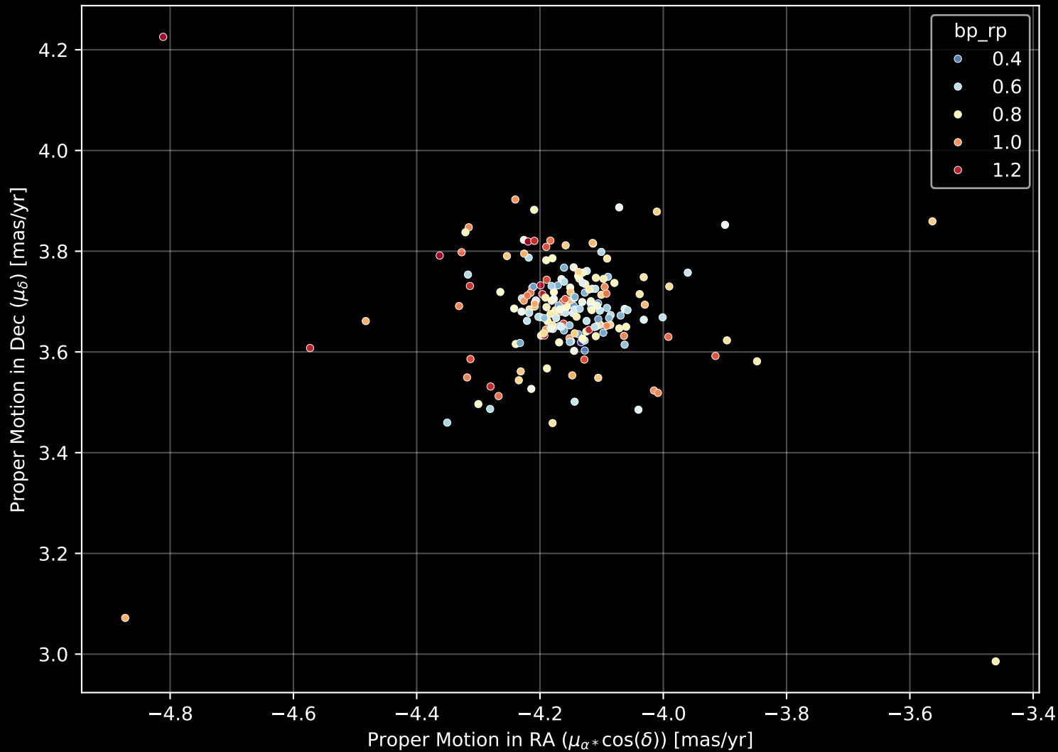
Gaia Cluster: [Melotte_72] Proper Motion Diagram (n= 194)
