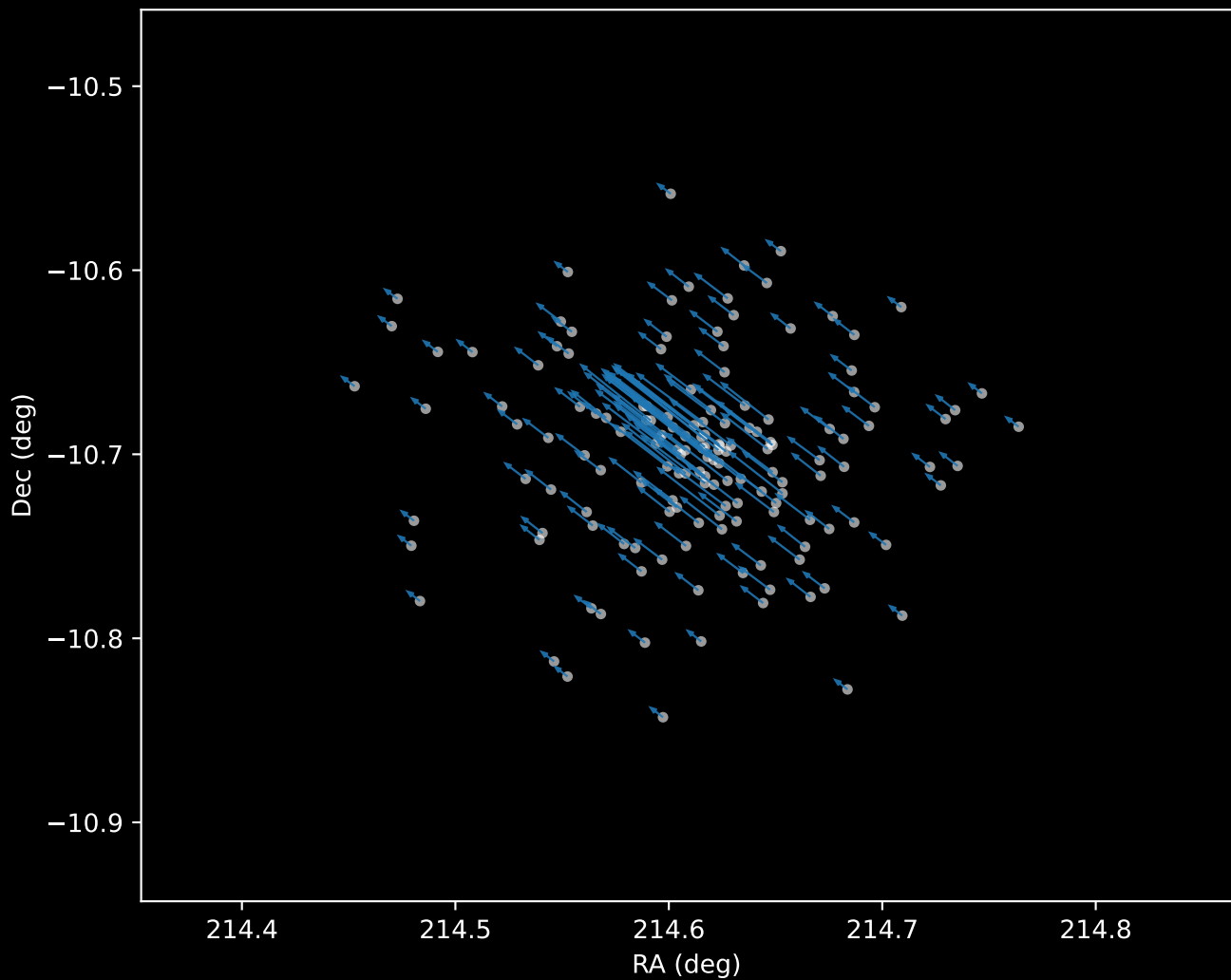
Gaia DR3 Cluster 0 Proper Motion Vectors (n=152)
