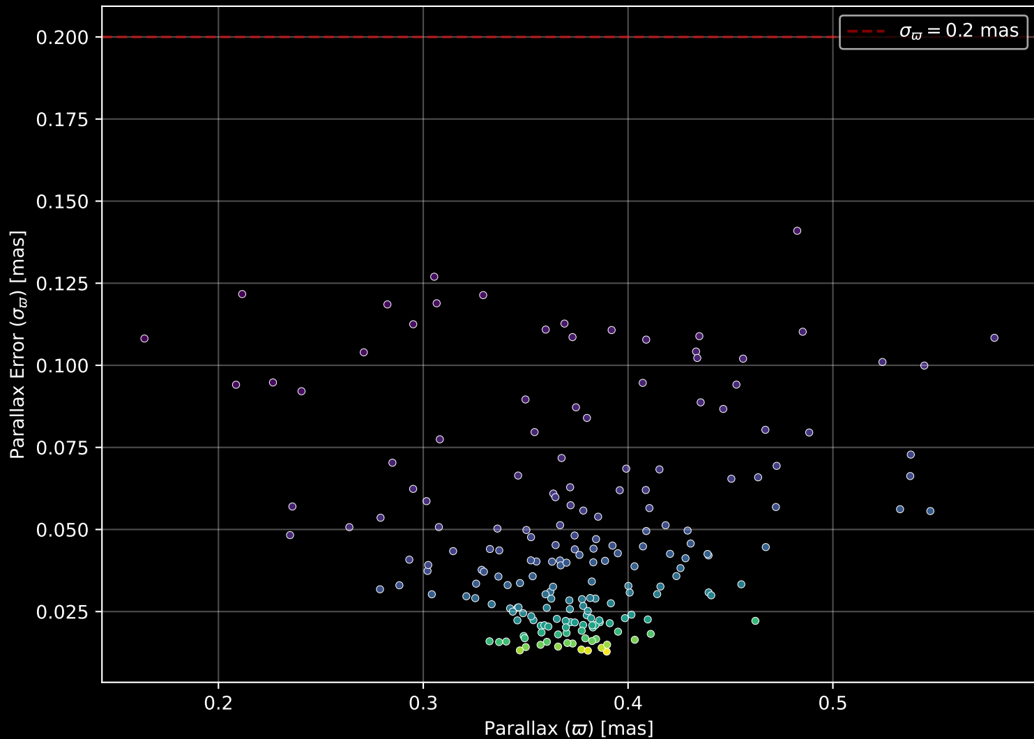
Gaia Cluster: [Melotte_72] Parallax Quality (n= 194)
