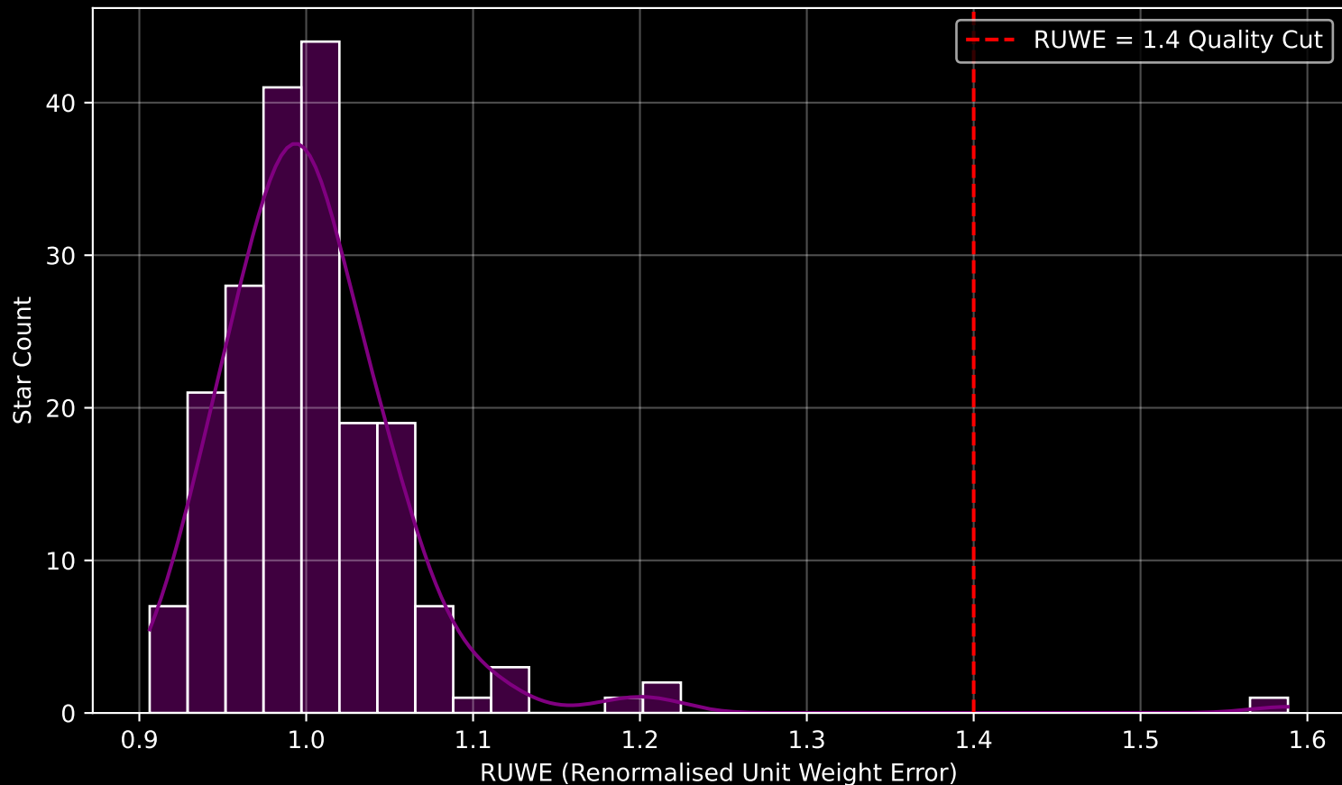
Gaia Cluster: [Melotte_72] RUWE Distribution (n= 194)
