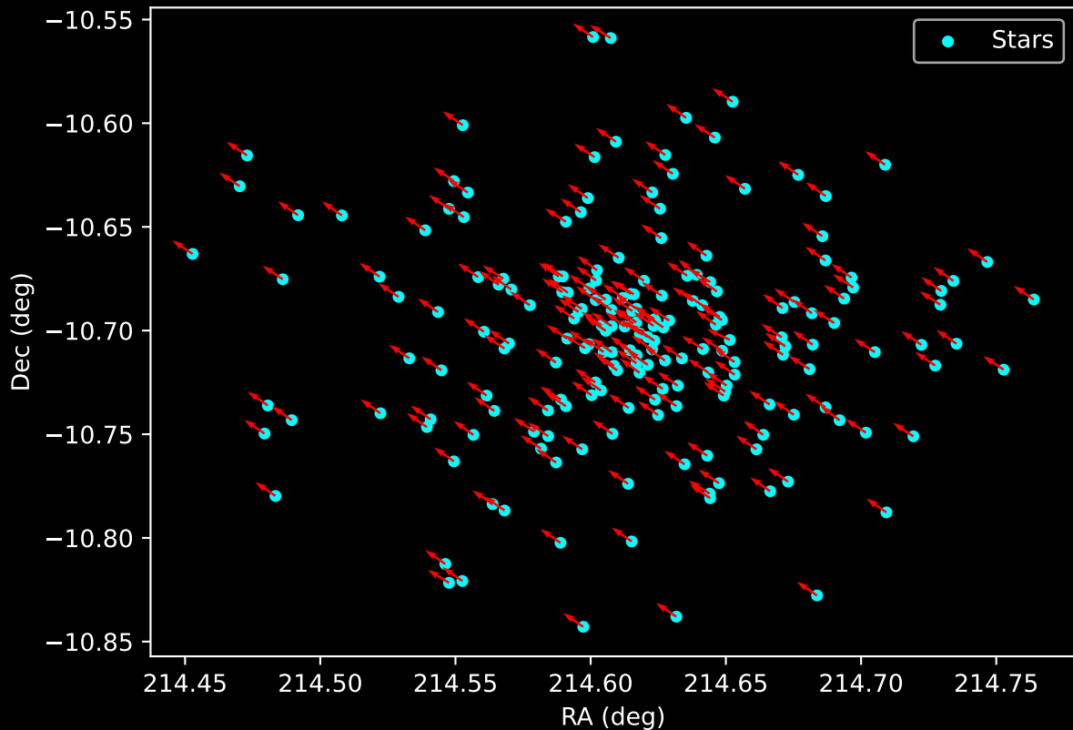
Gaia Cluster: [Melotte_72] Proper Motion Vectors for Gaia Star Field (n= 194)
