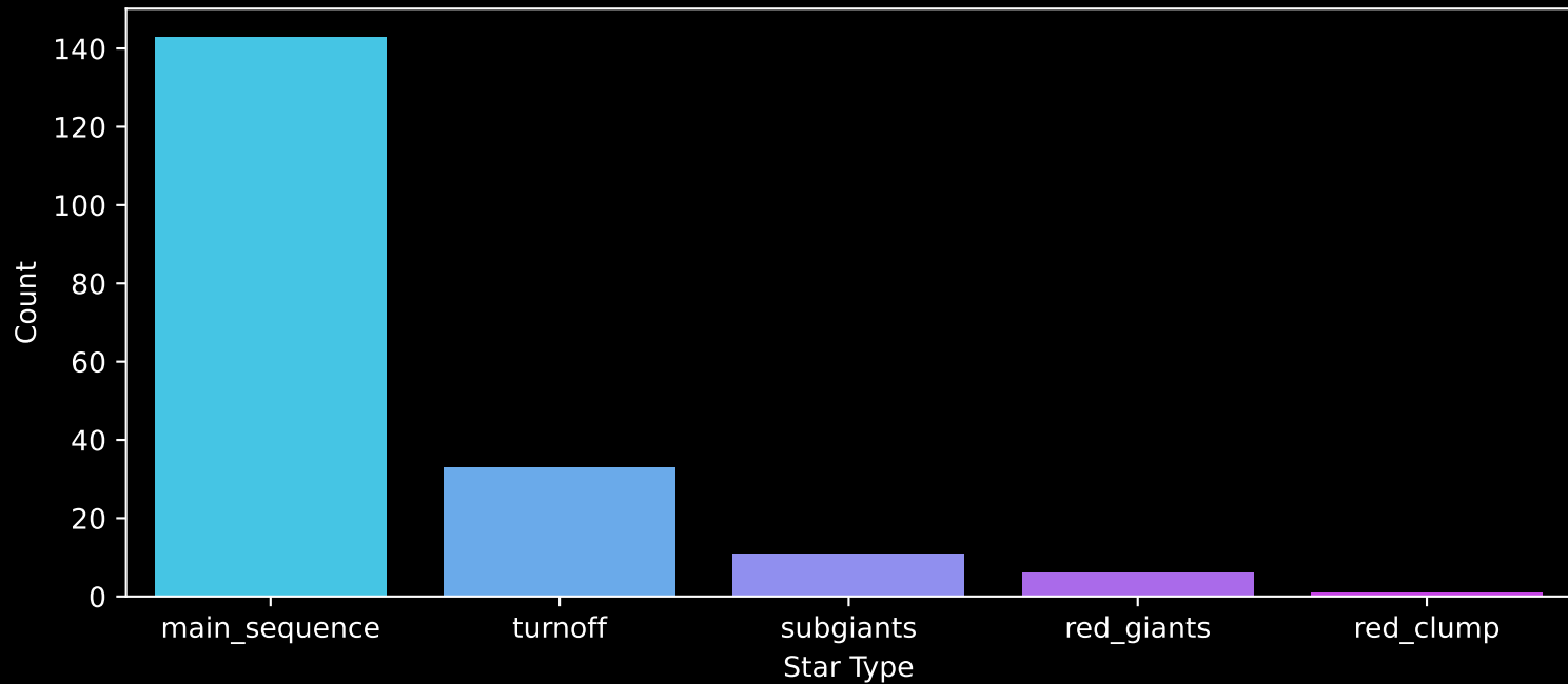
Gaia Cluster: [Melotte_72] Count plot of Star Type
