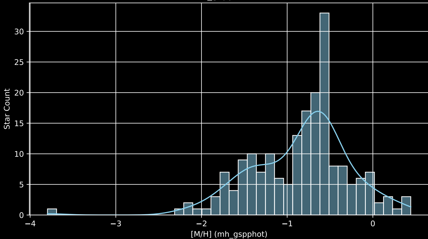
Gaia Cluster: [Melotte_72 [M/H] (mh_gspphot) (n= 193)
