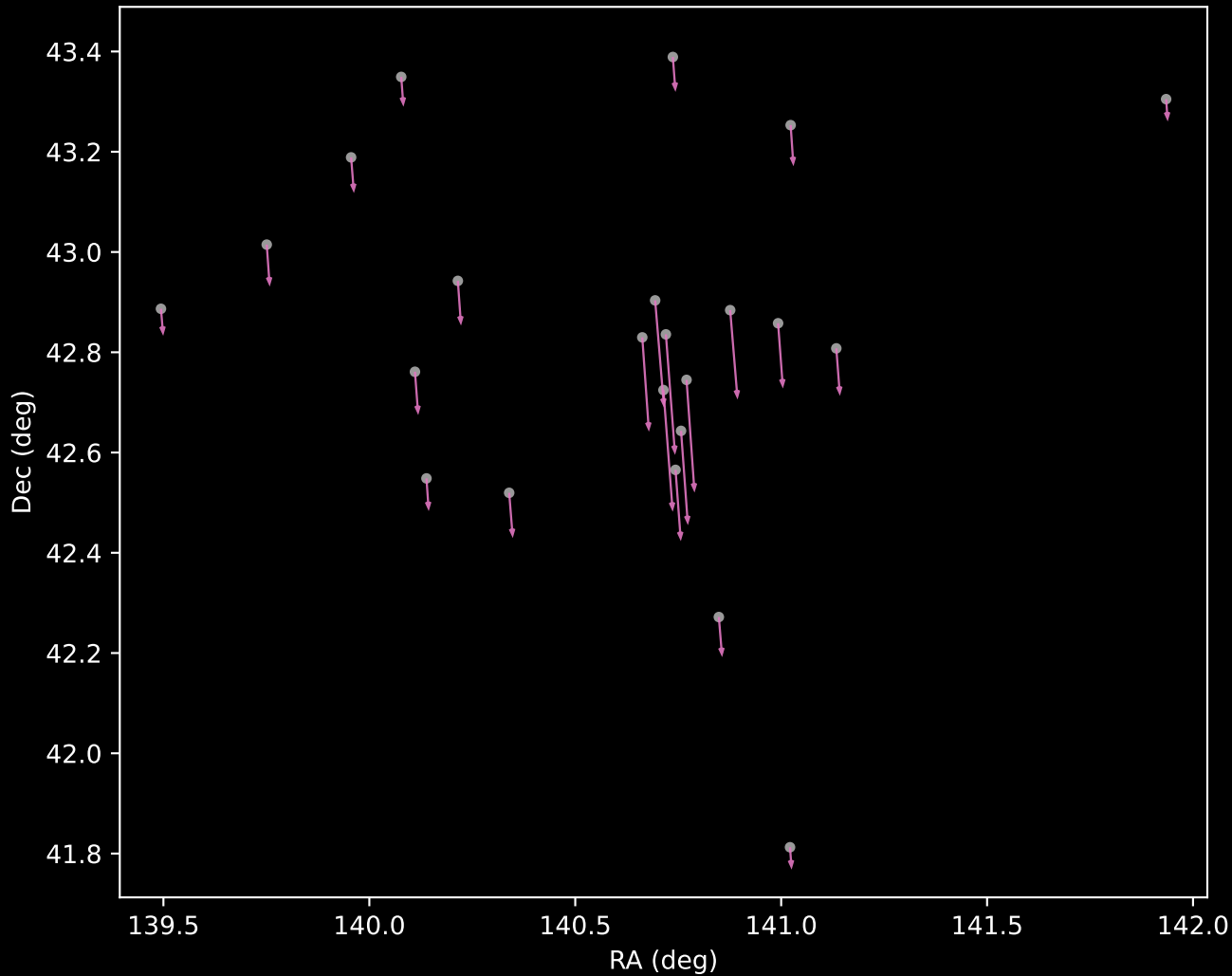
Gaia DR3 Cluster 32 Proper Motion Vectors (n=23)
