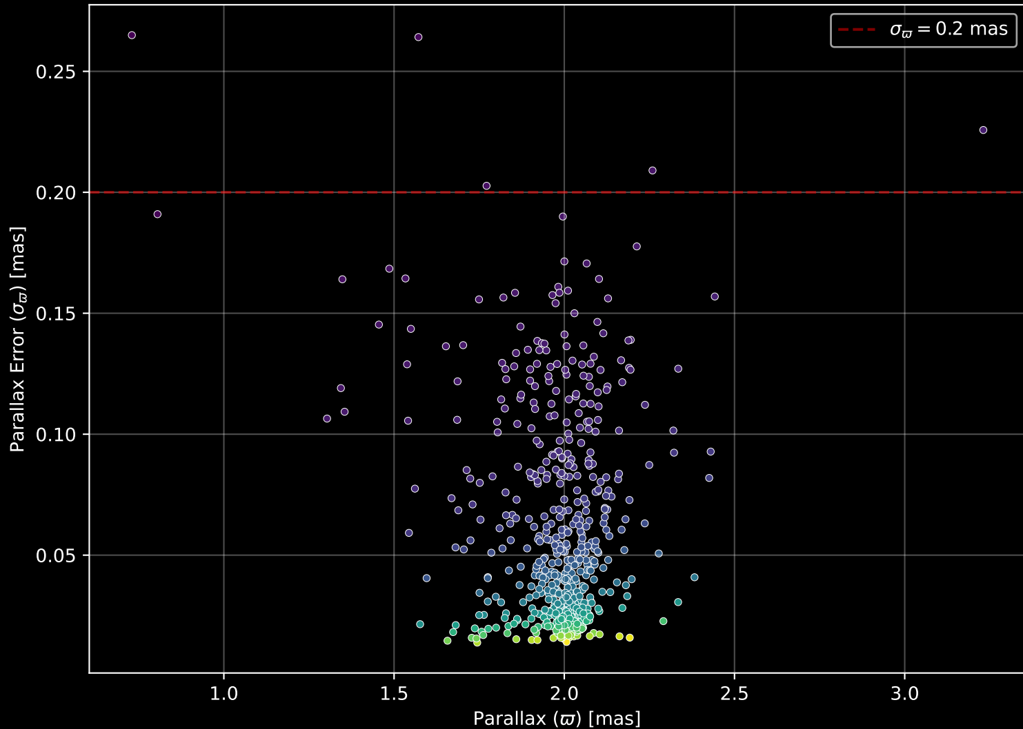
Gaia Cluster: [NGC_1039] Parallax Quality (n= 607)
