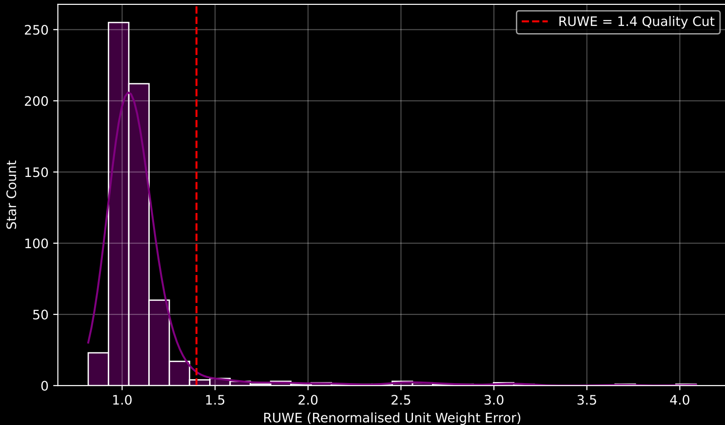
Gaia Cluster: [NGC_1039] RUWE Distribution (n= 601)
