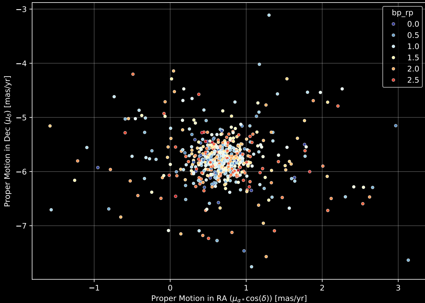
Gaia Cluster: [NGC_1039] Proper Motion Diagram (n= 607)
