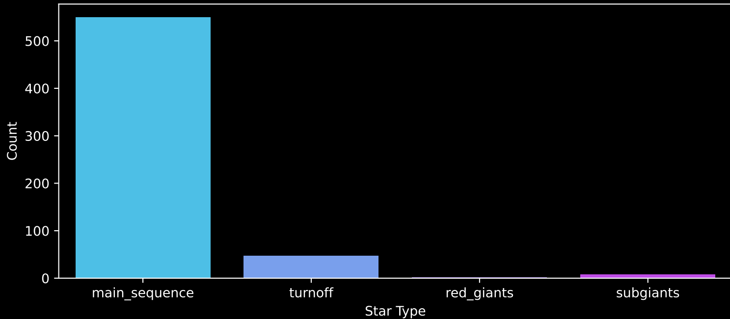
Gaia Cluster: [NGC_1039] Count plot of Star Type
