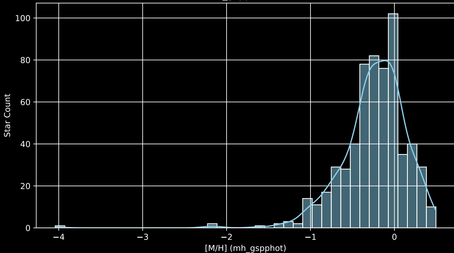
Gaia Cluster: [NGC_1039 [M/H] (mh_gspphot) (n= 602)
