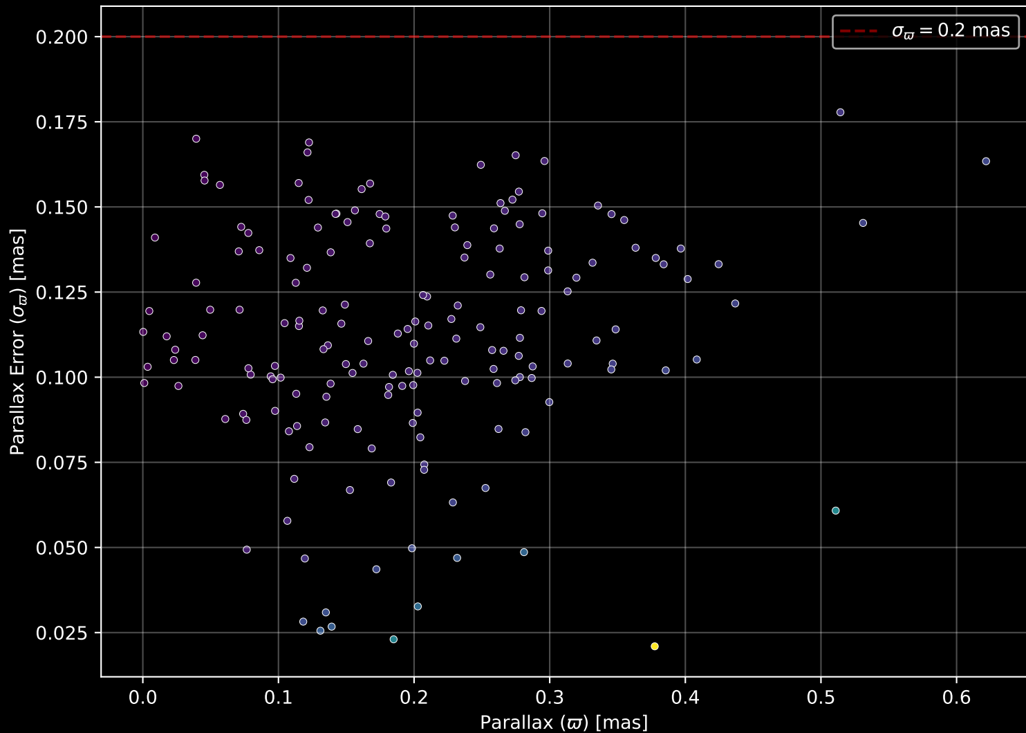
Gaia Cluster: [NGC_1193] Parallax Quality (n= 175)
