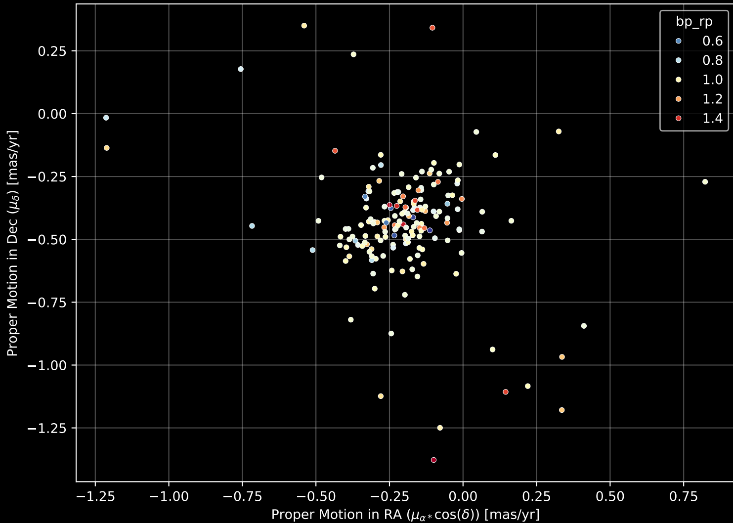
Gaia Cluster: [NGC_1193] Proper Motion Diagram (n= 175)
