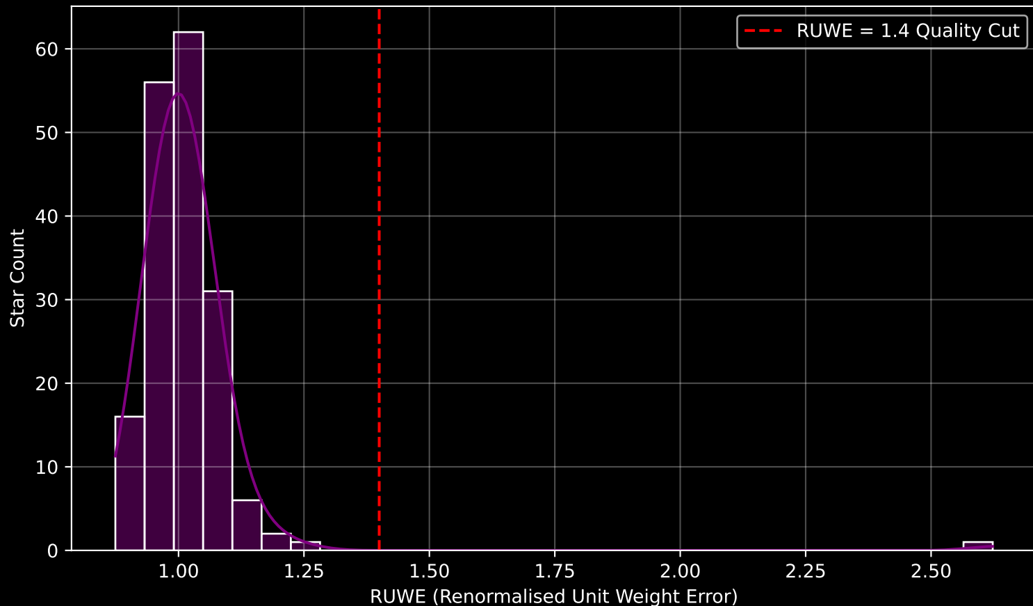
Gaia Cluster: [NGC_1193] RUWE Distribution (n= 175)
