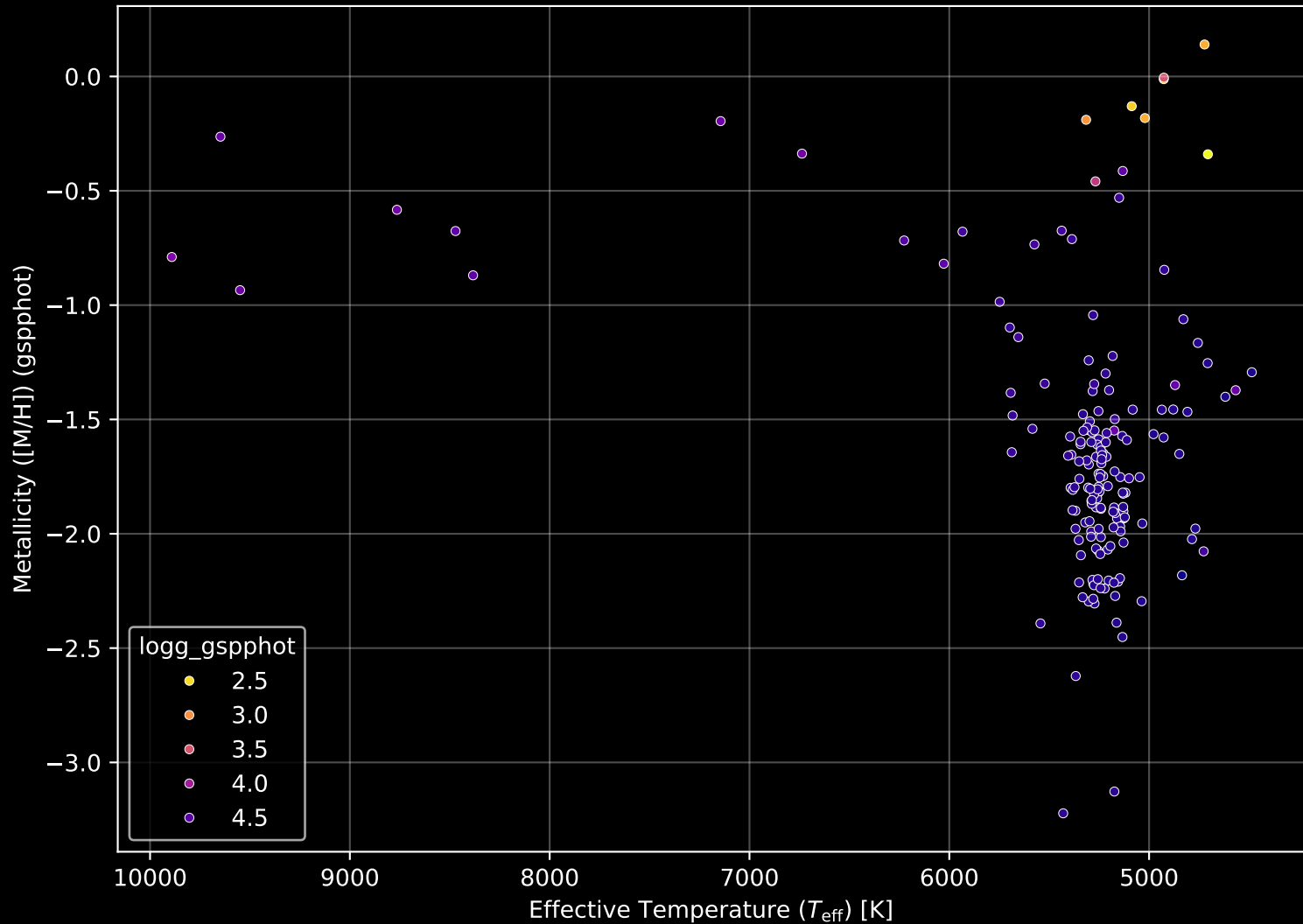
Gaia Cluster: [NGC_1193] Stellar Population Parameters (n= 175)
