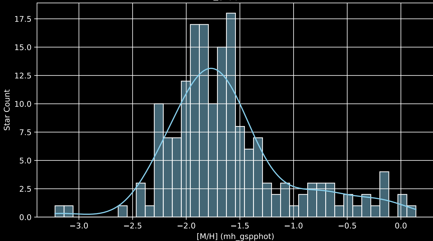
Gaia Cluster: [NGC_1193 [M/H] (mh_gspphot) (n= 175)
