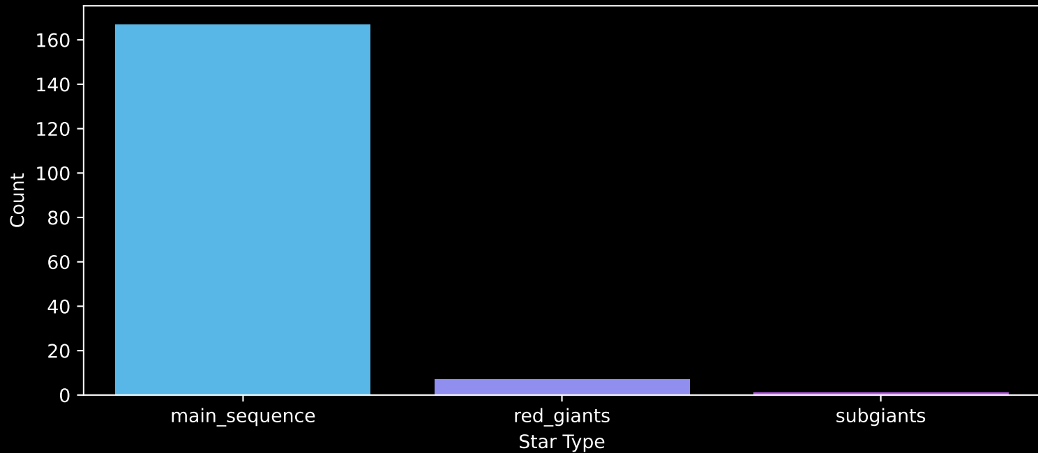
Gaia Cluster: [NGC_1193] Count plot of Star Type
