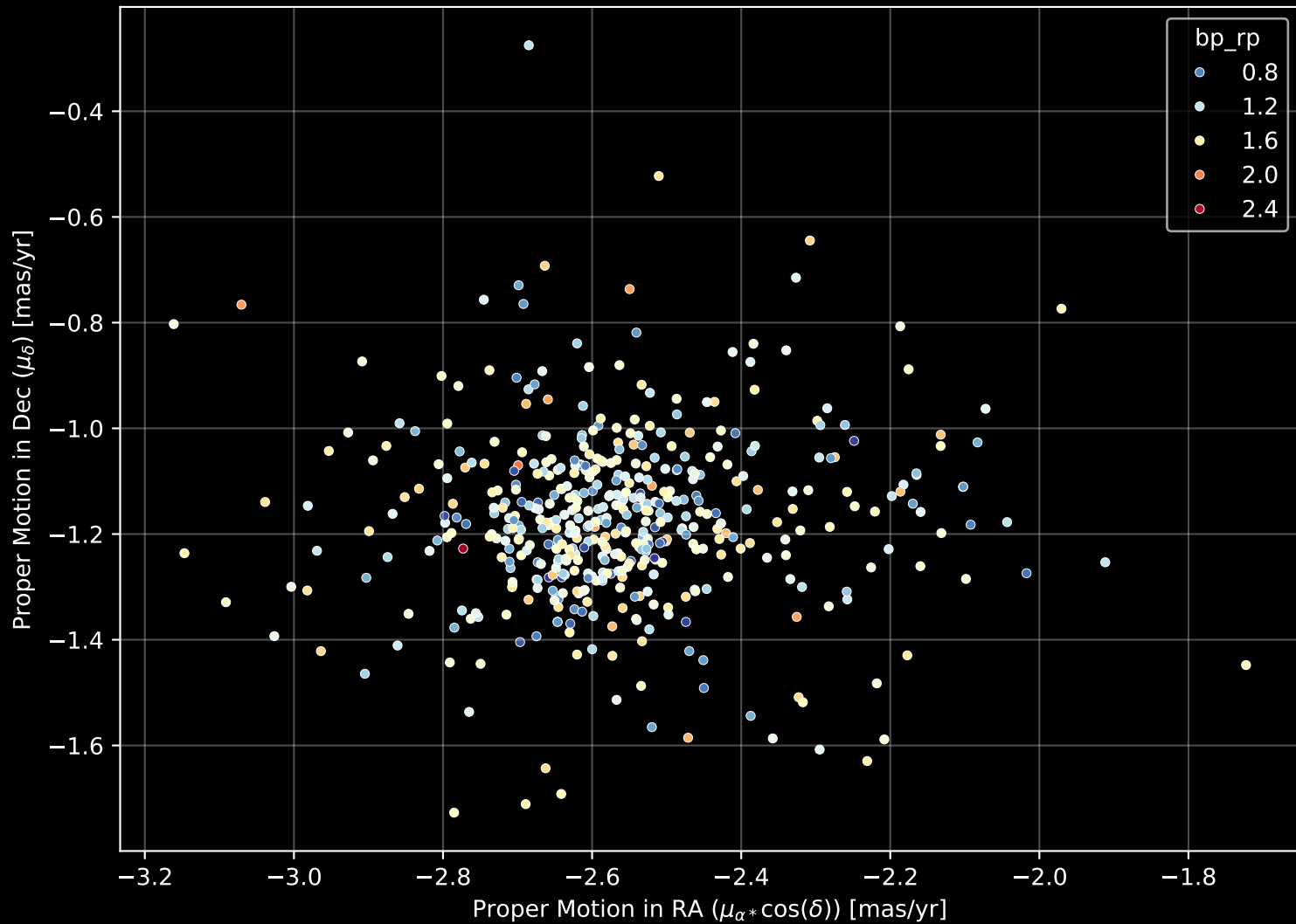
Gaia Cluster: [NGC_129] Proper Motion Diagram (n= 486)
