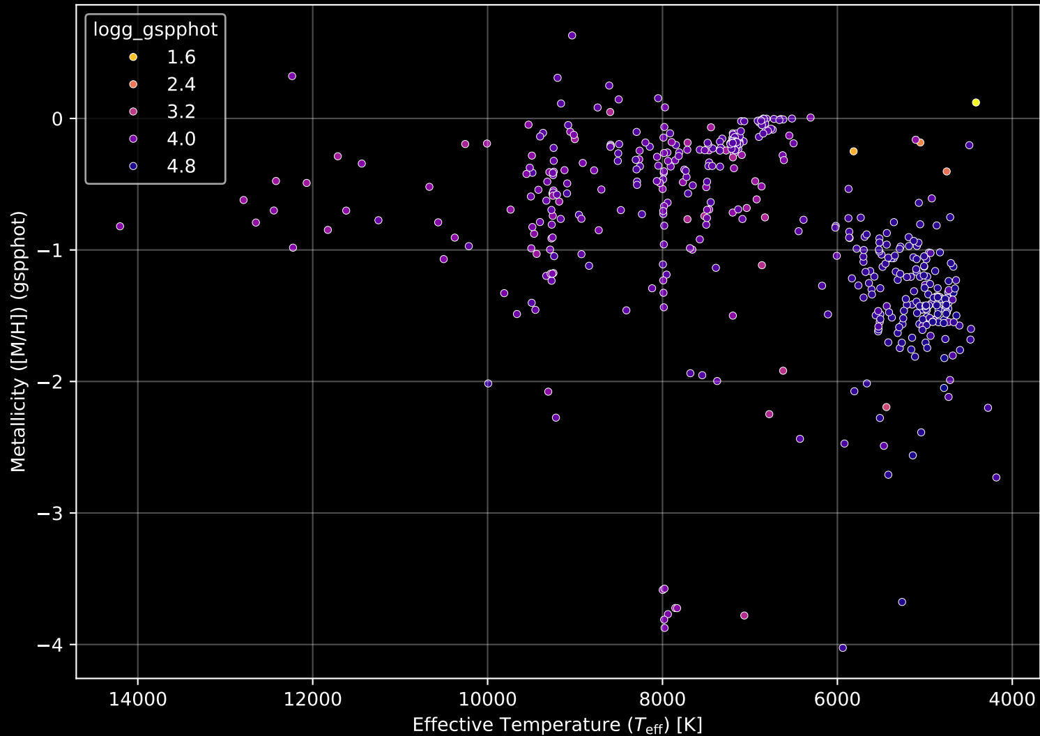
Gaia Cluster: [NGC_129] Stellar Population Parameters (n= 486)
