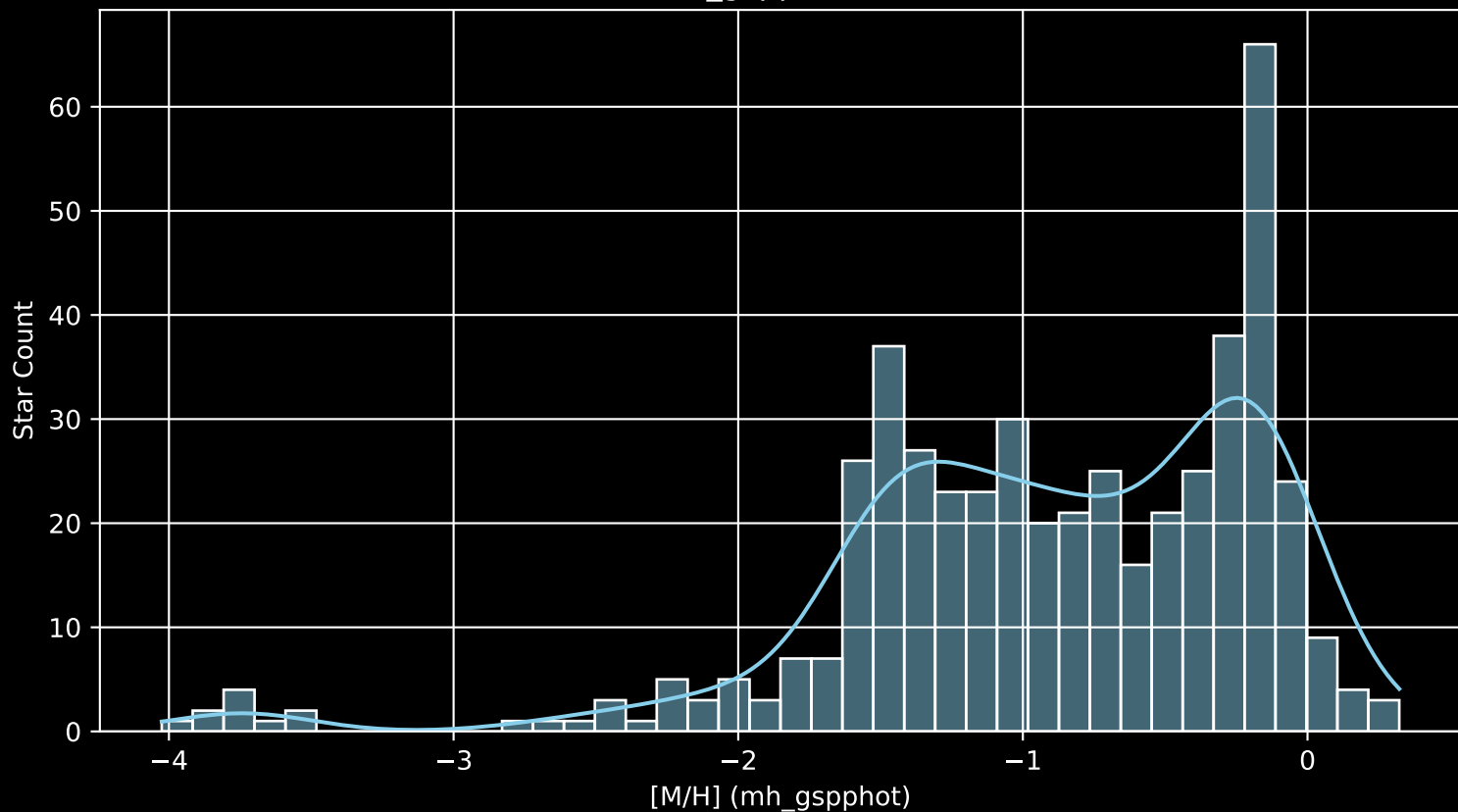
Gaia Cluster: [NGC_129 [M/H] (mh_gspphot) (n= 485)
