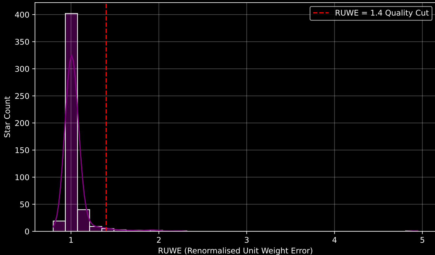
Gaia Cluster: [NGC_129] RUWE Distribution (n= 486)
