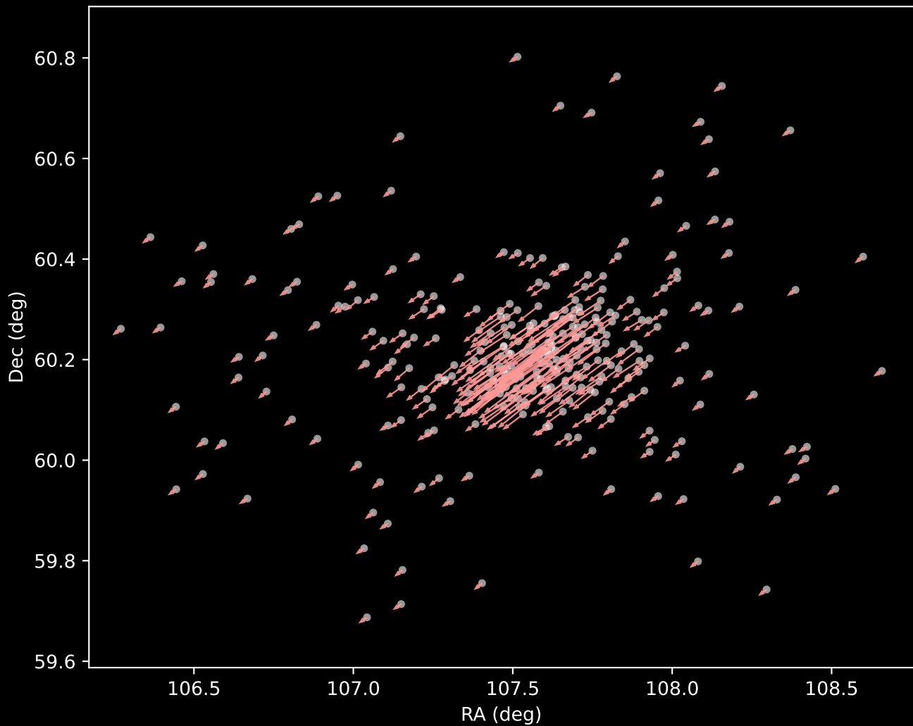
Gaia DR3 Cluster 7 Proper Motion Vectors (n=313)
