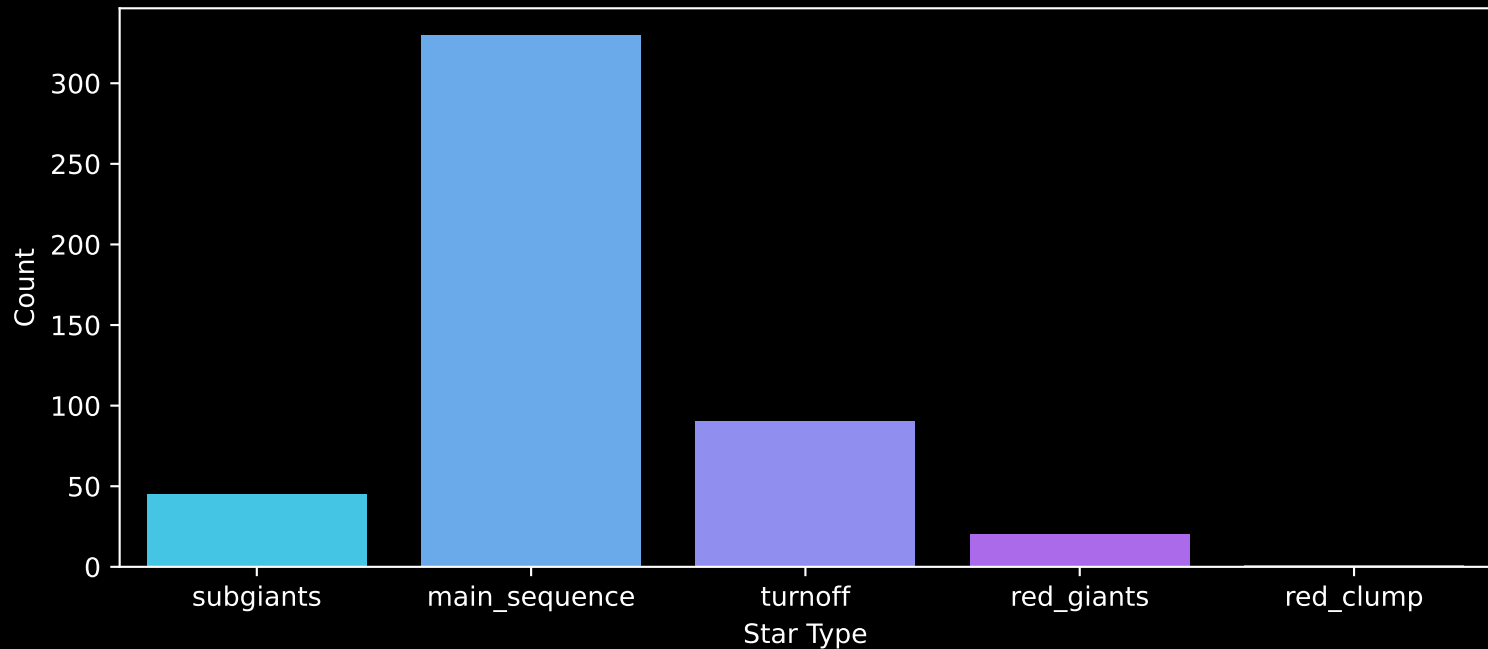
Gaia Cluster: [NGC_129] Count plot of Star Type
