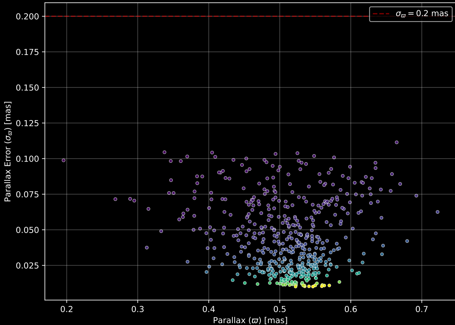
Gaia Cluster: [NGC_129] Parallax Quality (n= 486)
