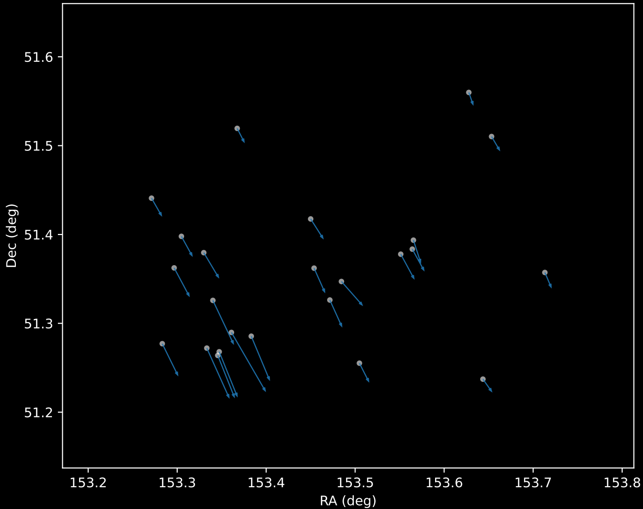
Gaia DR3 Cluster 0 Proper Motion Vectors (n=24)
