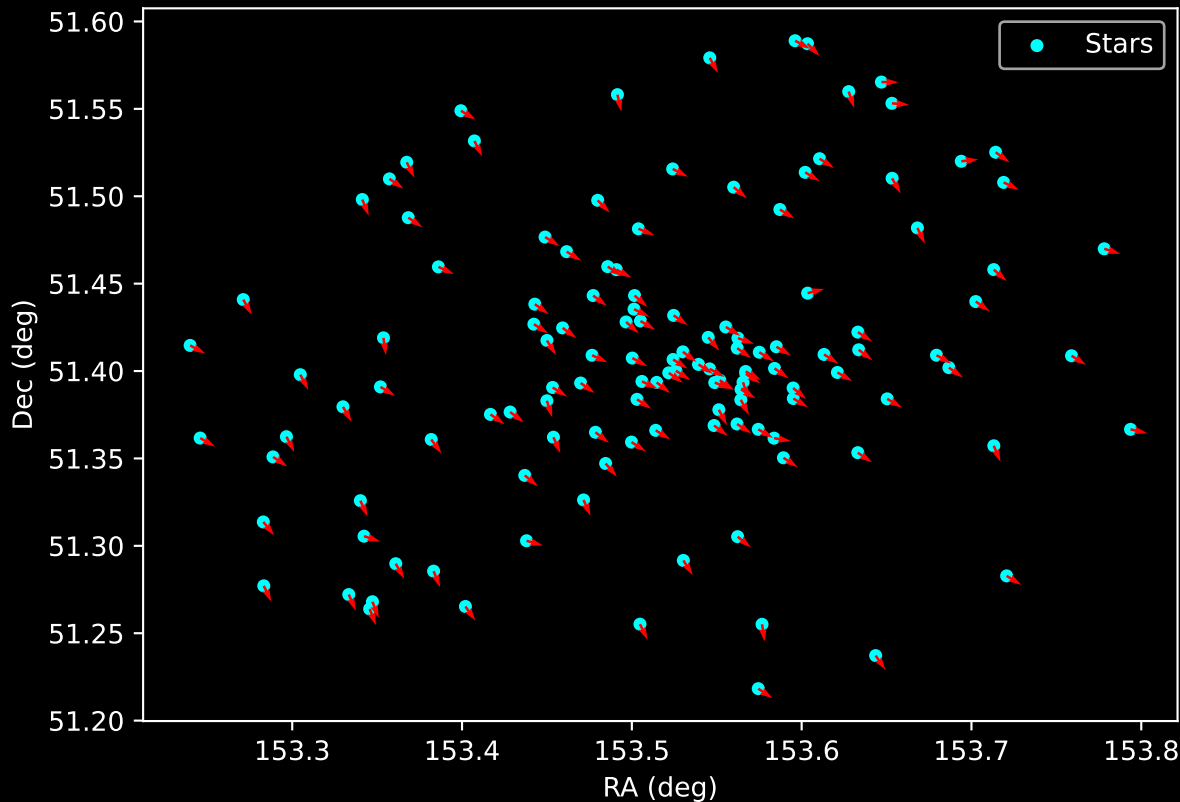
Gaia Cluster: [NGC_1348] Proper Motion Vectors for Gaia Star Field (n= 128)
