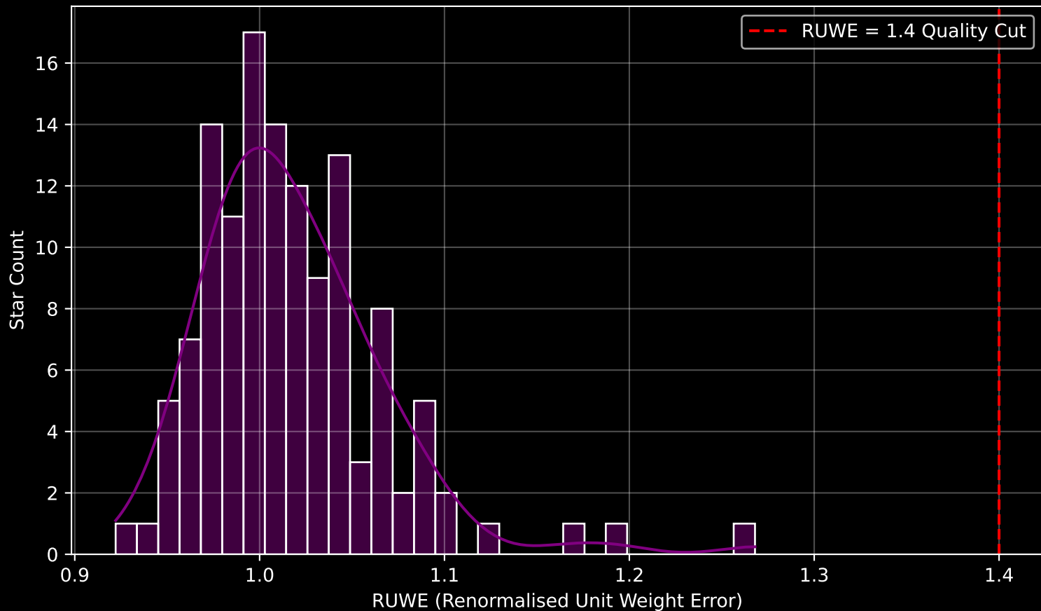
Gaia Cluster: [NGC_1348] RUWE Distribution (n= 128)
