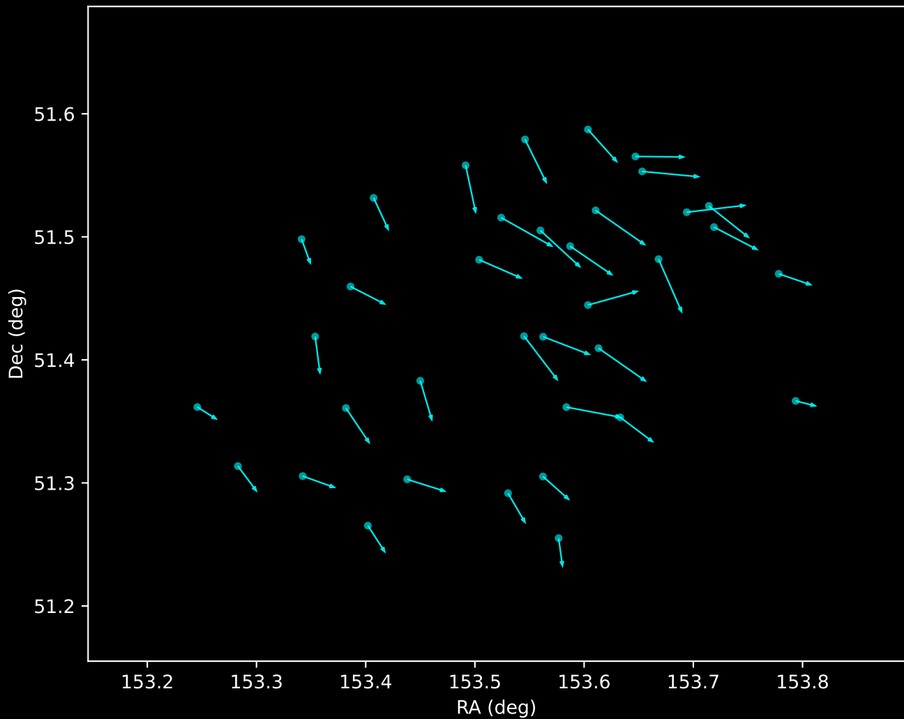
Gaia DR3 Noise Stream Proper Motion Vectors (n=36)
