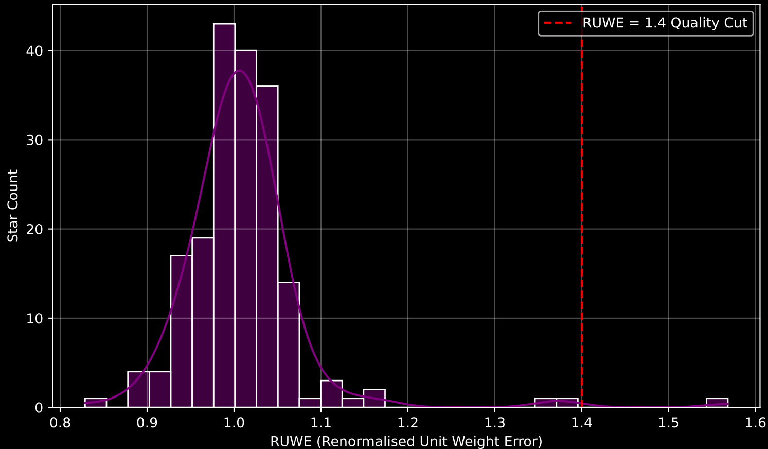
Gaia Cluster: [NGC_146] RUWE Distribution (n= 188)
