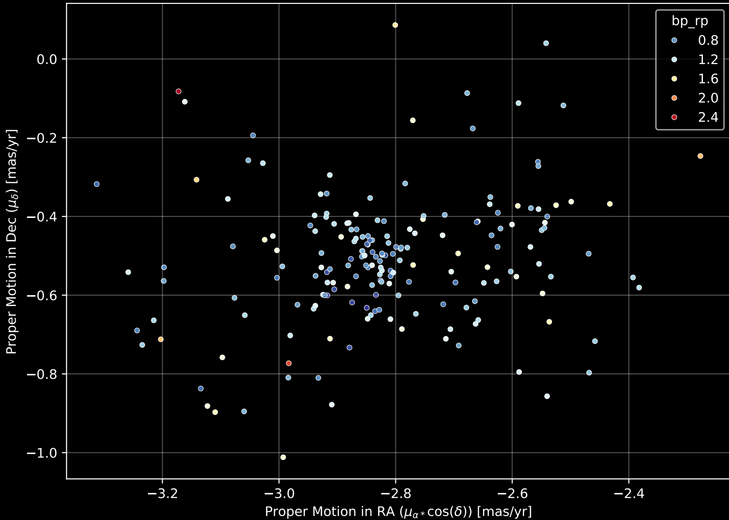
Gaia Cluster: [NGC_146] Proper Motion Diagram (n= 188)
