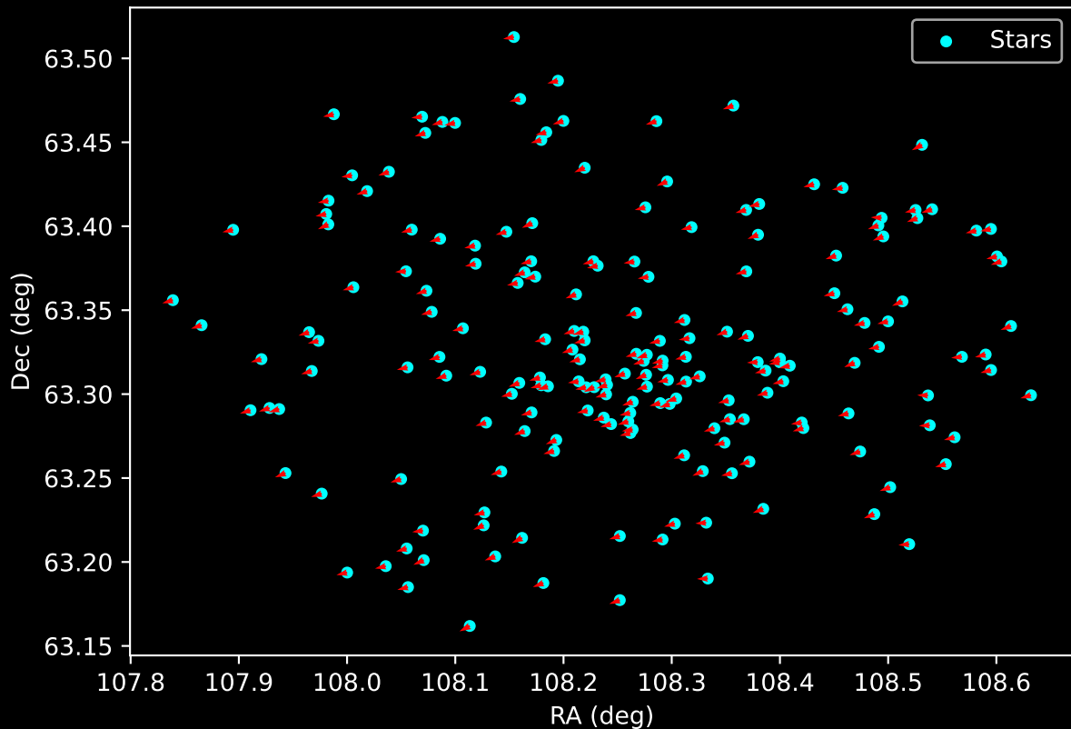
Gaia Cluster: [NGC_146] Proper Motion Vectors for Gaia Star Field (n= 188)
