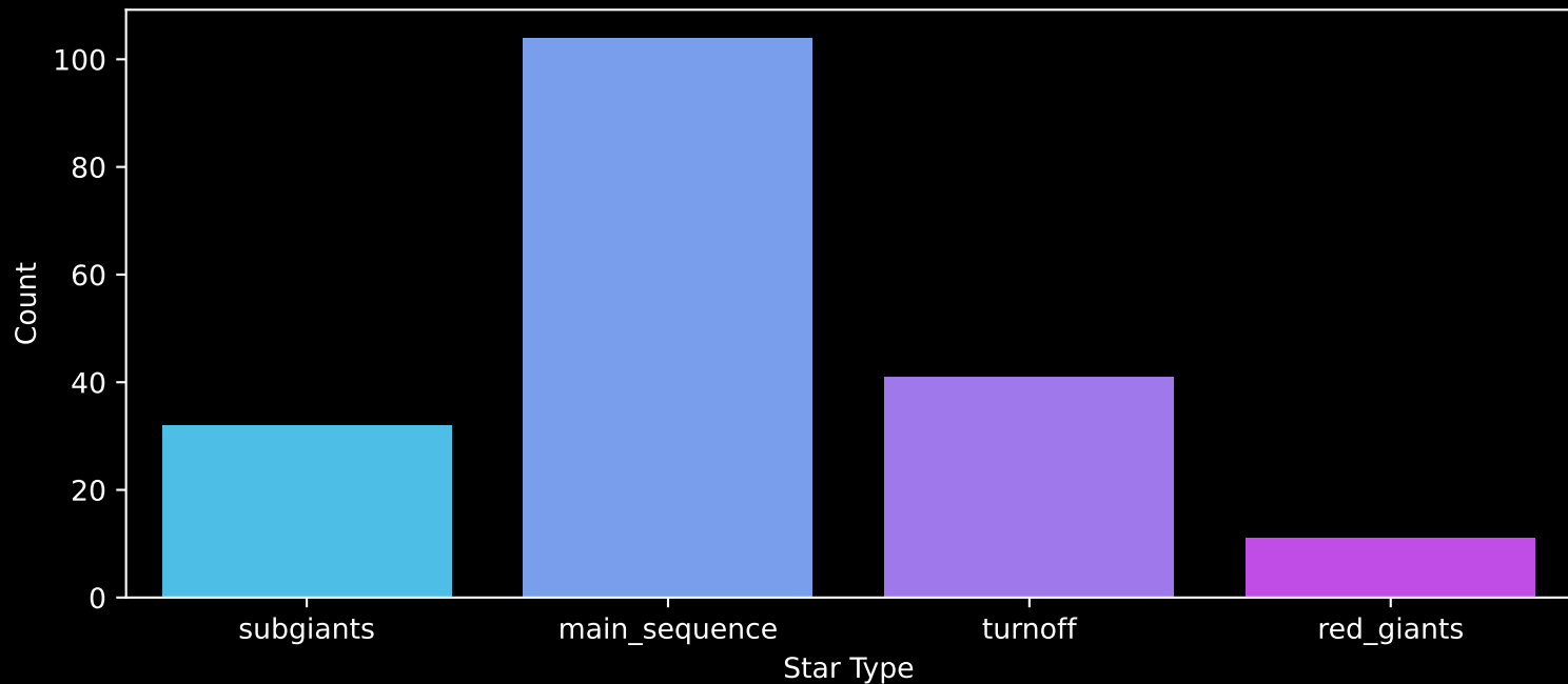
Gaia Cluster: [NGC_146] Count plot of Star Type
