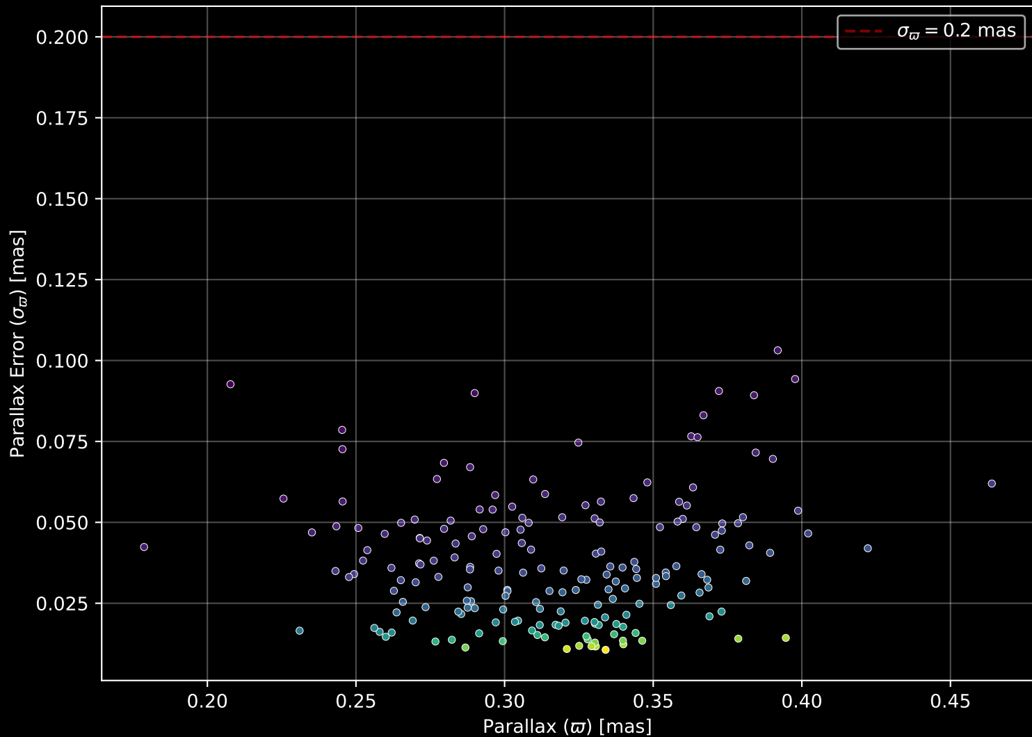
Gaia Cluster: [NGC_146] Parallax Quality (n= 188)
