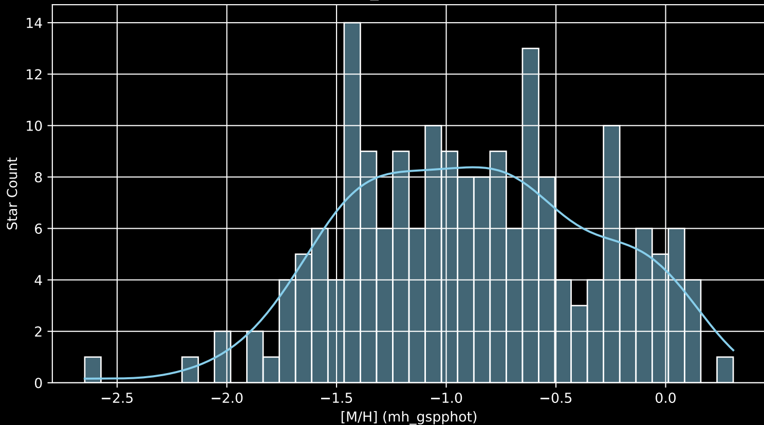
Gaia Cluster: [NGC_146 [M/H] (mh_gspphot) (n= 188)
