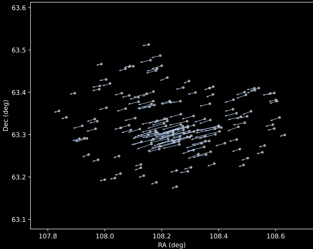
Gaia DR3 Cluster 1 Proper Motion Vectors (n=156)
