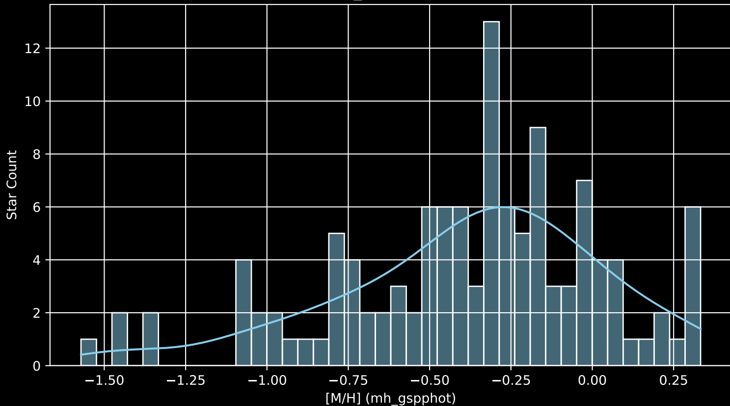
Gaia Cluster: [NGC_1502 [M/H] (mh_gspphot) (n= 120)
