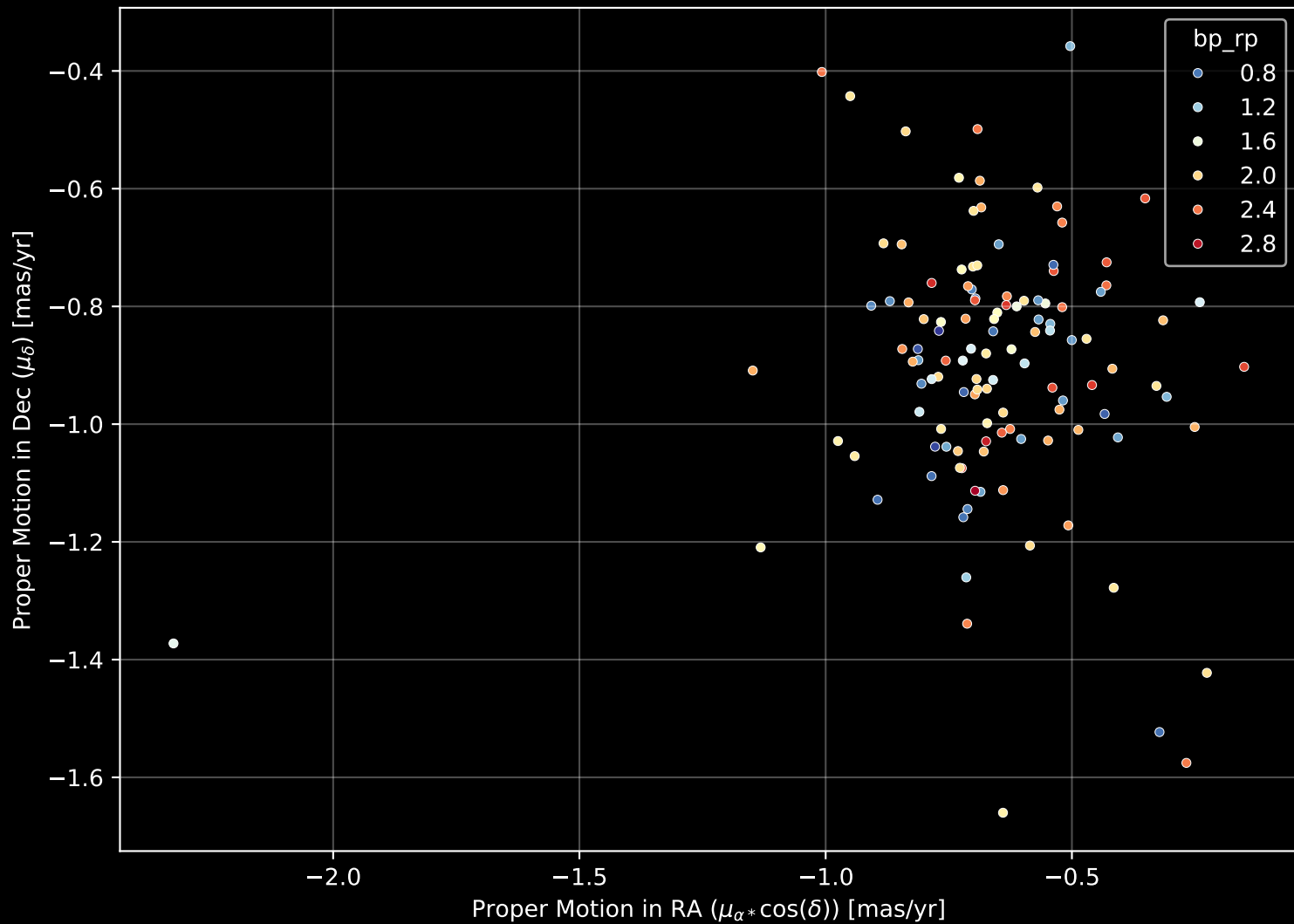
Gaia Cluster: [NGC_1502] Proper Motion Diagram (n= 121)
