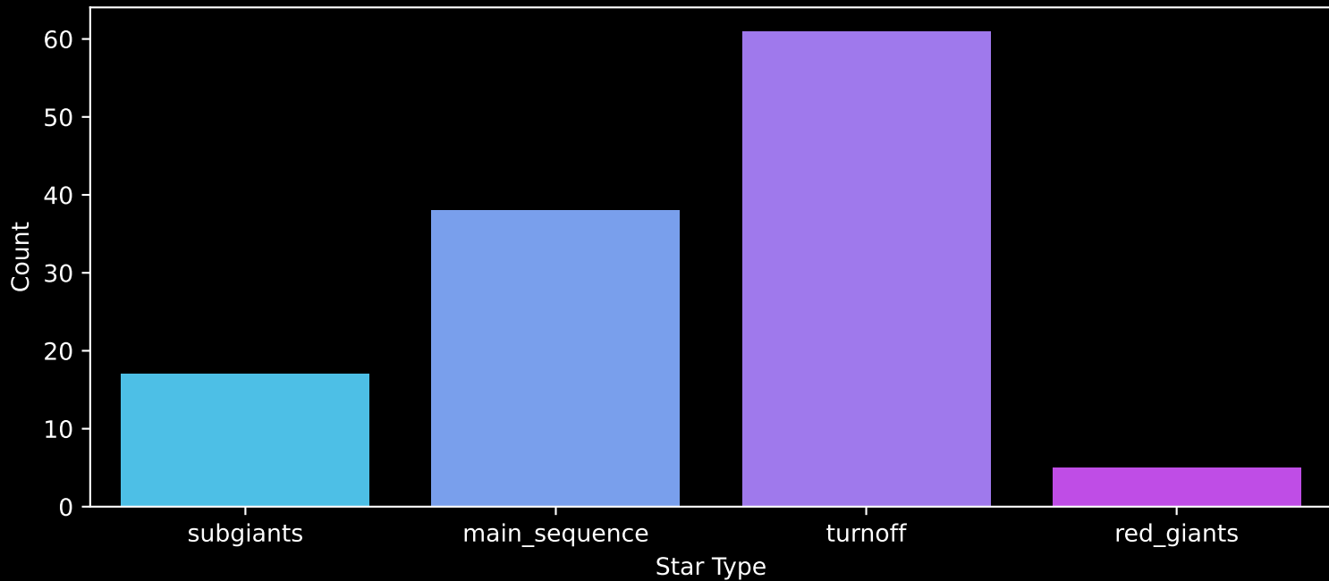
Gaia Cluster: [NGC_1502] Count plot of Star Type
