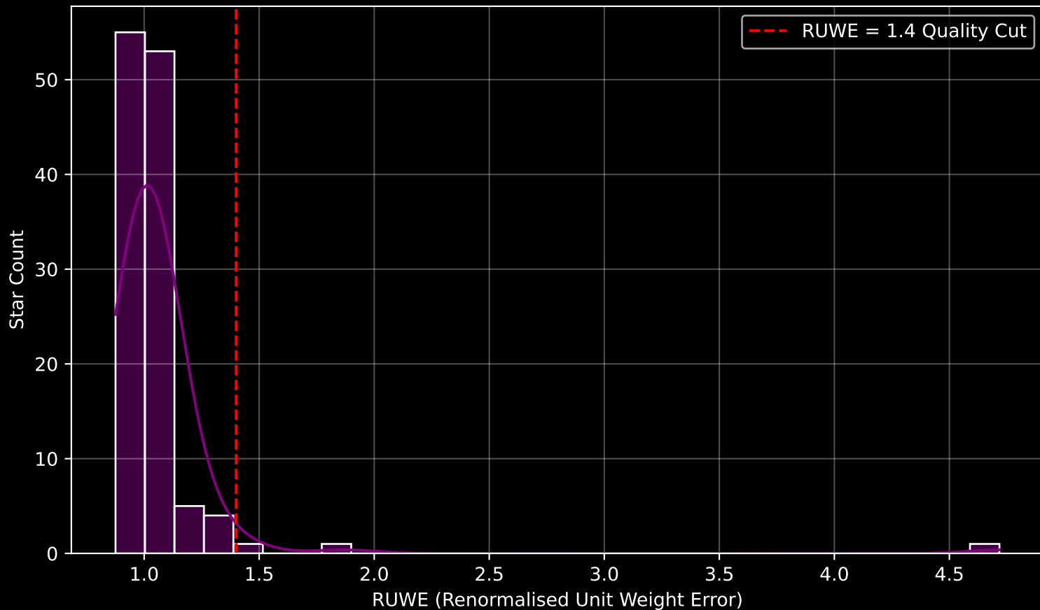
Gaia Cluster: [NGC_1502] RUWE Distribution (n= 120)
