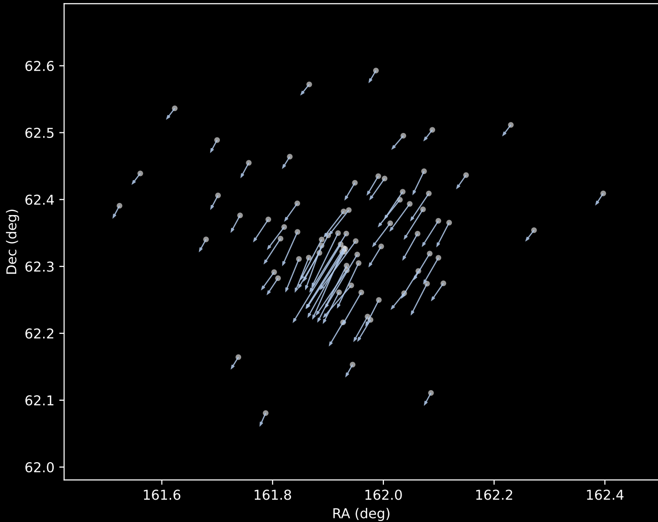
Gaia DR3 Cluster 1 Proper Motion Vectors (n=75)
