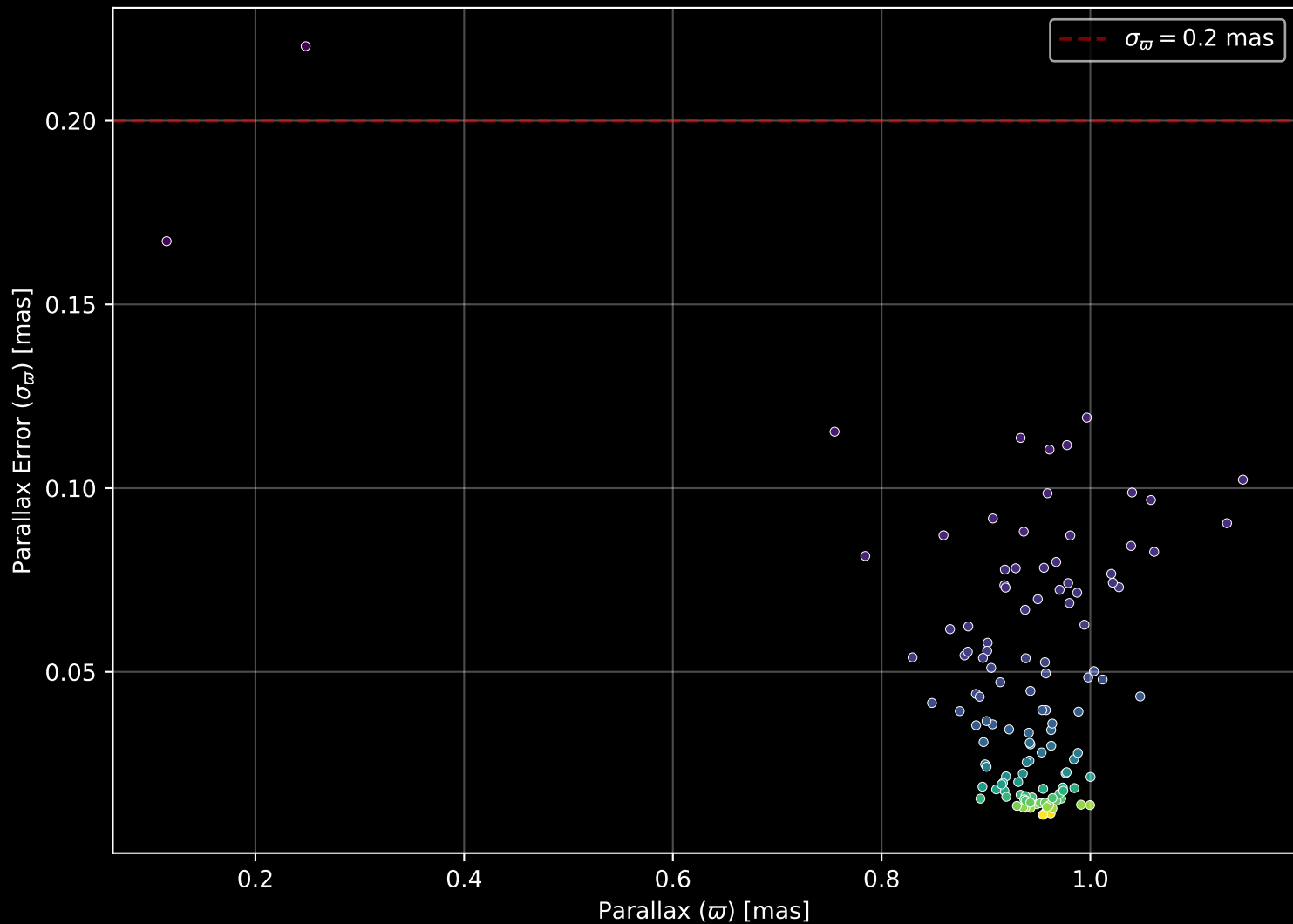
Gaia Cluster: [NGC_1502] Parallax Quality (n= 121)
