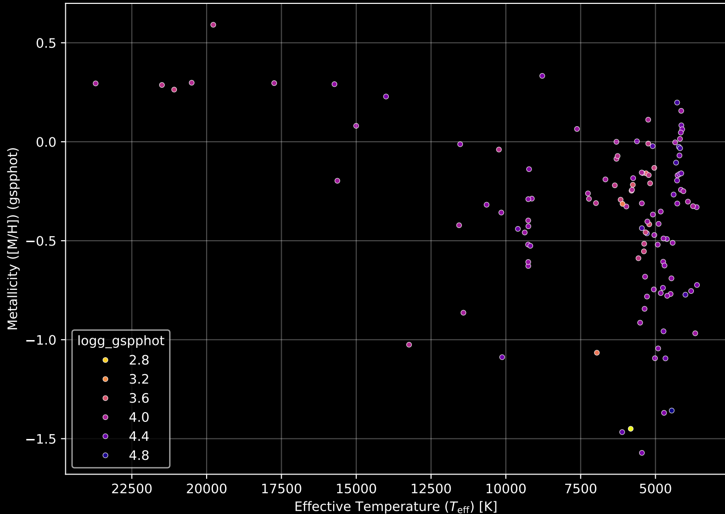
Gaia Cluster: [NGC_1502] Stellar Population Parameters (n= 121)
