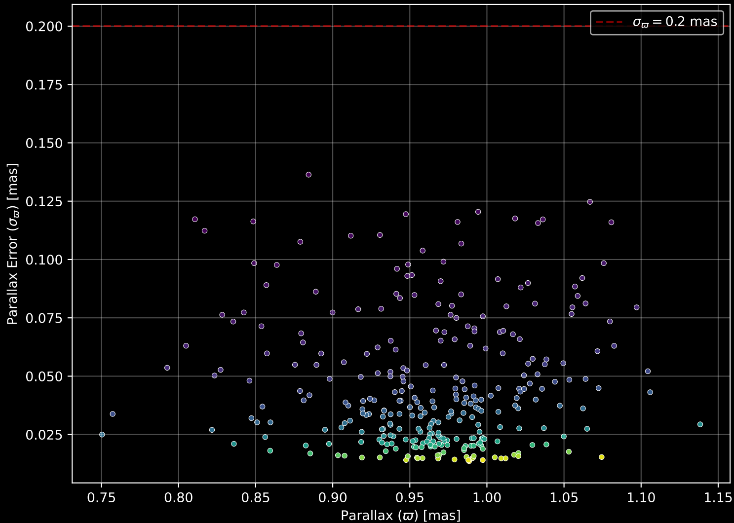
Gaia Cluster: [NGC_1528] Parallax Quality (n= 303)
