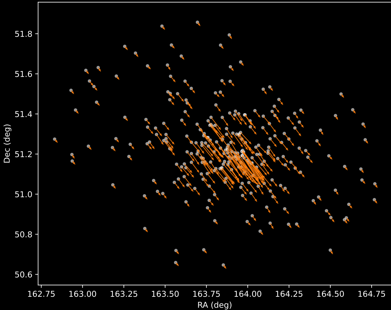
Gaia DR3 Cluster 2 Proper Motion Vectors (n=263)
