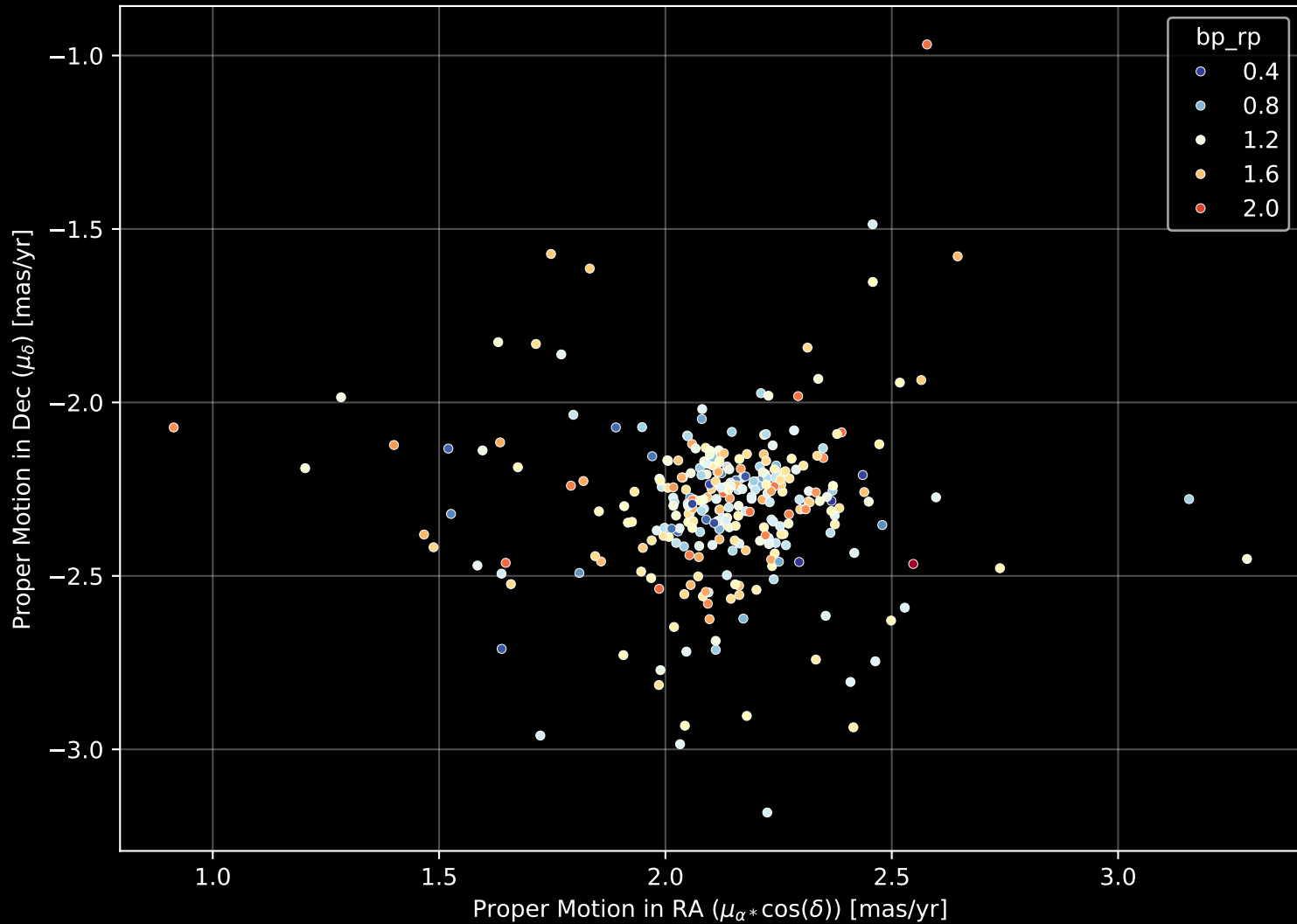
Gaia Cluster: [NGC_1528] Proper Motion Diagram (n= 303)
