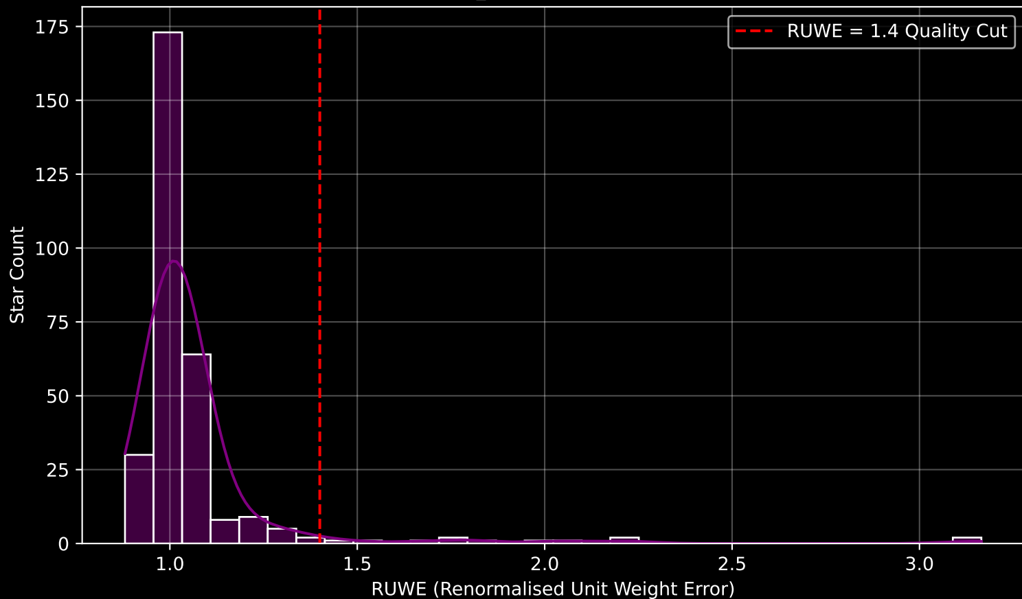
Gaia Cluster: [NGC_1528] RUWE Distribution (n= 303)
