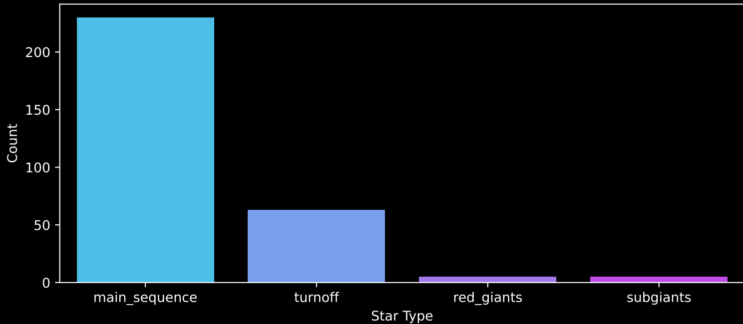
Gaia Cluster: [NGC_1528] Count plot of Star Type
