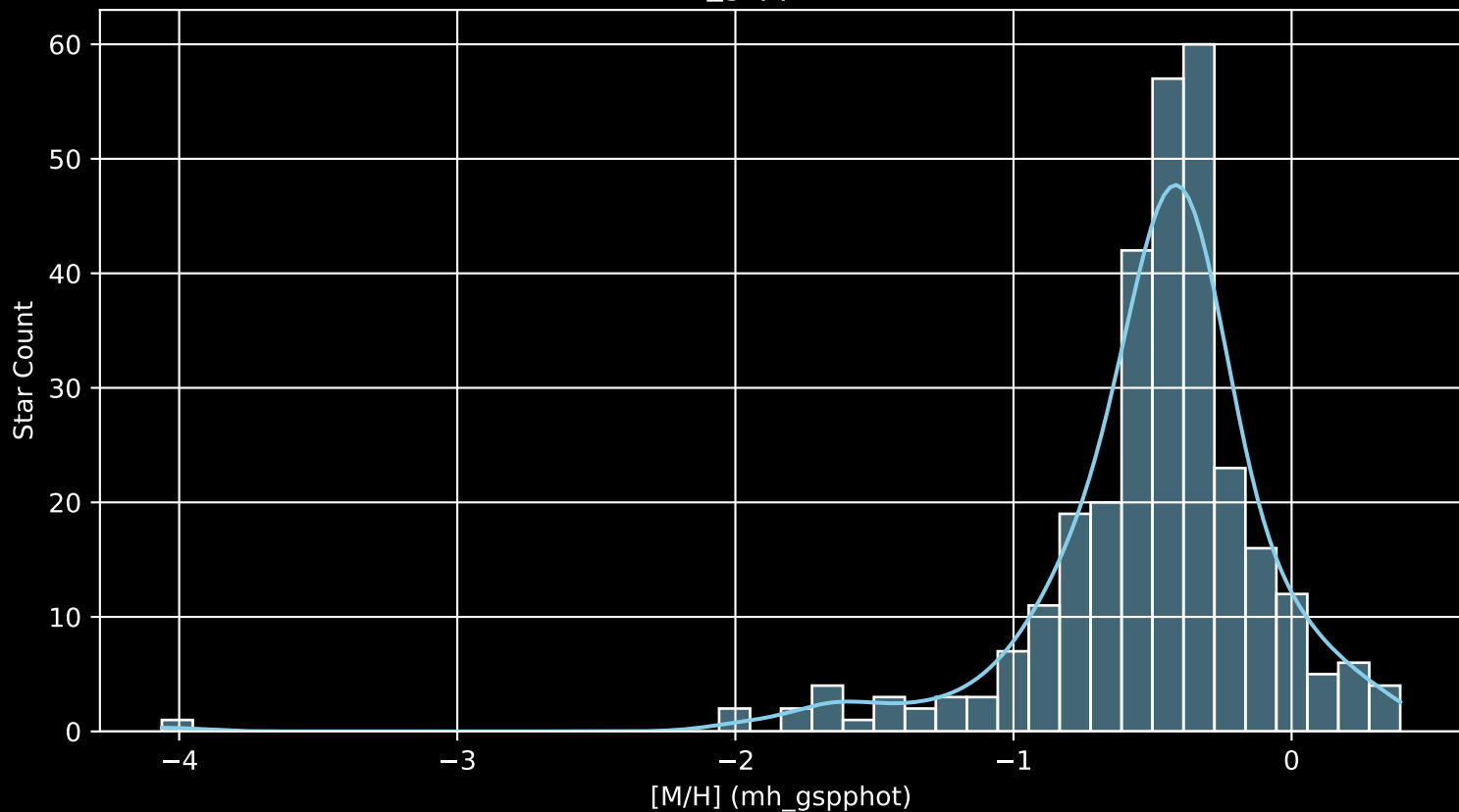
Gaia Cluster: [NGC_1528 [M/H] (mh_gspphot) (n= 303)
