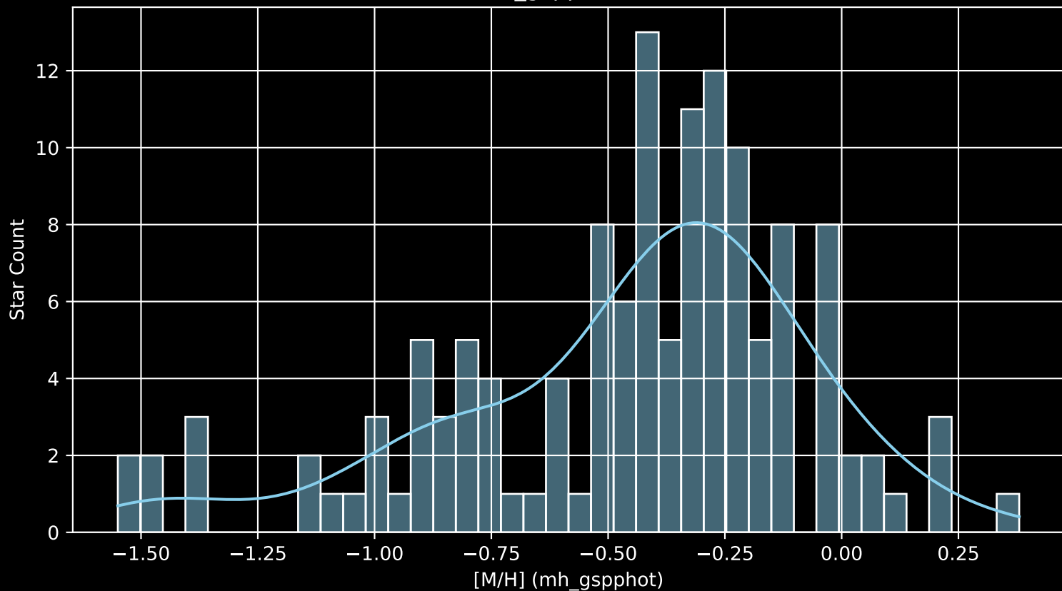
Gaia Cluster: [NGC_1545 [M/H] (mh_gspphot) (n= 134)
