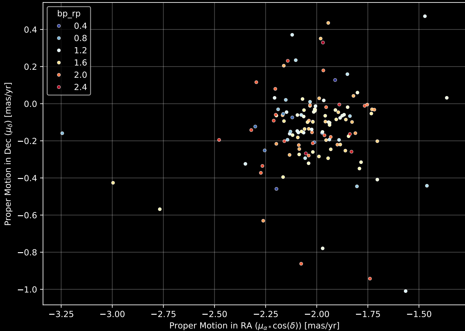
Gaia Cluster: [NGC_1545] Proper Motion Diagram (n= 134)
