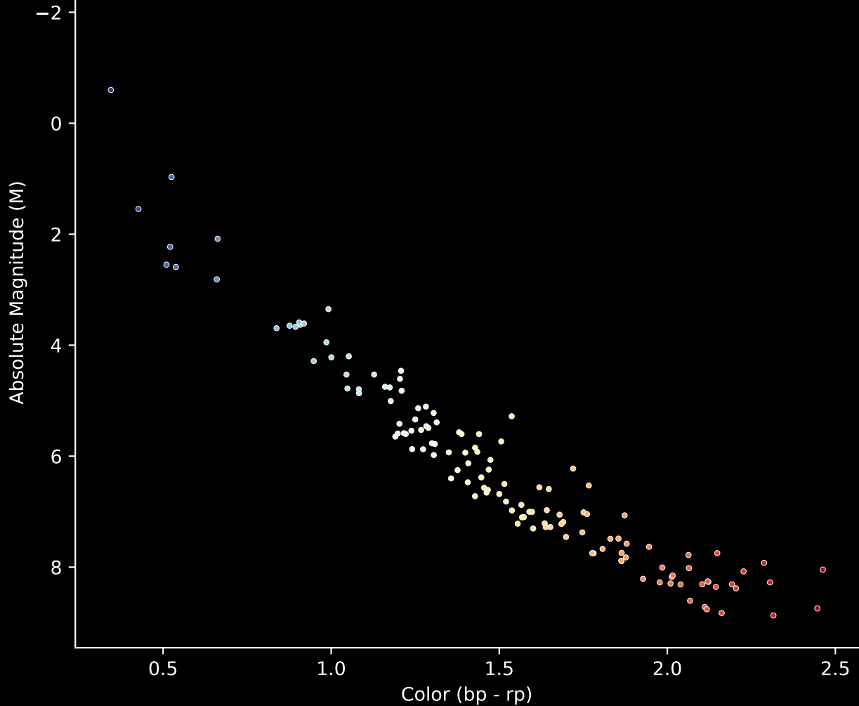
Gaia Cluster: [NGC_1545] Stars (n= 134) Hertzsprung-Russel Diagram
