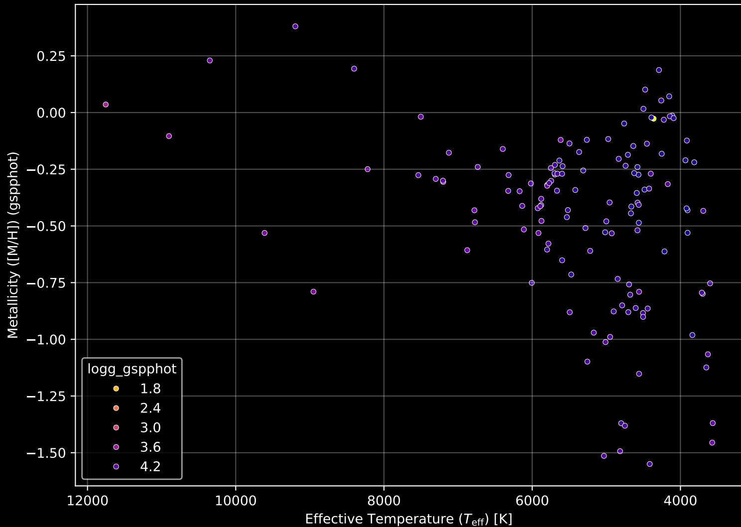
Gaia Cluster: [NGC_1545] Stellar Population Parameters (n= 134)
