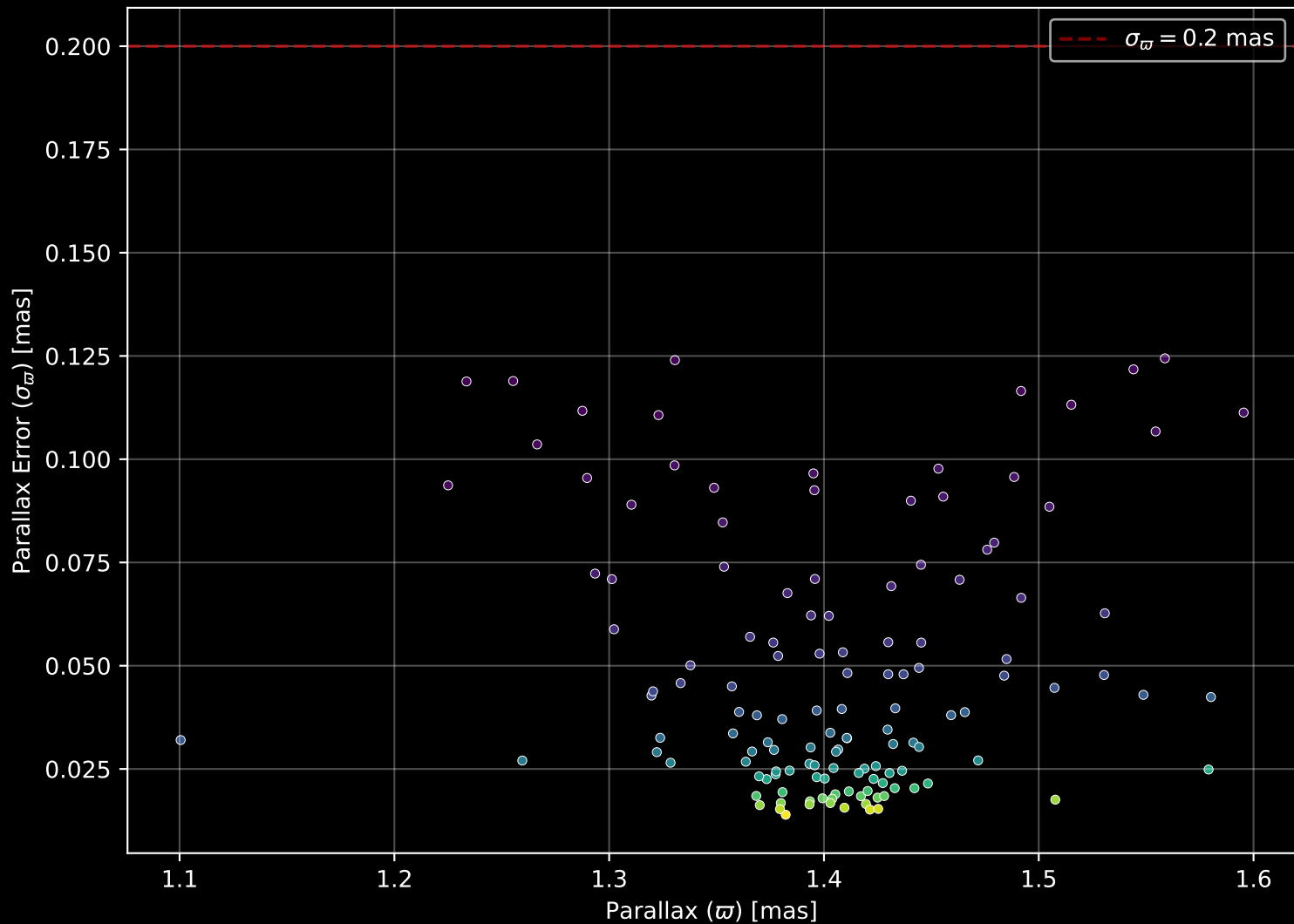
Gaia Cluster: [NGC_1545] Parallax Quality (n= 134)
