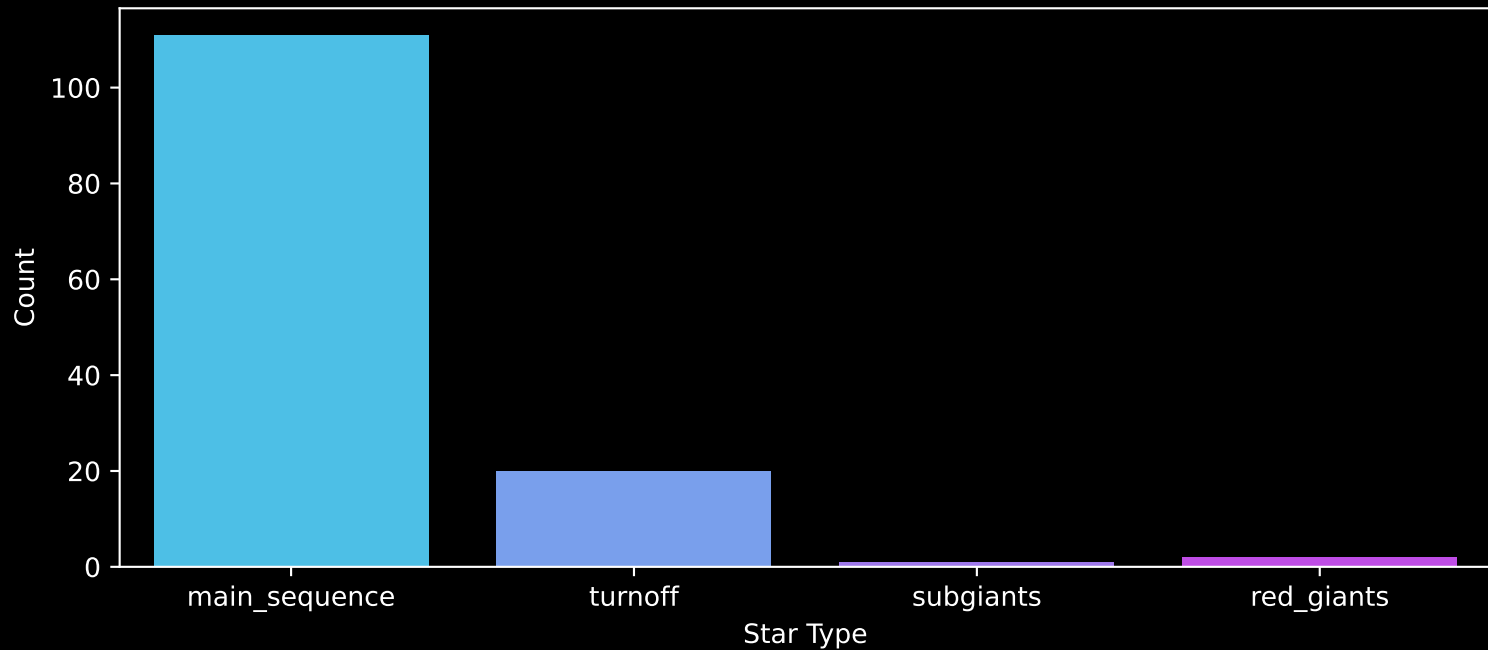
Gaia Cluster: [NGC_1545] Count plot of Star Type
