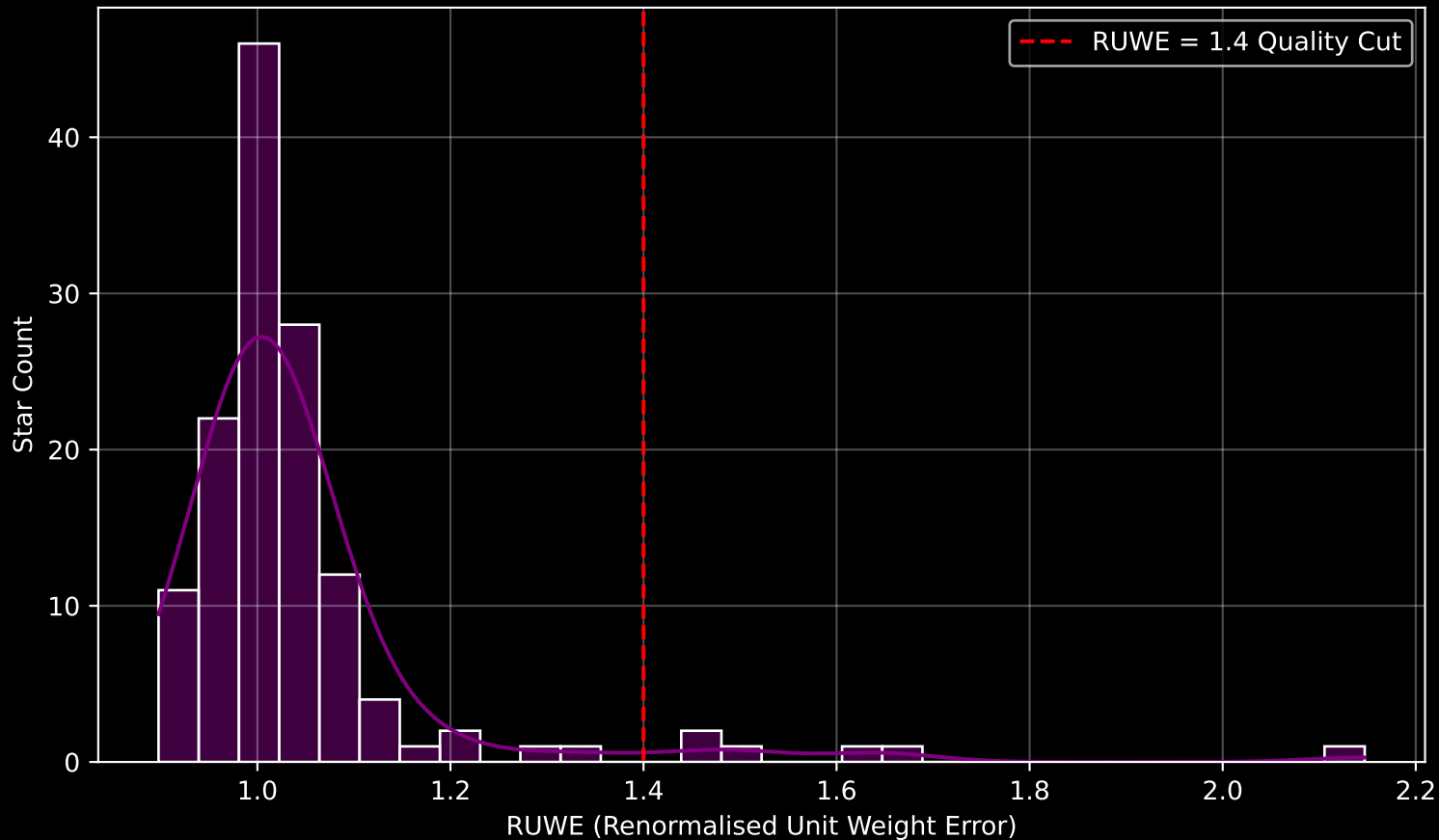
Gaia Cluster: [NGC_1545] RUWE Distribution (n= 134)
