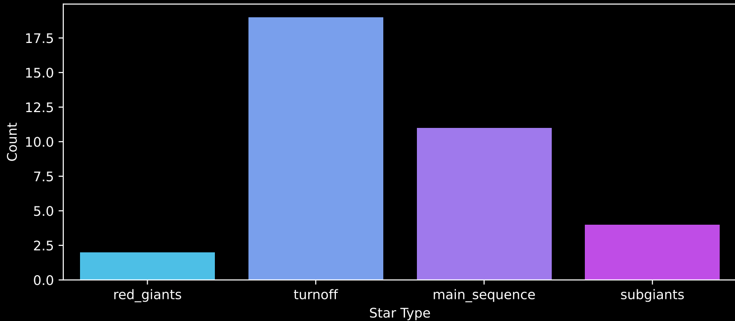
Gaia Cluster: [NGC_1579] Count plot of Star Type
