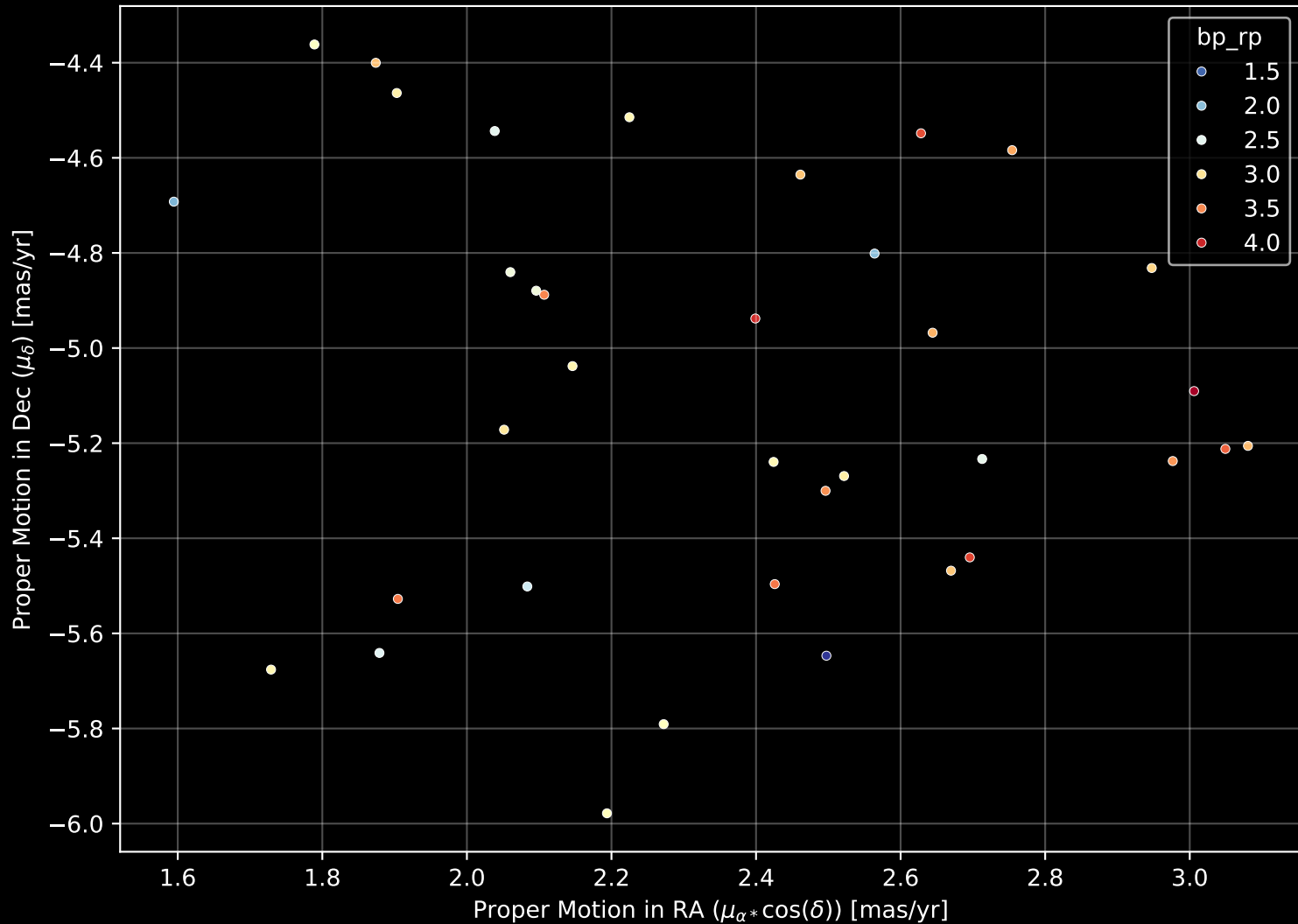
Gaia Cluster: [NGC_1579] Proper Motion Diagram (n= 36)
