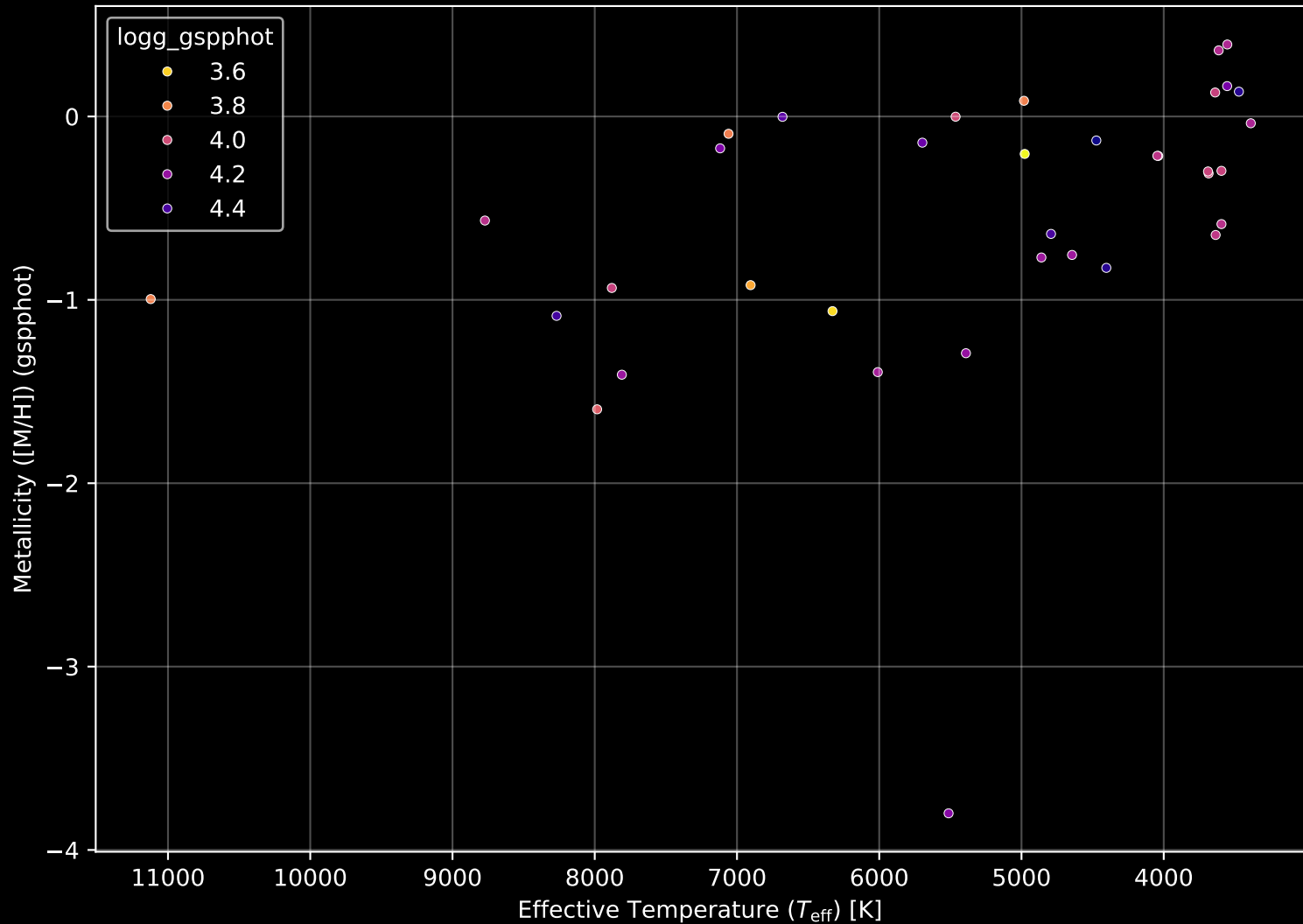
Gaia Cluster: [NGC_1579] Stellar Population Parameters (n= 36)
