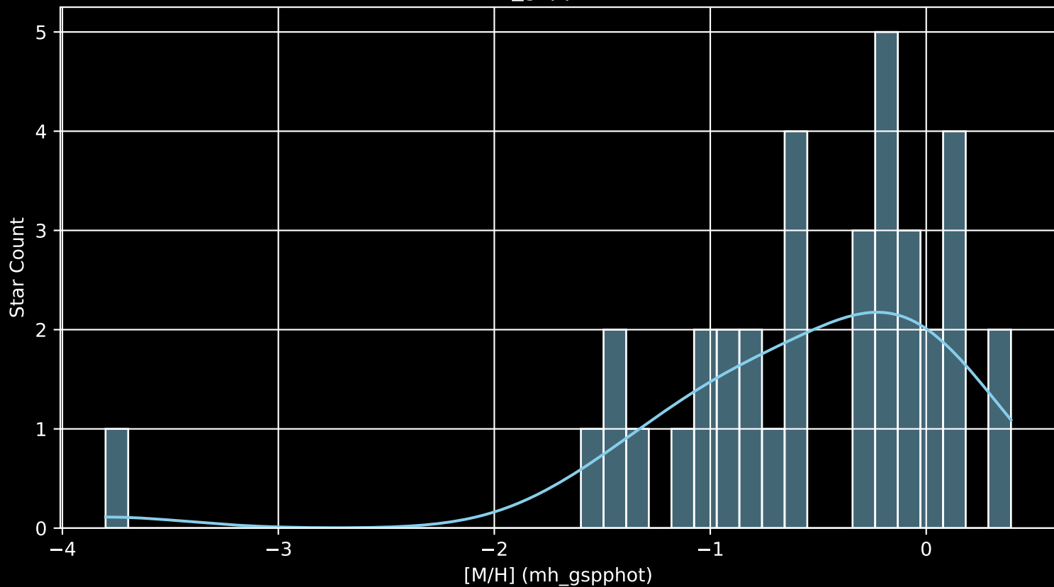
Gaia Cluster: [NGC_1579 [M/H] (mh_gspphot) (n= 36)
