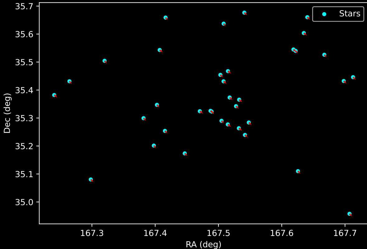
Gaia Cluster: [NGC_1579] Proper Motion Vectors for Gaia Star Field (n= 36)
