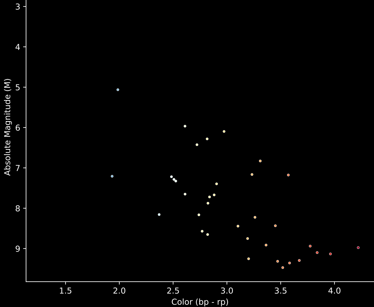
Gaia Cluster: [NGC_1579] Stars (n= 36) Hertzprung-Russel Diagram
