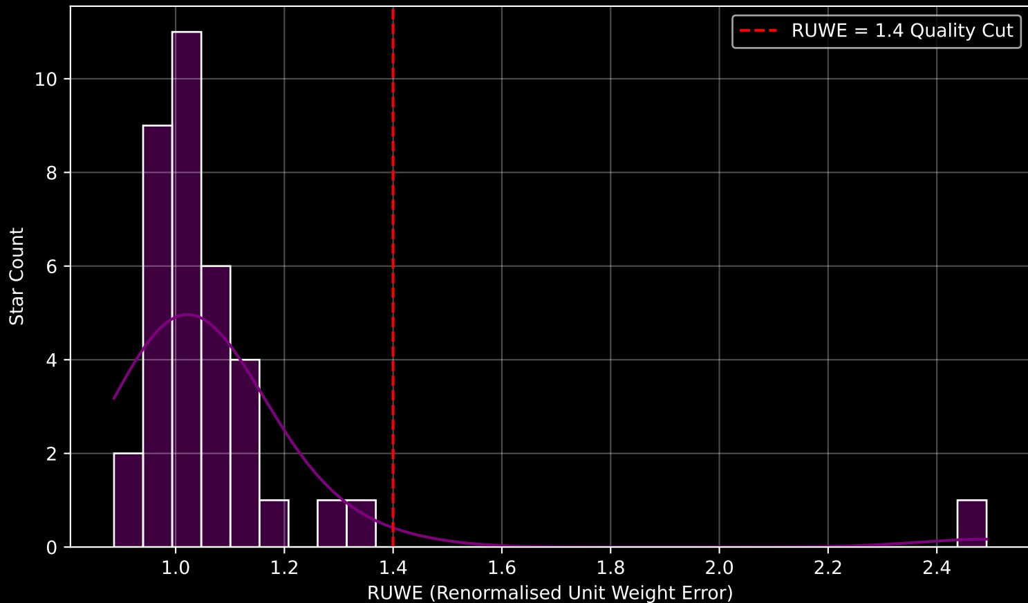
Gaia Cluster: [NGC_1579] RUWE Distribution (n= 36)
