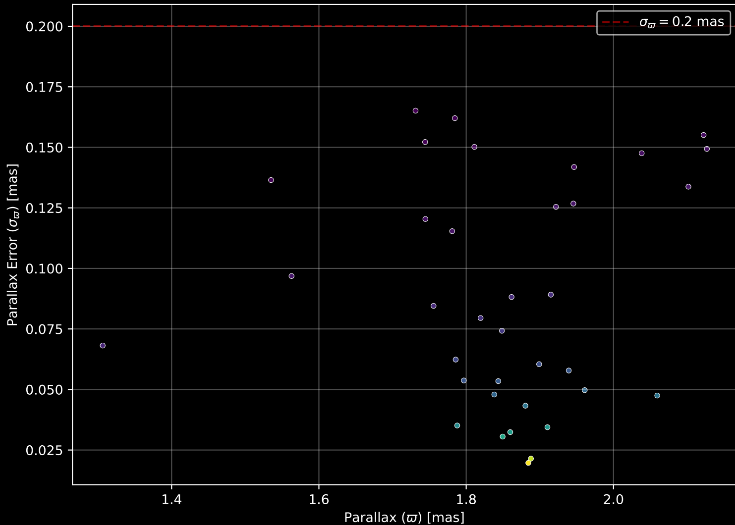
Gaia Cluster: [NGC_1579] Parallax Quality (n= 36)
