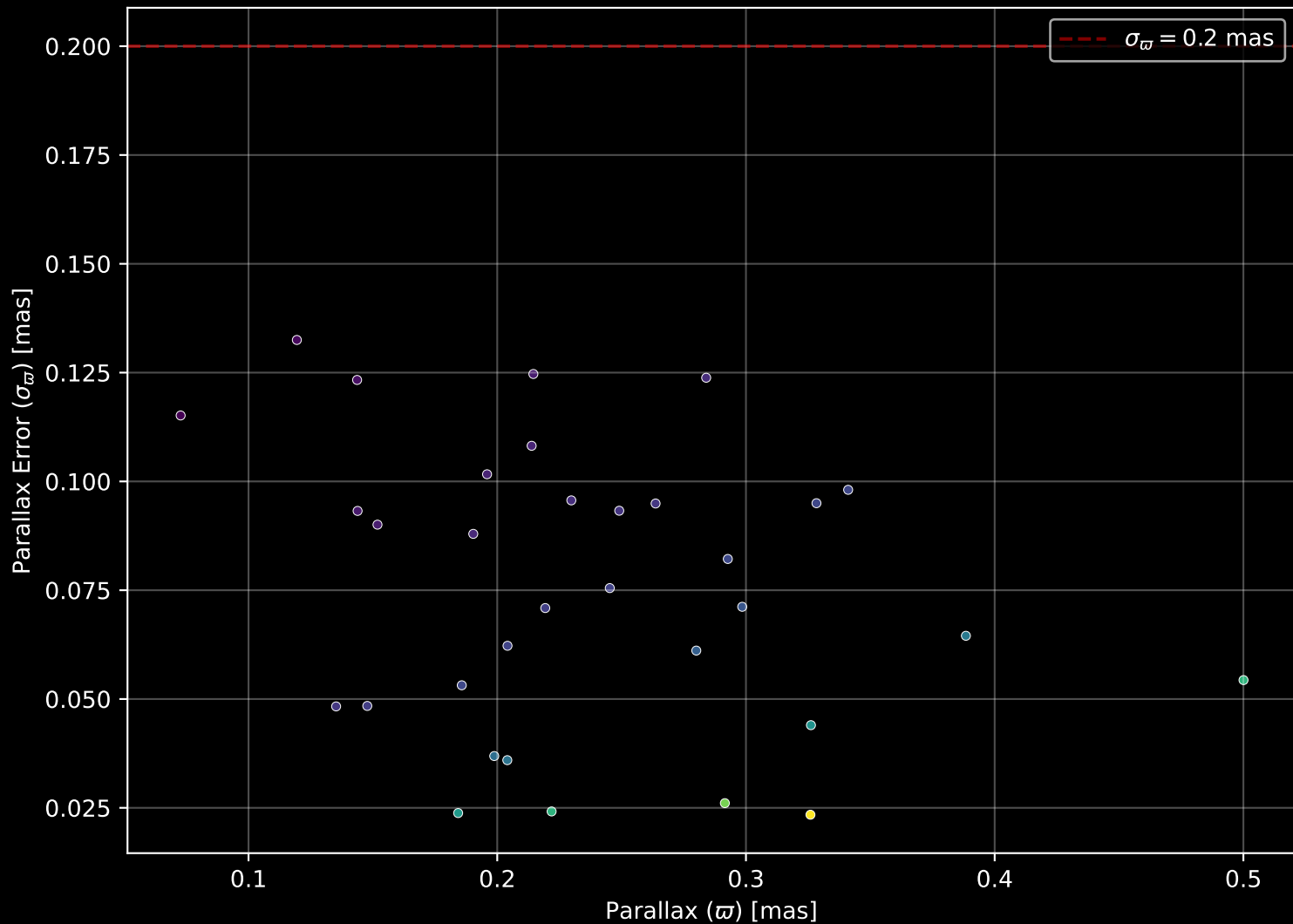
Gaia Cluster: [NGC_1624] Parallax Quality (n= 33)
