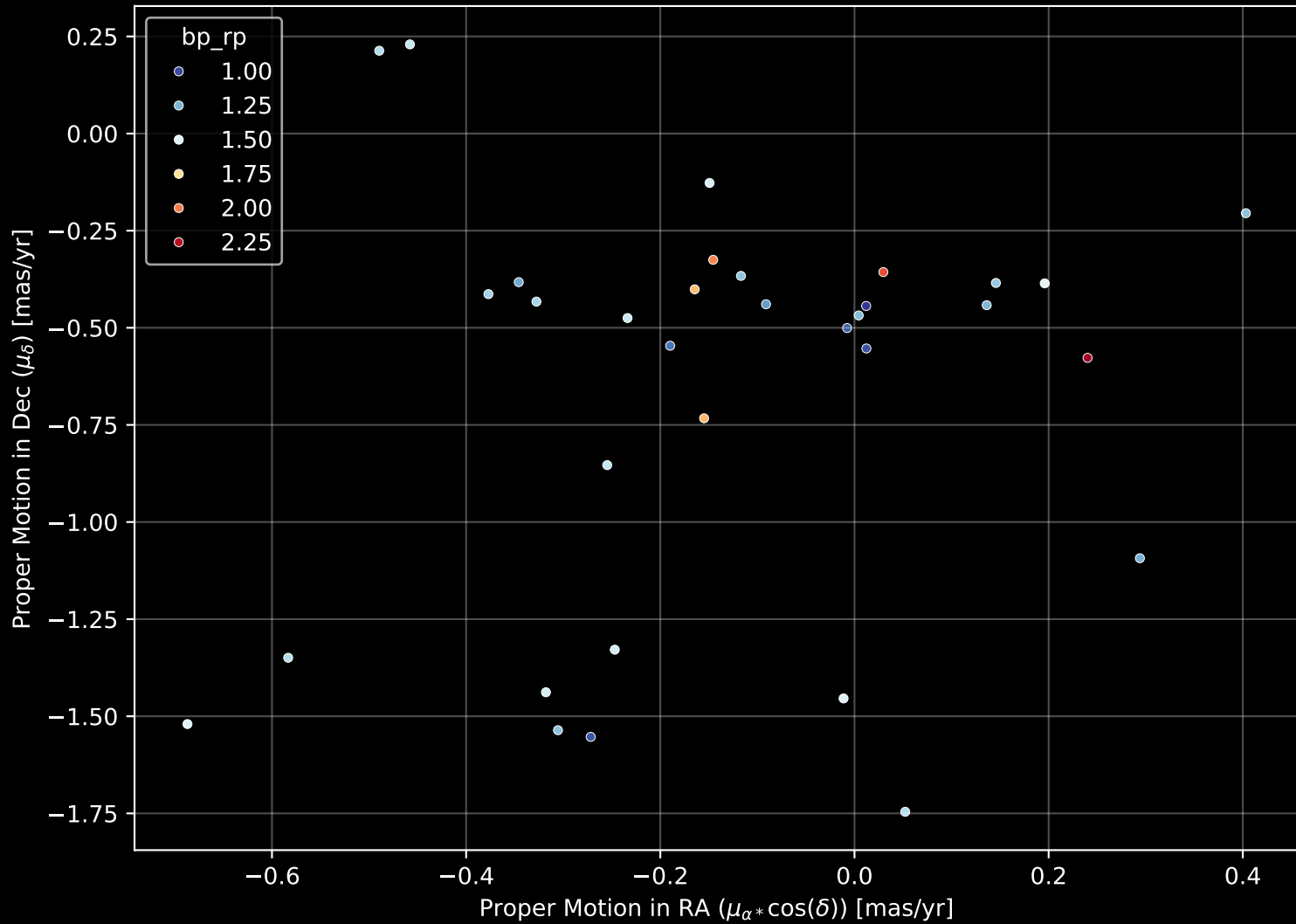
Gaia Cluster: [NGC_1624] Proper Motion Diagram (n= 33)
