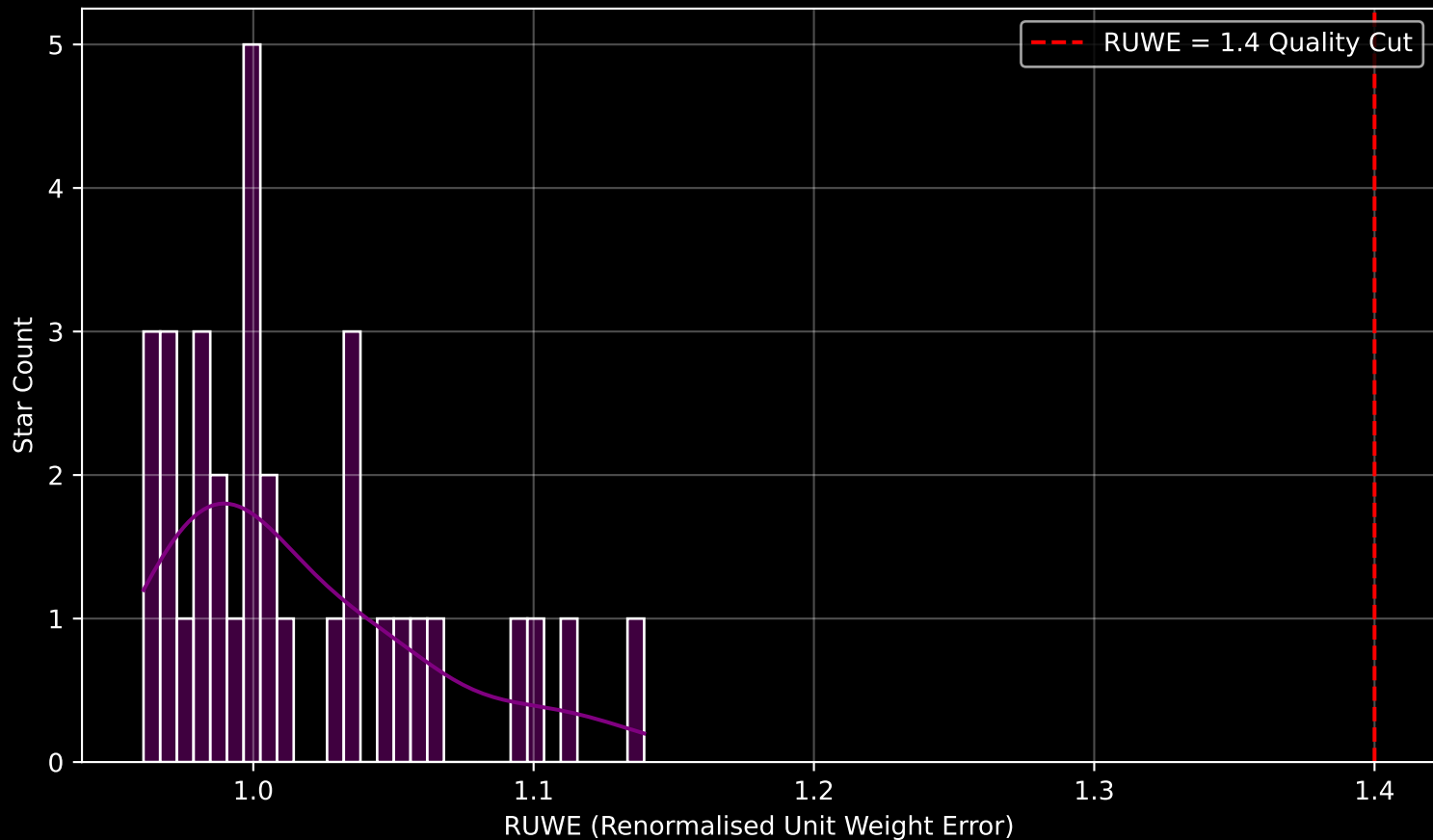
Gaia Cluster: [NGC_1624] RUWE Distribution (n= 33)
