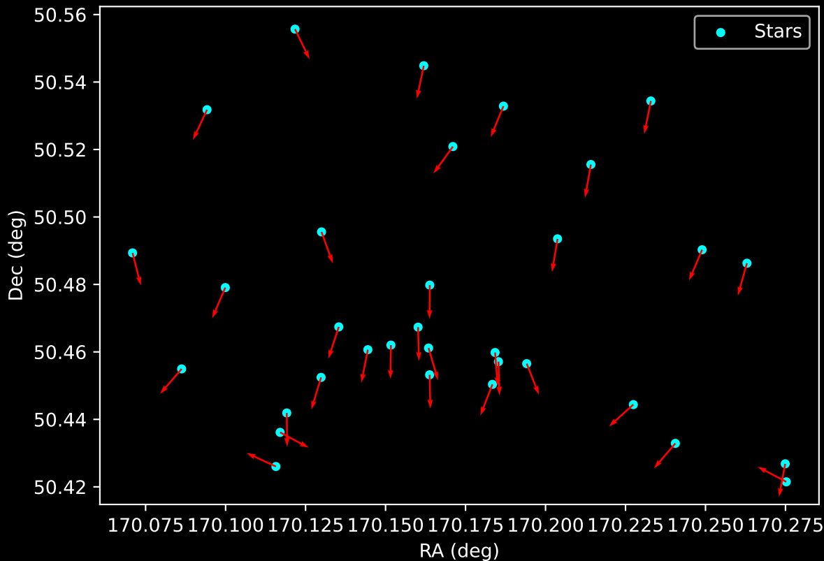
Gaia Cluster: [NGC_1624] Proper Motion Vectors for Gaia Star Field (n= 33)
