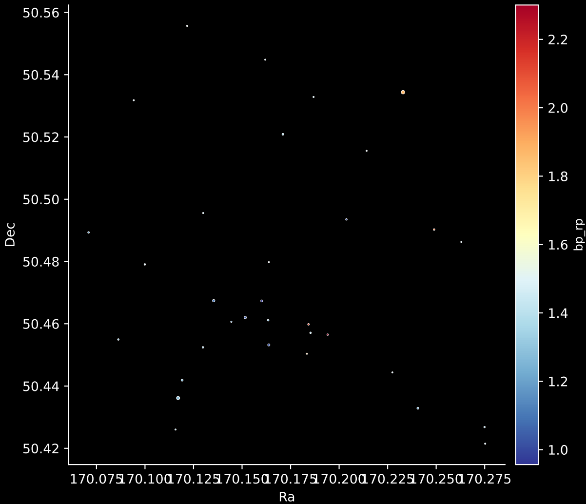
Gaia Cluster: [NGC_1624] Stars: 33
