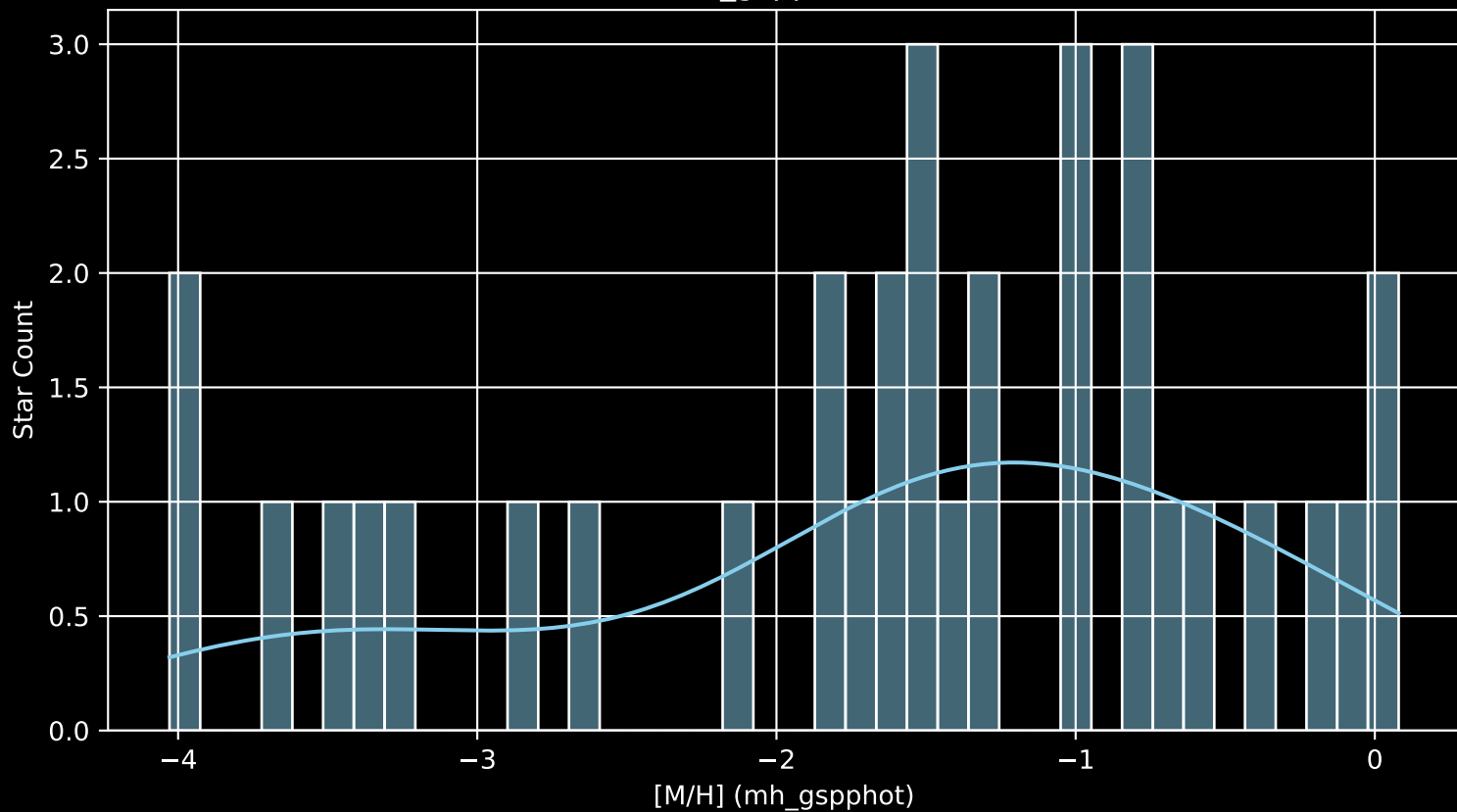
Gaia Cluster: [NGC_1624 [M/H] (mh_gspphot) (n= 33)
