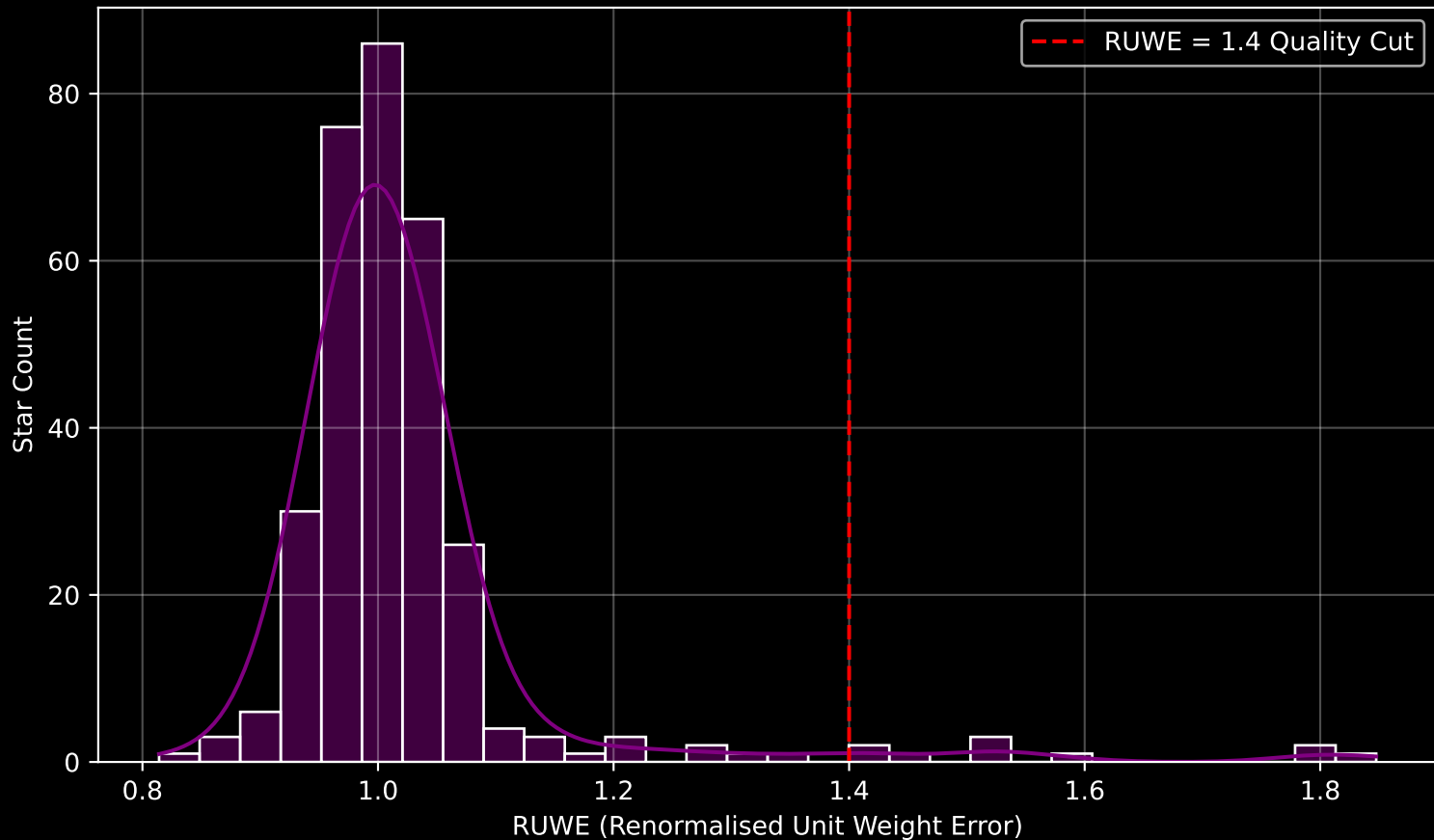
Gaia Cluster: [NGC_1664] RUWE Distribution (n= 318)
