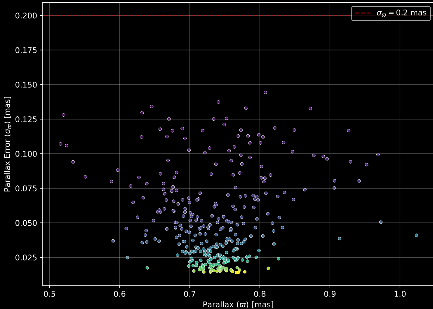
Gaia Cluster: [NGC_1664] Parallax Quality (n= 320)
