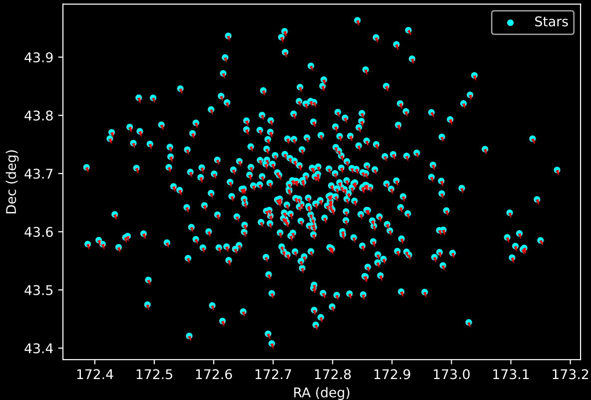
Gaia Cluster: [NGC_1664] Proper Motion Vectors for Gaia Star Field (n= 320)
