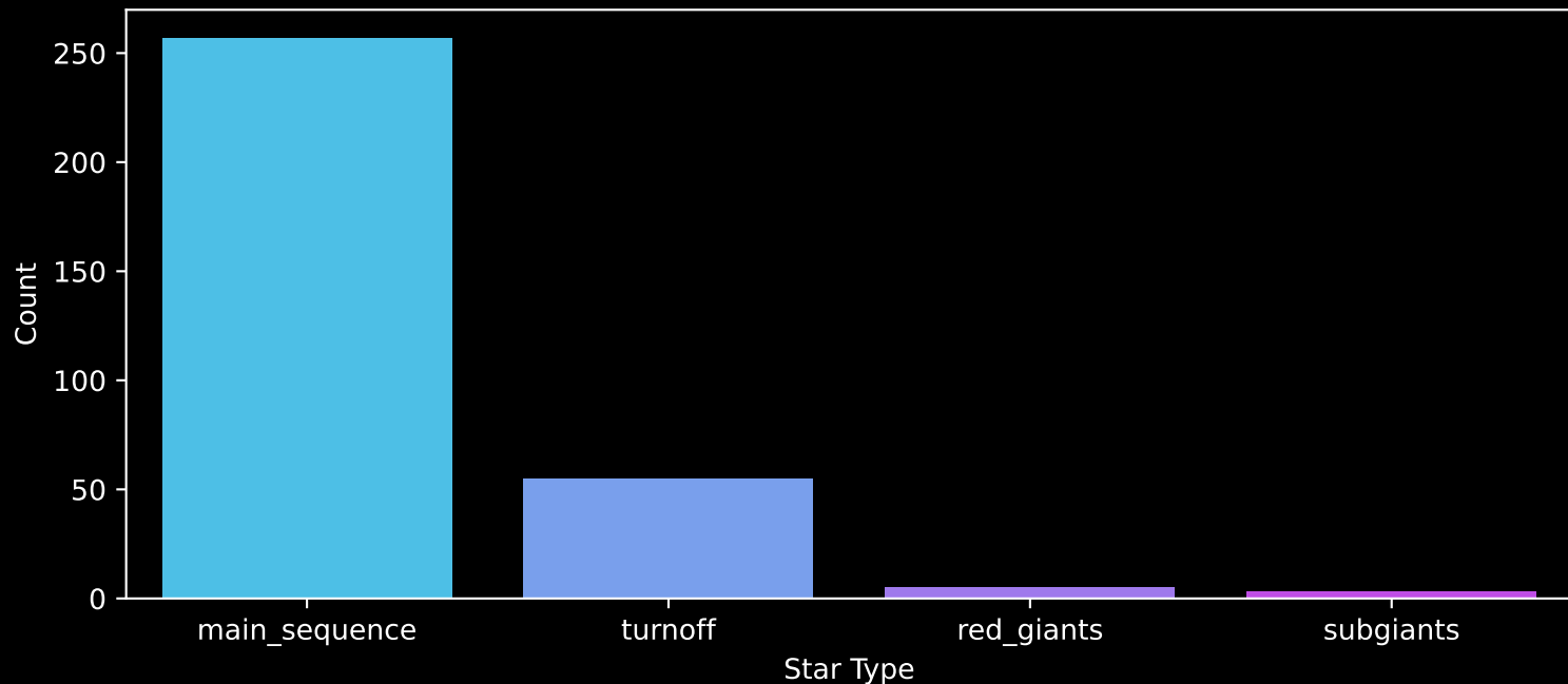
Gaia Cluster: [NGC_1664] Count plot of Star Type
