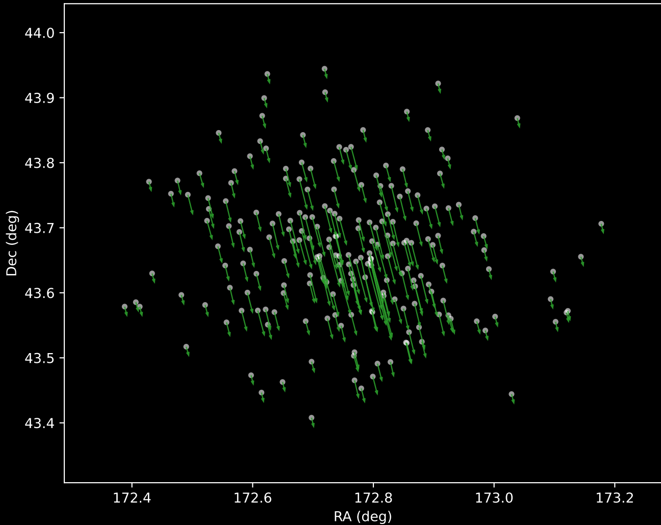
Gaia DR3 Cluster 4 Proper Motion Vectors (n=206)
