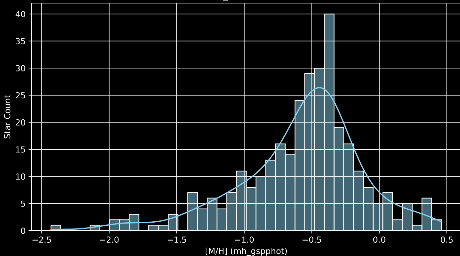
Gaia Cluster: [NGC_1664 [M/H] (mh_gspphot) (n= 319)
