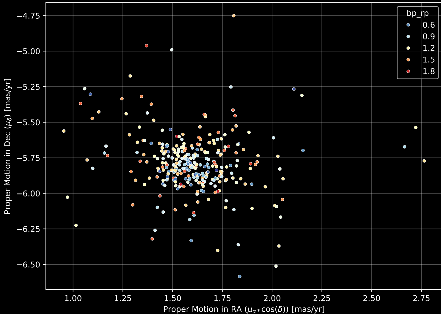
Gaia Cluster: [NGC_1664] Proper Motion Diagram (n= 320)
