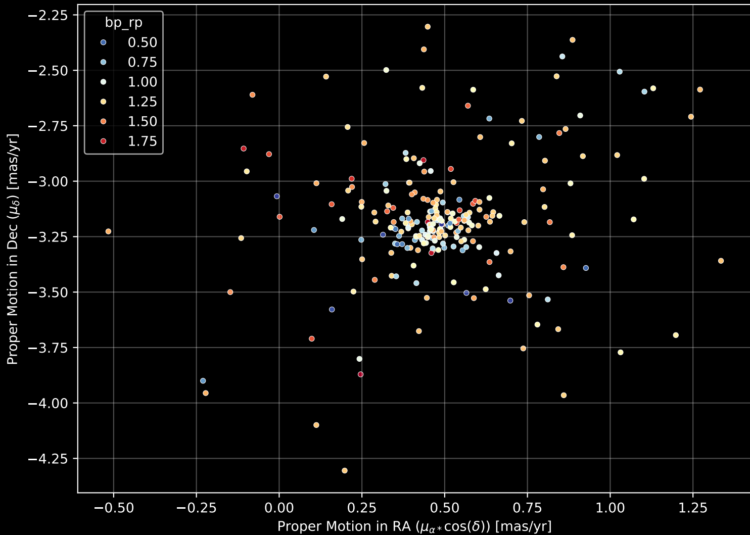
Gaia Cluster: [NGC_1778] Proper Motion Diagram (n= 243)
