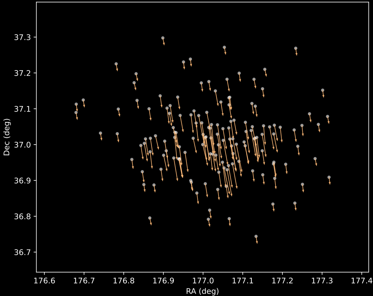
Gaia DR3 Cluster 3 Proper Motion Vectors (n=143)
