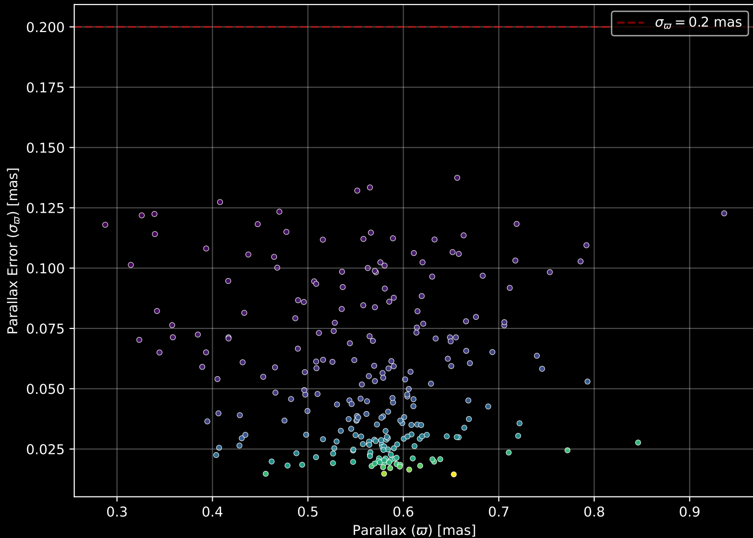
Gaia Cluster: [NGC_1778] Parallax Quality (n= 243)
