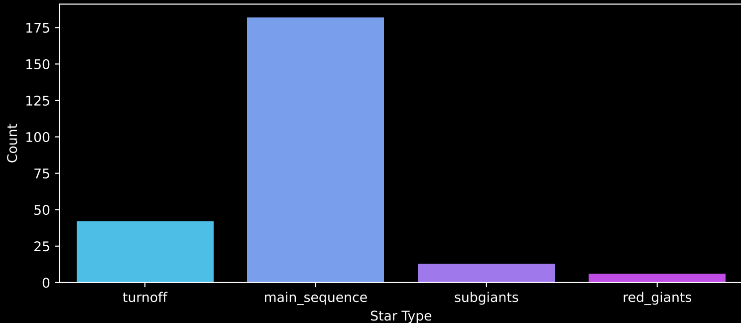
Gaia Cluster: [NGC_1778] Count plot of Star Type
