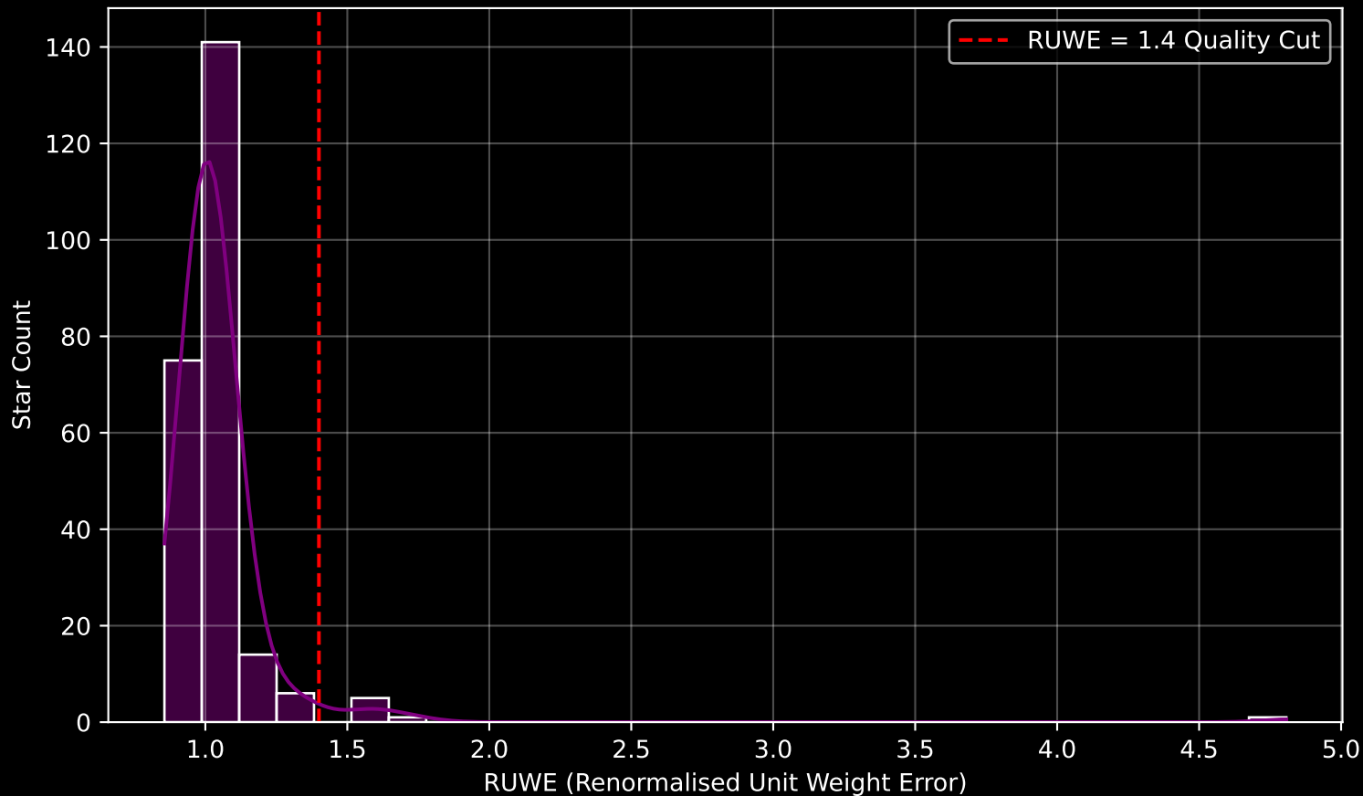
Gaia Cluster: [NGC_1778] RUWE Distribution (n= 243)
