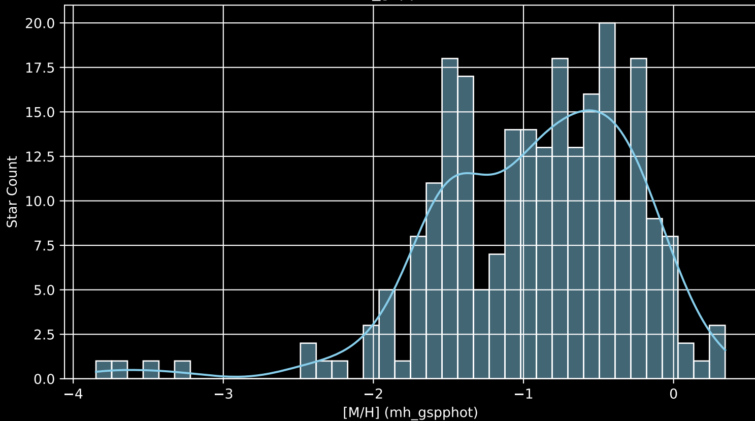
Gaia Cluster: [NGC_1778 [M/H] (mh_gspphot) (n= 242)
