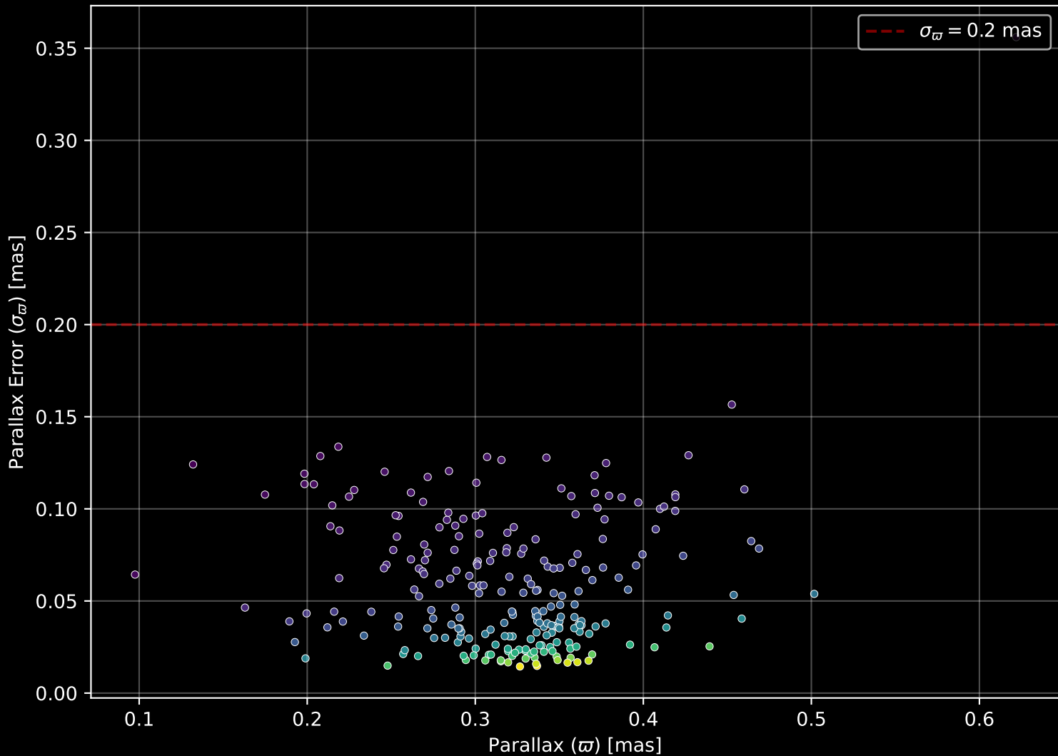
Gaia Cluster: [NGC_1857] Parallax Quality (n= 236)
