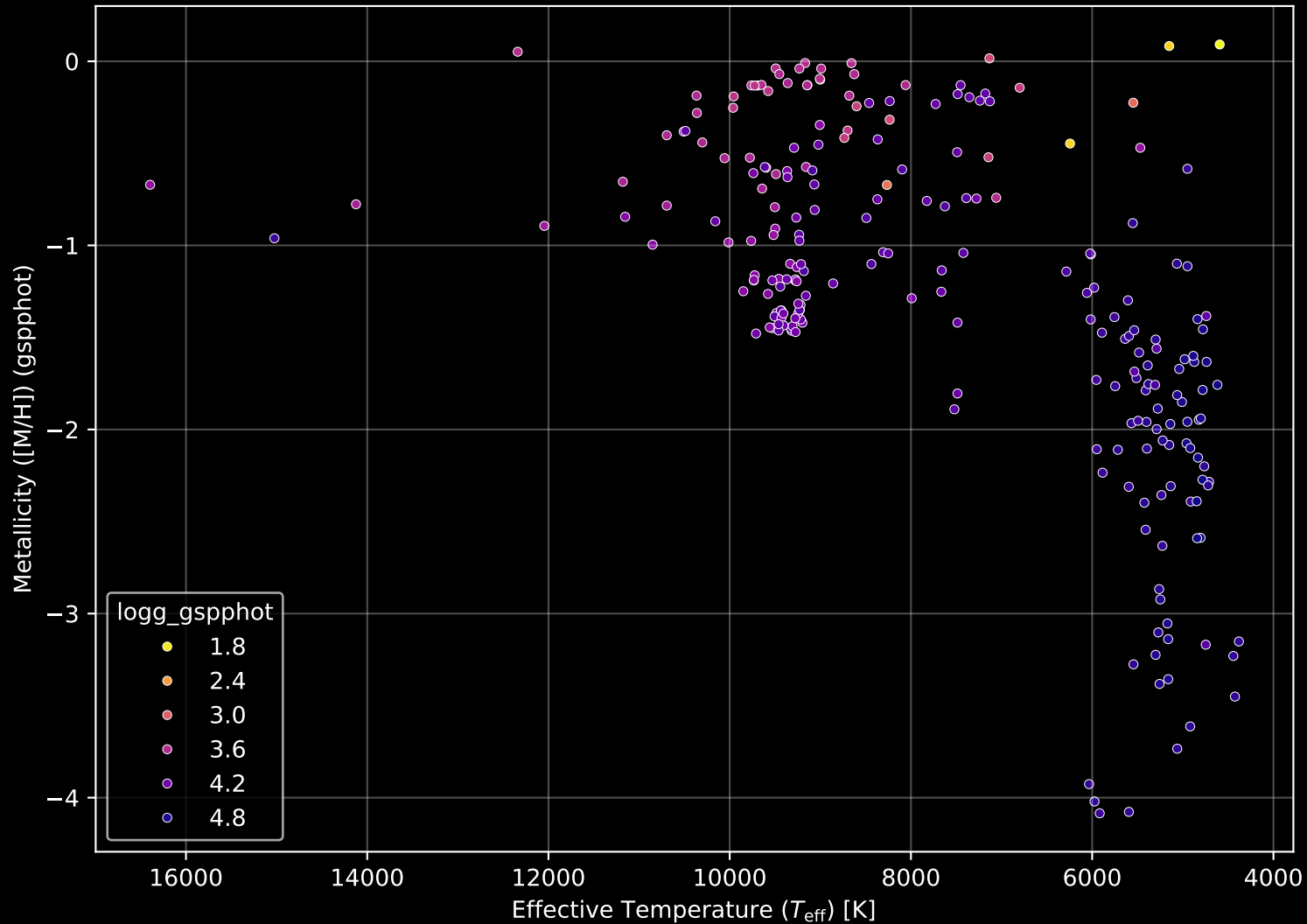
Gaia Cluster: [NGC_1857] Stellar Population Parameters (n= 236)
