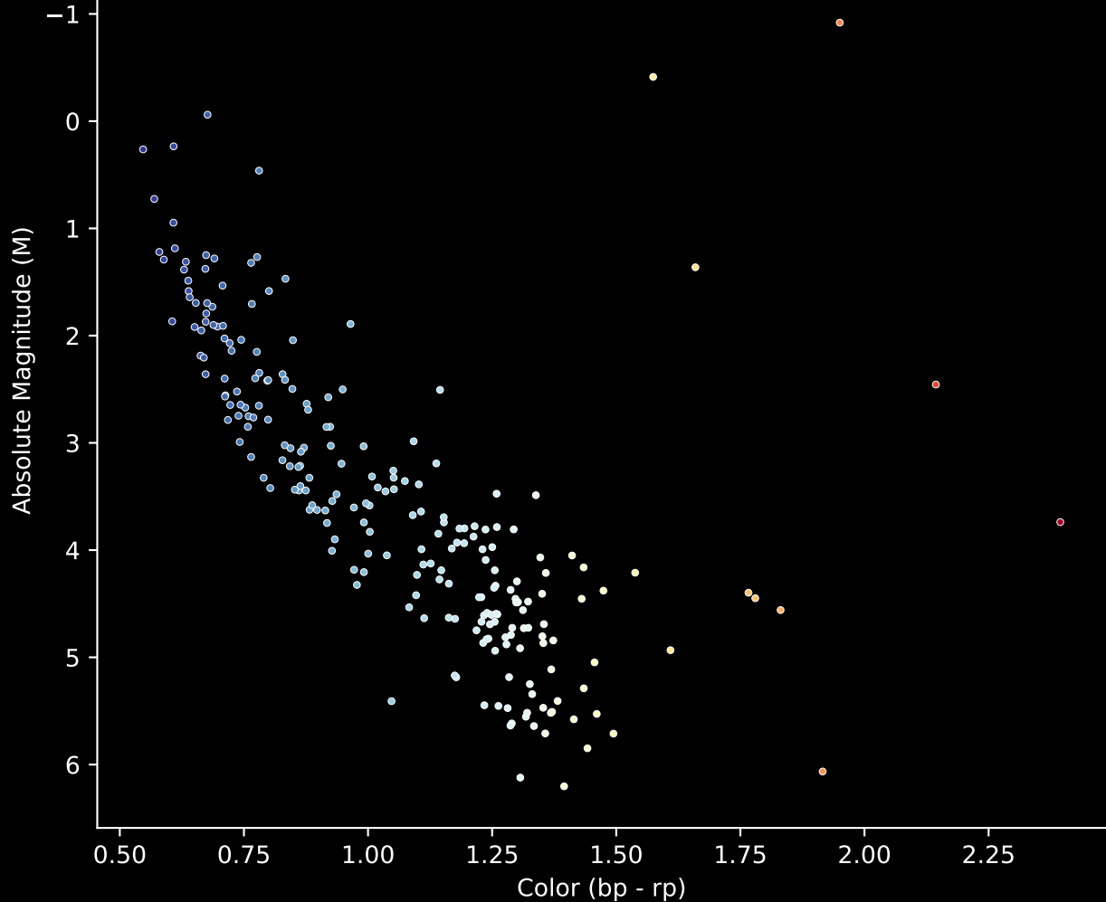
Gaia Cluster: [NGC_1857] Stars (n= 236) Hertzprung-Russel Diagram
