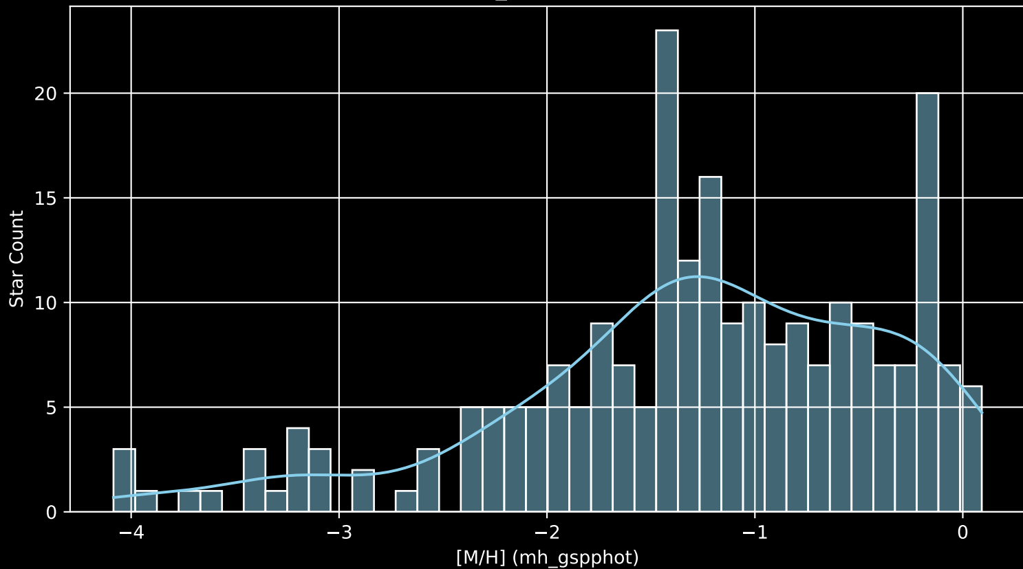
Gaia Cluster: [NGC_1857 [M/H] (mh_gspphot) (n= 236)
