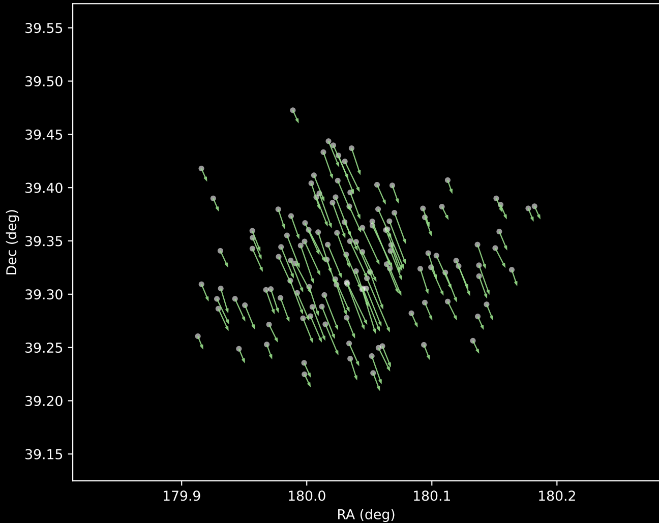
Gaia DR3 Cluster 5 Proper Motion Vectors (n=125)
