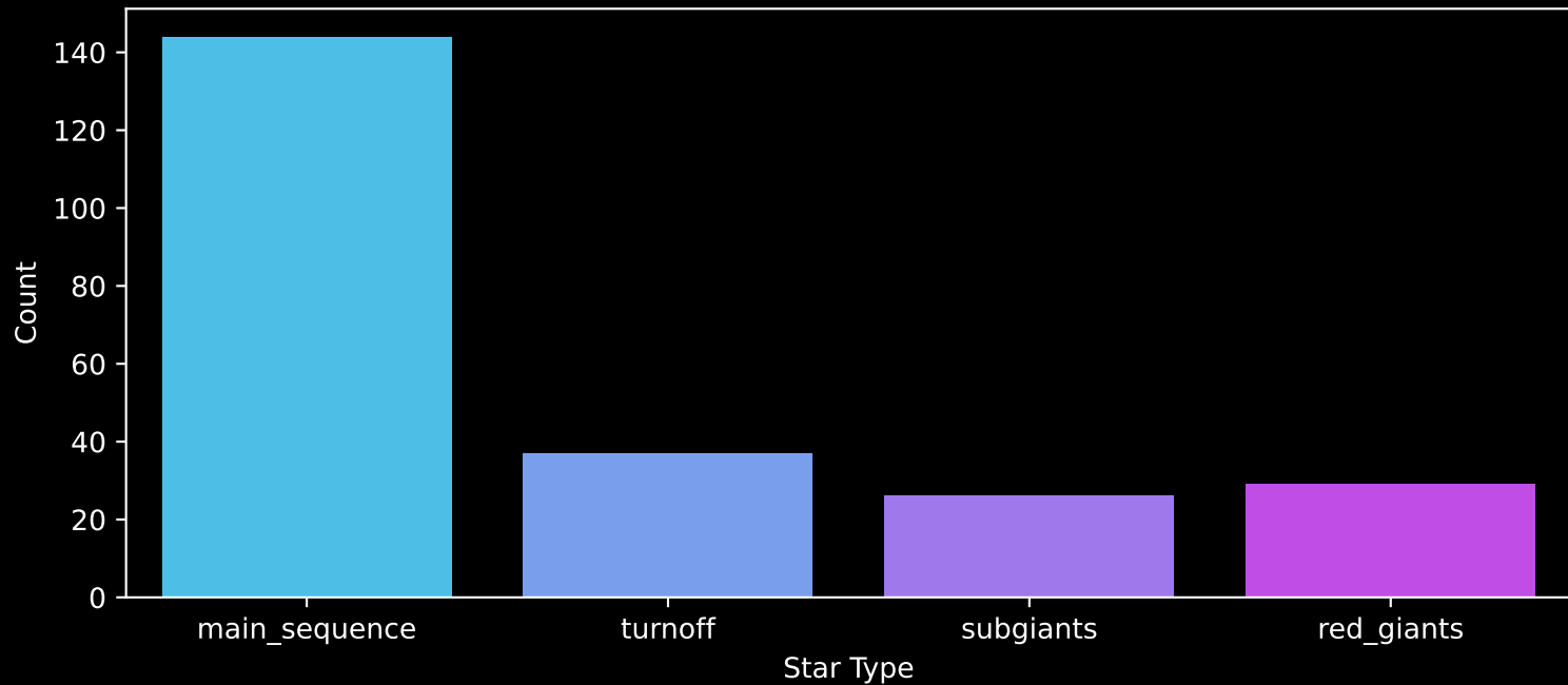
Gaia Cluster: [NGC_1857] Count plot of Star Type
