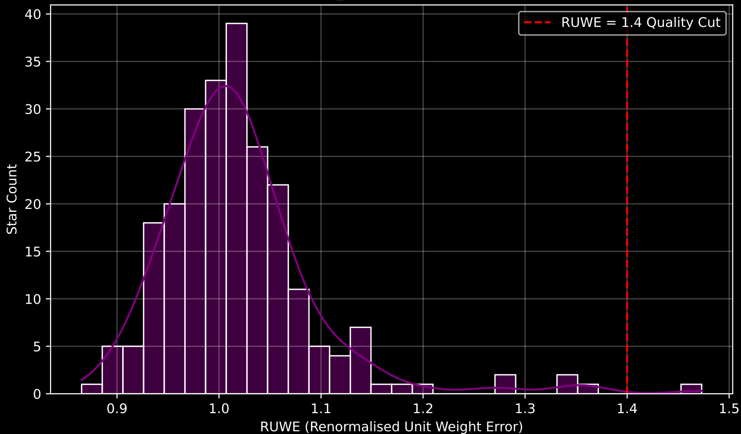
Gaia Cluster: [NGC_1857] RUWE Distribution (n= 235)
