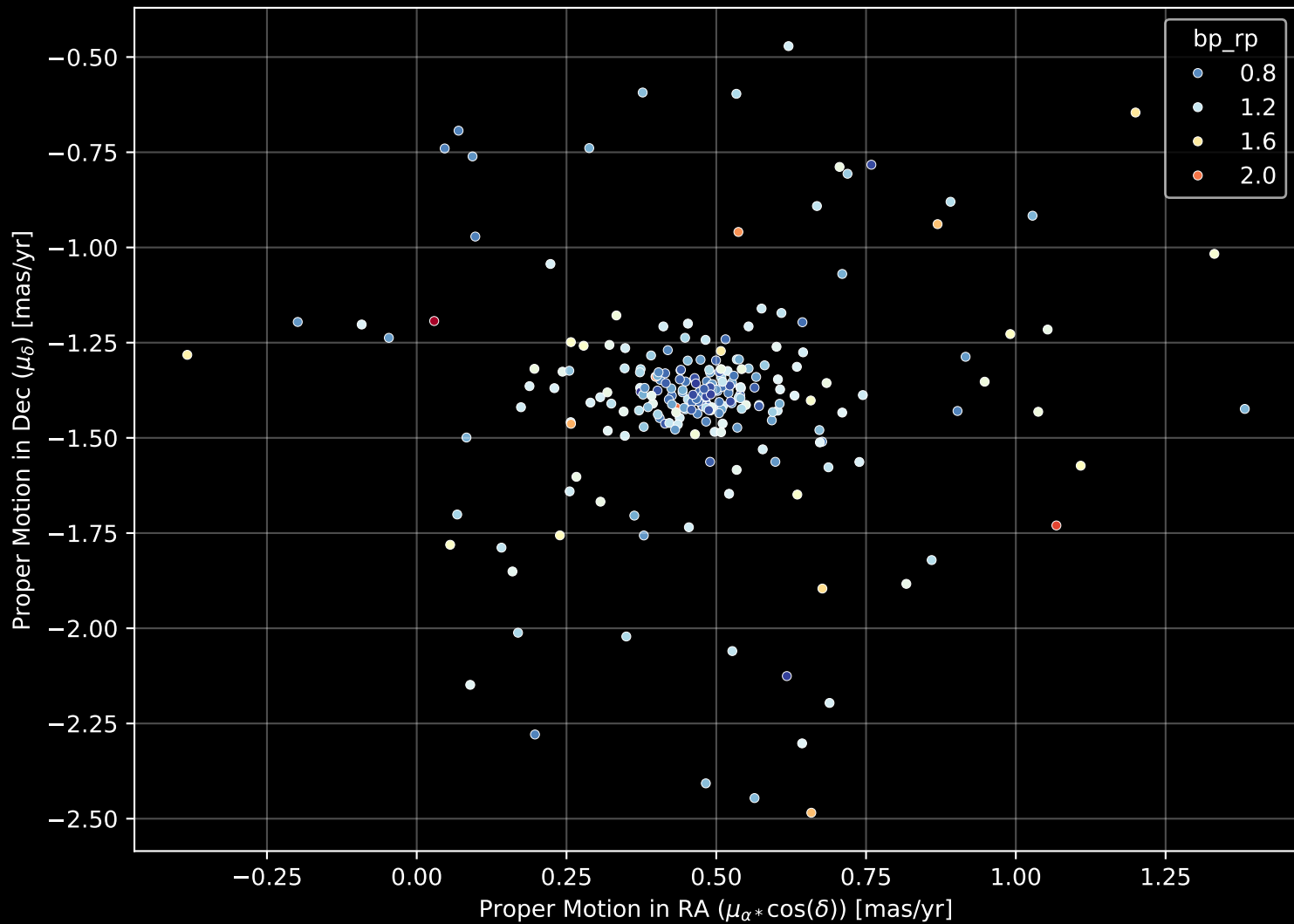
Gaia Cluster: [NGC_1857] Proper Motion Diagram (n= 236)
