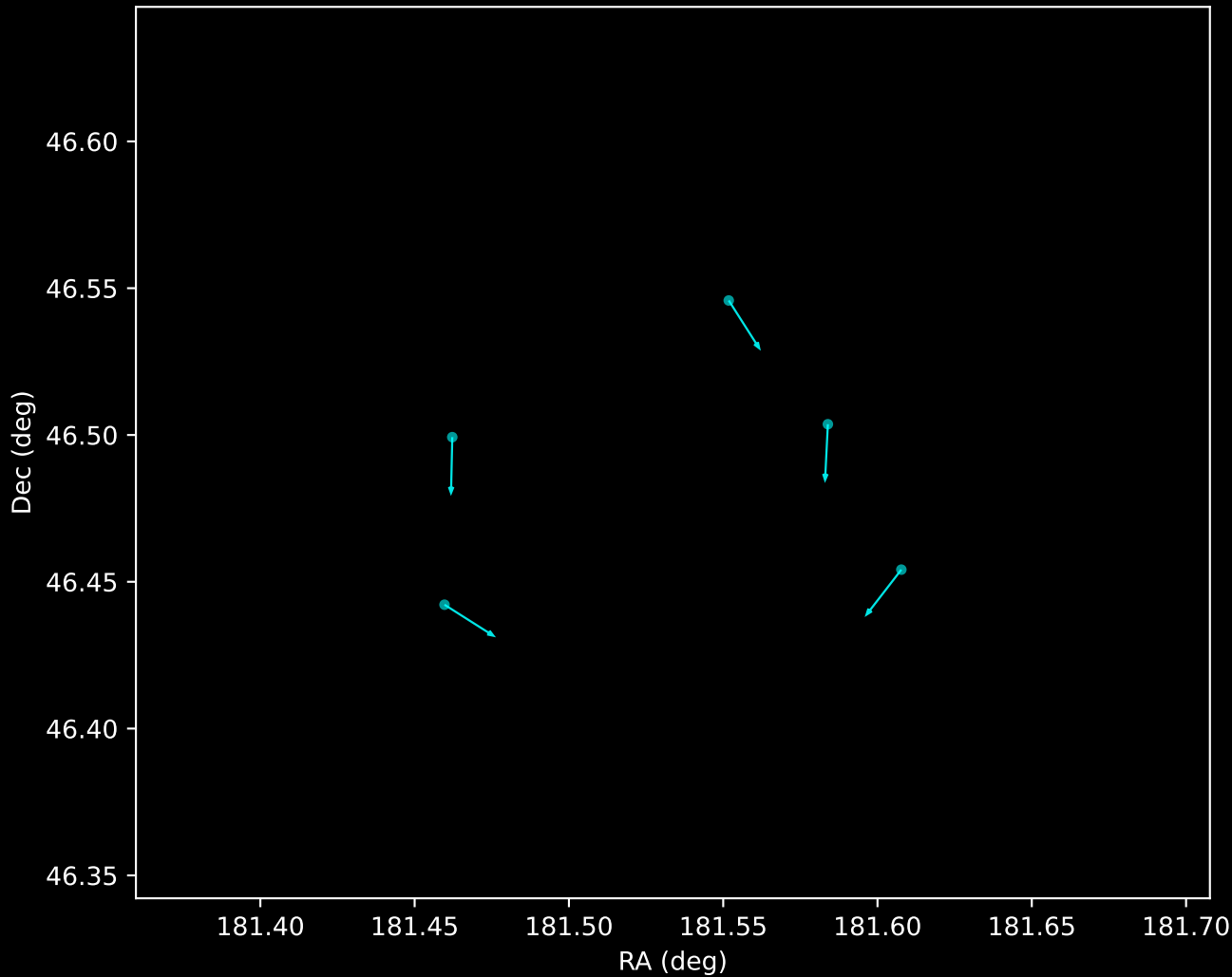
Gaia DR3 Noise Stream Proper Motion Vectors (n=5)
