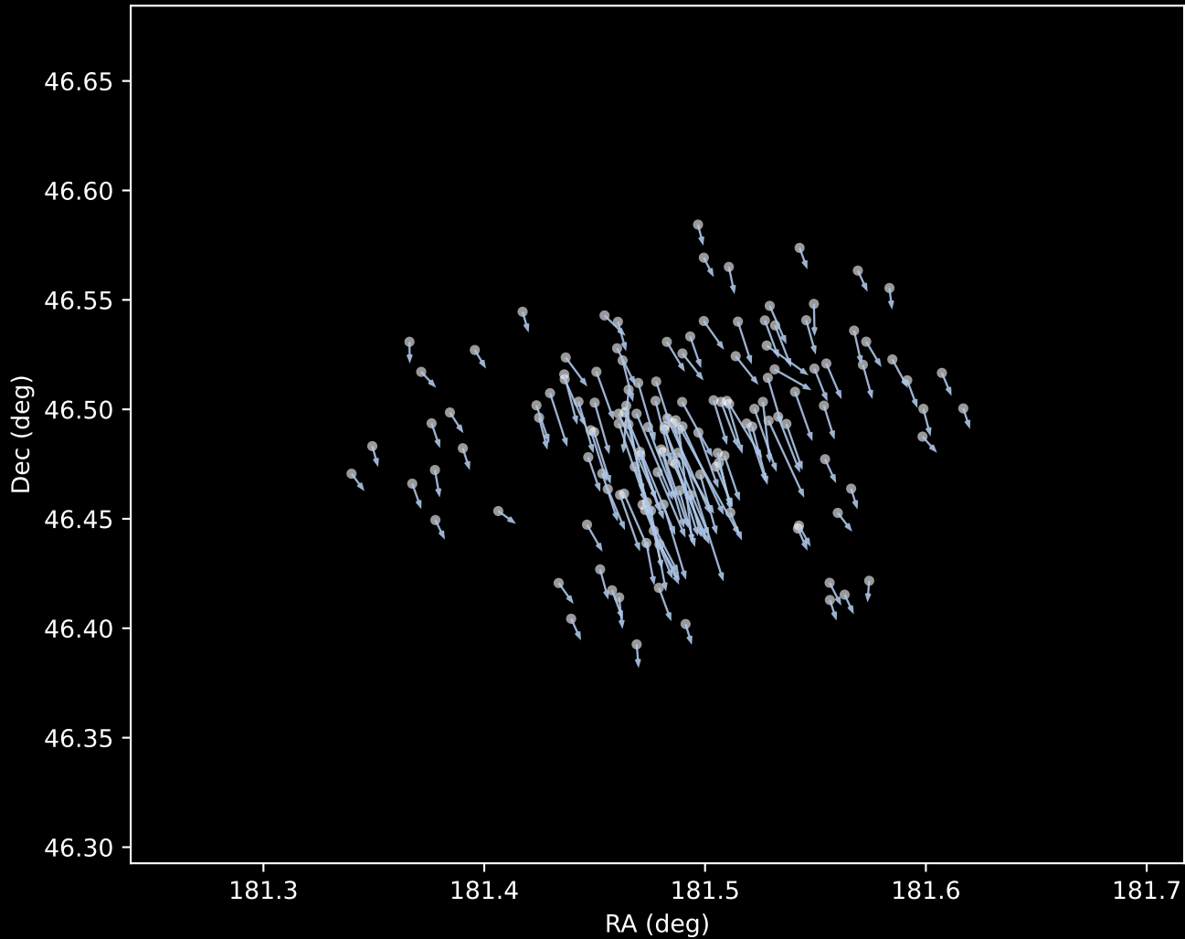
Gaia DR3 Cluster 1 Proper Motion Vectors (n=140)
