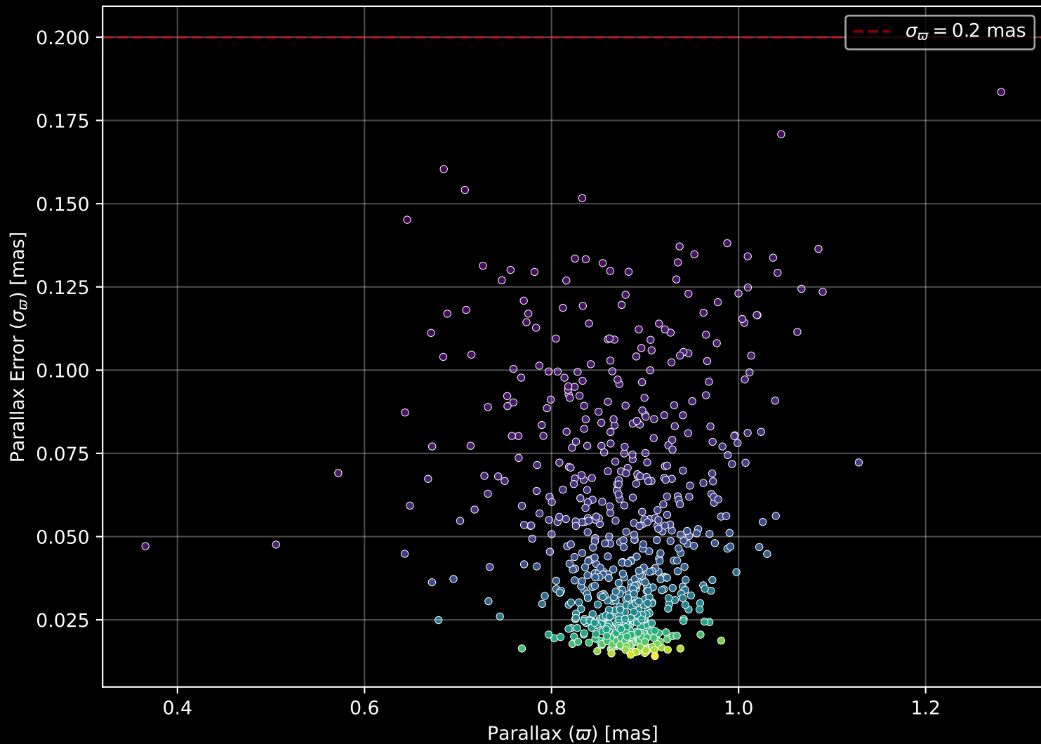
Gaia Cluster: [NGC_1912] Parallax Quality (n= 668)
