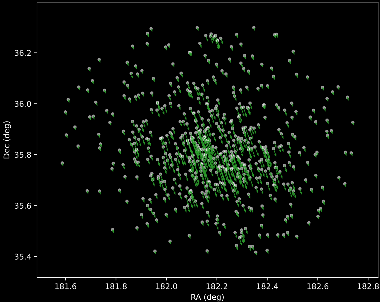
Gaia DR3 Cluster 4 Proper Motion Vectors (n=580)
