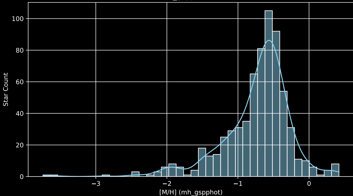
Gaia Cluster: [NGC_1912 [M/H] (mh_gspphot) (n= 668)
