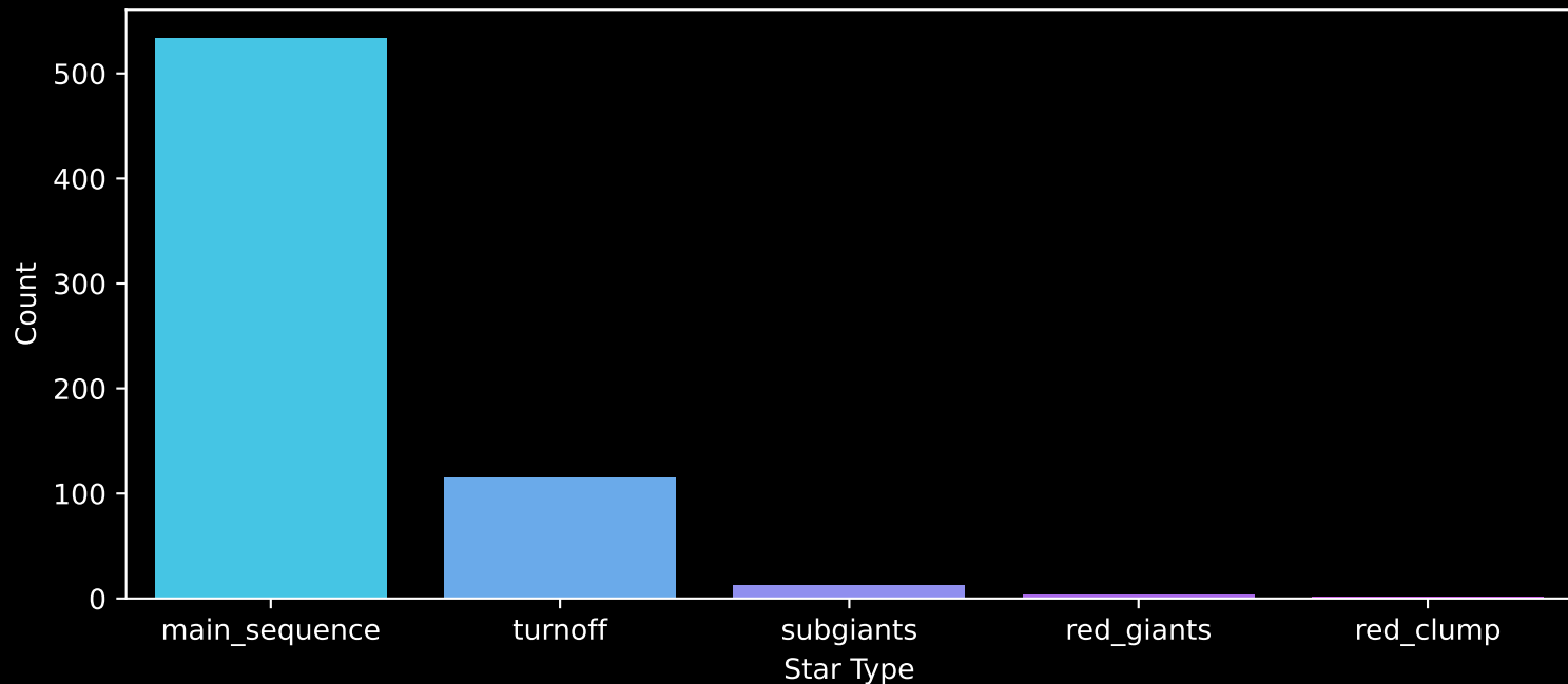
Gaia Cluster: [NGC_1912] Count plot of Star Type
