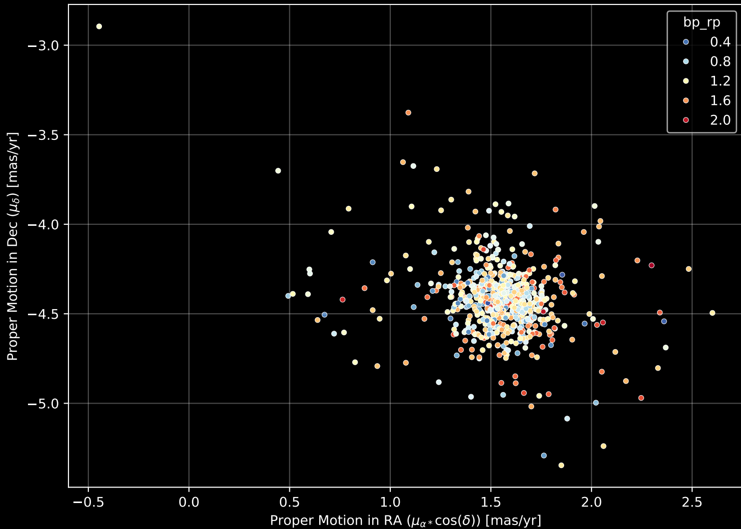
Gaia Cluster: [NGC_1912] Proper Motion Diagram (n= 668)
