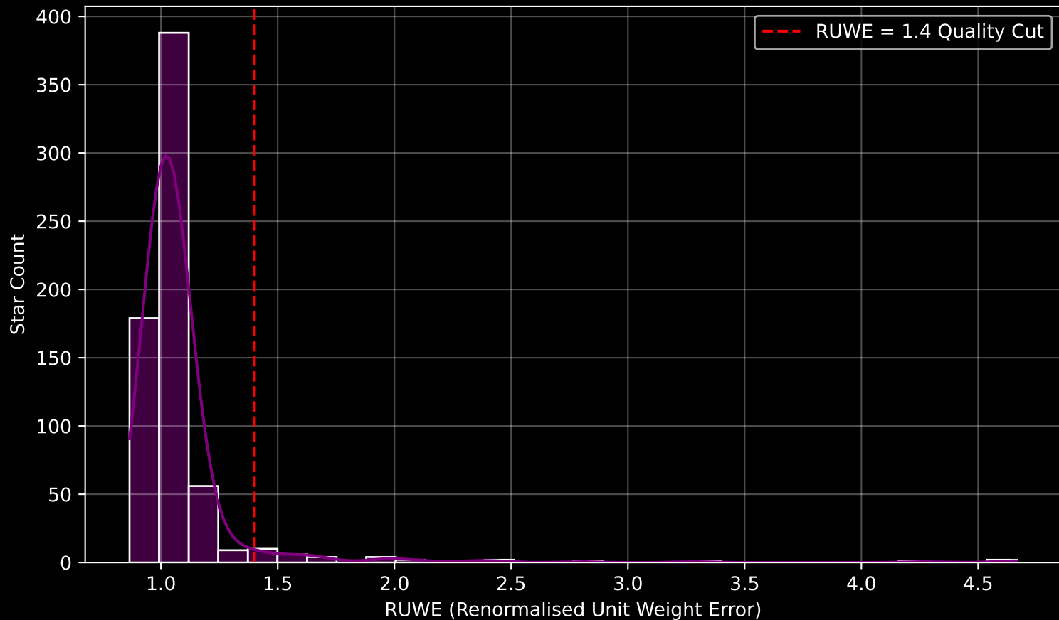
Gaia Cluster: [NGC_1912] RUWE Distribution (n= 666)
