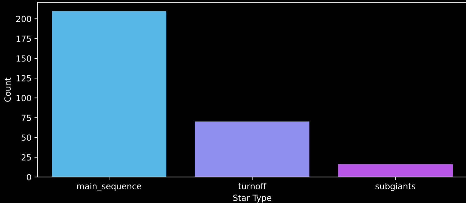
Gaia Cluster: [NGC_1960] Count plot of Star Type
