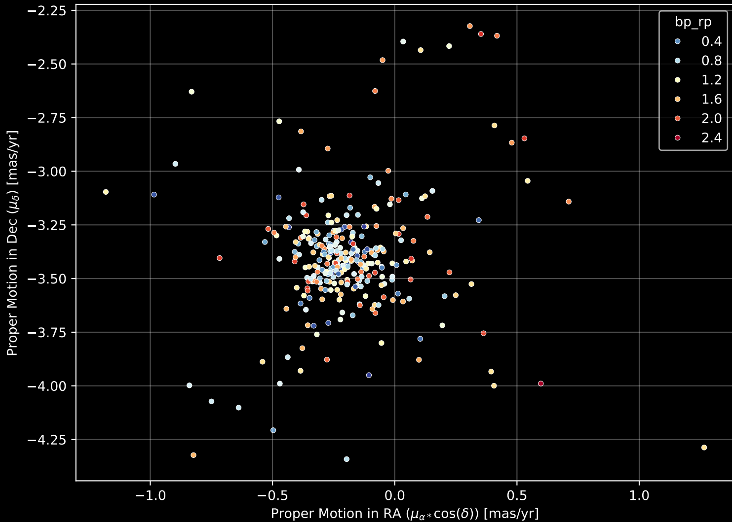
Gaia Cluster: [NGC_1960] Proper Motion Diagram (n= 296)
