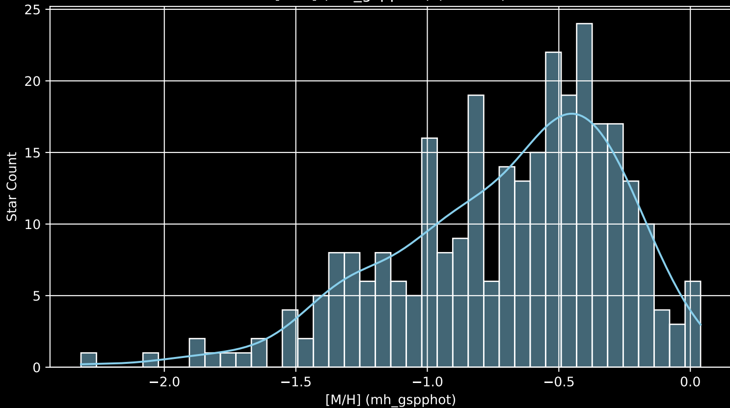
Gaia Cluster: [NGC_1960 [M/H] (mh_gspphot) (n= 296)
