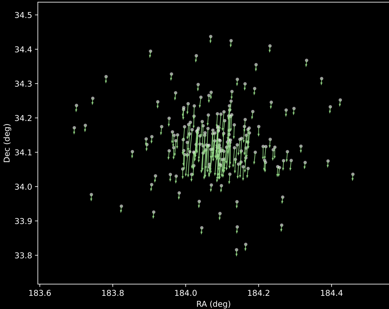
Gaia DR3 Cluster 5 Proper Motion Vectors (n=184)
