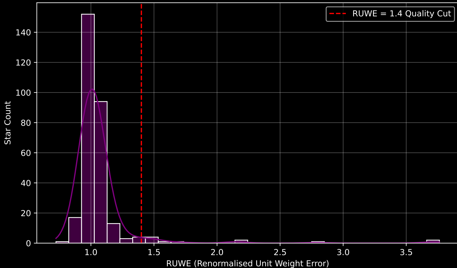
Gaia Cluster: [NGC_1960] RUWE Distribution (n= 295)
