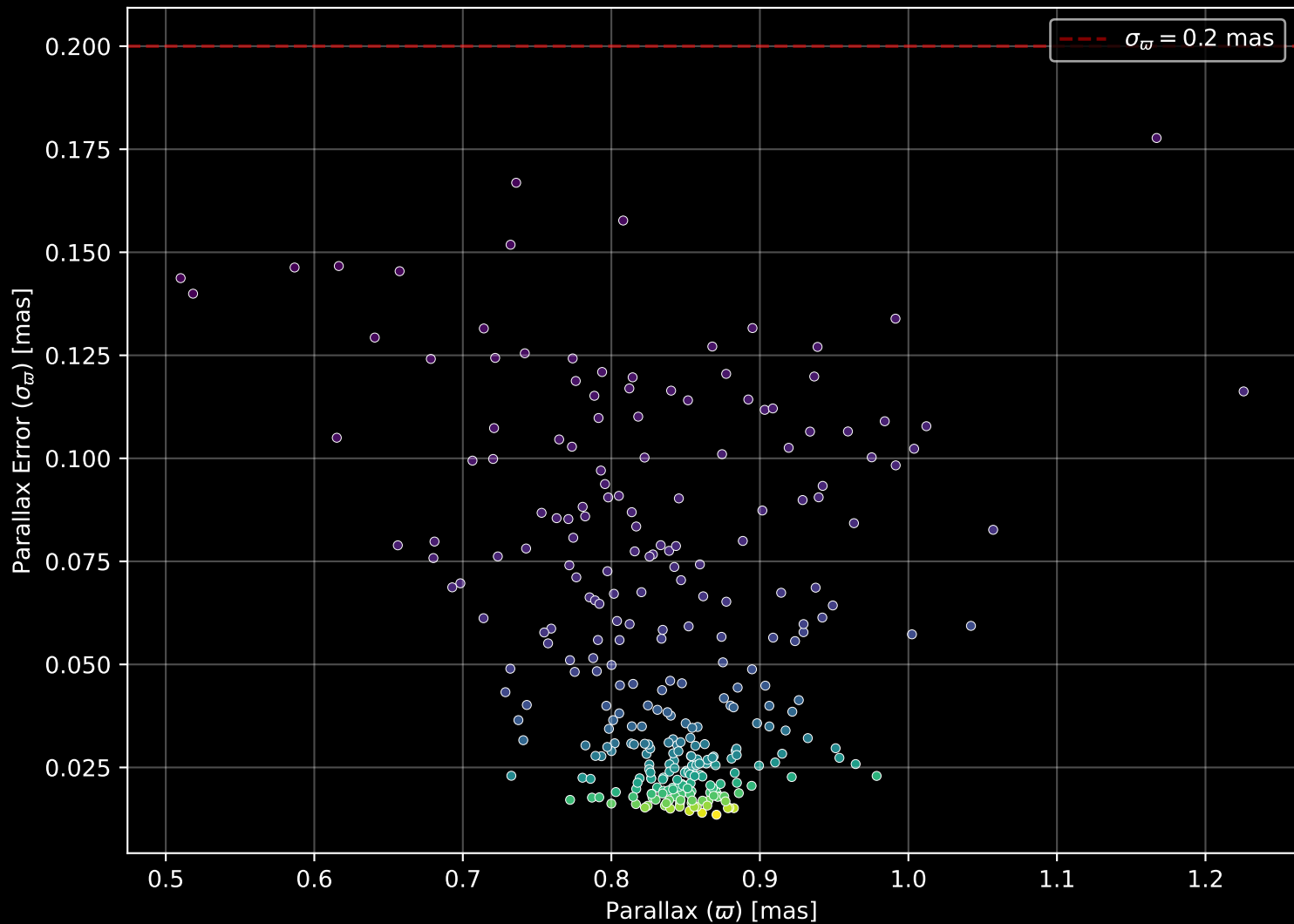
Gaia Cluster: [NGC_1960] Parallax Quality (n= 296)
