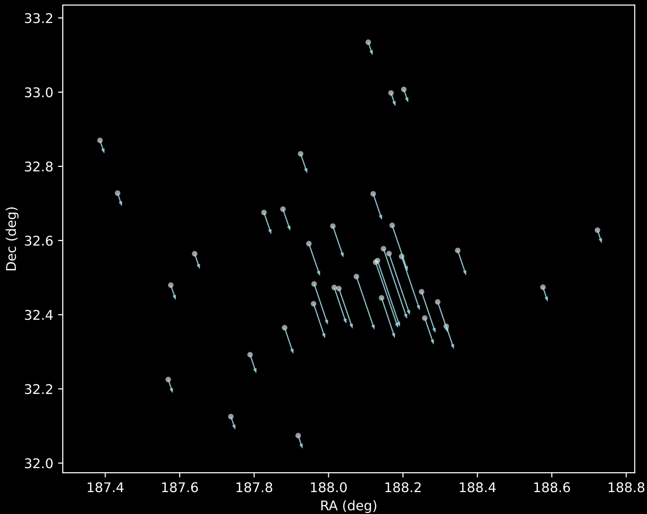
Gaia DR3 Cluster 79 Proper Motion Vectors (n=37)
