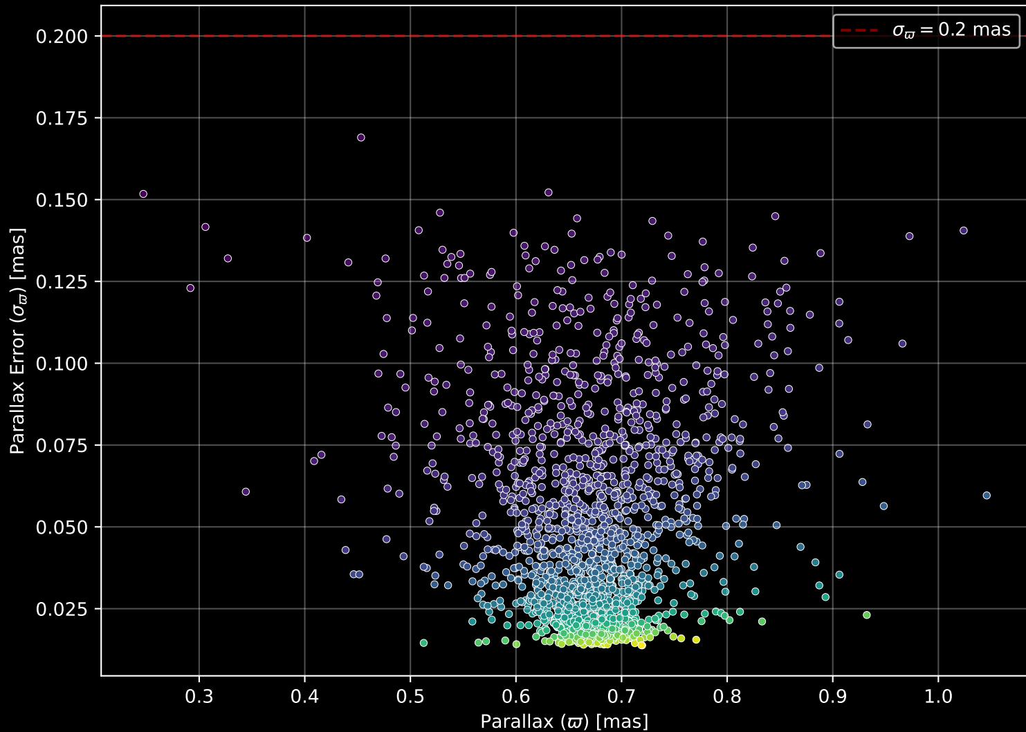
Gaia Cluster: [NGC_2099] Parallax Quality (n= 1644)
