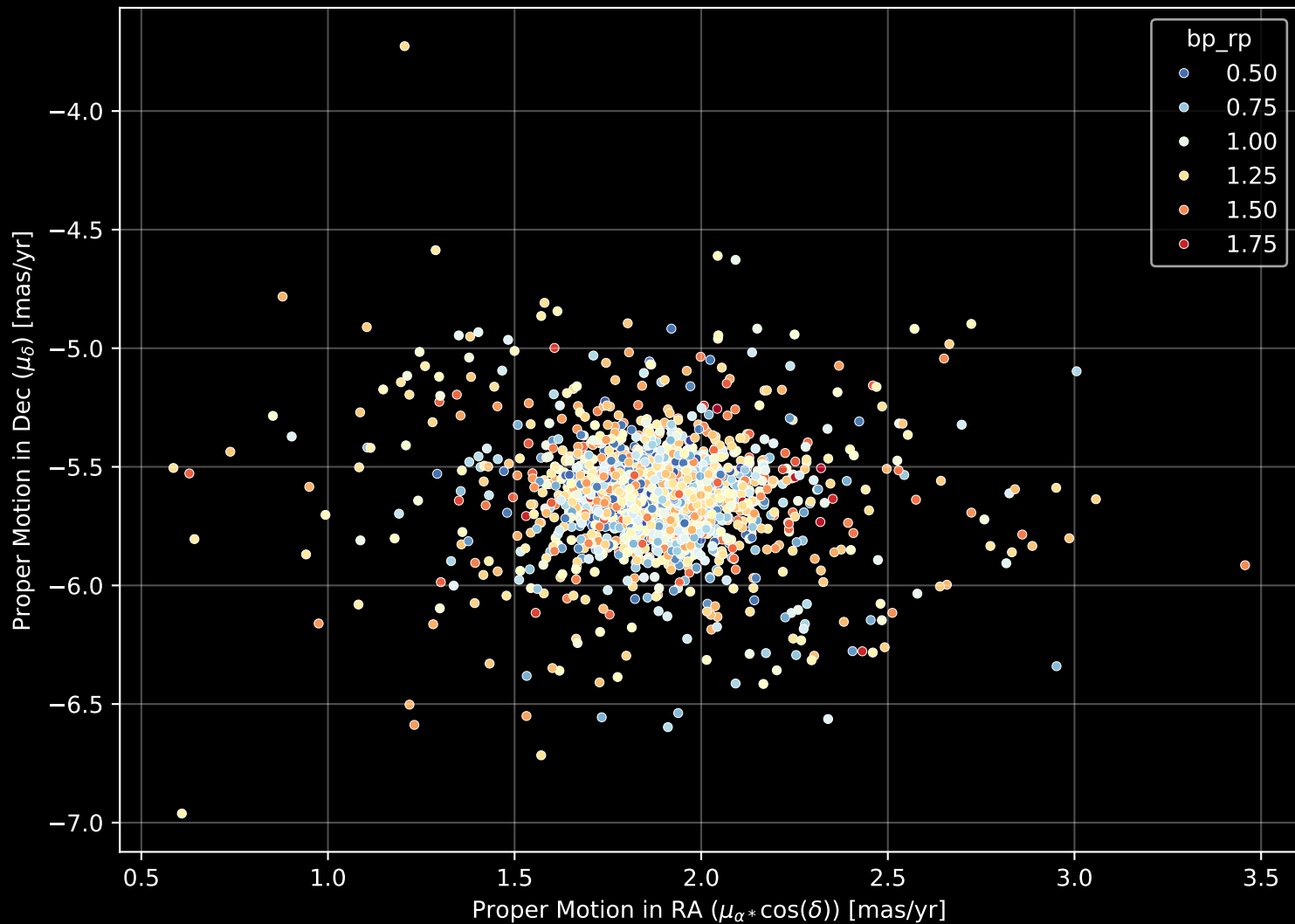
Gaia Cluster: [NGC_2099] Proper Motion Diagram (n= 1644)
