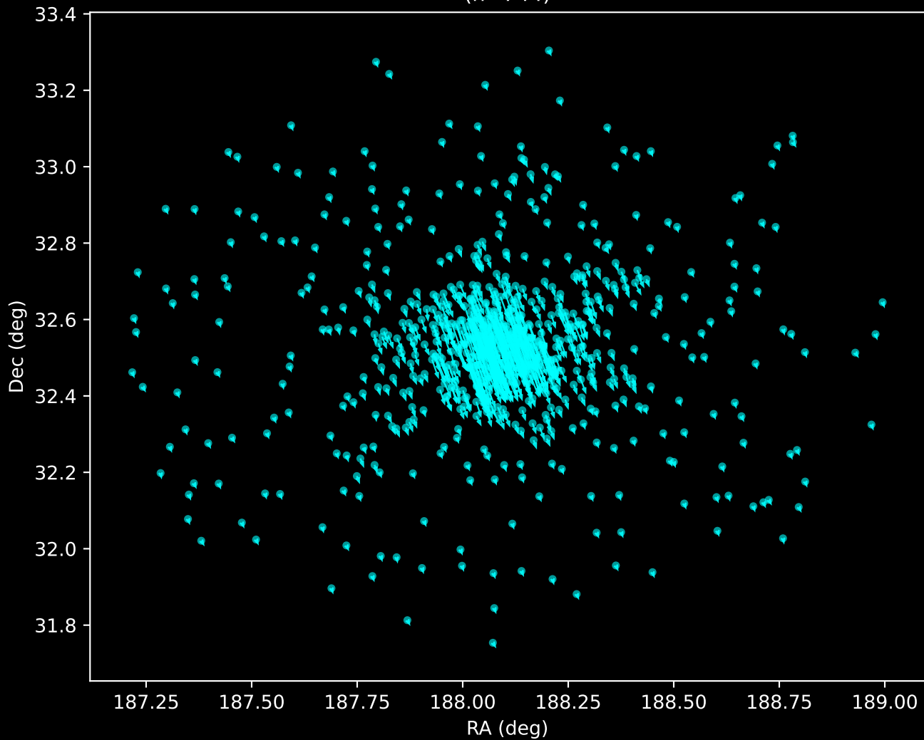
Gaia DR3 Noise Stream Proper Motion Vectors (n=744)
