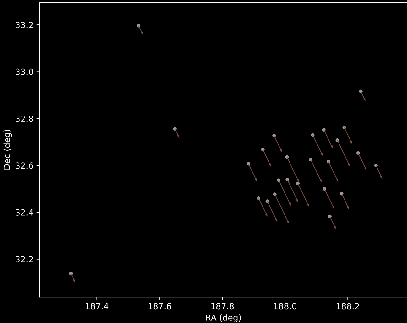
Gaia DR3 Cluster 50 Proper Motion Vectors (n=25)
