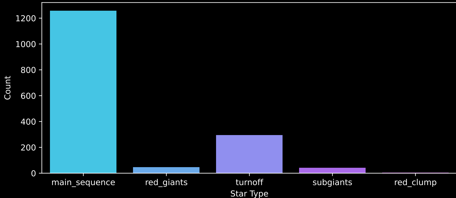
Gaia Cluster: [NGC_2099] Count plot of Star Type
