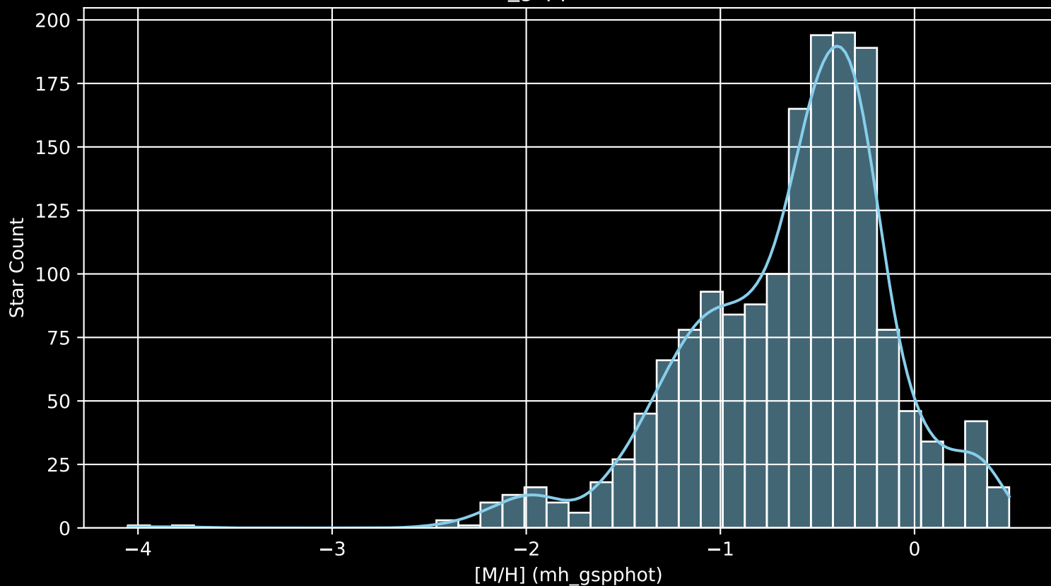
Gaia Cluster: [NGC_2099 [M/H] (mh_gspphot) (n= 1644)
