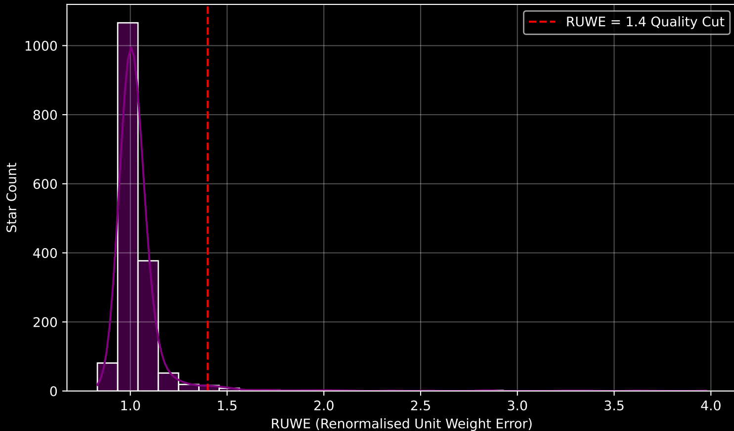
Gaia Cluster: [NGC_2099] RUWE Distribution (n= 1640)
