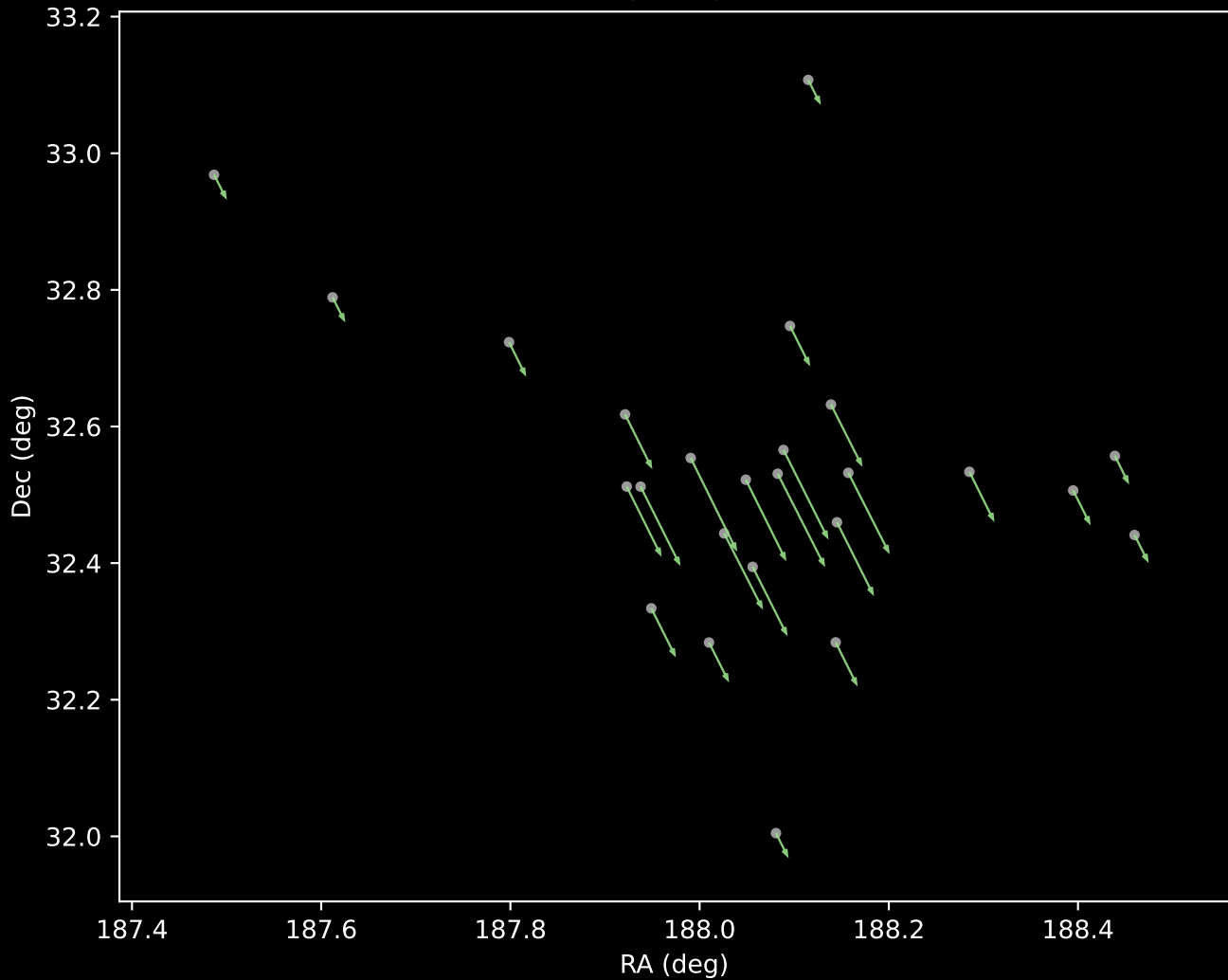
Gaia DR3 Cluster 65 Proper Motion Vectors (n=25)
