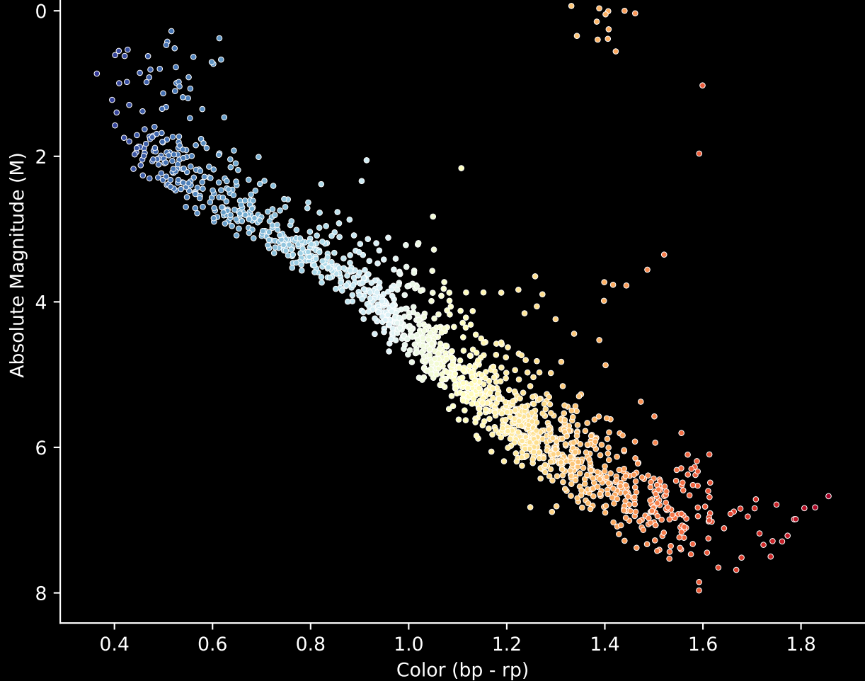
Gaia Cluster: [NGC_2099] Stars (n= 1644) Hertzprung-Russel Diagram
