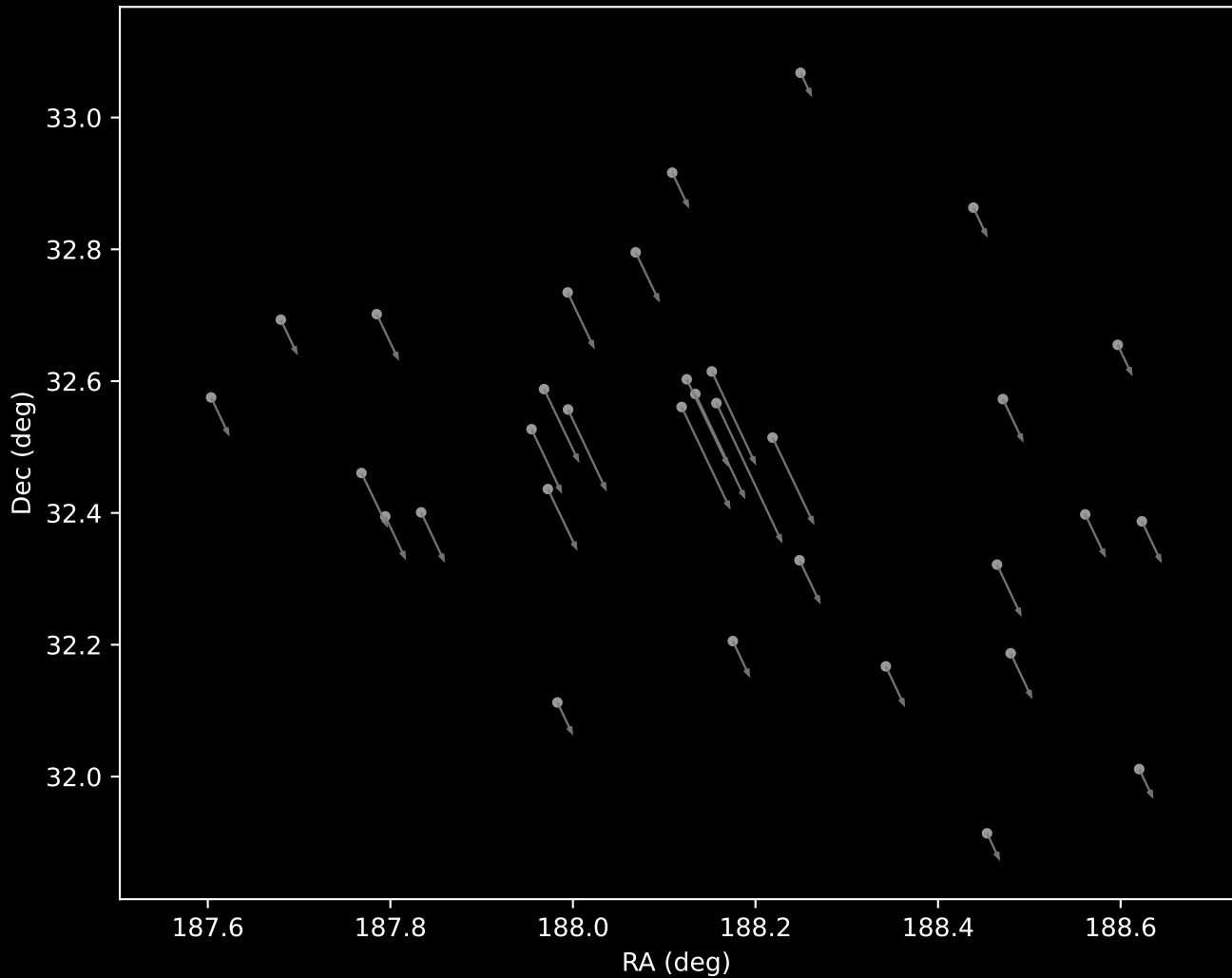
Gaia DR3 Cluster 74 Proper Motion Vectors (n=33)
