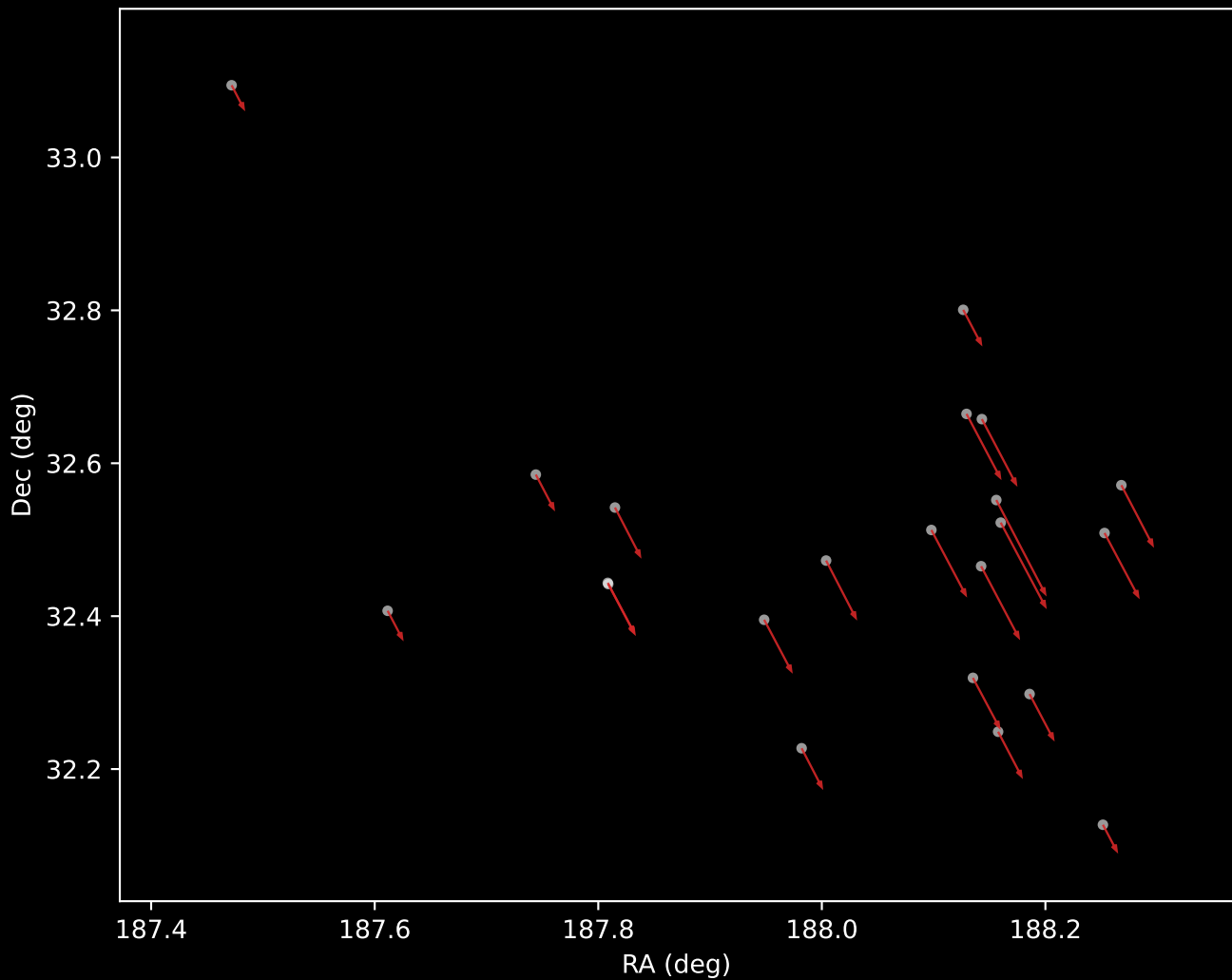
Gaia DR3 Cluster 66 Proper Motion Vectors (n=22)
