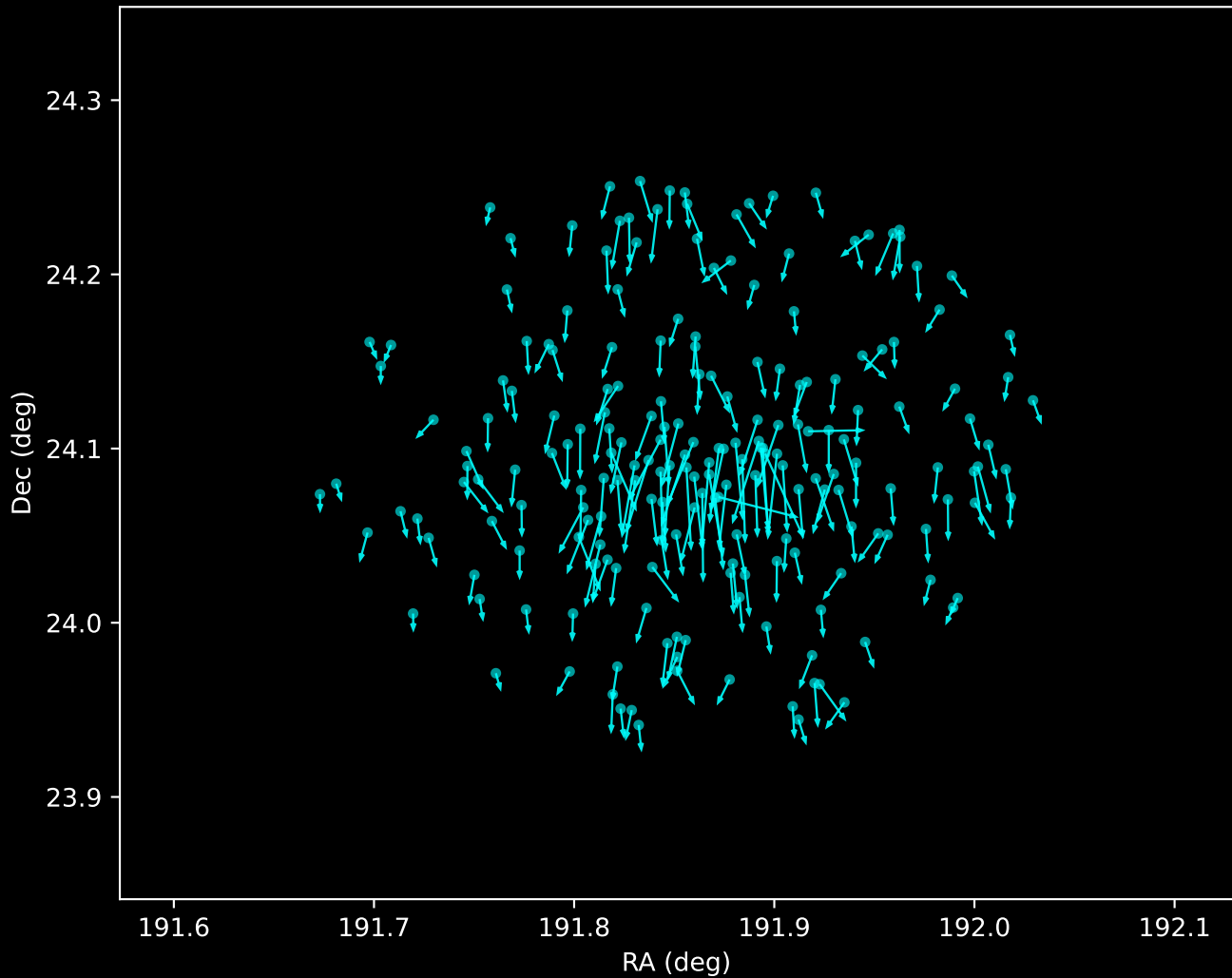
Gaia DR3 Noise Stream Proper Motion Vectors (n=204)
