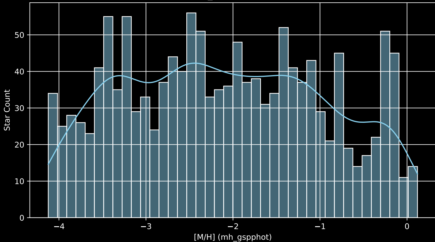
Gaia Cluster: [NGC_2158 [M/H] (mh_gspphot) (n= 1389)
