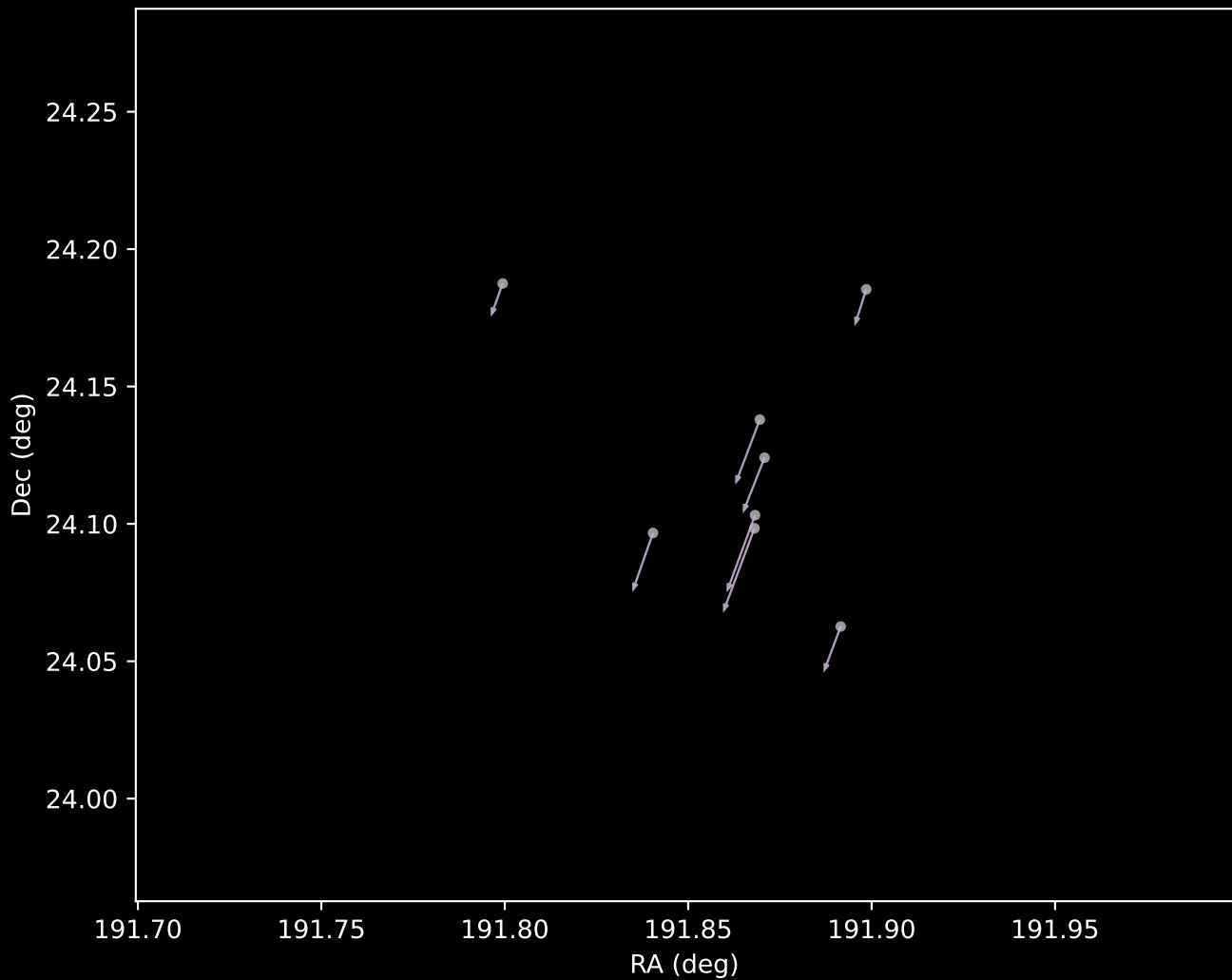
Gaia DR3 Cluster 9 Proper Motion Vectors (n=8)
