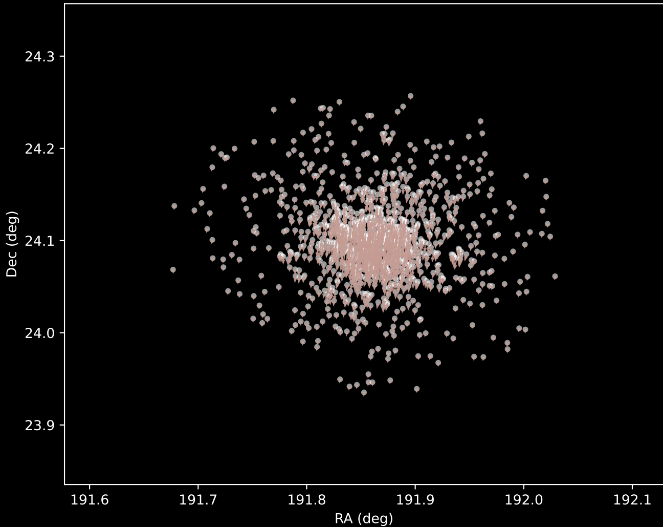
Gaia DR3 Cluster 11 Proper Motion Vectors (n=1108)
