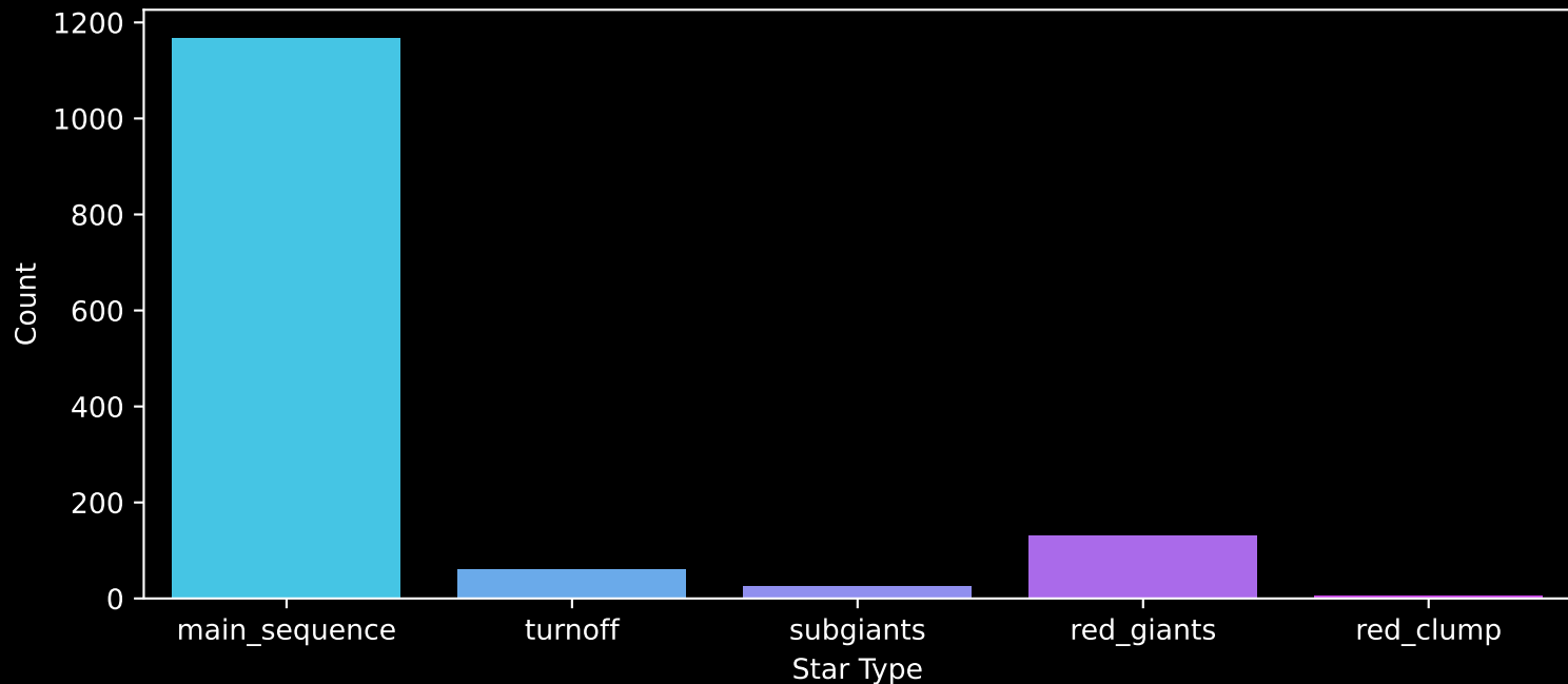
Gaia Cluster: [NGC_2158] Count plot of Star Type
