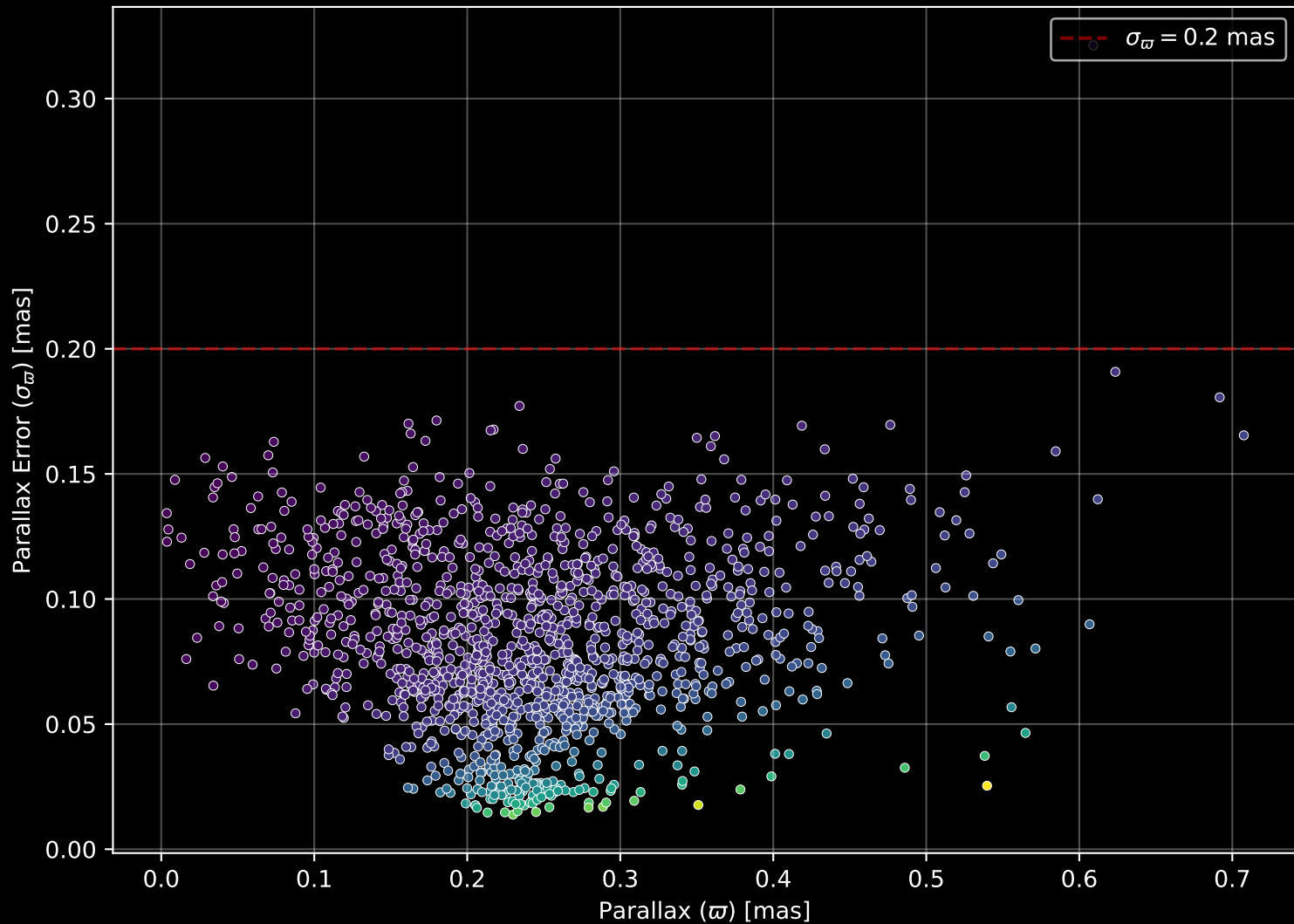
Gaia Cluster: [NGC_2158] Parallax Quality (n= 1390)
