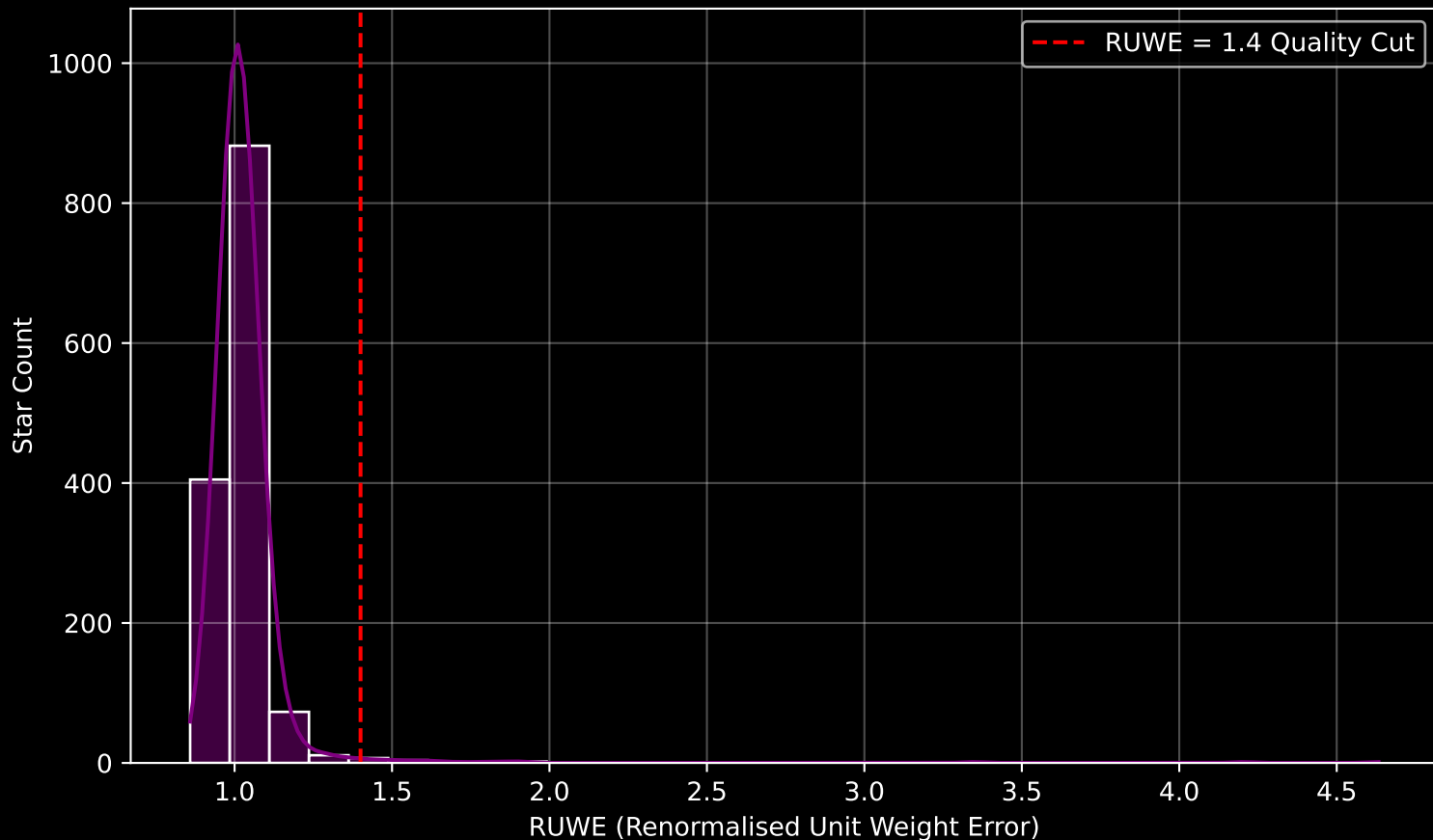
Gaia Cluster: [NGC_2158] RUWE Distribution (n= 1389)
