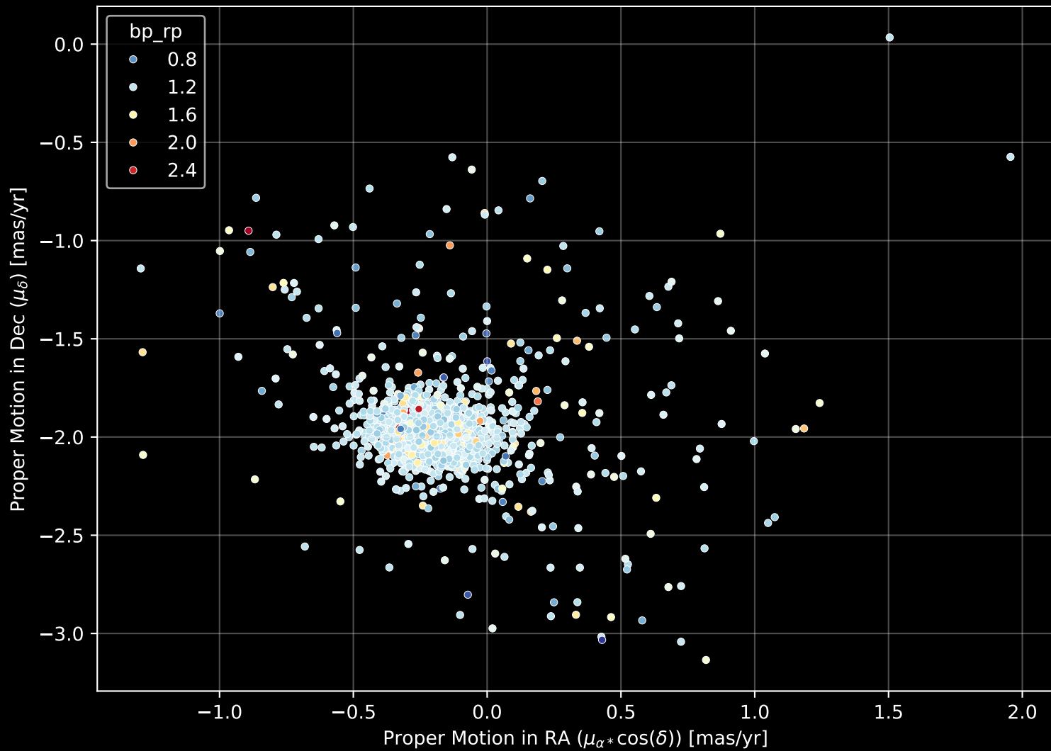
Gaia Cluster: [NGC_2158] Proper Motion Diagram (n= 1390)
