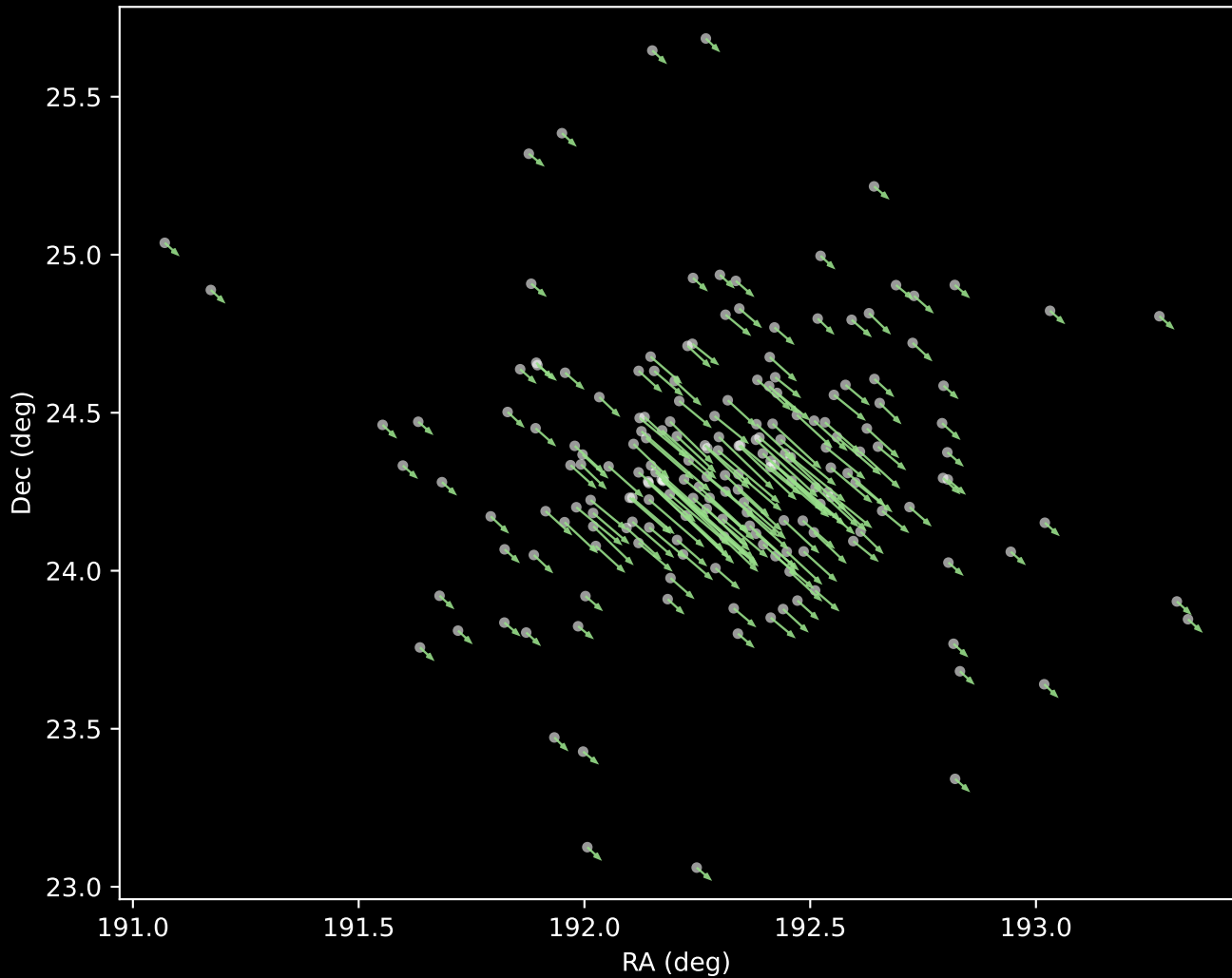
Gaia DR3 Cluster 65 Proper Motion Vectors (n=191)
