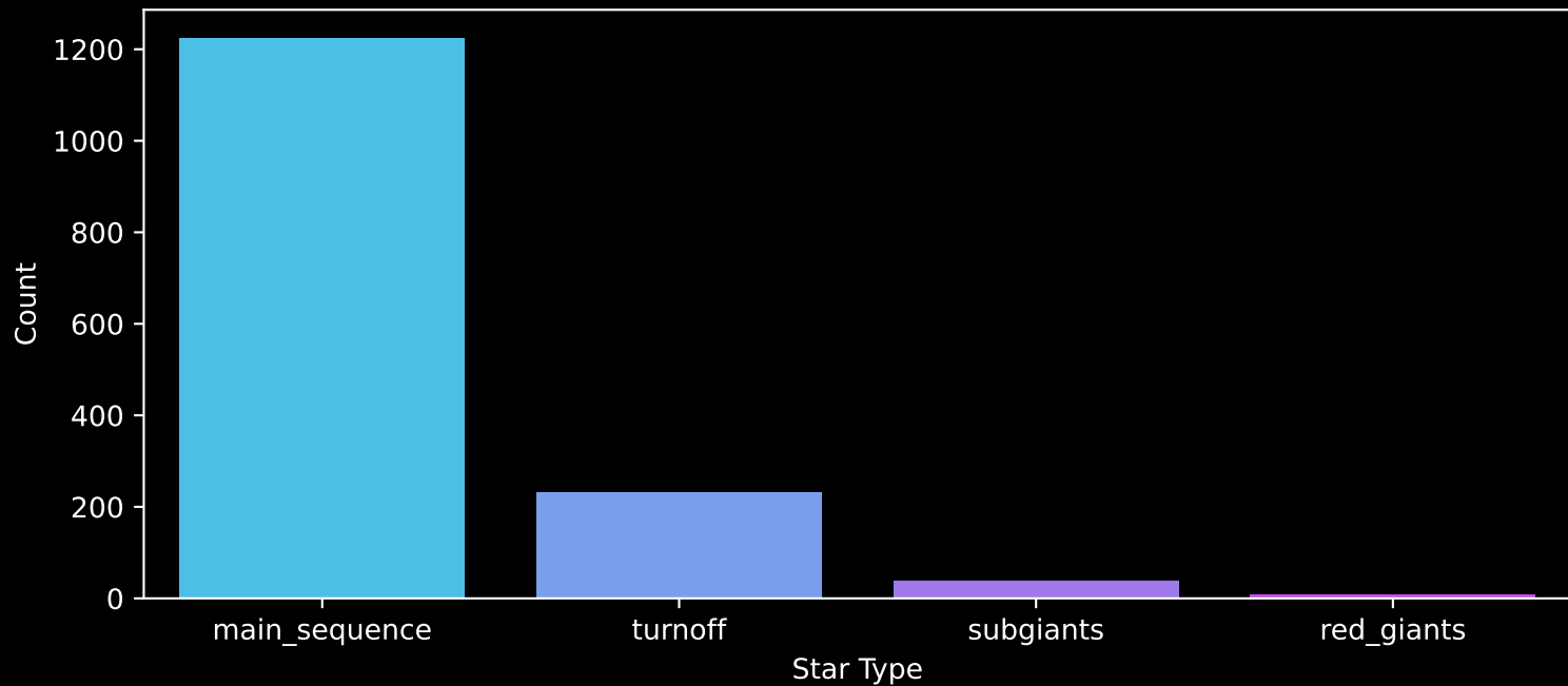
Gaia Cluster: [NGC_2168] Count plot of Star Type
