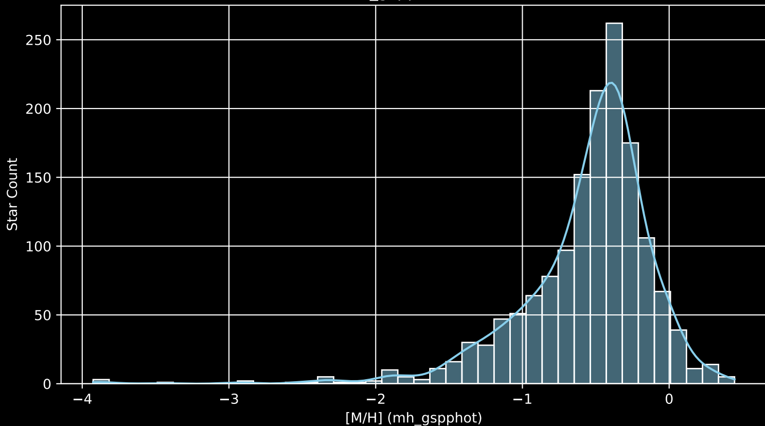
Gaia Cluster: [NGC_2168 [M/H] (mh_gspphot) (n= 1501)
