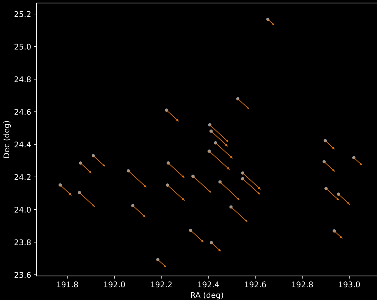
Gaia DR3 Cluster 62 Proper Motion Vectors (n=29)
