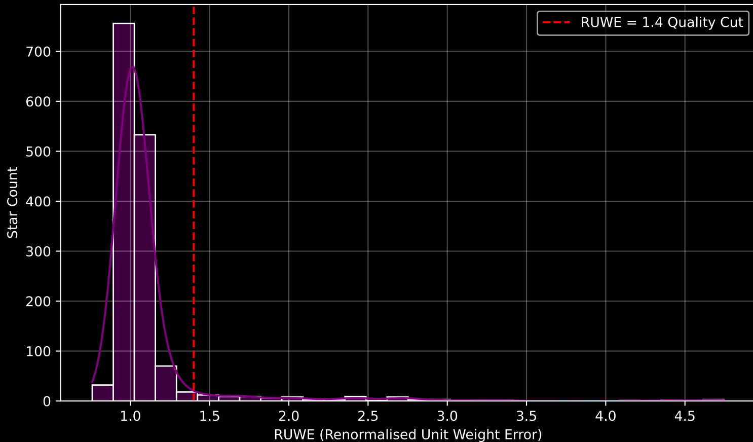
Gaia Cluster: [NGC_2168] RUWE Distribution (n= 1495)
