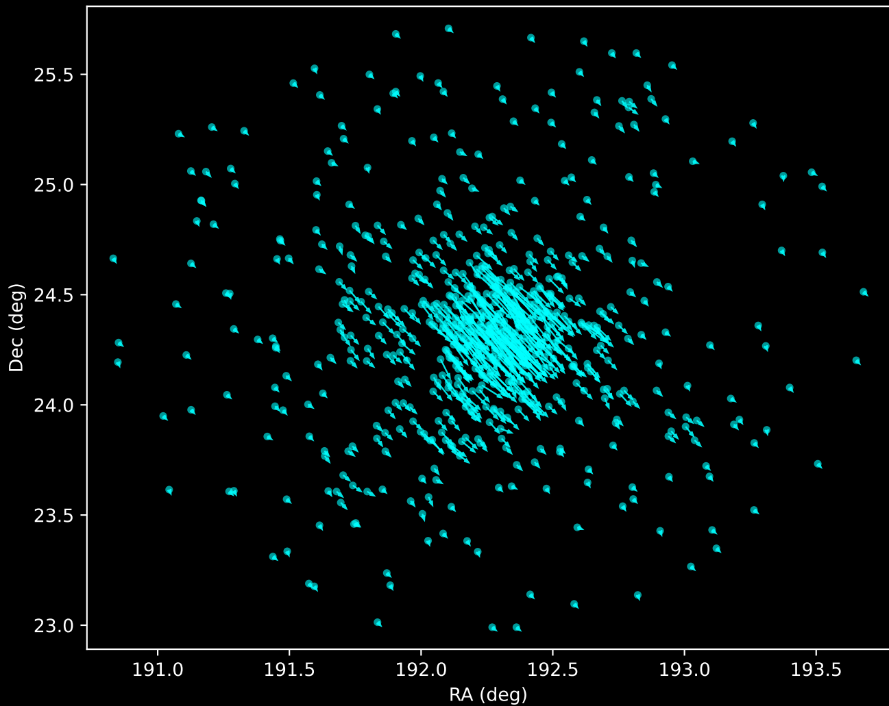
Gaia DR3 Noise Stream Proper Motion Vectors (n=625)
