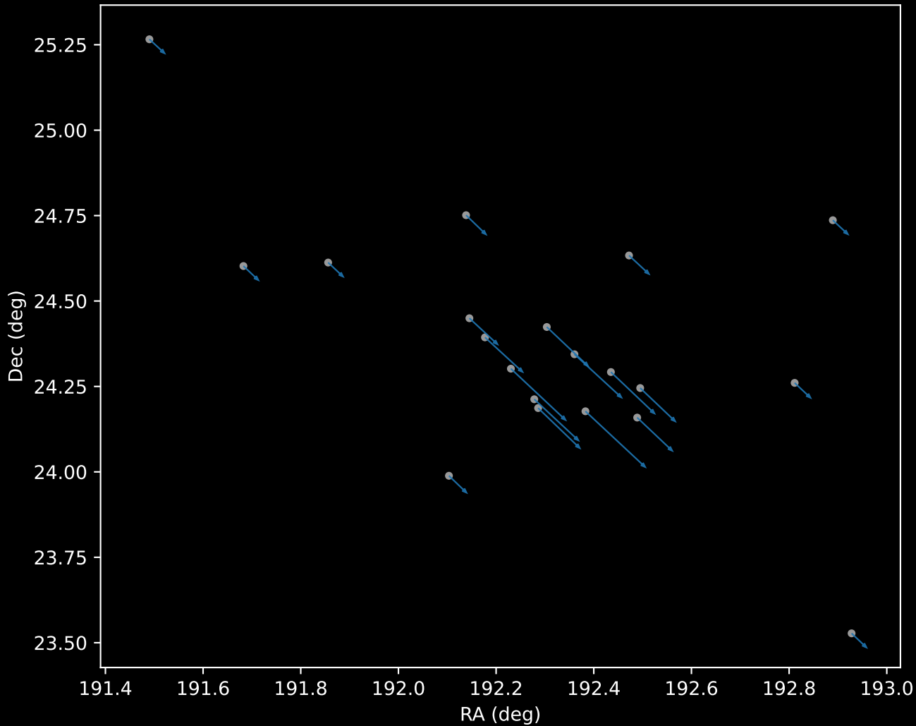
Gaia DR3 Cluster 60 Proper Motion Vectors (n=20)
