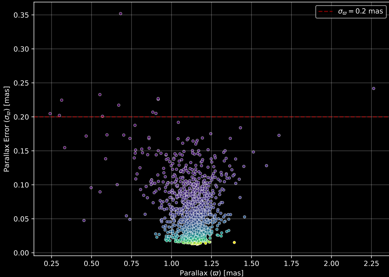
Gaia Cluster: [NGC_2168] Parallax Quality (n= 1503)
