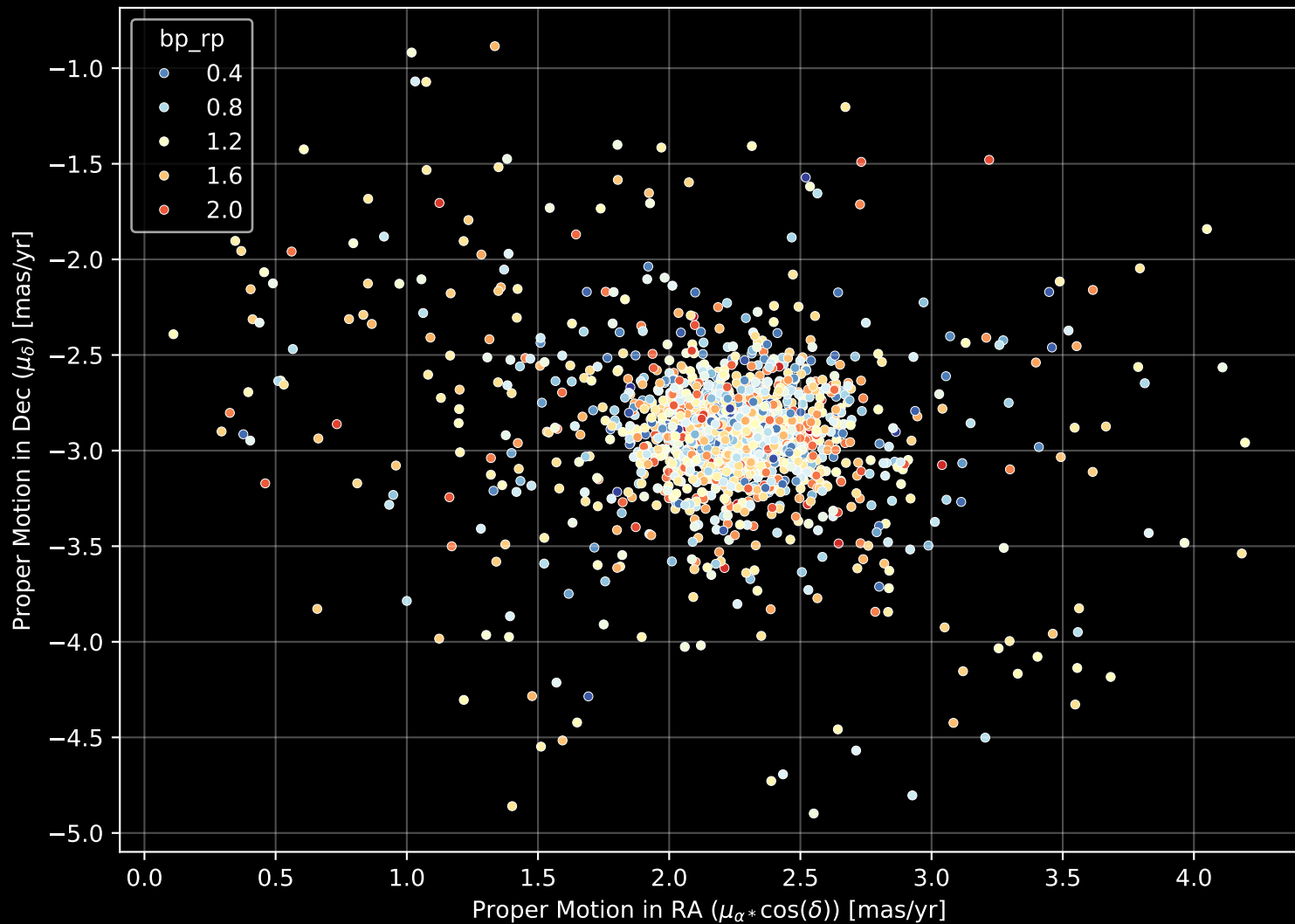
Gaia Cluster: [NGC_2168] Proper Motion Diagram (n= 1503)
