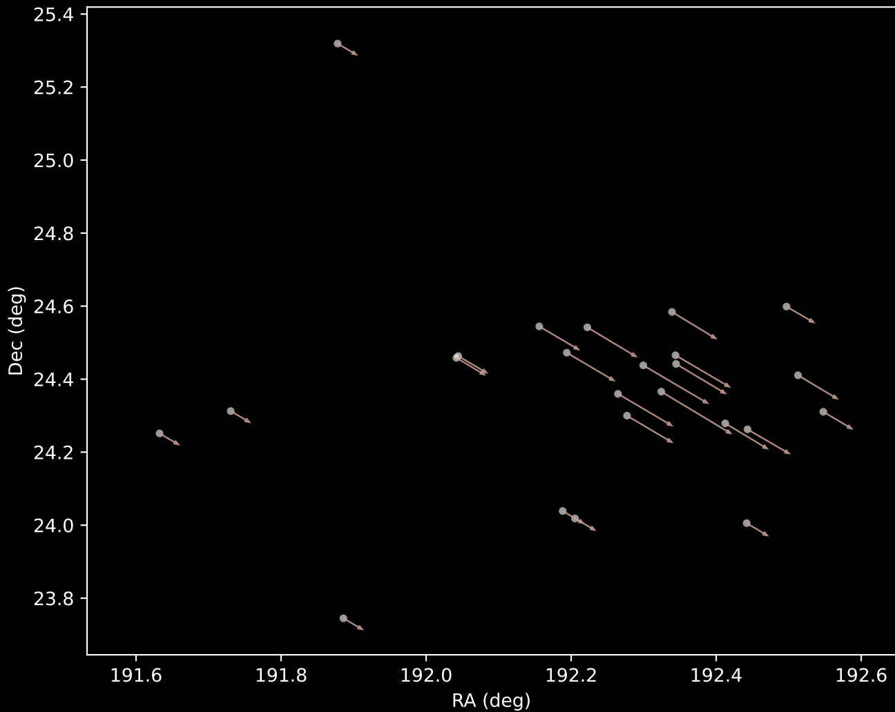
Gaia DR3 Cluster 71 Proper Motion Vectors (n=24)
