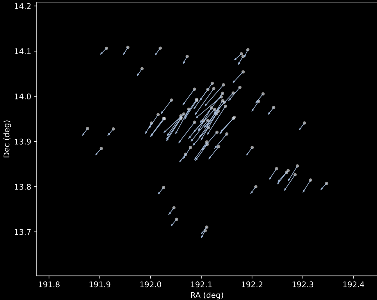
Gaia DR3 Cluster 1 Proper Motion Vectors (n=71)
