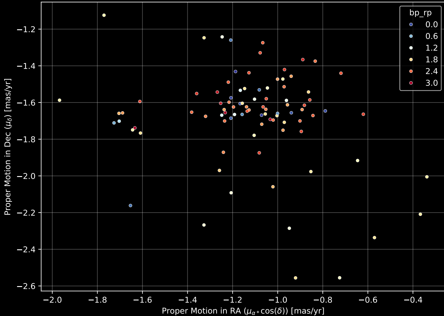
Gaia Cluster: [NGC_2169] Proper Motion Diagram (n= 91)
