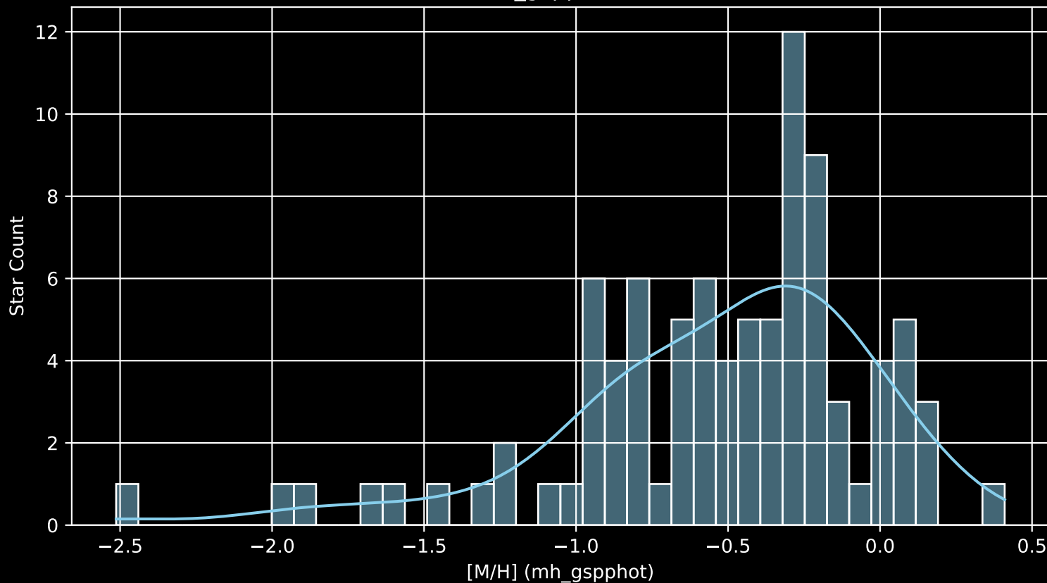
Gaia Cluster: [NGC_2169 [M/H] (mh_gspphot) (n= 91)
