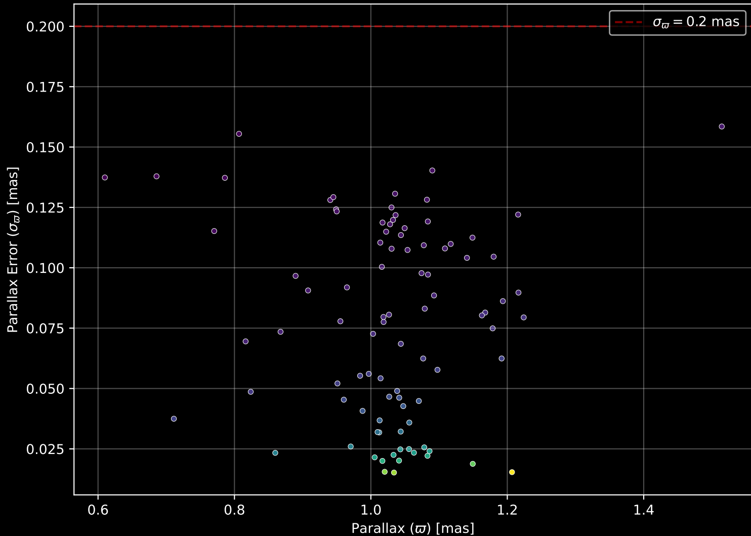
Gaia Cluster: [NGC_2169] Parallax Quality (n= 91)
