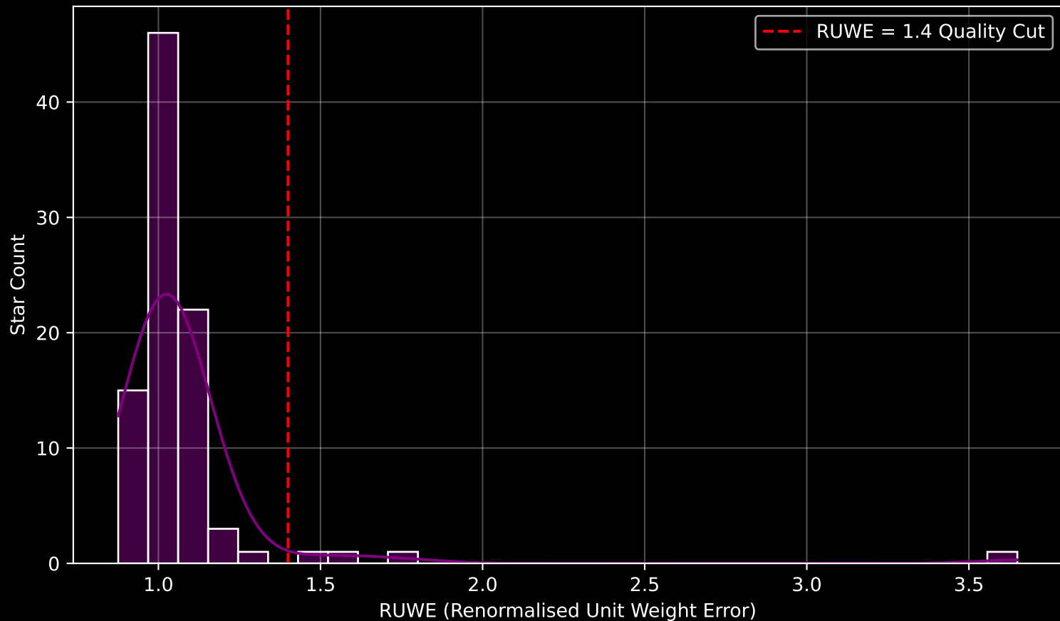
Gaia Cluster: [NGC_2169] RUWE Distribution (n= 91)
