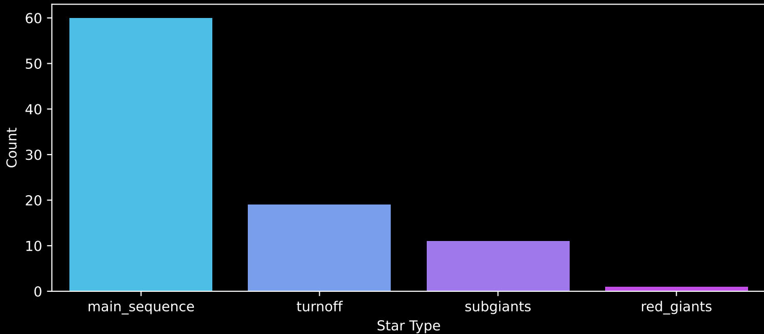
Gaia Cluster: [NGC_2169] Count plot of Star Type
