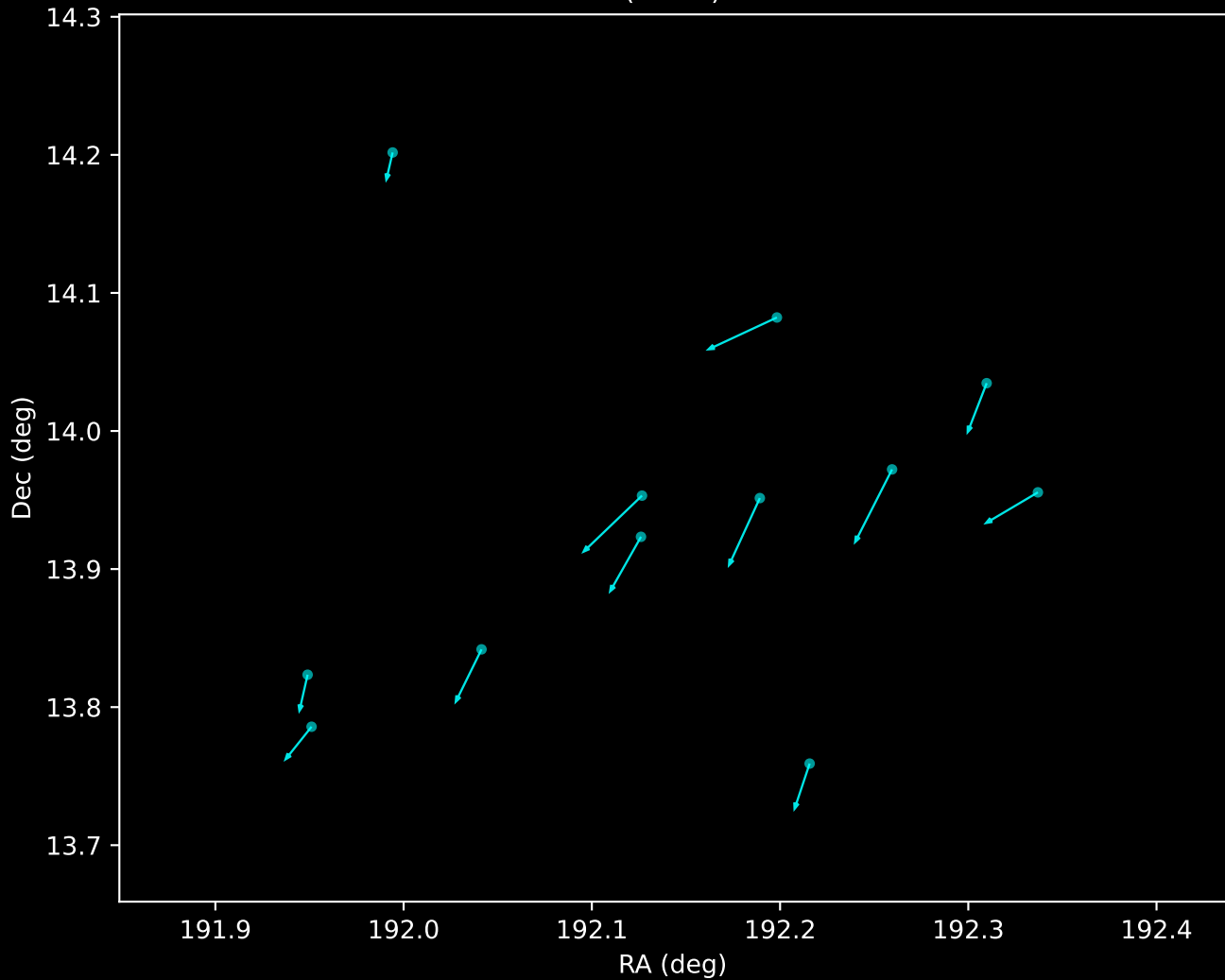
Gaia DR3 Noise Stream Proper Motion Vectors (n=12)
