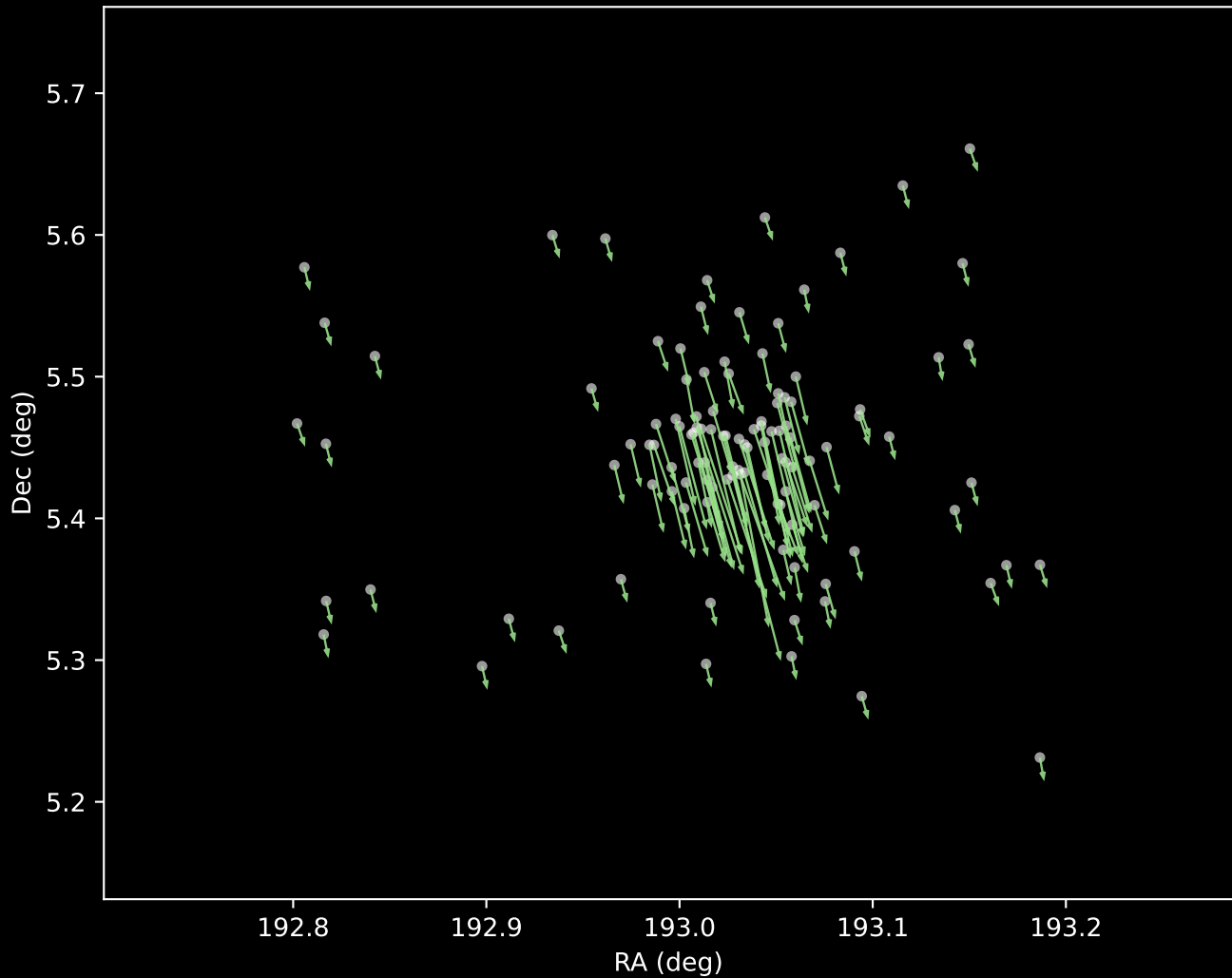
Gaia DR3 Cluster 5 Proper Motion Vectors (n=112)
