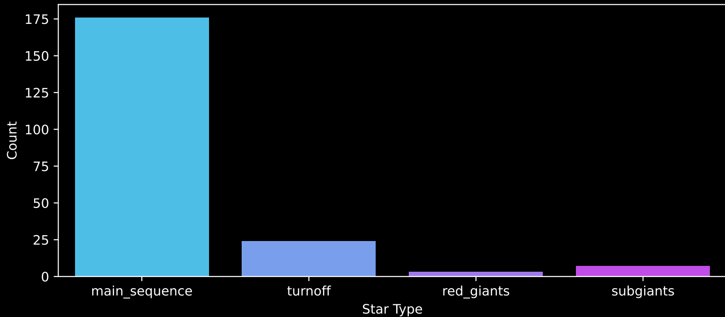
Gaia Cluster: [NGC_2186] Count plot of Star Type
