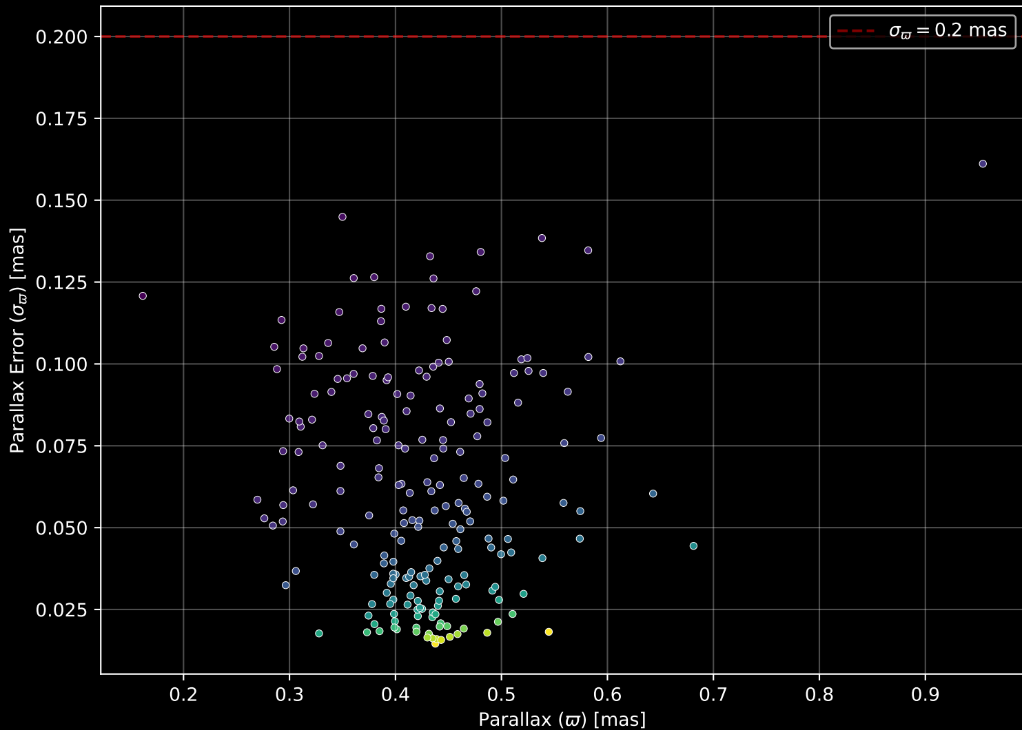
Gaia Cluster: [NGC_2186] Parallax Quality (n= 210)
