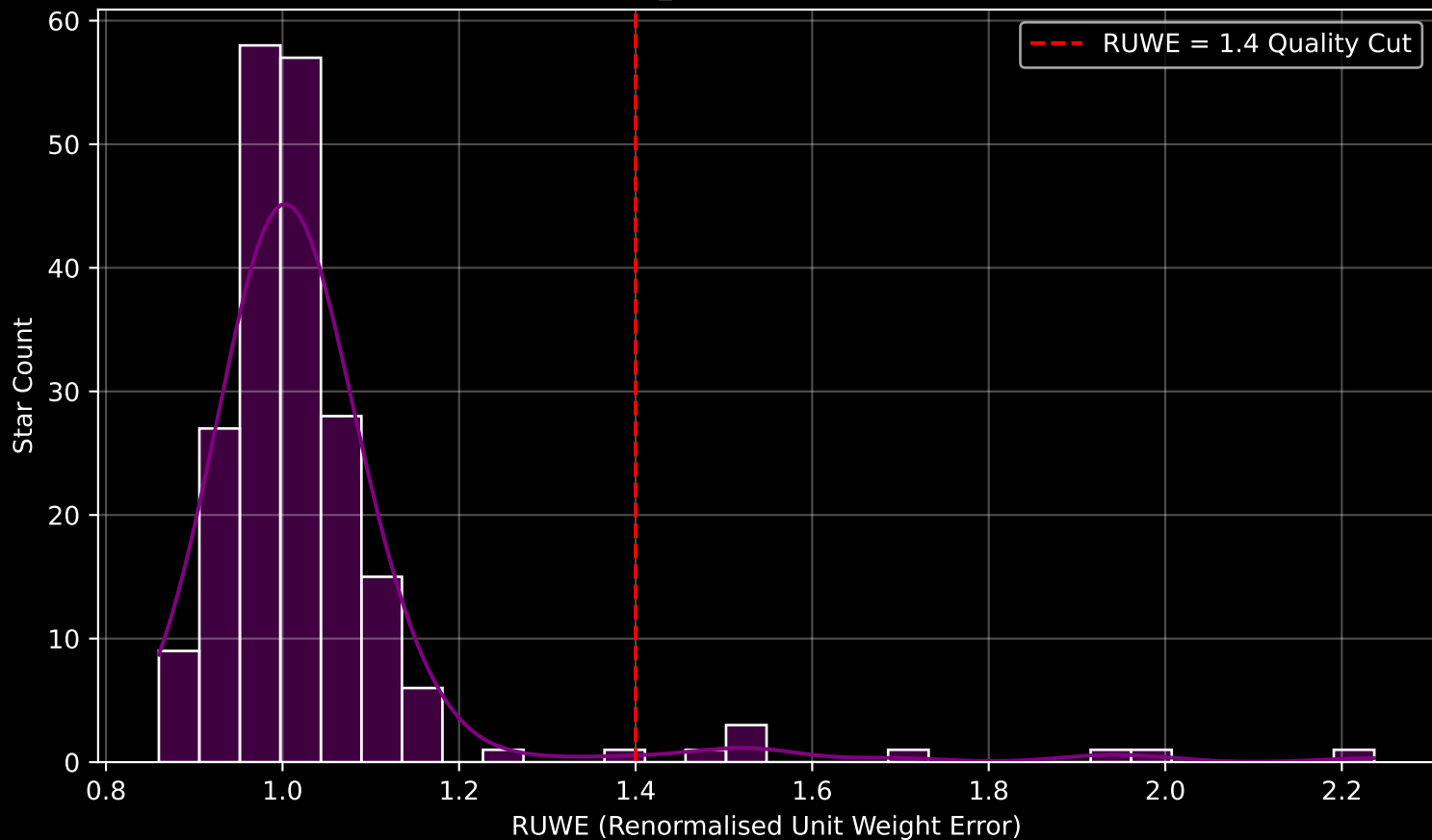
Gaia Cluster: [NGC_2186] RUWE Distribution (n= 210)
