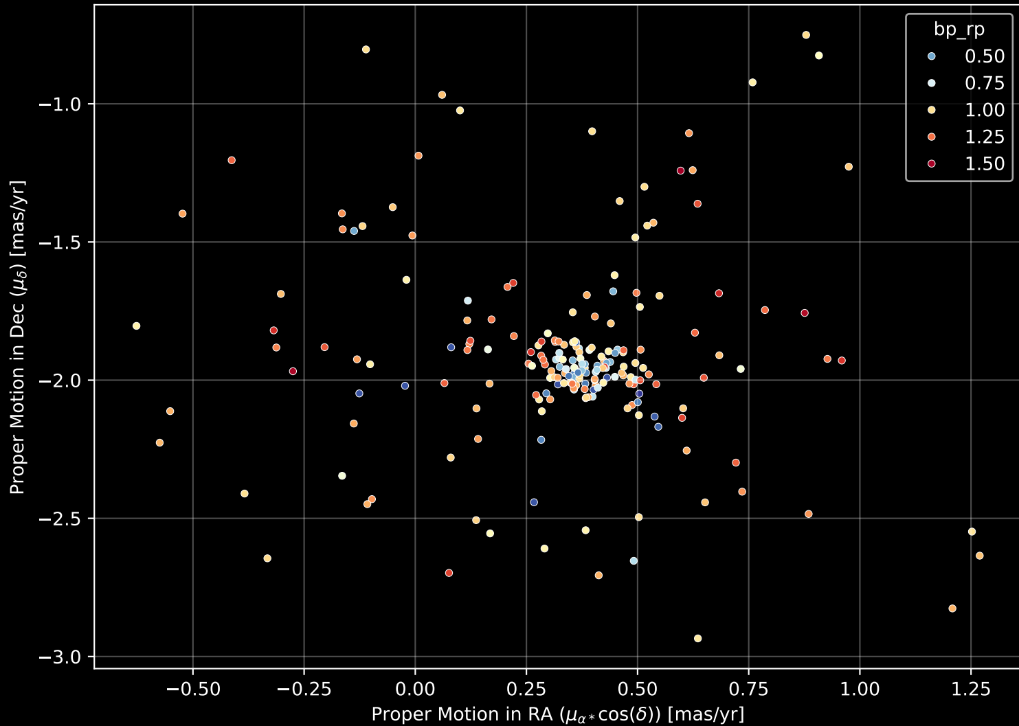
Gaia Cluster: [NGC_2186] Proper Motion Diagram (n= 210)
