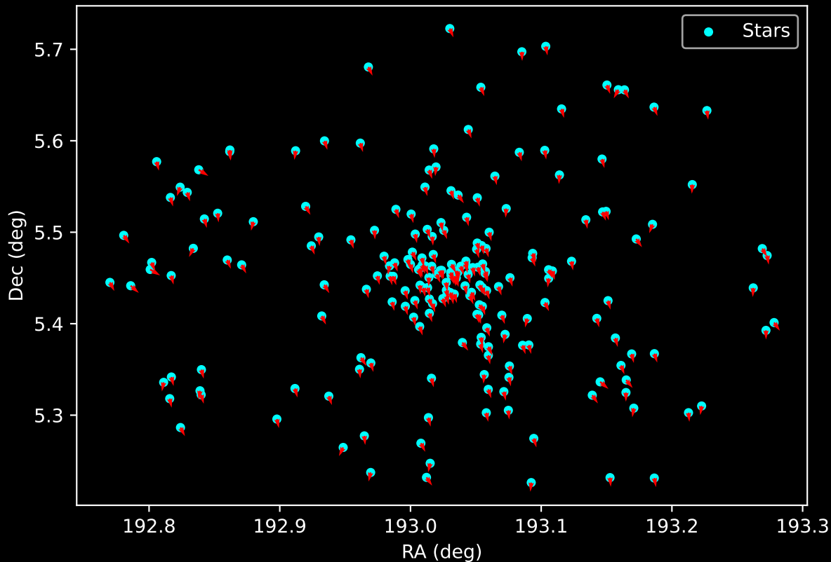
Gaia Cluster: [NGC_2186] Proper Motion Vectors for Gaia Star Field (n= 210)
