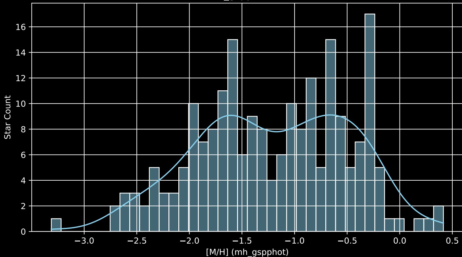
Gaia Cluster: [NGC_2186 [M/H] (mh_gspphot) (n= 210)
