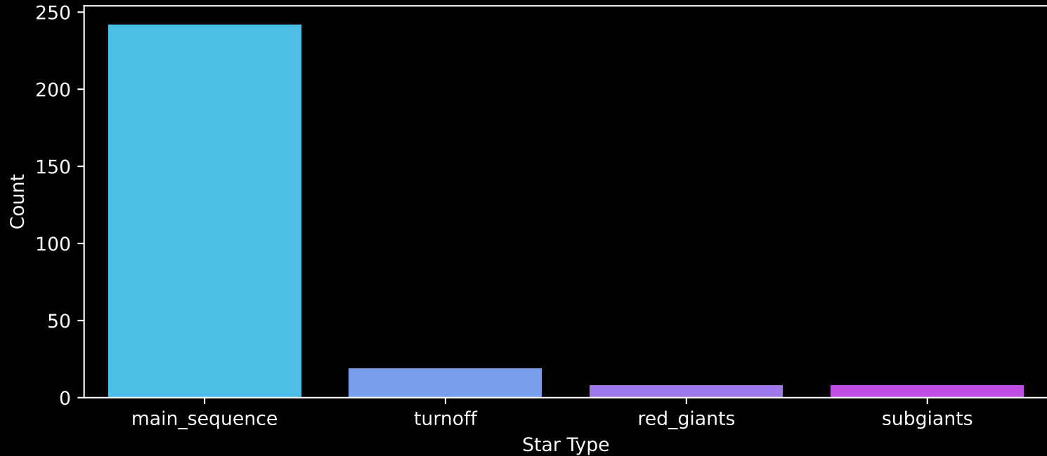
Gaia Cluster: [NGC_2192] Count plot of Star Type
