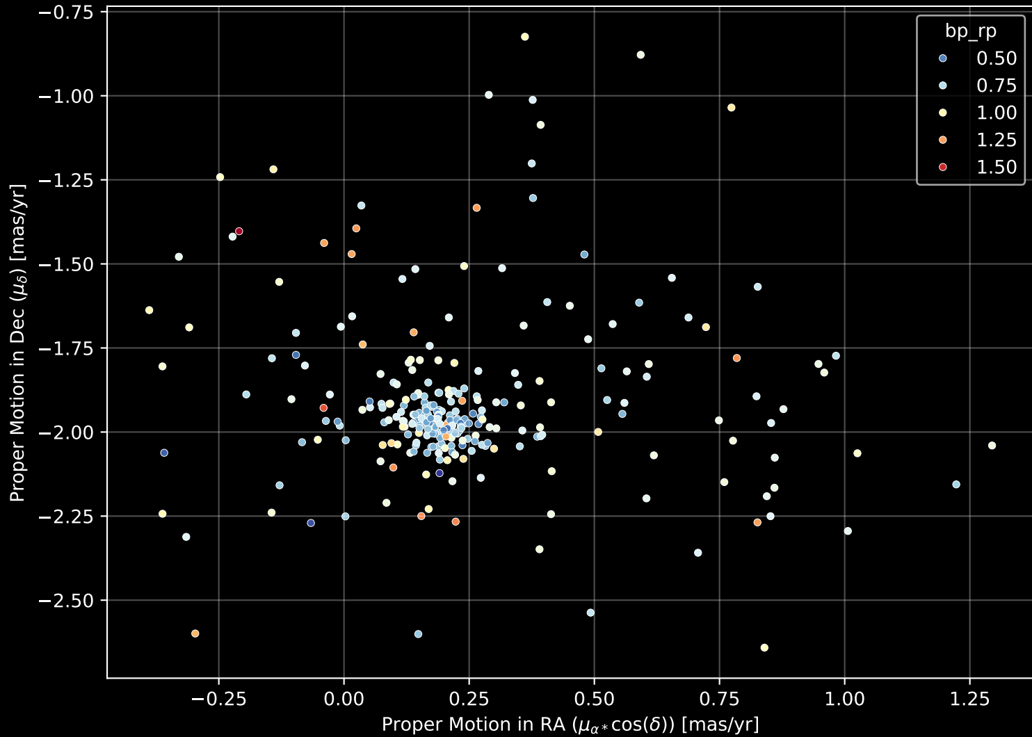
Gaia Cluster: [NGC_2192] Proper Motion Diagram (n= 277)
