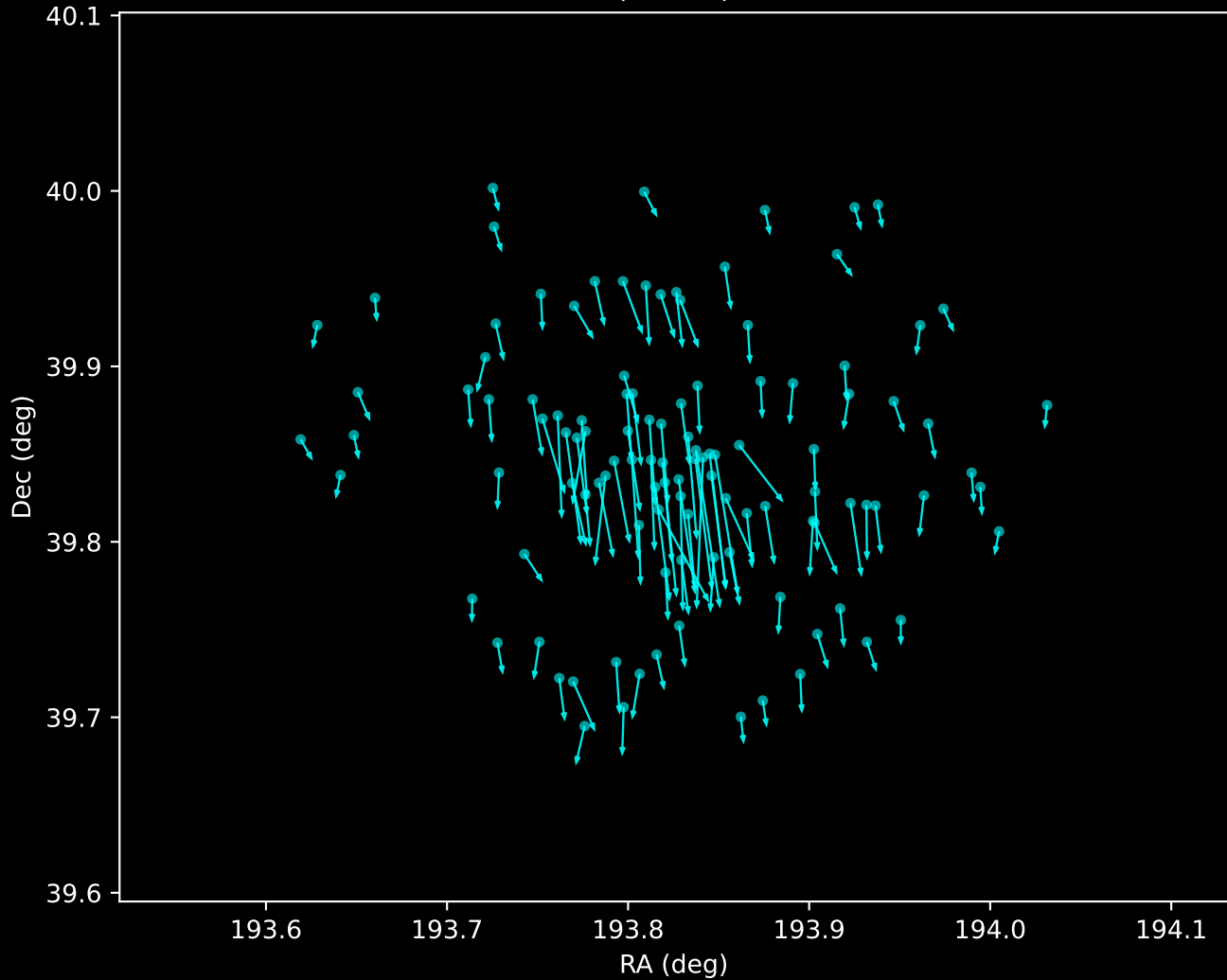
Gaia DR3 Noise Stream Proper Motion Vectors (n=113)
