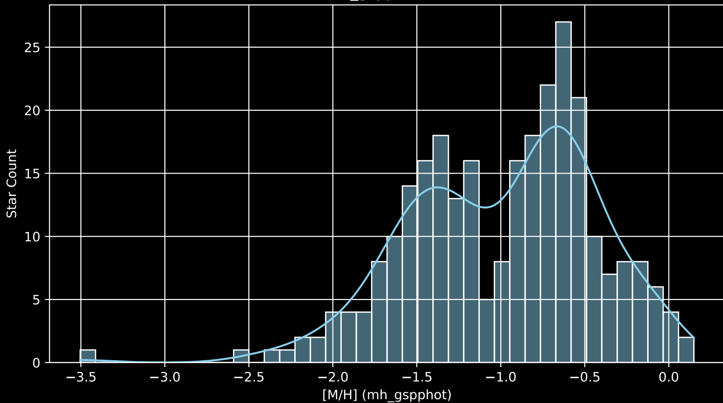
Gaia Cluster: [NGC_2192 [M/H] (mh_gspphot) (n= 277)
