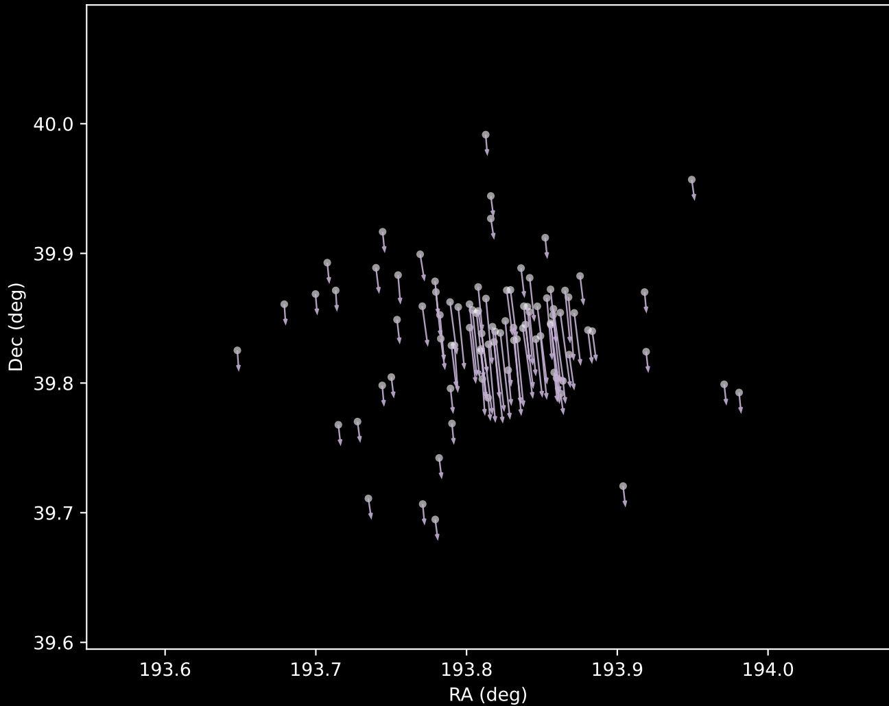
Gaia DR3 Cluster 9 Proper Motion Vectors (n=91)
