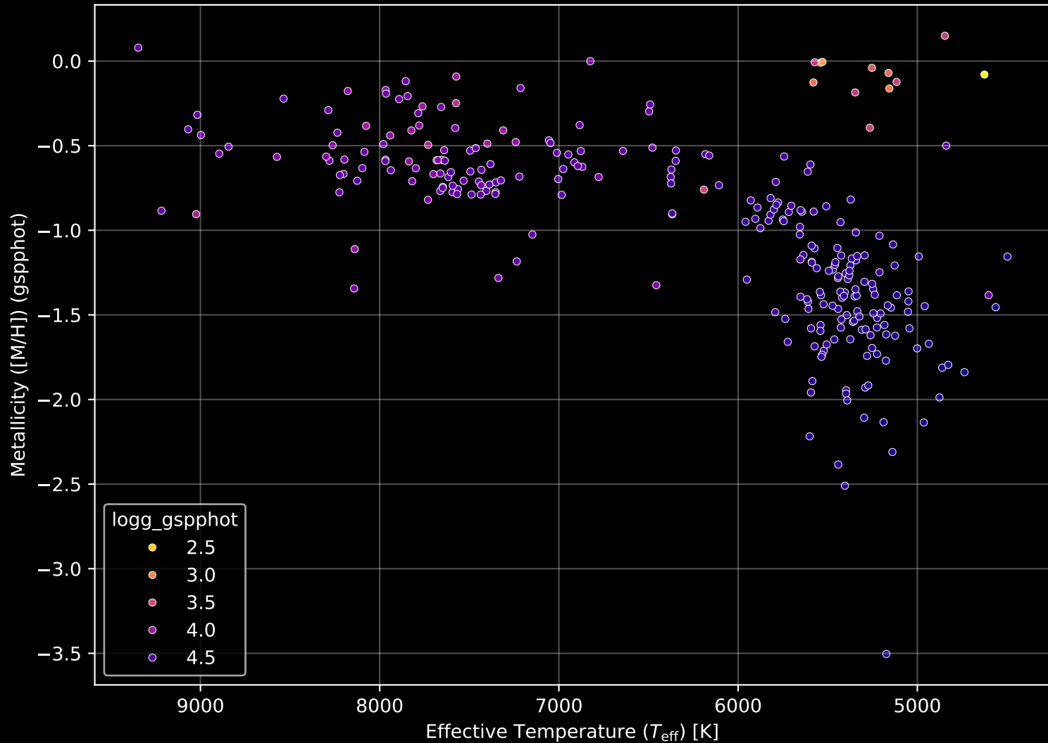
Gaia Cluster: [NGC_2192] Stellar Population Parameters (n= 277)
