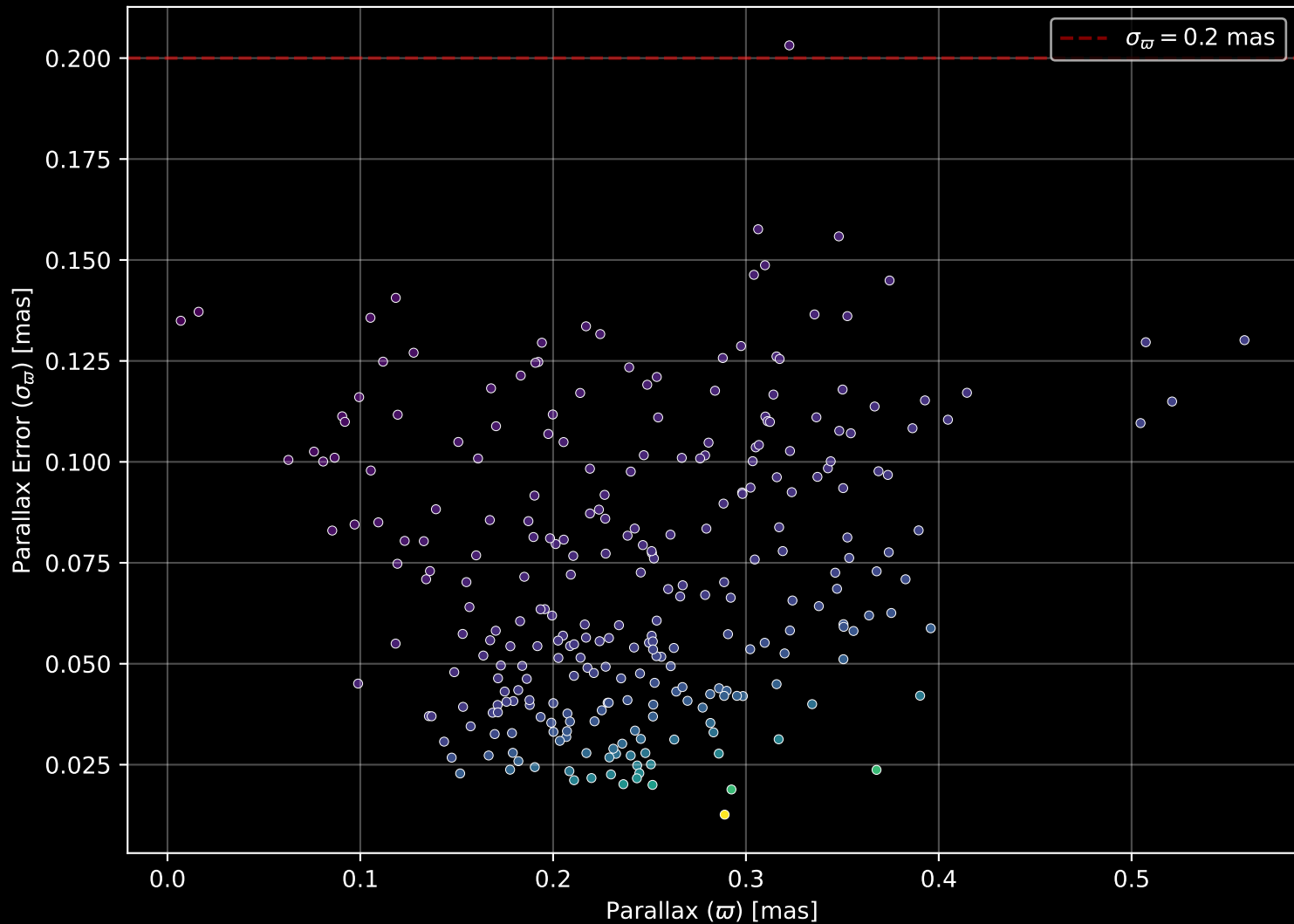
Gaia Cluster: [NGC_2192] Parallax Quality (n= 277)
