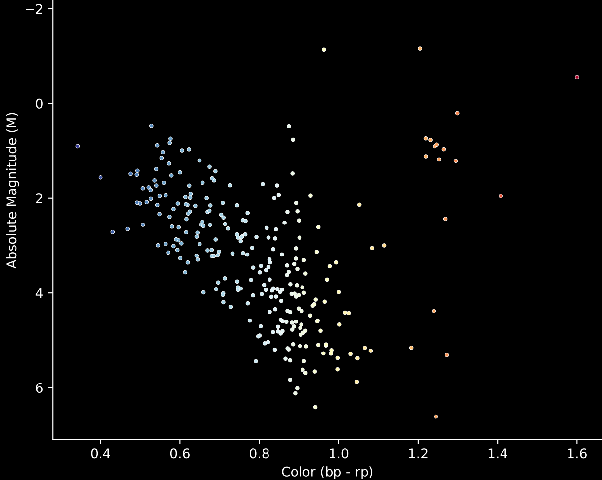
Gaia Cluster: [NGC 2192] Stars (n= 277) Hertzsprung-Russel Diagram
