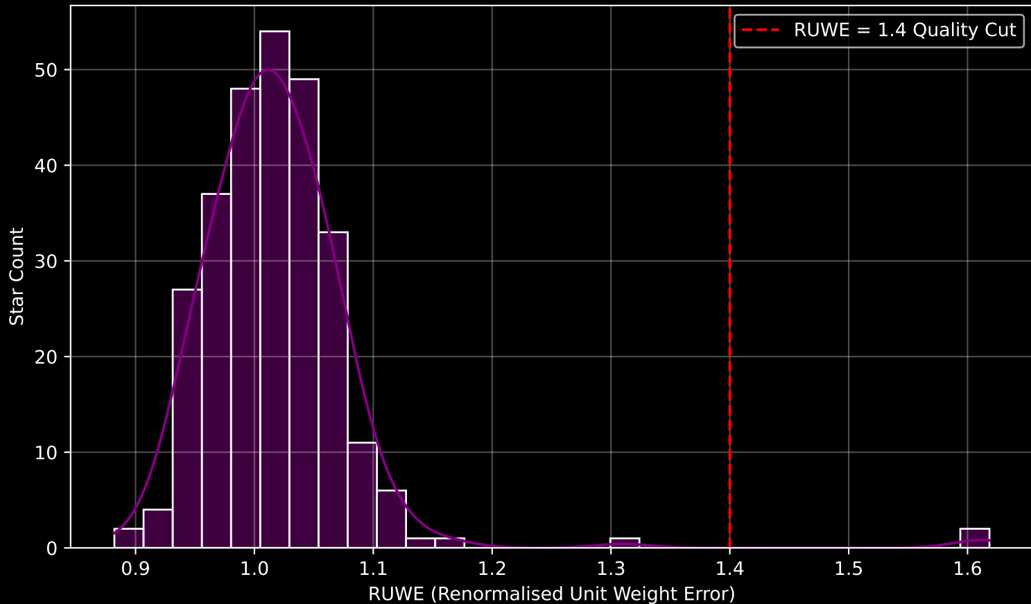
Gaia Cluster: [NGC_2192] RUWE Distribution (n= 276)
