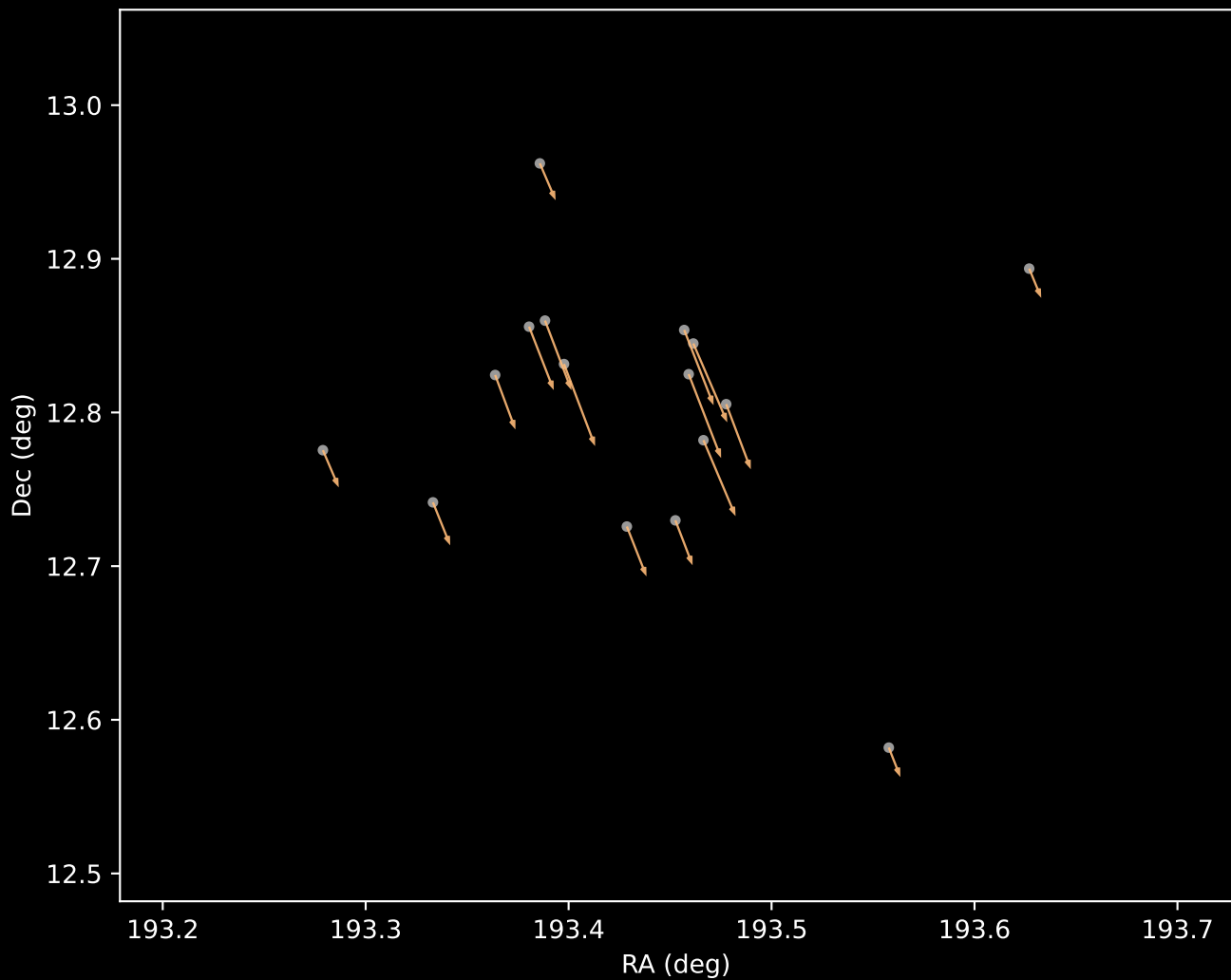
Gaia DR3 Cluster 23 Proper Motion Vectors (n=16)
