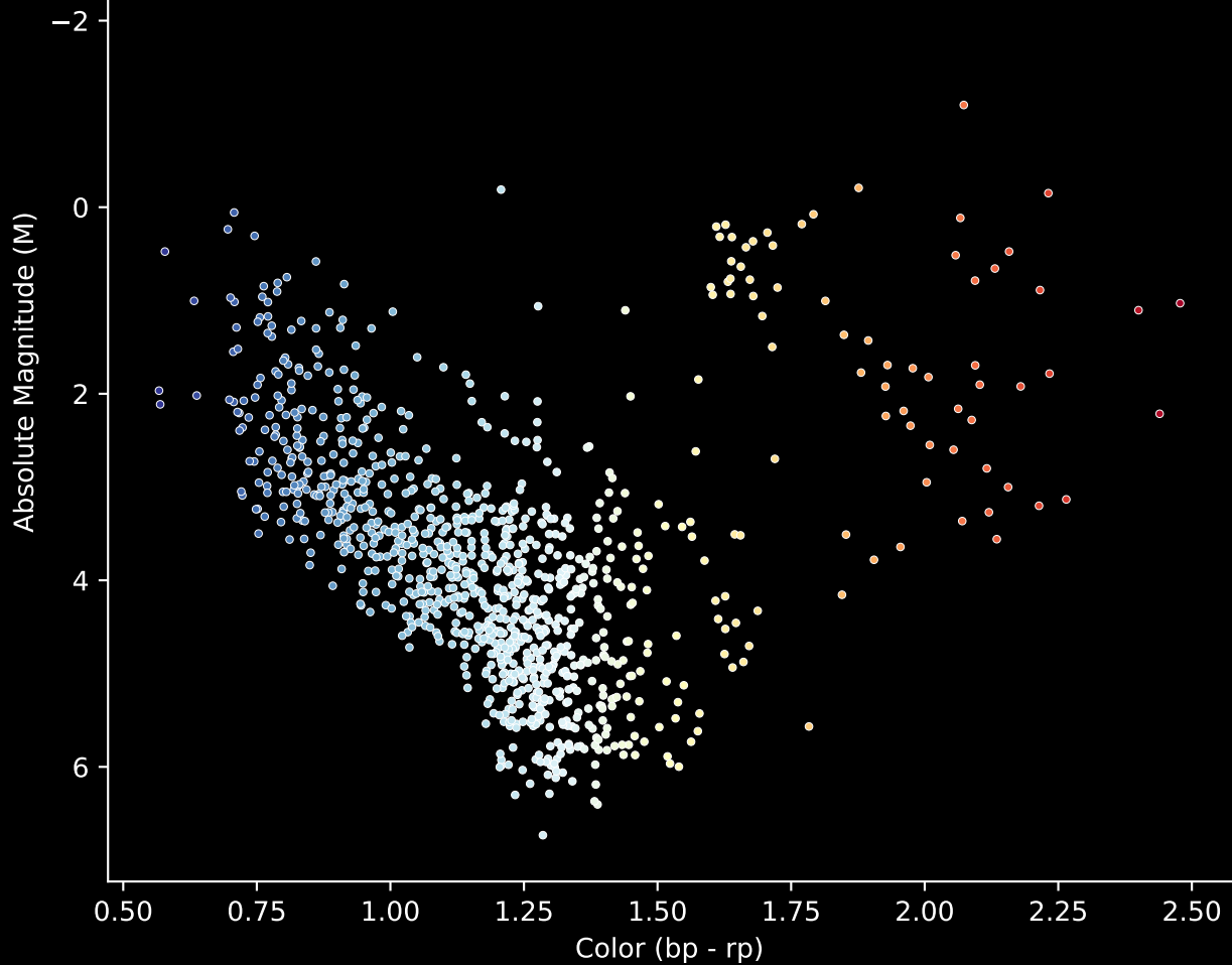
Gaia Cluster: [NGC_2194] Stars (n= 1017) Hertzsprung-Russel Diagram
