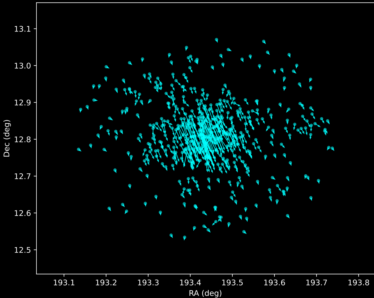
Gaia DR3 Noise Stream Proper Motion Vectors (n=466)
