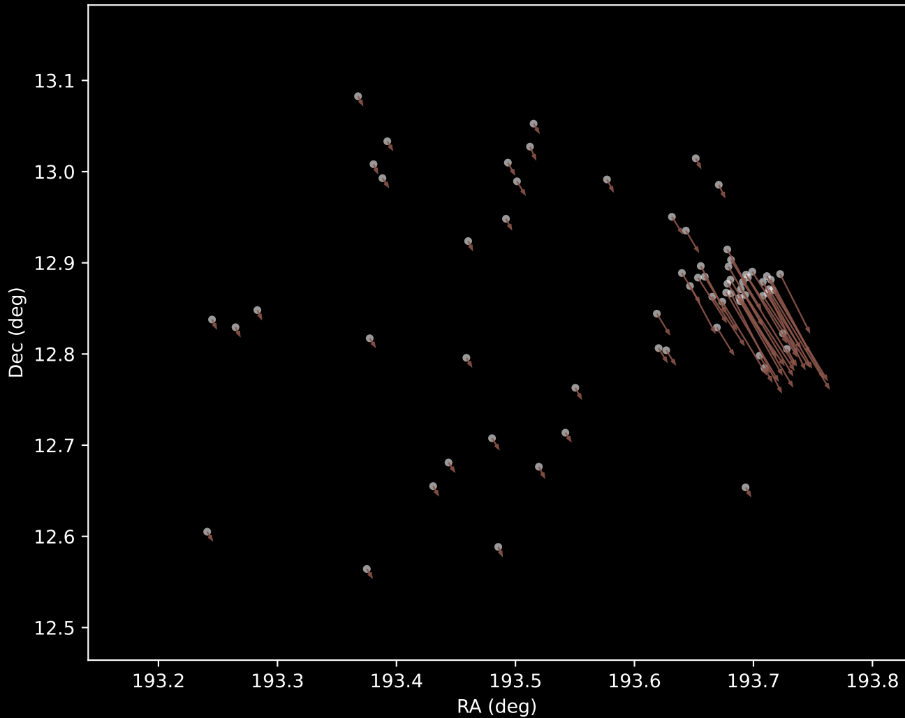
Gaia DR3 Cluster 10 Proper Motion Vectors (n=68)
