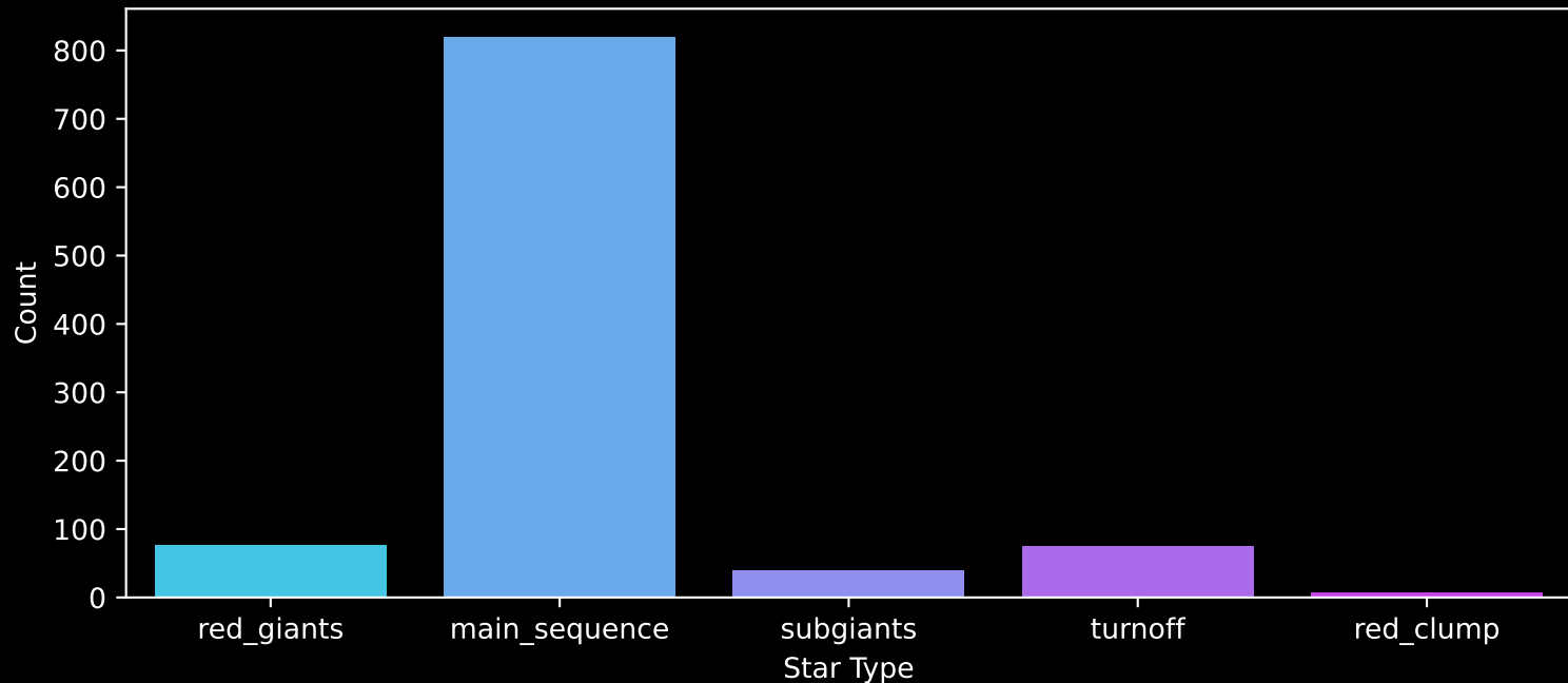
Gaia Cluster: [NGC_2194] Count plot of Star Type
