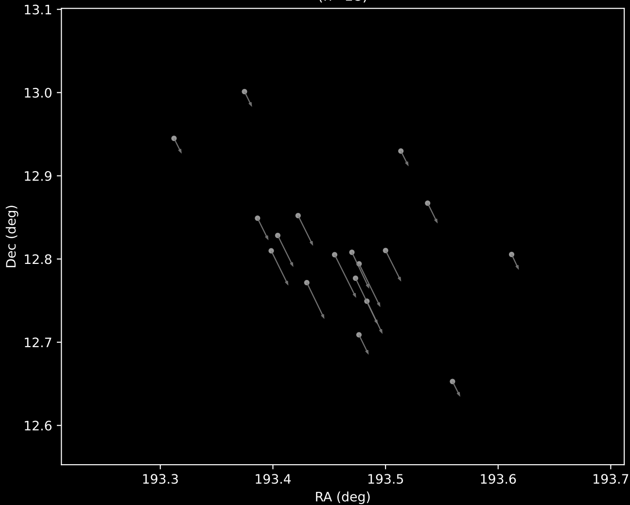
Gaia DR3 Cluster 34 Proper Motion Vectors (n=18)
