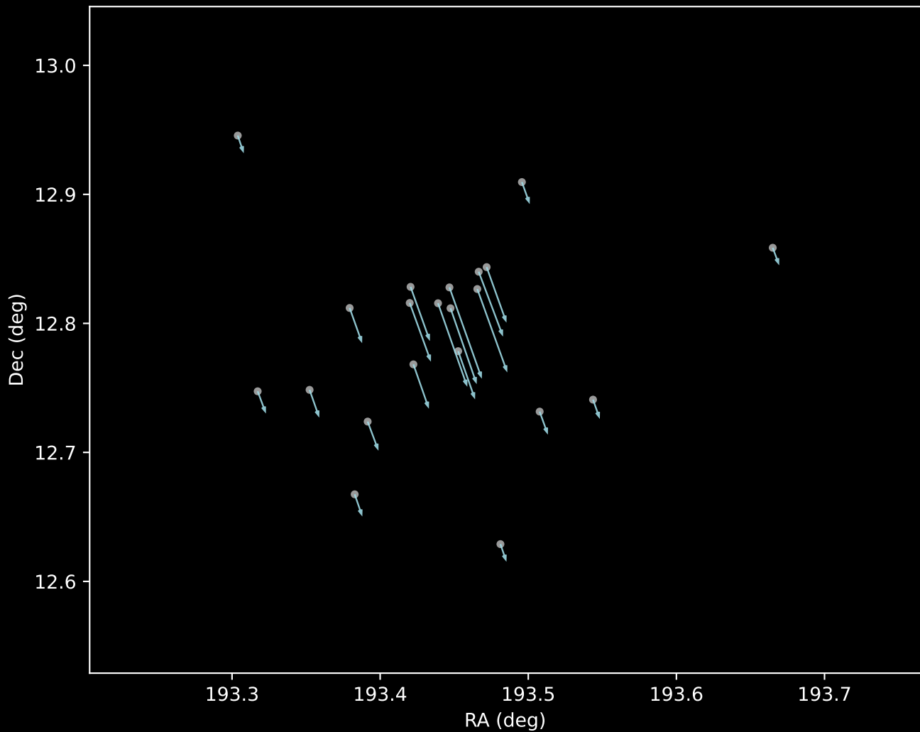
Gaia DR3 Cluster 39 Proper Motion Vectors (n=21)
