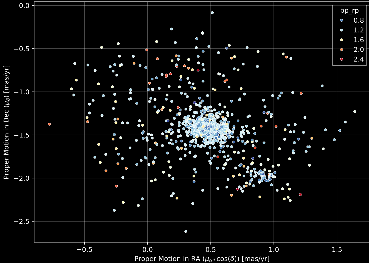
Gaia Cluster: [NGC_2194] Proper Motion Diagram (n= 1017)
