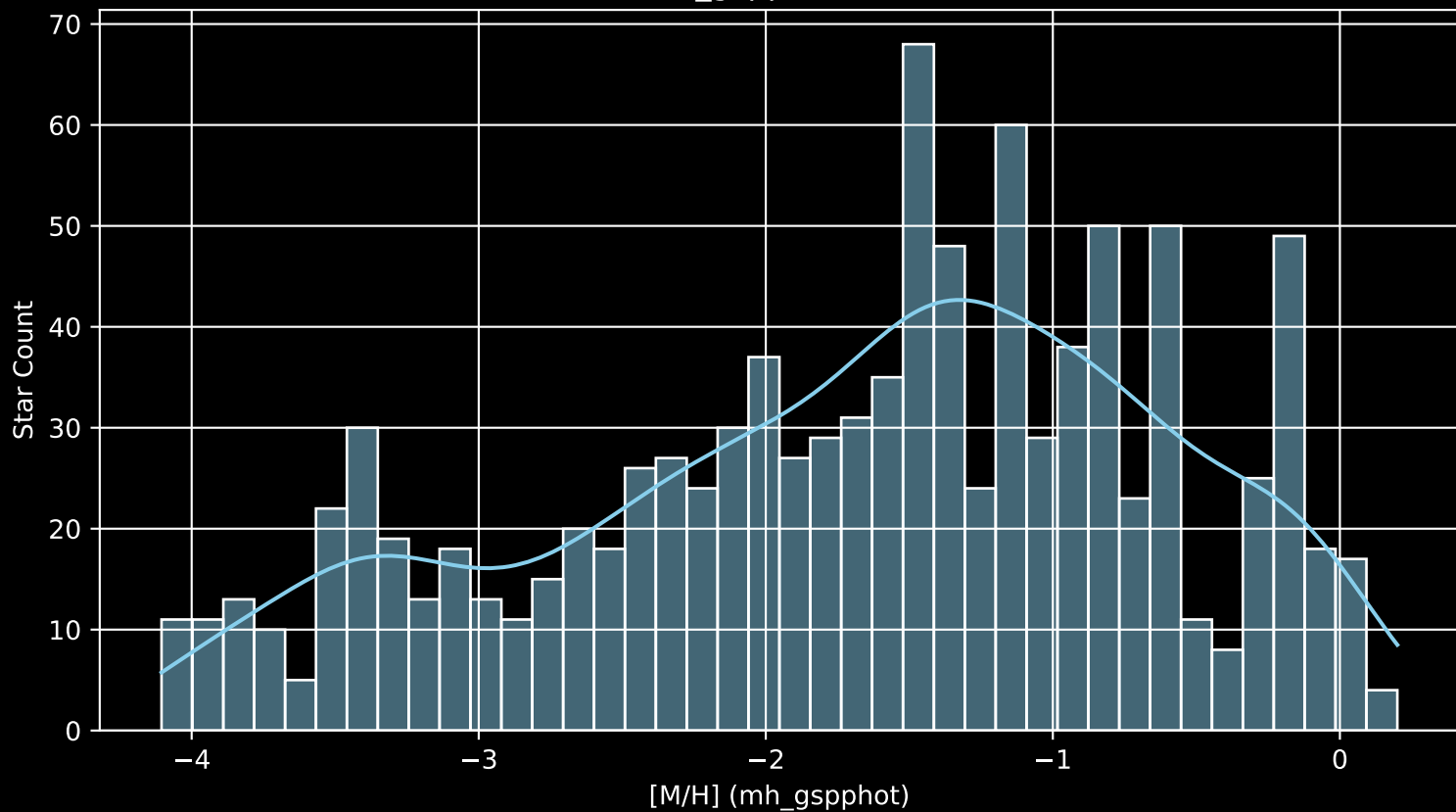
Gaia Cluster: [NGC_2194 [M/H] (mh_gspphot) ( \bar{n}= 1017 )
