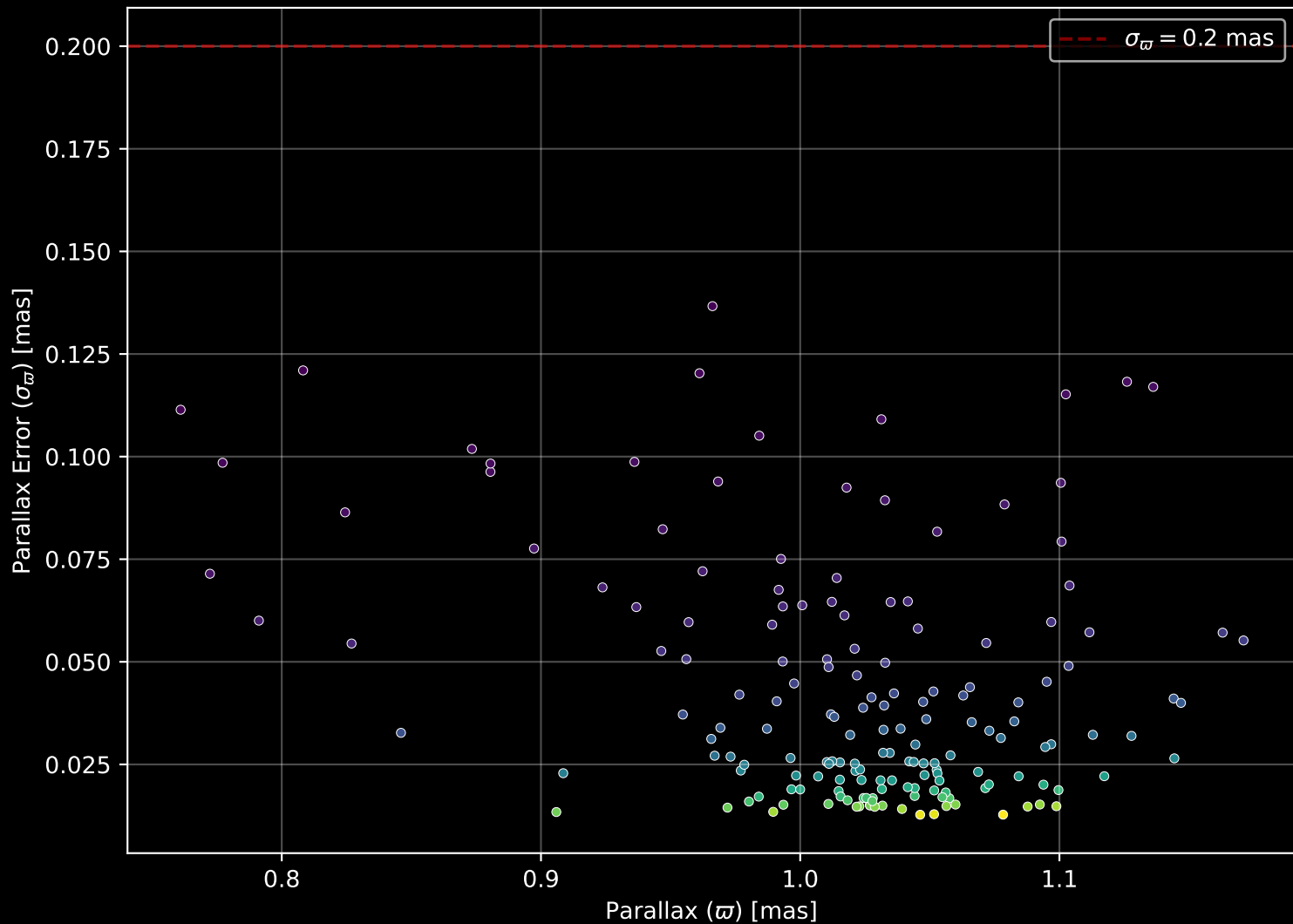
Gaia Cluster: [NGC_2215] Parallax Quality (n= 169)
