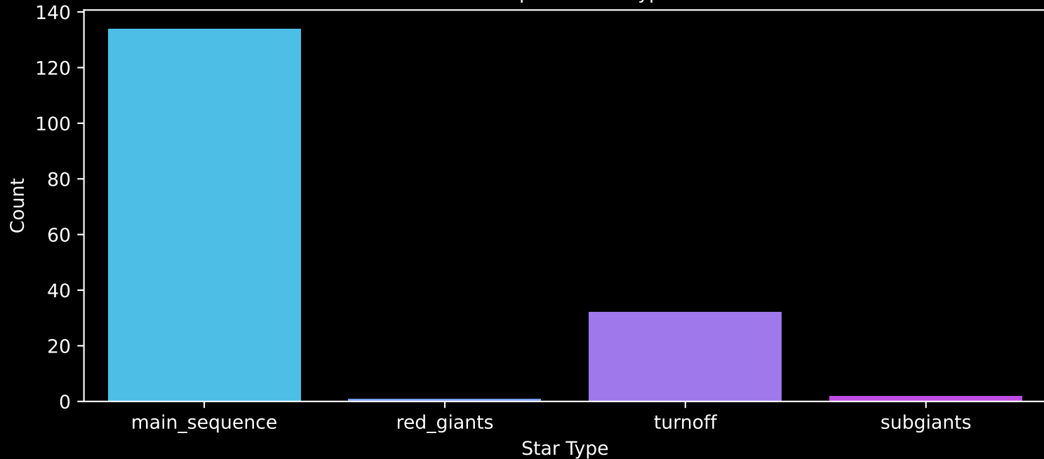
Gaia Cluster: [NGC_2215] Count plot of Star Type
