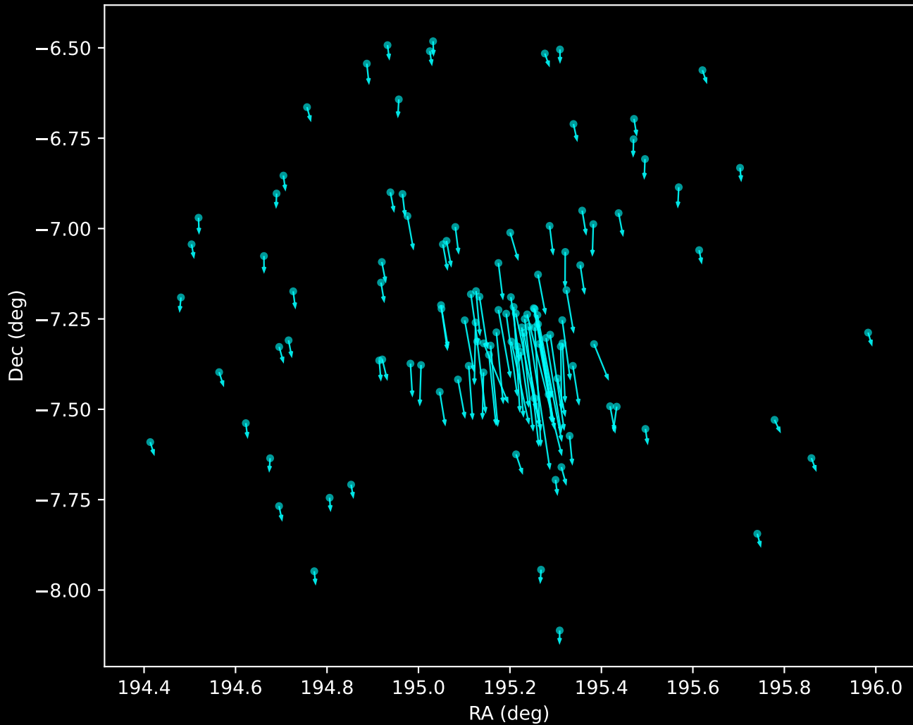
Gaia DR3 Noise Stream Proper Motion Vectors (n=113)
