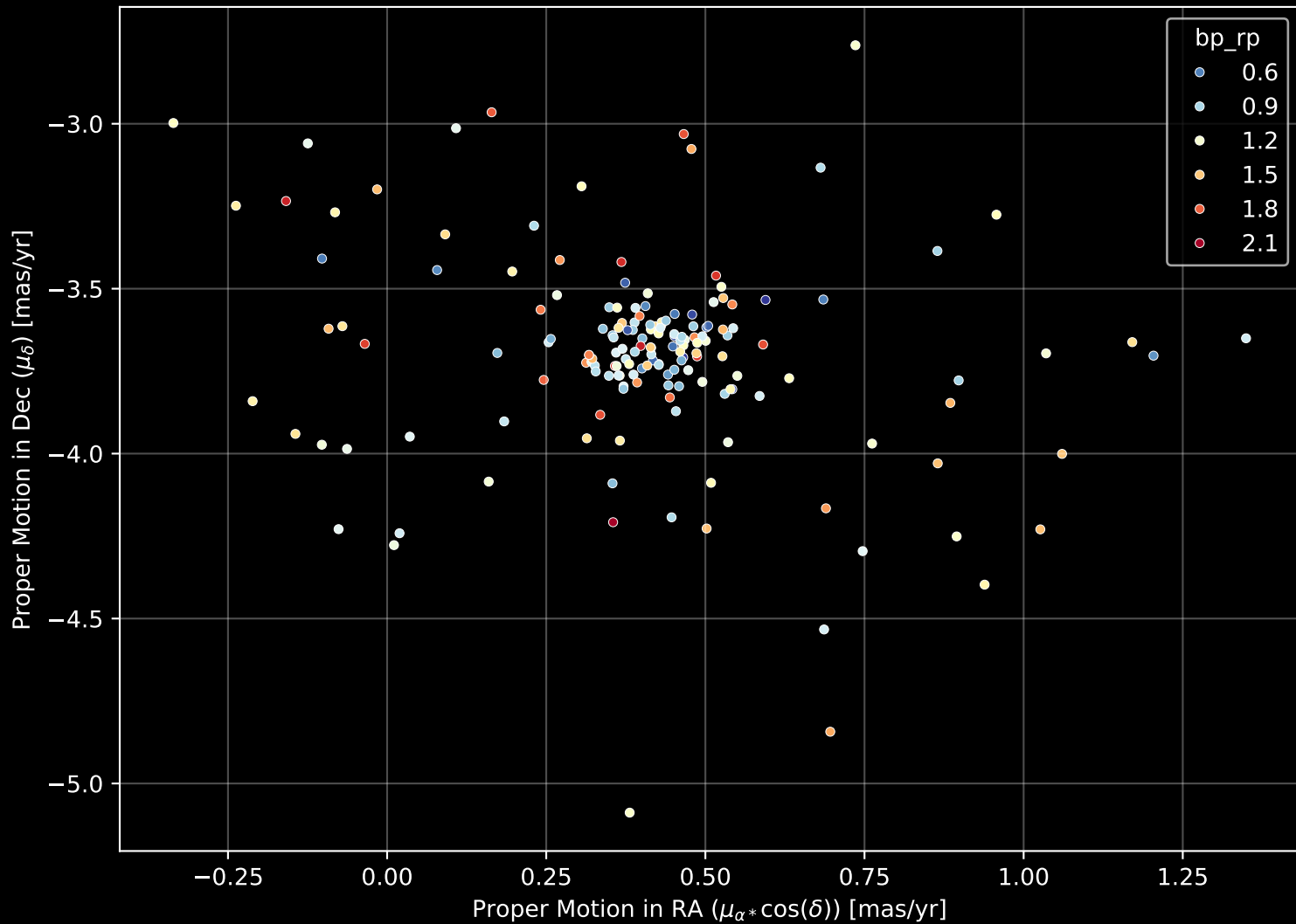
Gaia Cluster: [NGC_2215] Proper Motion Diagram (n= 169)
