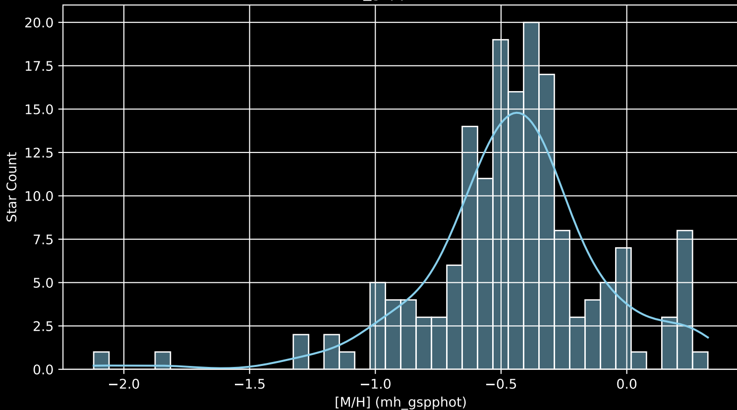
Gaia Cluster: [NGC_2215 [M/H] (mh_gspphot) (n= 169)
