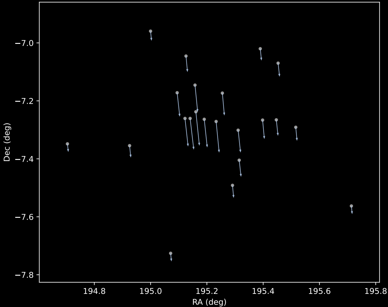
Gaia DR3 Cluster 1 Proper Motion Vectors (n=22)
