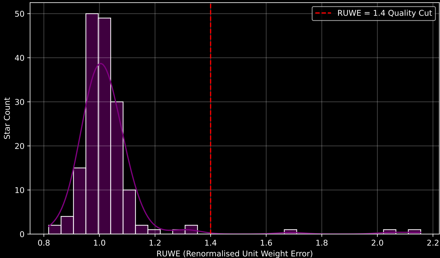
Gaia Cluster: [NGC_2215] RUWE Distribution (n= 169)
