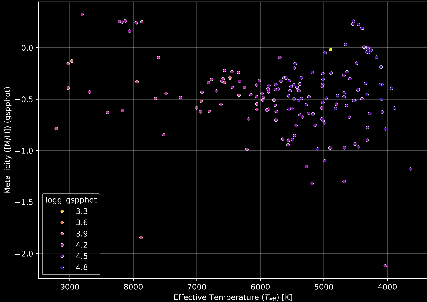
Gaia Cluster: [NGC_2215] Stellar Population Parameters (n= 169)
