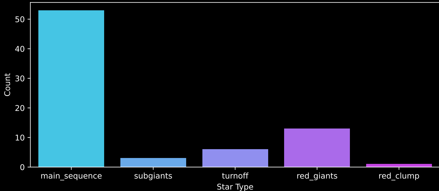
Gaia Cluster: [NGC_2225] Count plot of Star Type
