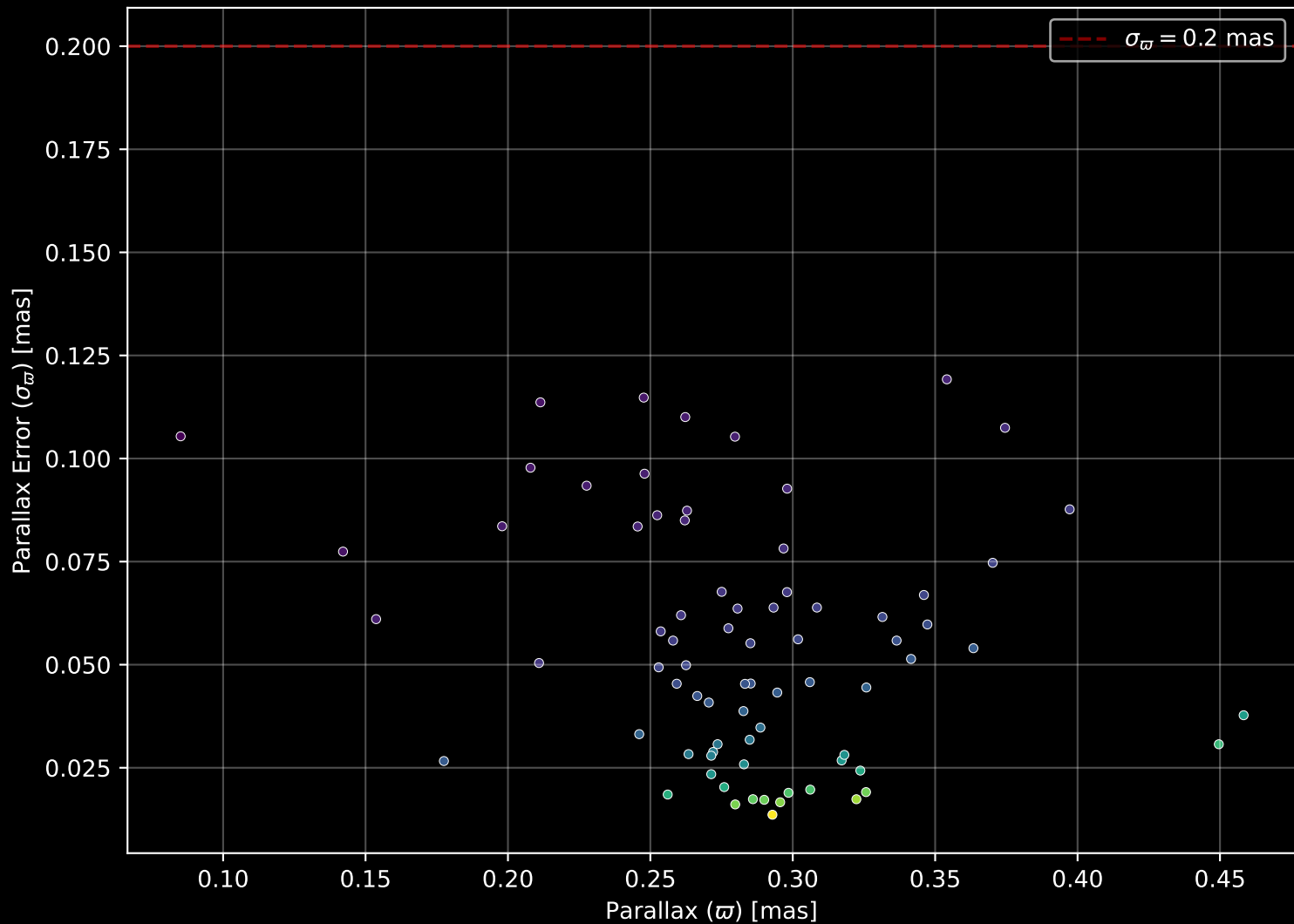
Gaia Cluster: [NGC_2225] Parallax Quality (n= 76)
