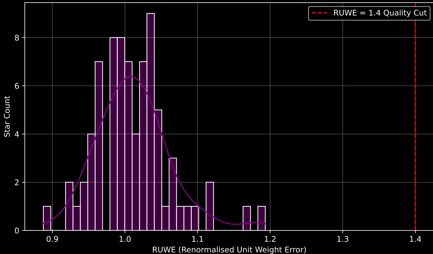
Gaia Cluster: [NGC_2225] RUWE Distribution (n= 76)
