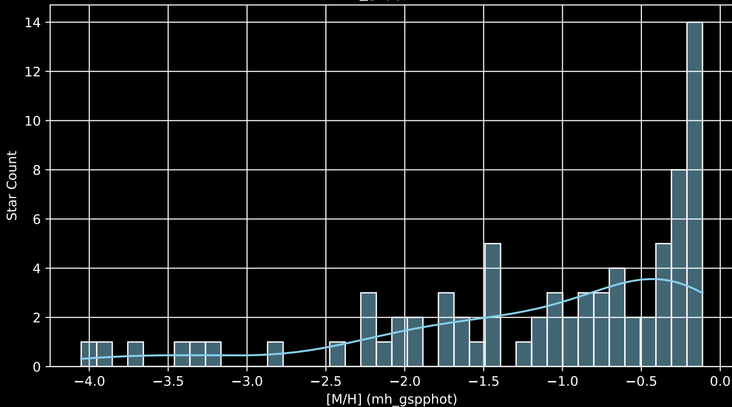
Gaia Cluster: [NGC_2225 [M/H] (mh_gspphot) (n= 76)
