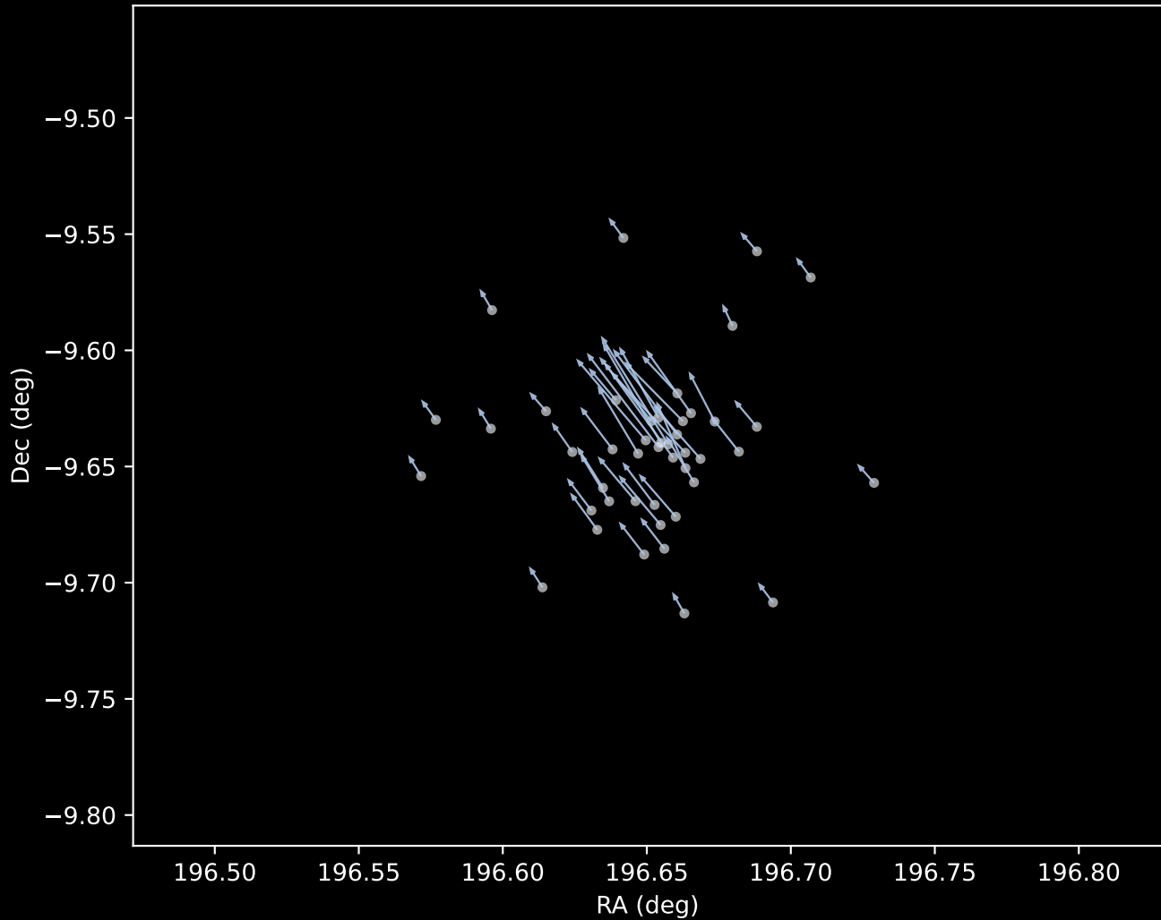
Gaia DR3 Cluster 1 Proper Motion Vectors (n=45)
