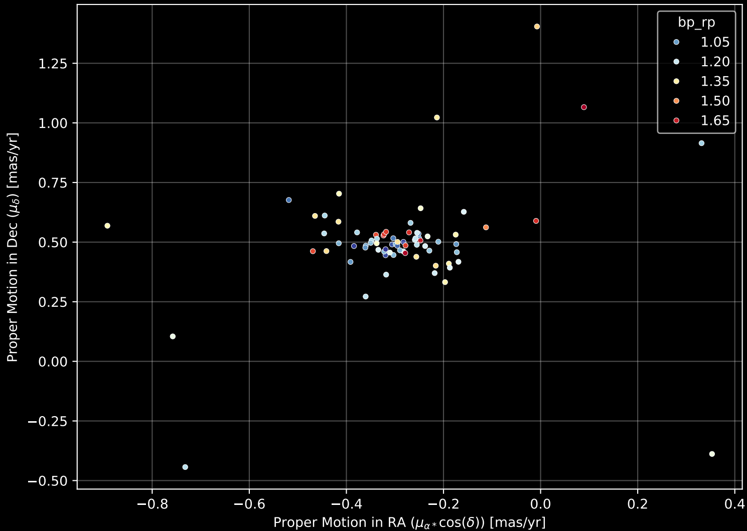
Gaia Cluster: [NGC_2225] Proper Motion Diagram (n= 76)
