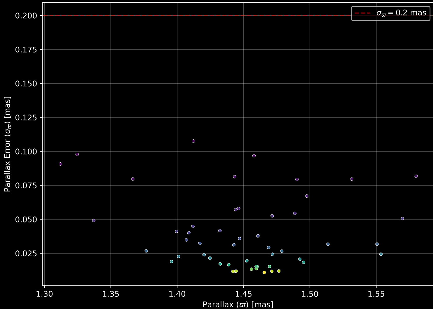
Gaia Cluster: [NGC_225] Parallax Quality (n= 52)
