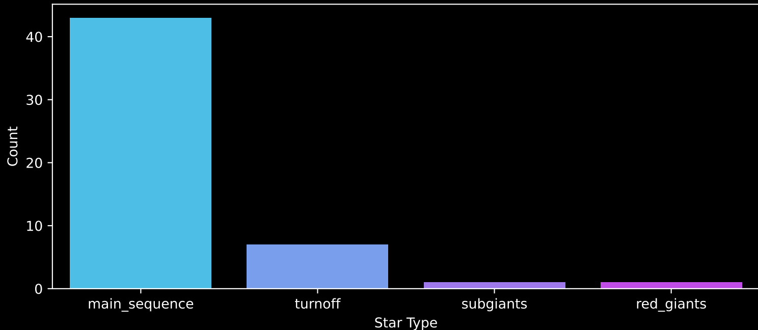
Gaia Cluster: [NGC_225] Count plot of Star Type
