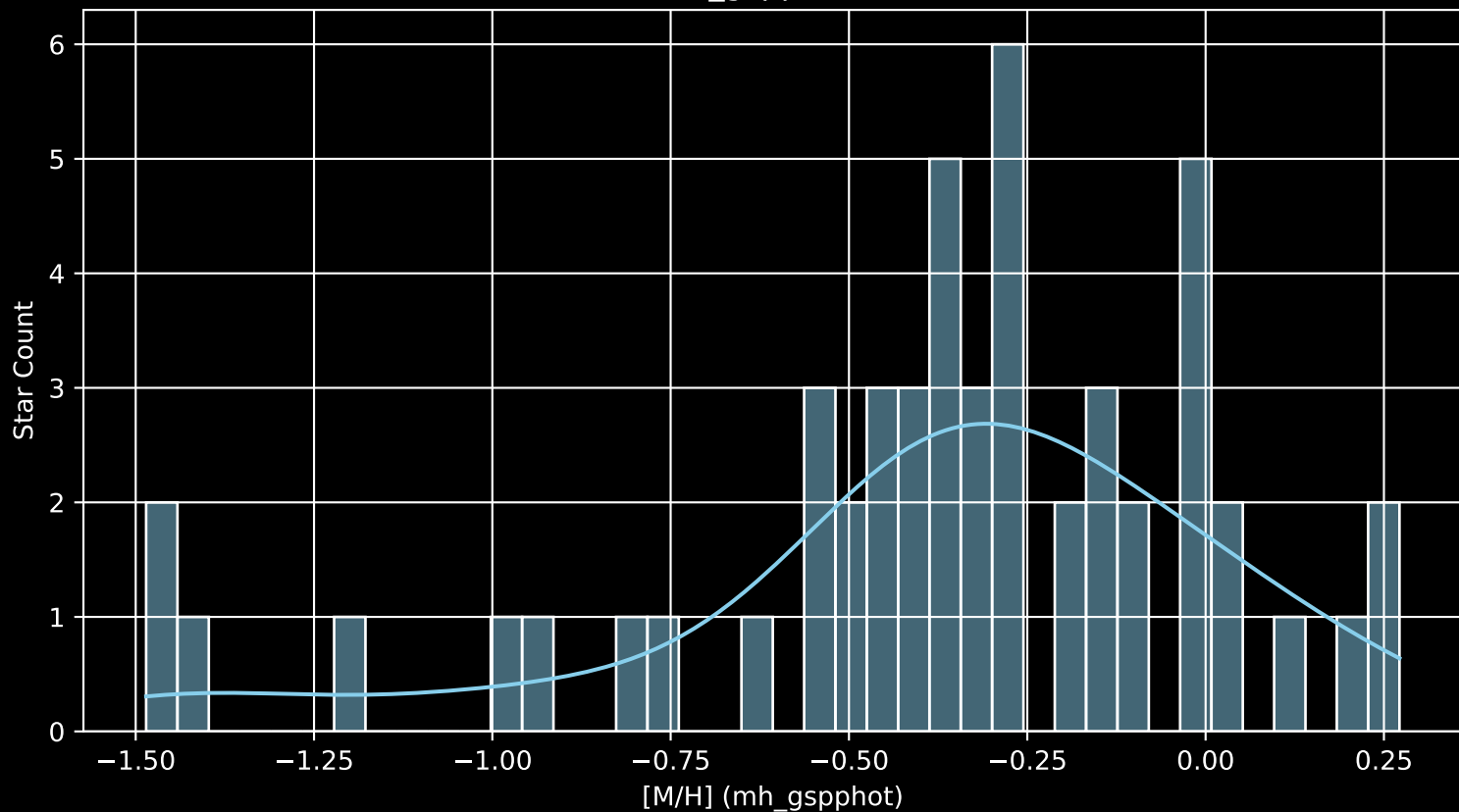
Gaia Cluster: [NGC_225 [M/H] (mh_gspphot) (n= 52)
