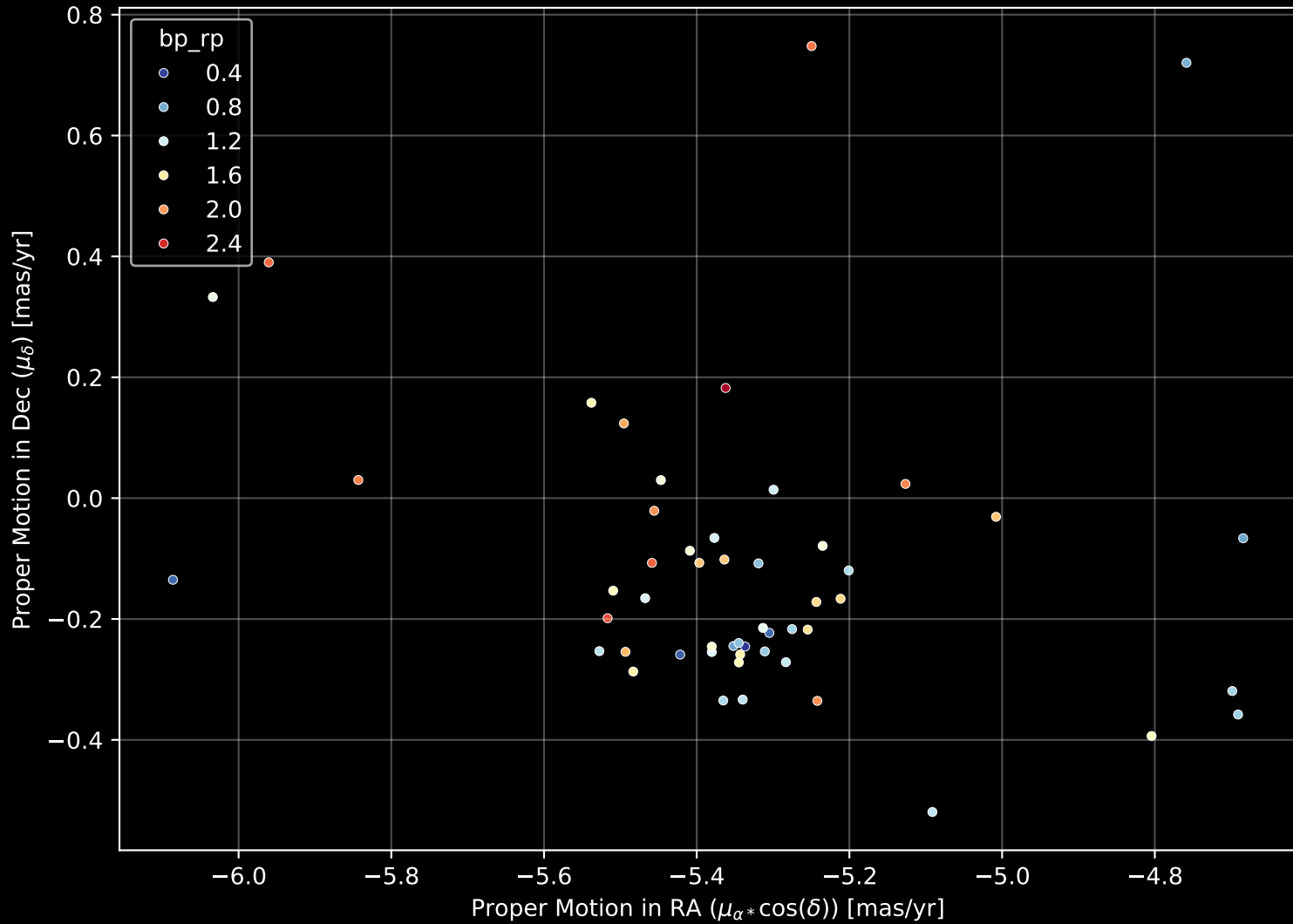
Gaia Cluster: [NGC_225] Proper Motion Diagram (n= 52)
