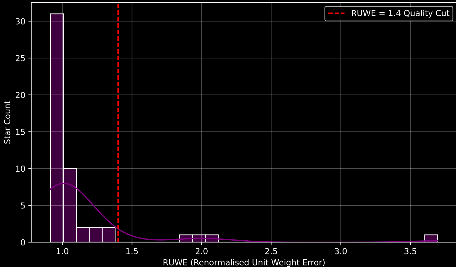
Gaia Cluster: [NGC_225] RUWE Distribution (n= 51)
