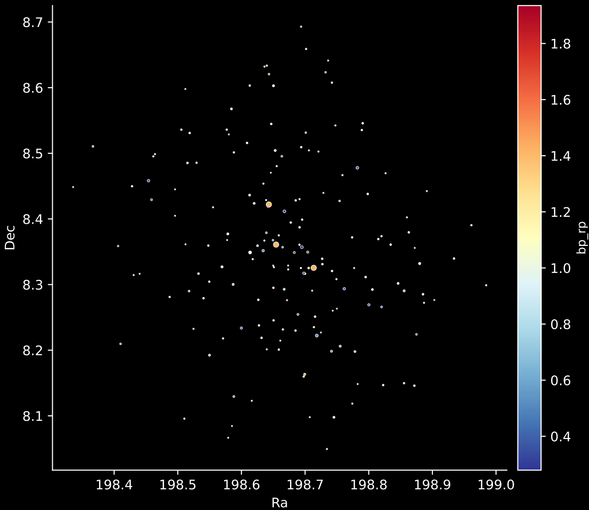
Gaia Cluster: [NGC_2251] Stars: 169
