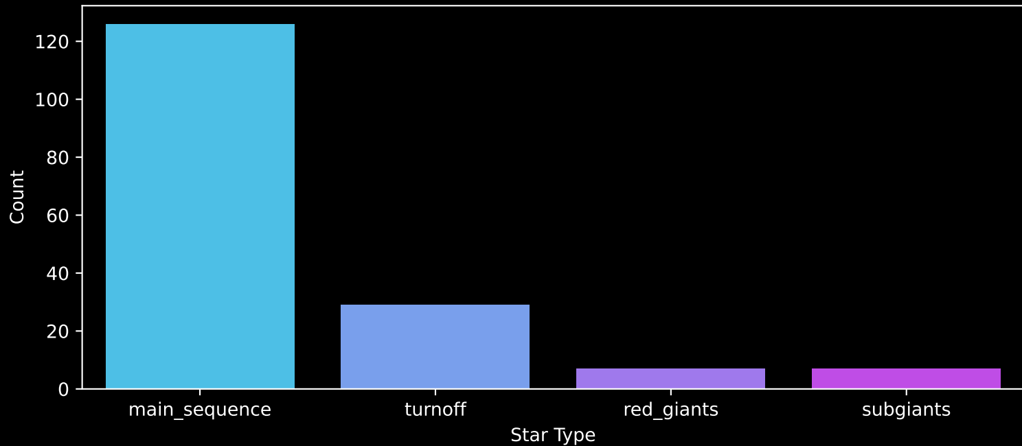
Gaia Cluster: [NGC_2251] Count plot of Star Type
