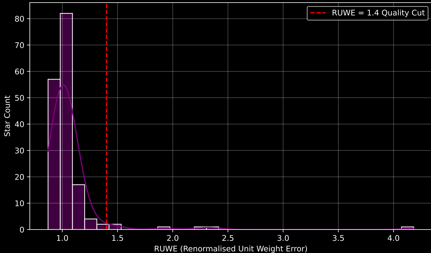
Gaia Cluster: [NGC_2251] RUWE Distribution (n= 168)
