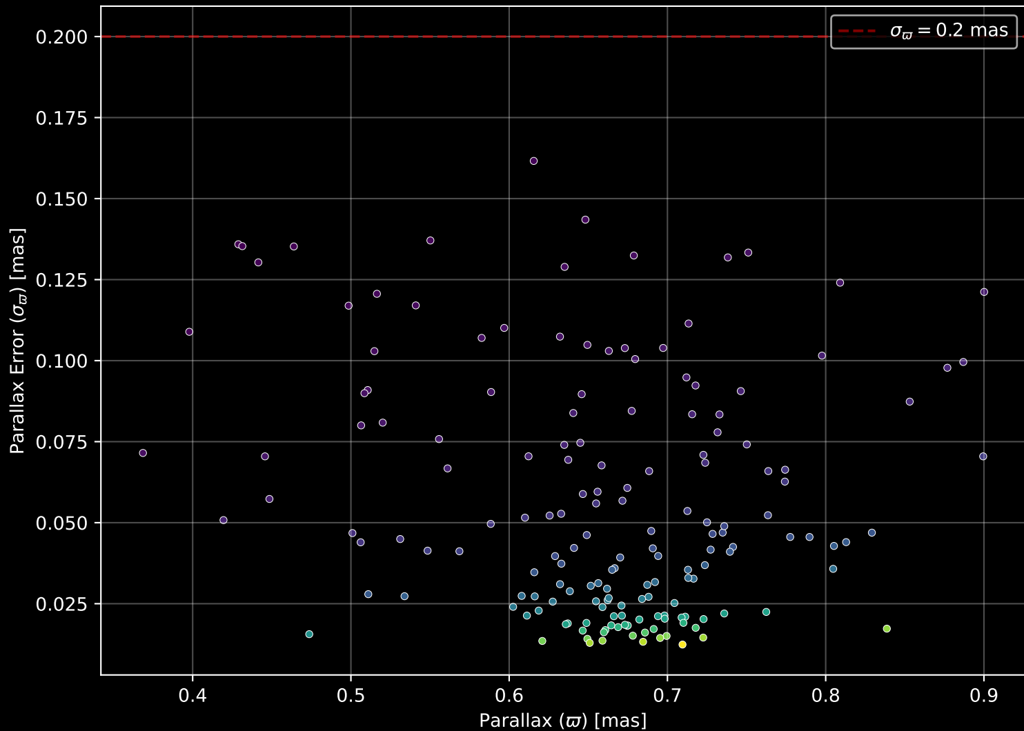
Gaia Cluster: [NGC_2251] Parallax Quality (n= 169)
