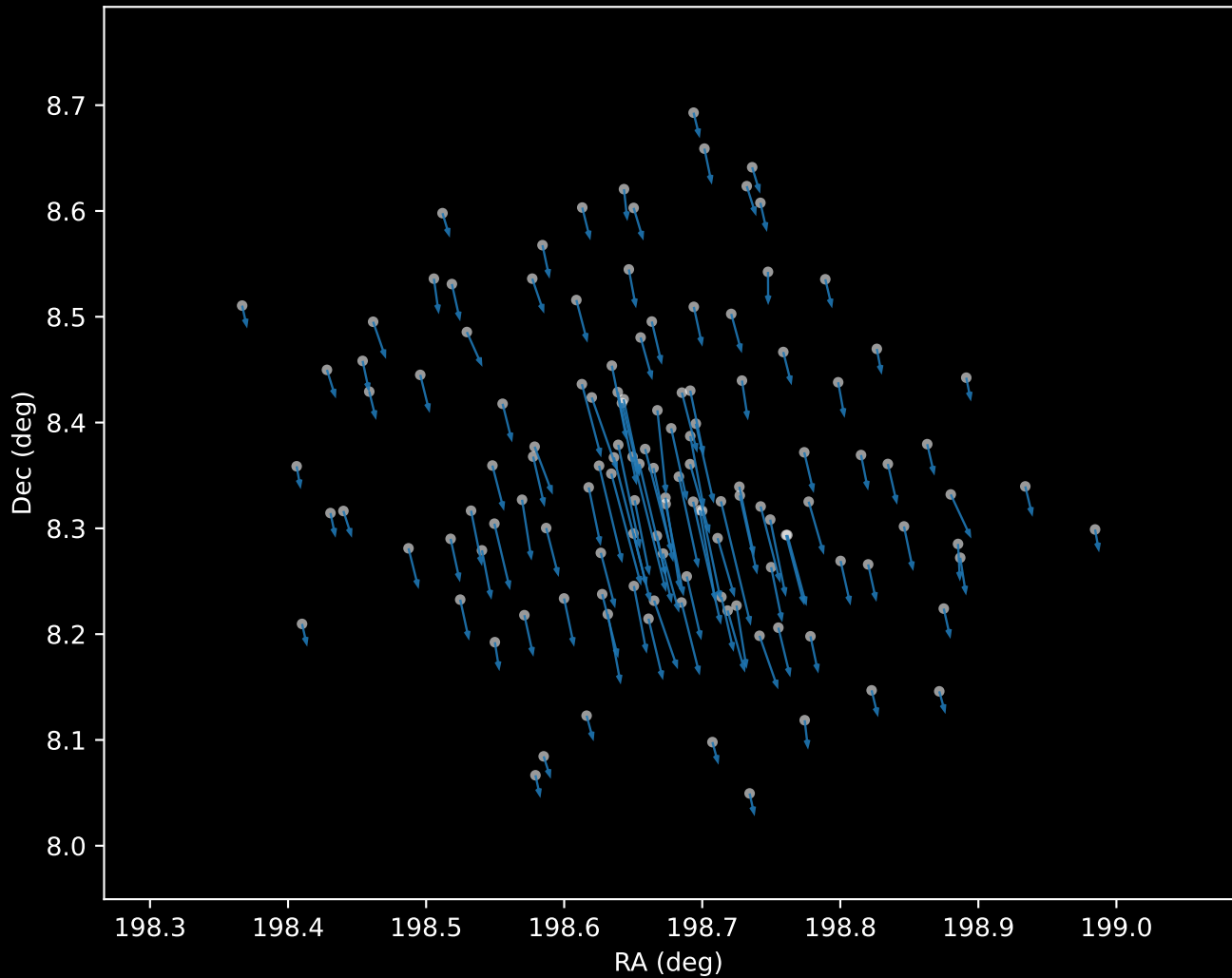
Gaia DR3 Cluster 0 Proper Motion Vectors (n=129)
