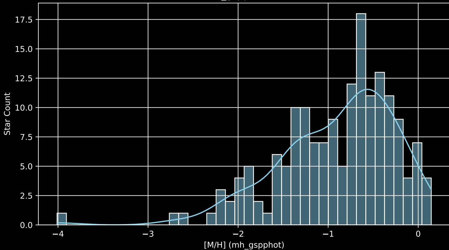
Gaia Cluster: [NGC_2251 [M/H] (mh_gspphot) (n= 169)
