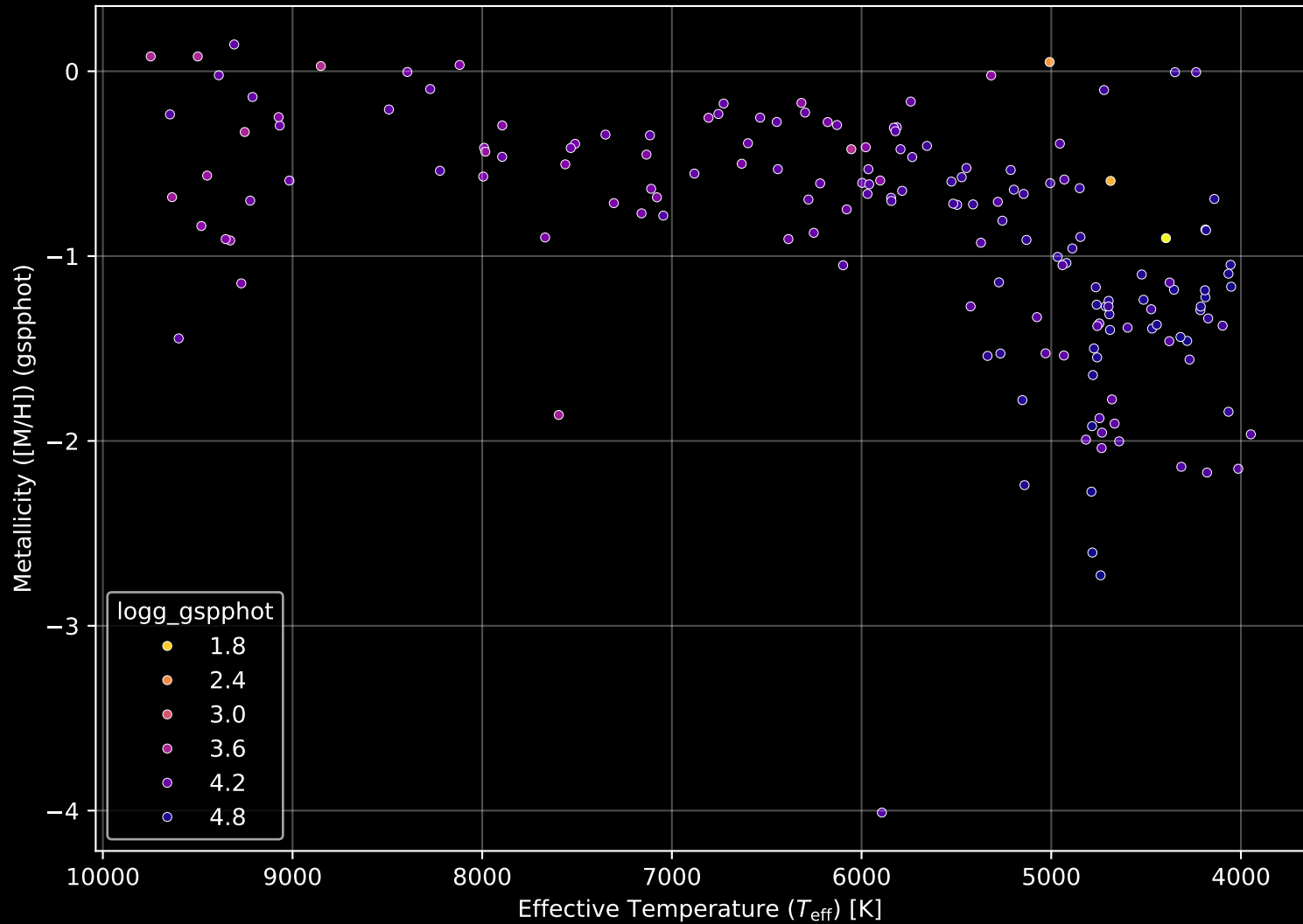
Gaia Cluster: [NGC_2251] Stellar Population Parameters (n= 169)
