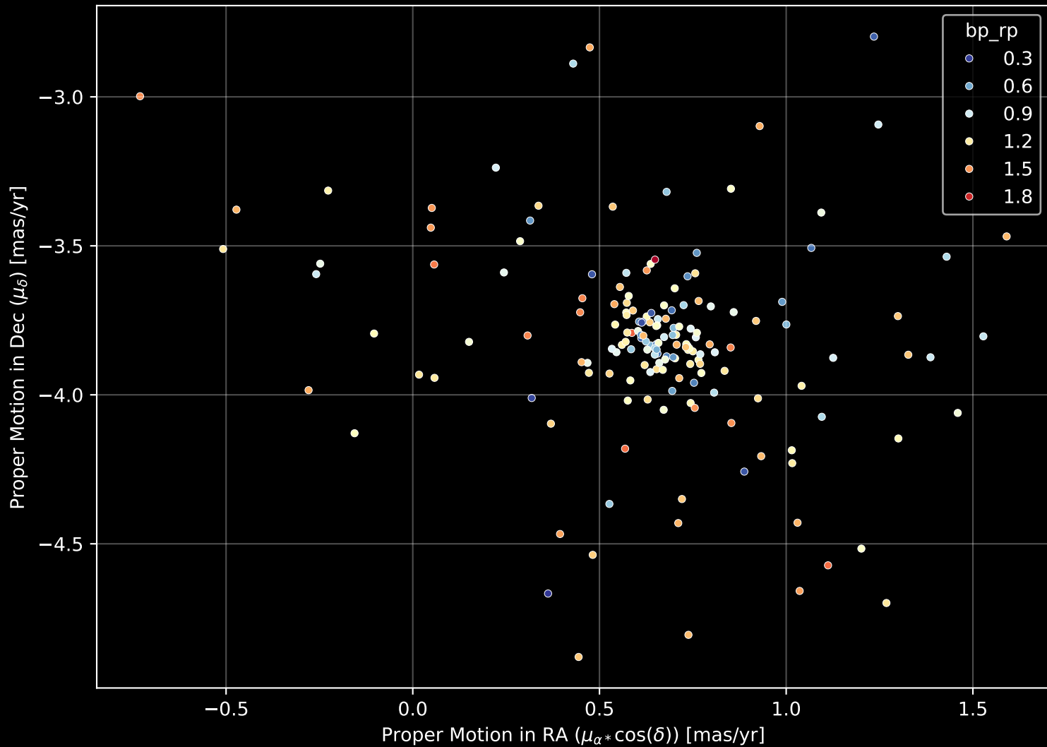
Gaia Cluster: [NGC_2251] Proper Motion Diagram (n= 169)
