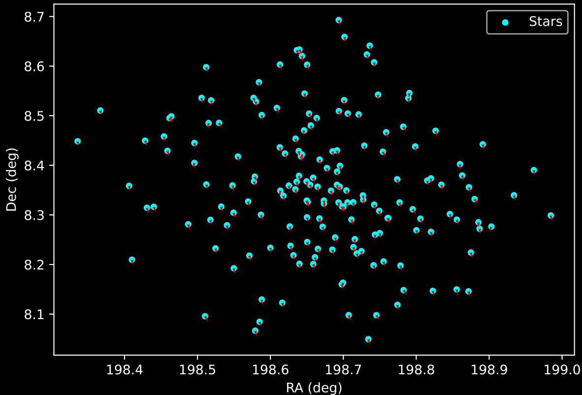
Gaia Cluster: [NGC_2251] Proper Motion Vectors for Gaia Star Field (n= 169)
