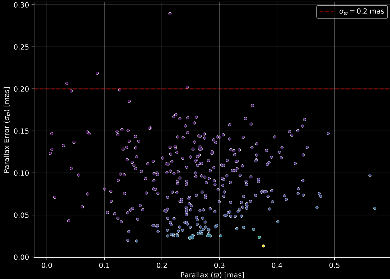
Gaia Cluster: [NGC_2262] Parallax Quality (n= 309)
