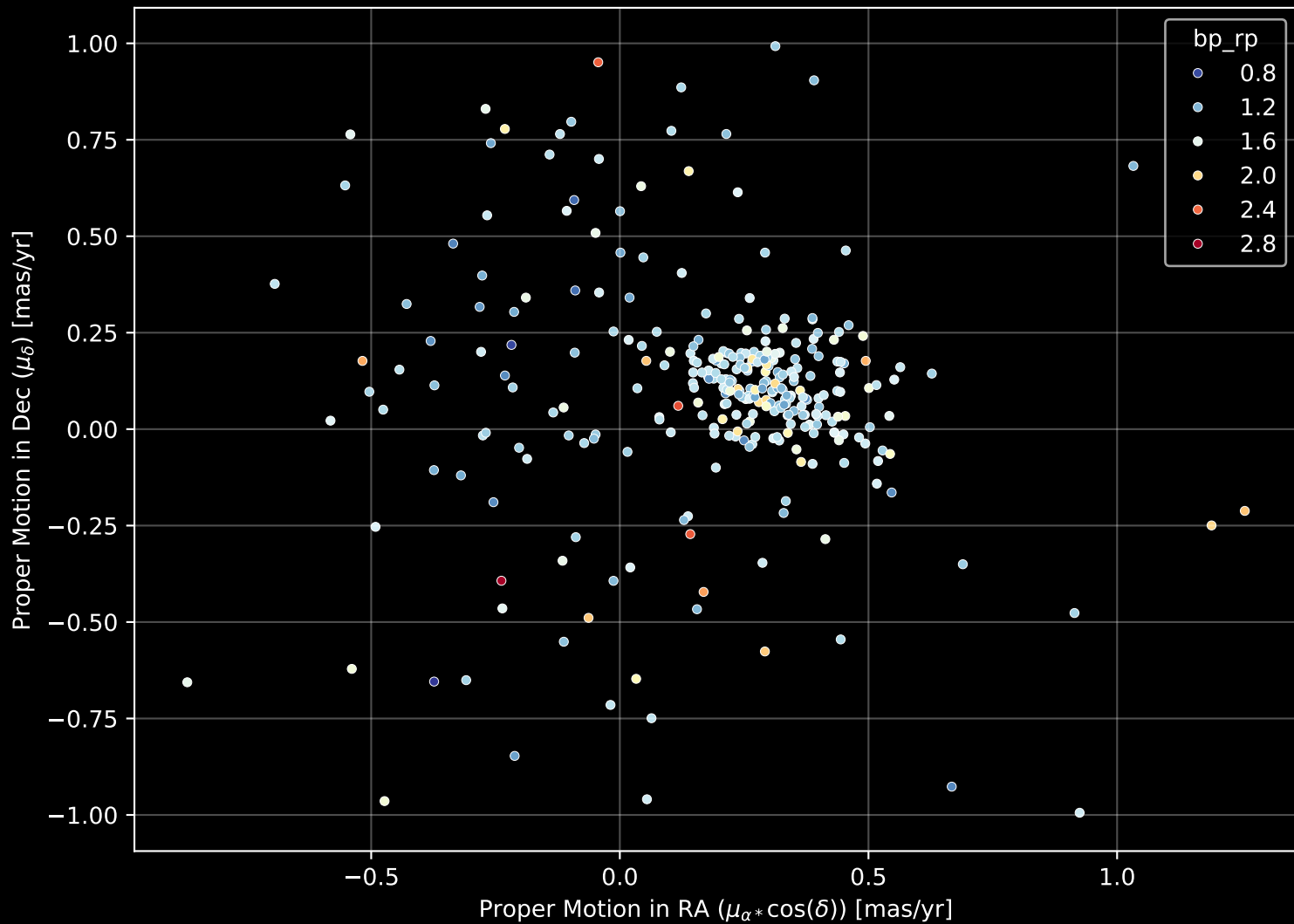
Gaia Cluster: [NGC_2262] Proper Motion Diagram (n= 309)
