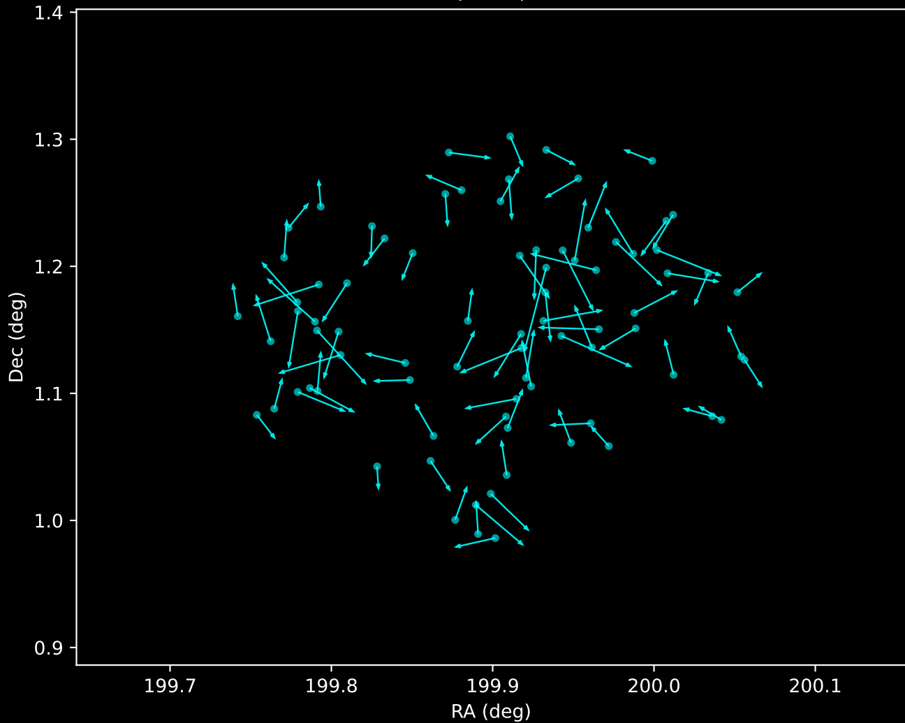
Gaia DR3 Noise Stream Proper Motion Vectors (n=80)
