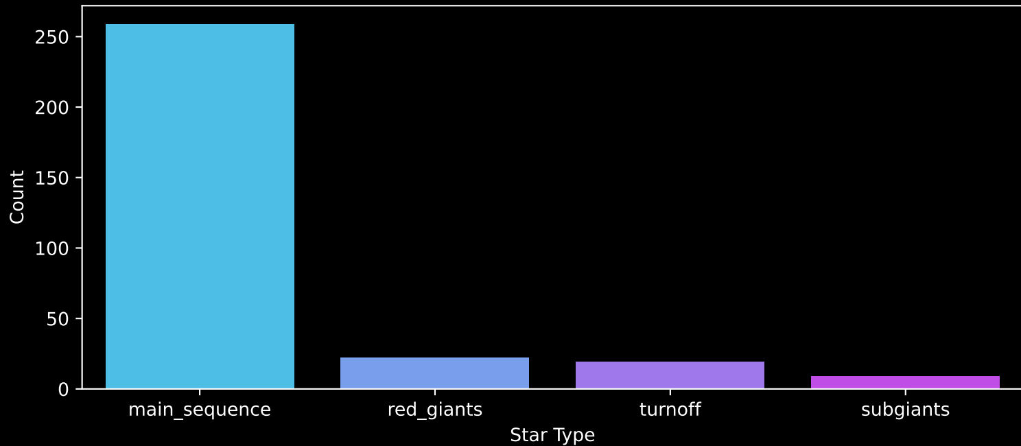
Gaia Cluster: [NGC_2262] Count plot of Star Type
