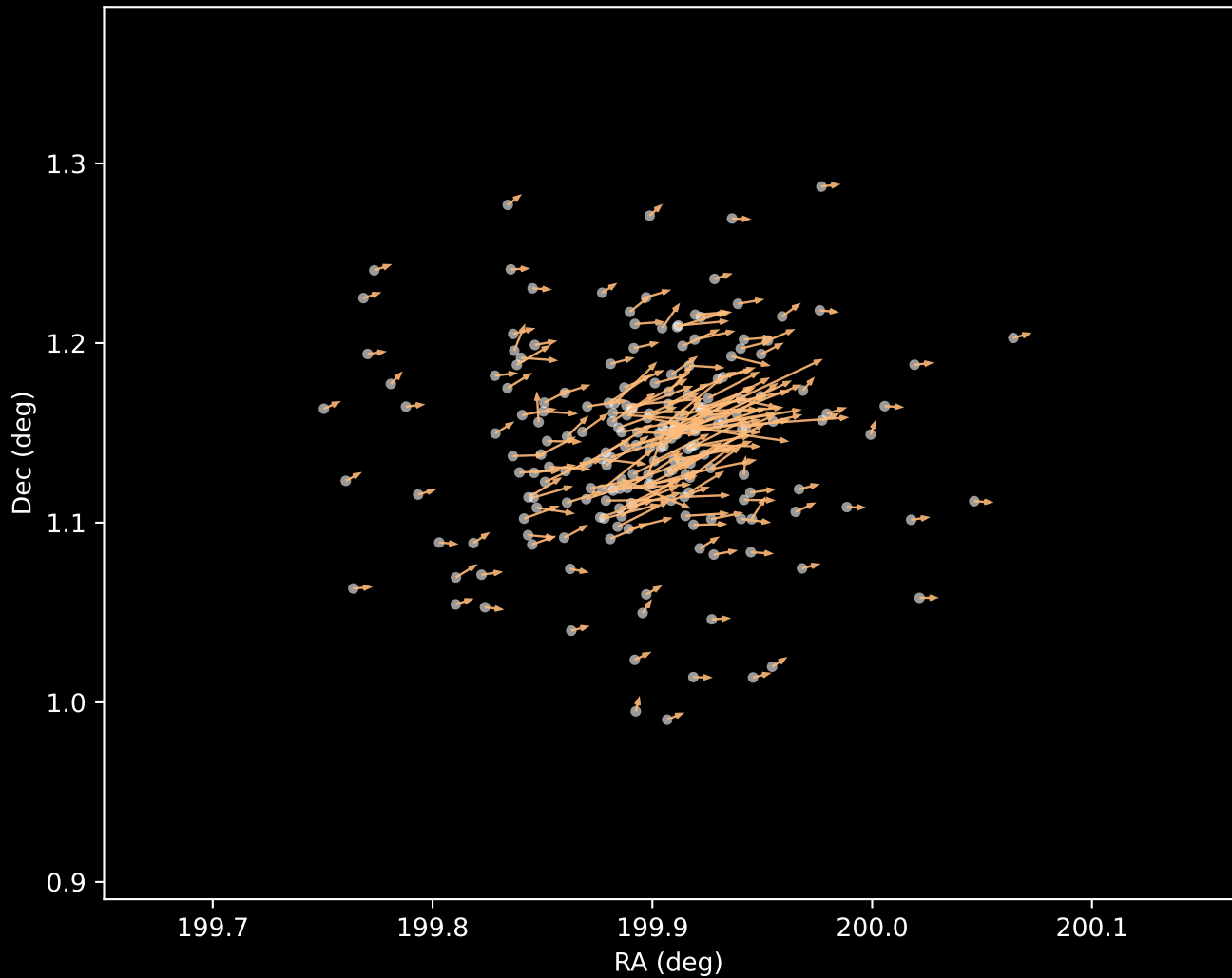
Gaia DR3 Cluster 3 Proper Motion Vectors (n=207)
