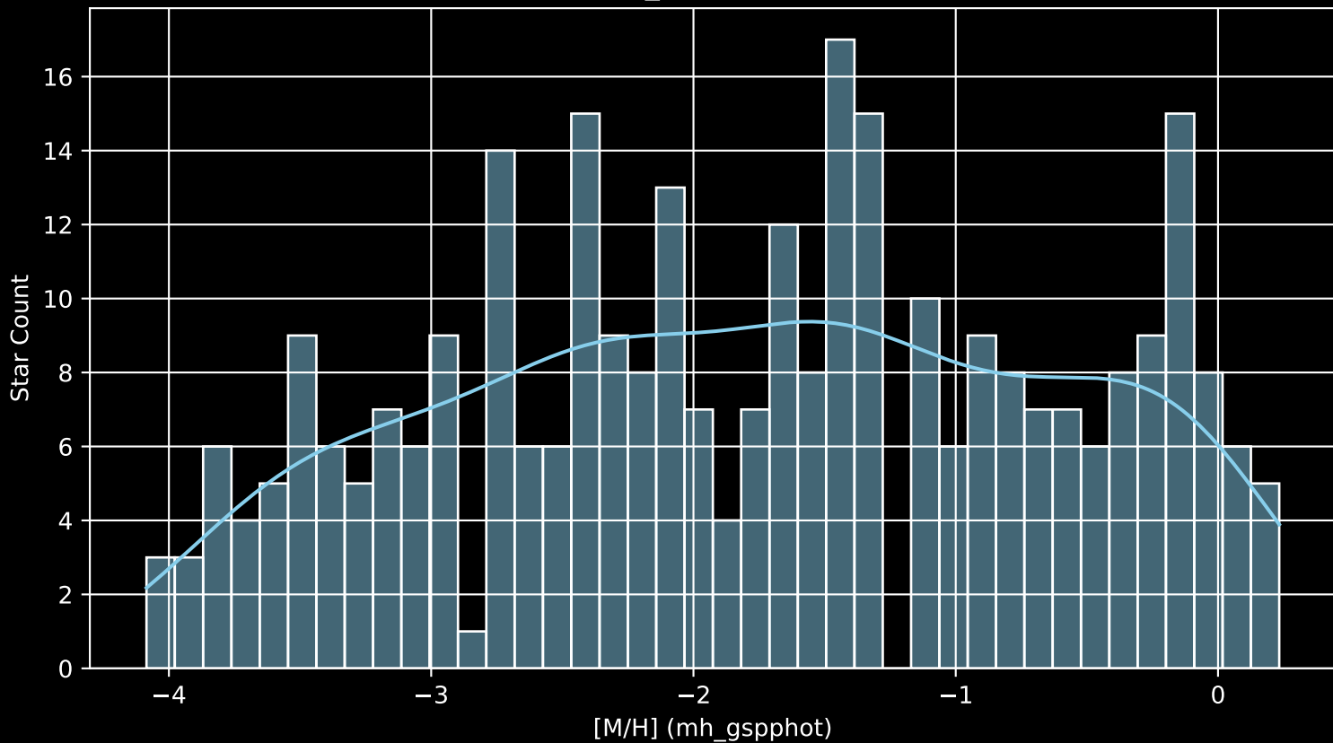
Gaia Cluster: [NGC_2262 [M/H] (mh_gspphot) (n= 309)
