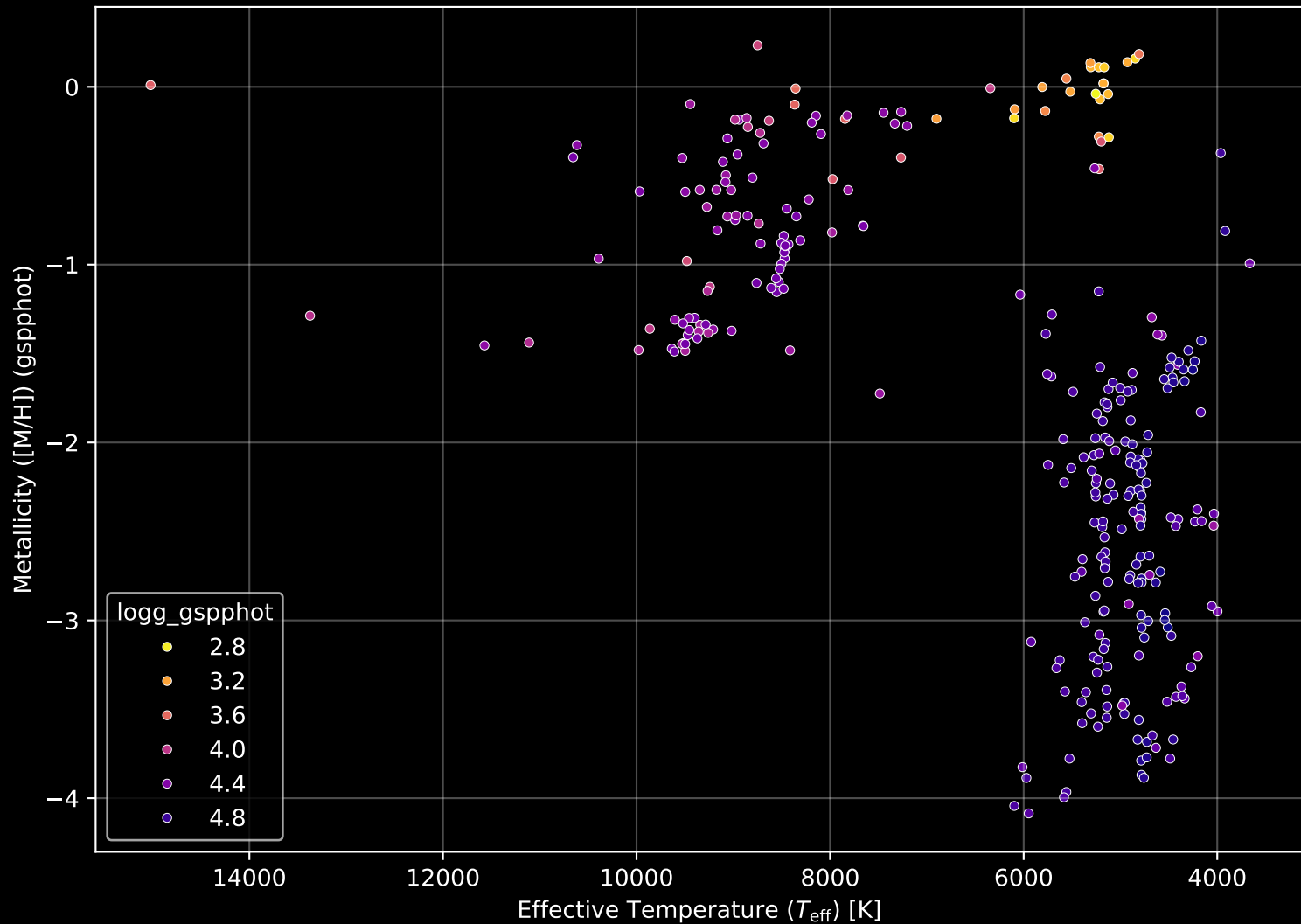
Gaia Cluster: [NGC_2262] Stellar Population Parameters (n= 309)
