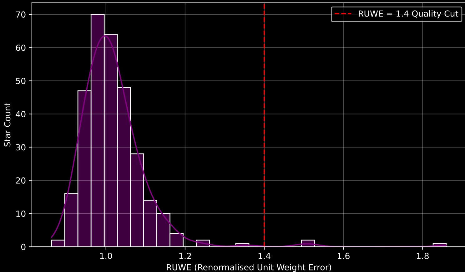
Gaia Cluster: [NGC_2262] RUWE Distribution (n= 309)
