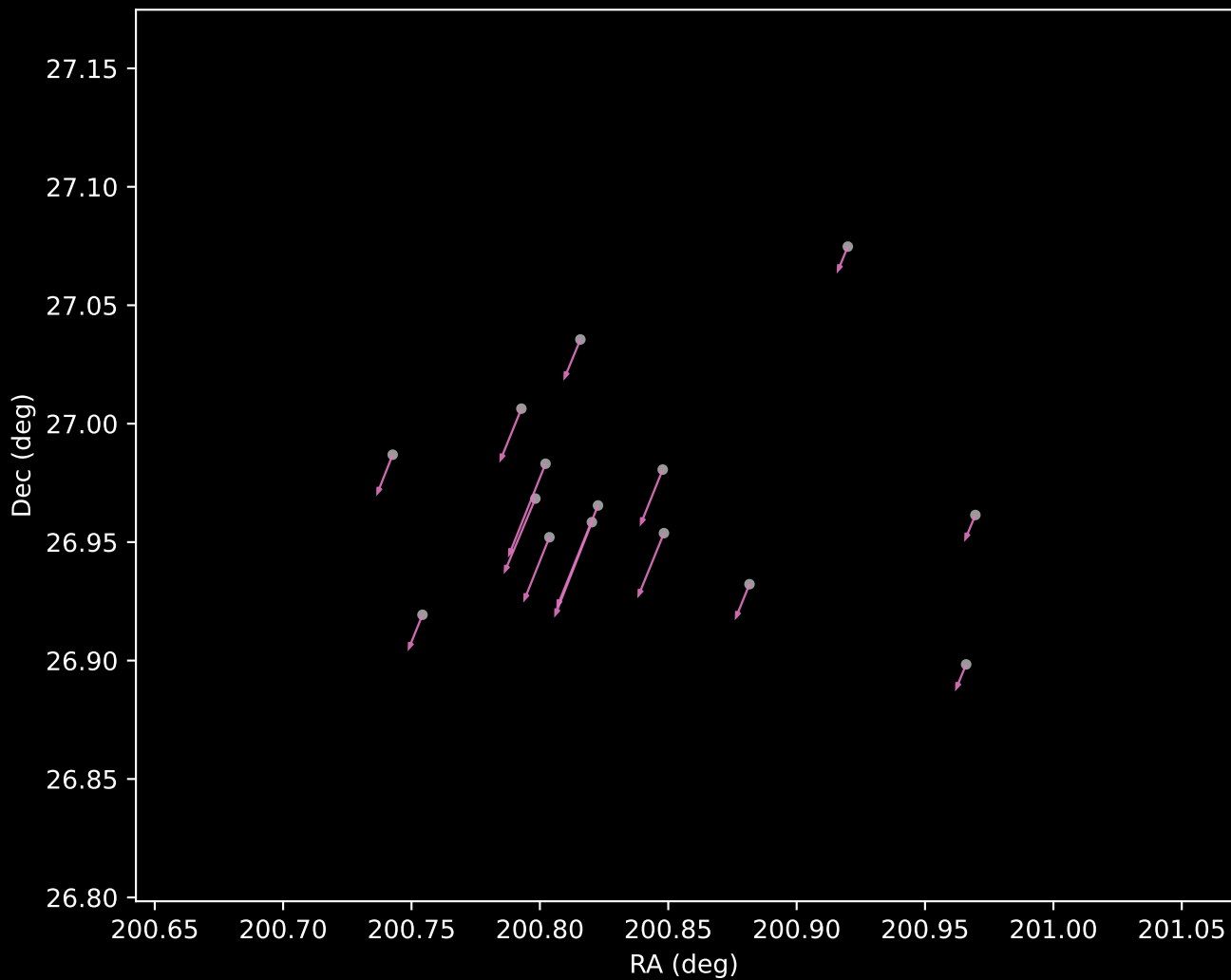
Gaia DR3 Cluster 12 Proper Motion Vectors (n=15)
