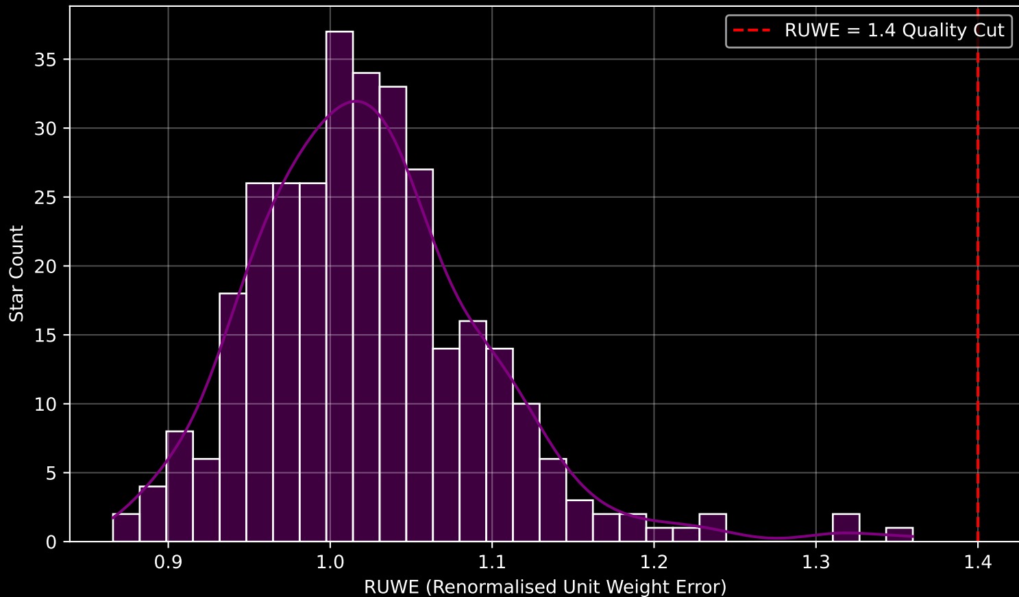
Gaia Cluster: [NGC_2266] RUWE Distribution (n= 321)
