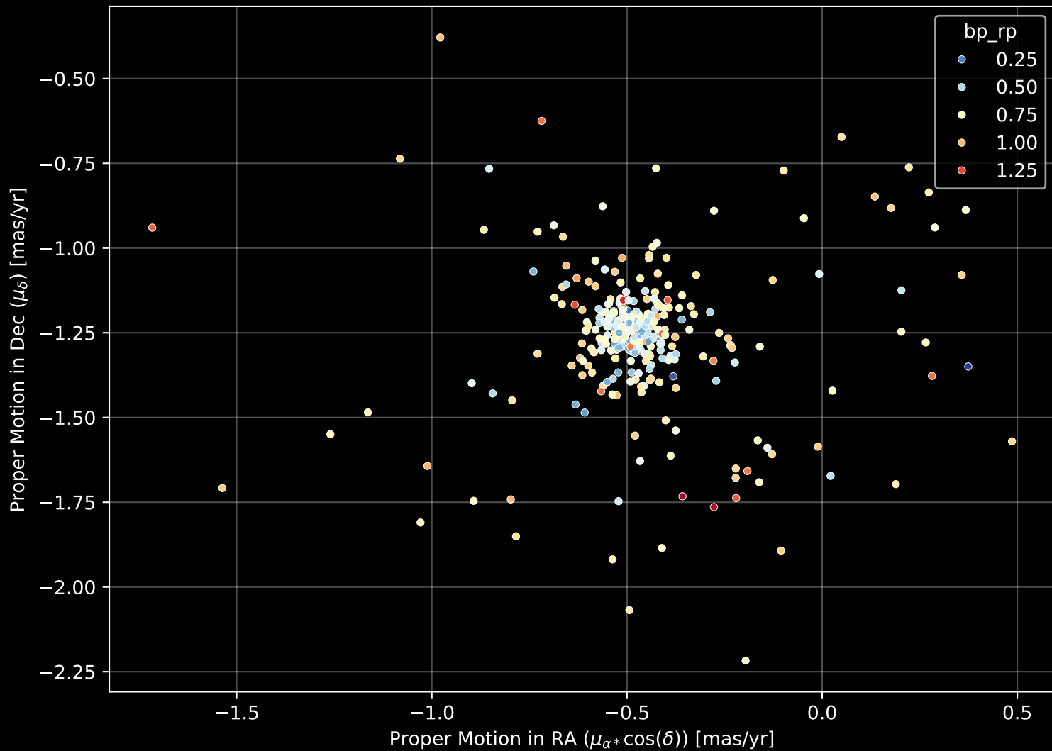
Gaia Cluster: [NGC_2266] Proper Motion Diagram (n= 321)
