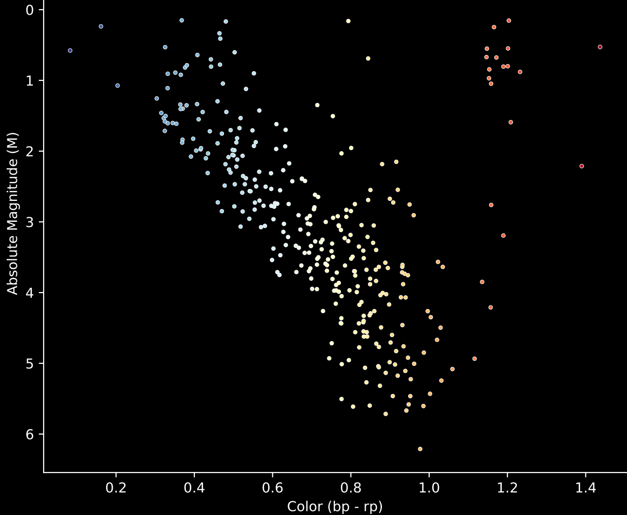
Gaia Cluster: [NGC 2266] Stars (n= 321) Hertzsprung-Russel Diagram
