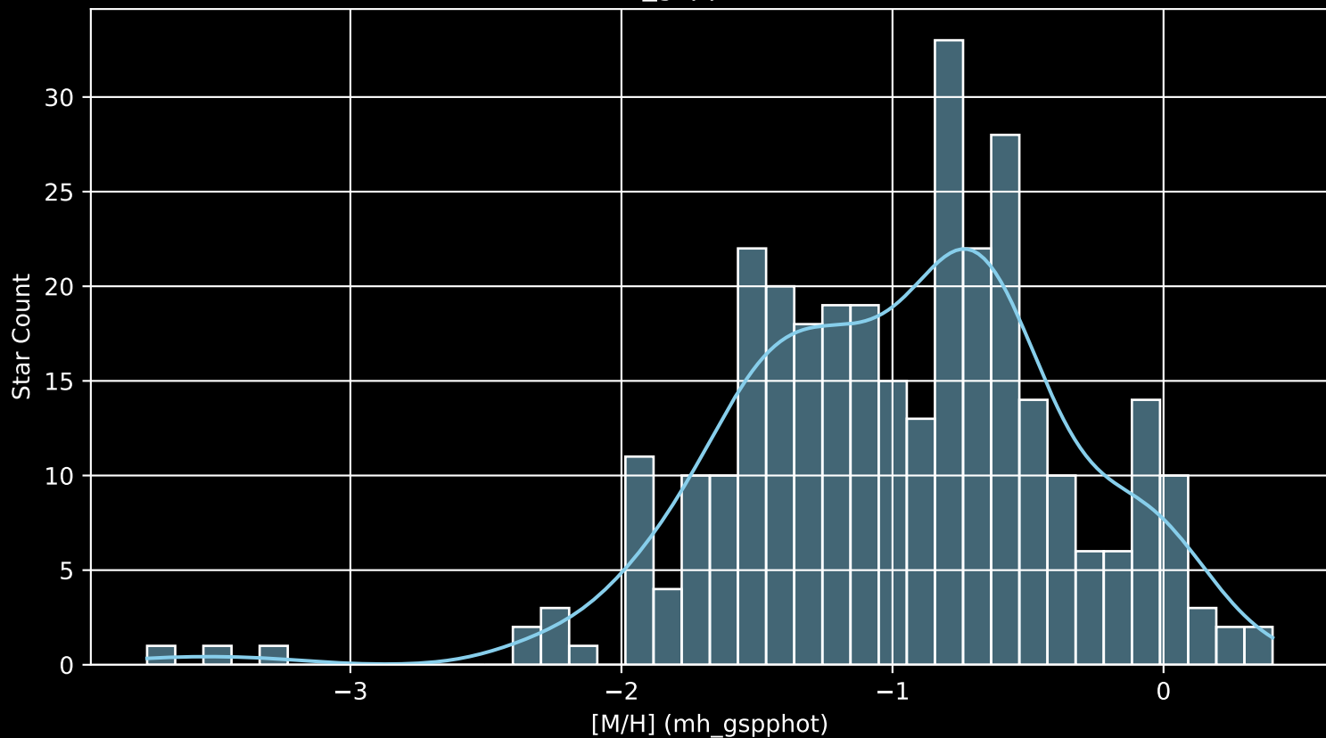
Gaia Cluster: [NGC_2266 [M/H] (mh_gspphot) (n= 320)
