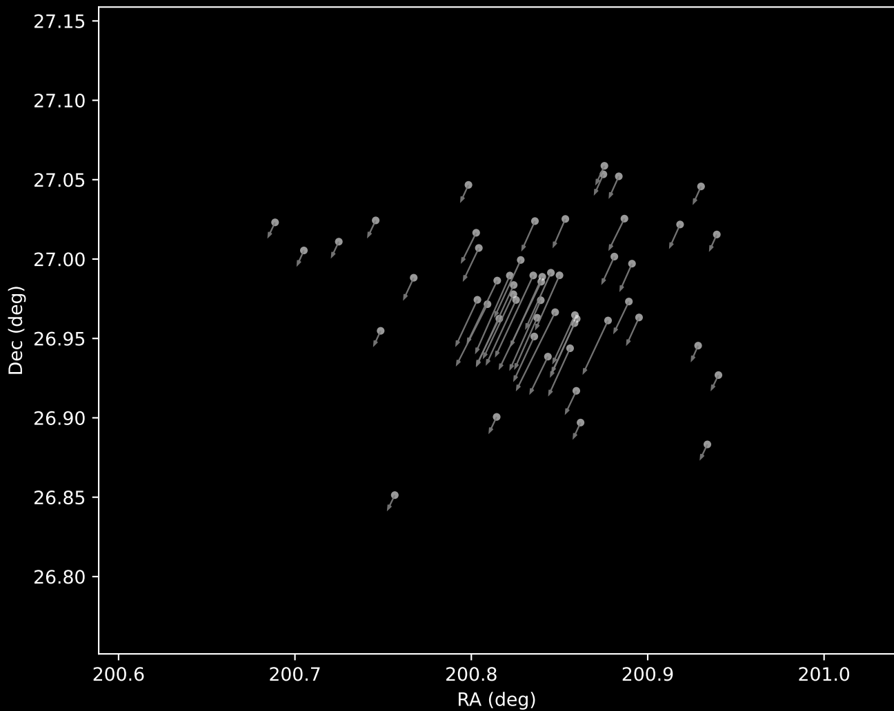
Gaia DR3 Cluster 14 Proper Motion Vectors (n=53)
