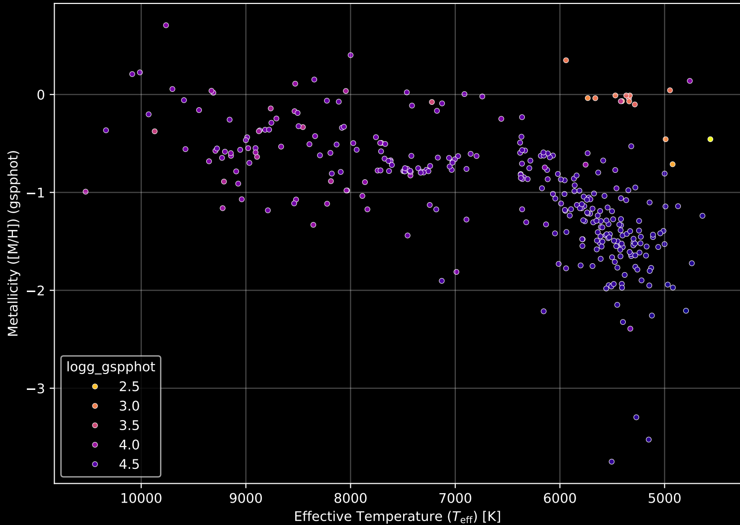
Gaia Cluster: [NGC_2266] Stellar Population Parameters (n= 321)
