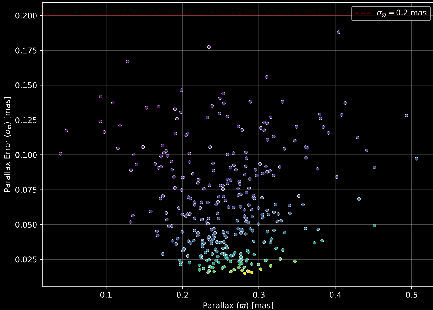
Gaia Cluster: [NGC_2266] Parallax Quality (n= 321)
