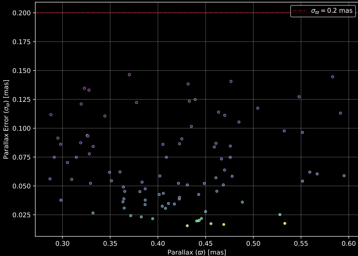
Gaia Cluster: [NGC_2269] Parallax Quality (n= 94)
