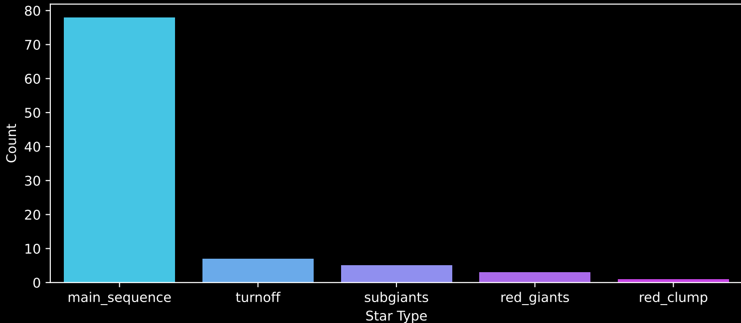
Gaia Cluster: [NGC_2269] Count plot of Star Type
