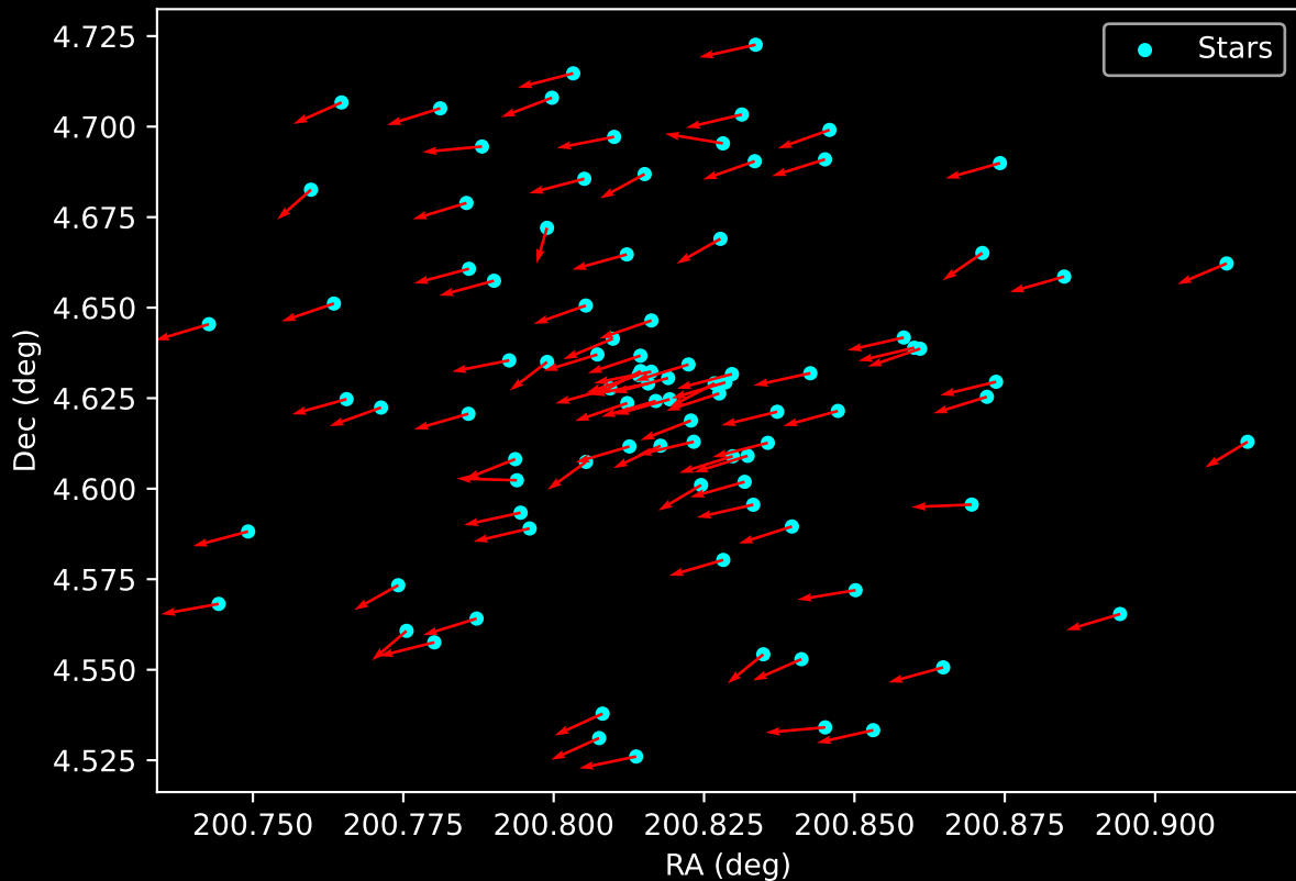
Gaia Cluster: [NGC_2269] Proper Motion Vectors for Gaia Star Field (n= 94)
