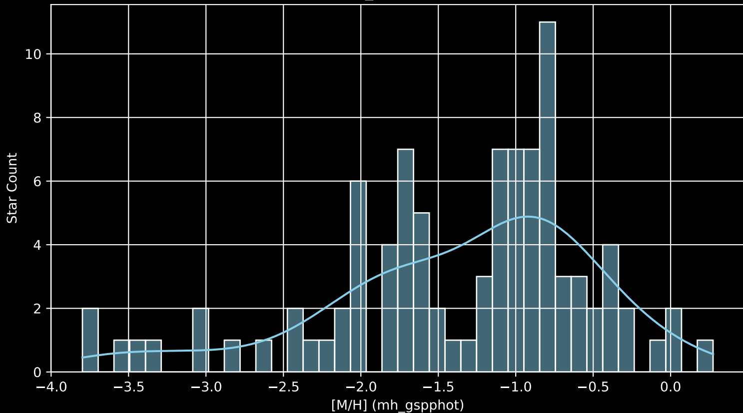
Gaia Cluster: [NGC_2269 [M/H] (mh_gspphot) (n= 94)
