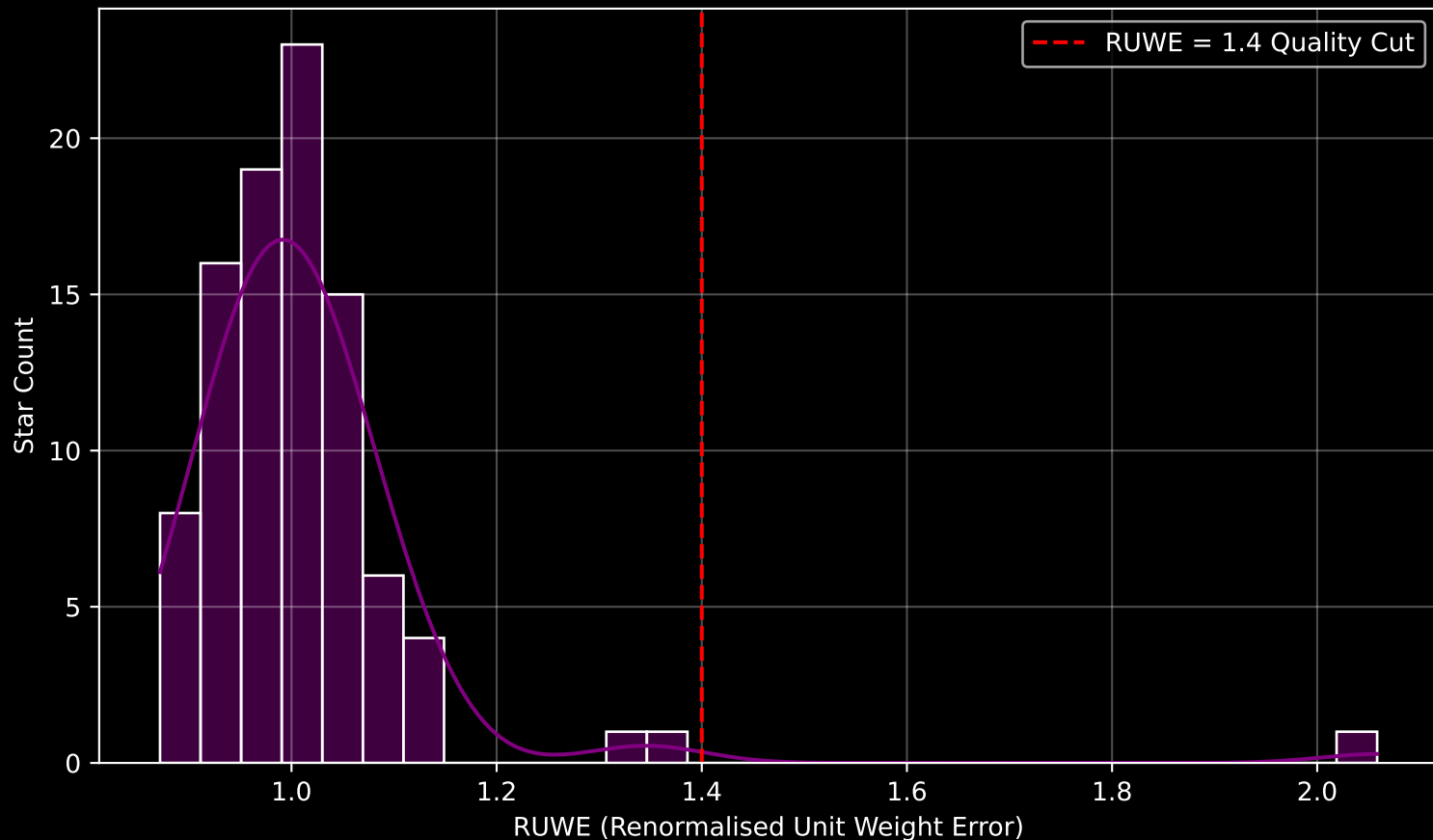
Gaia Cluster: [NGC_2269] RUWE Distribution (n= 94)
