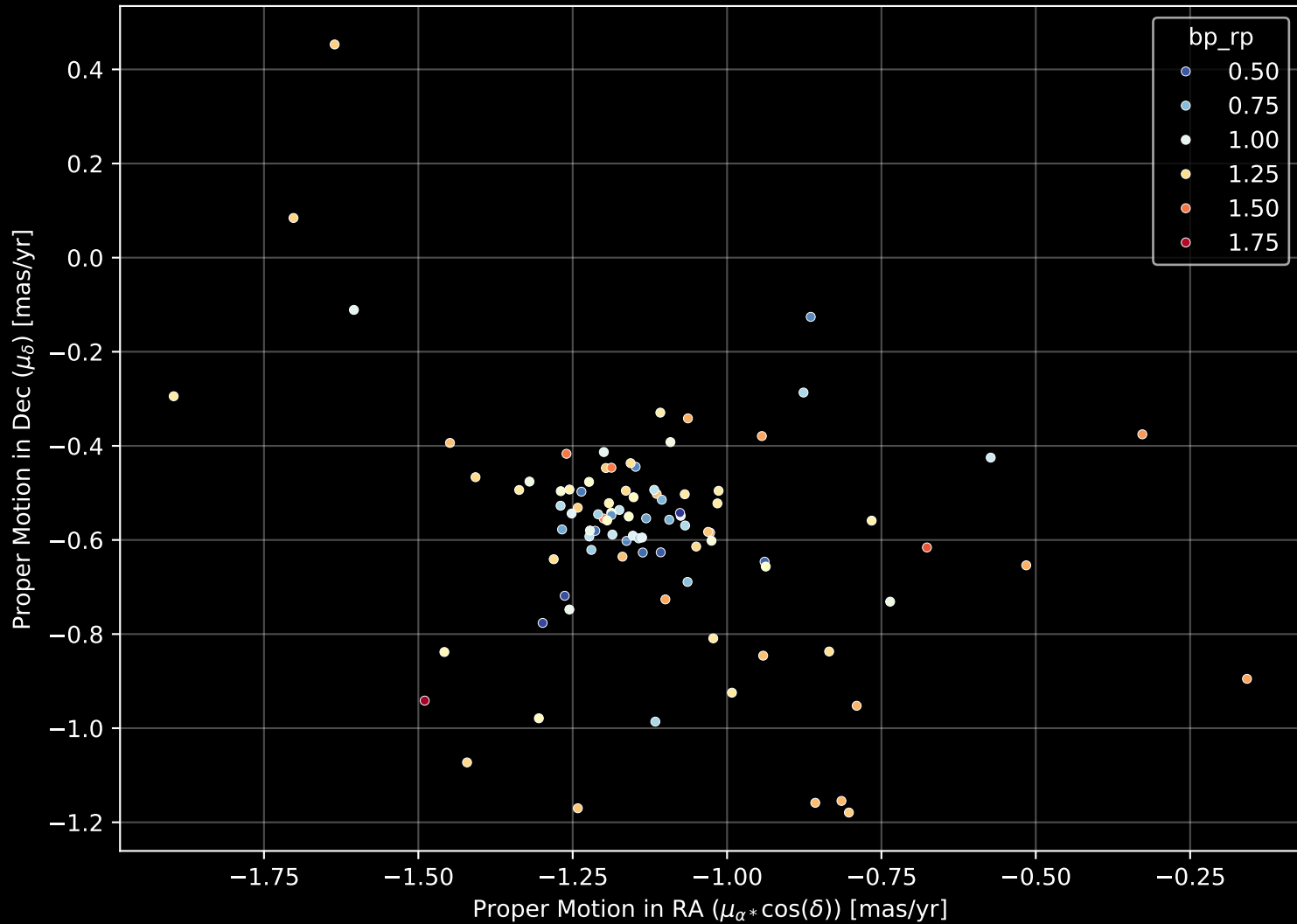
Gaia Cluster: [NGC_2269] Proper Motion Diagram (n= 94)
