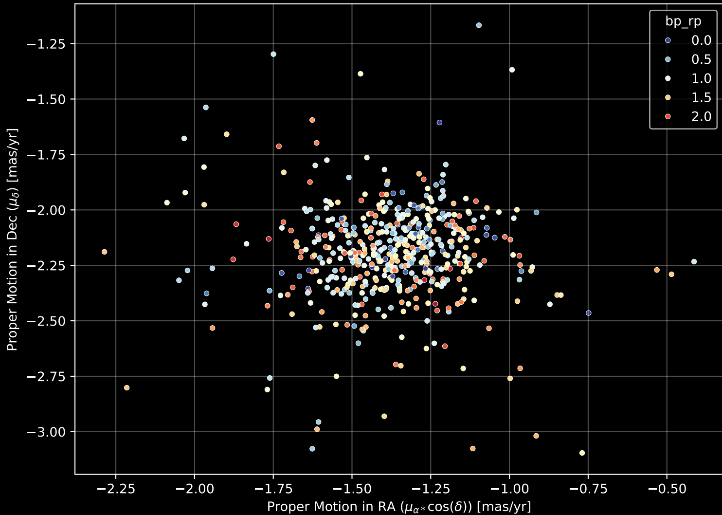
Gaia Cluster: [NGC_2301] Proper Motion Diagram (n= 516)
