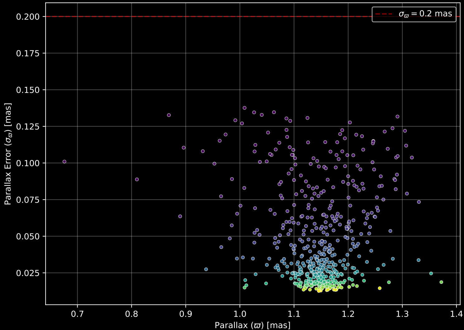
Gaia Cluster: [NGC_2301] Parallax Quality (n= 516)
