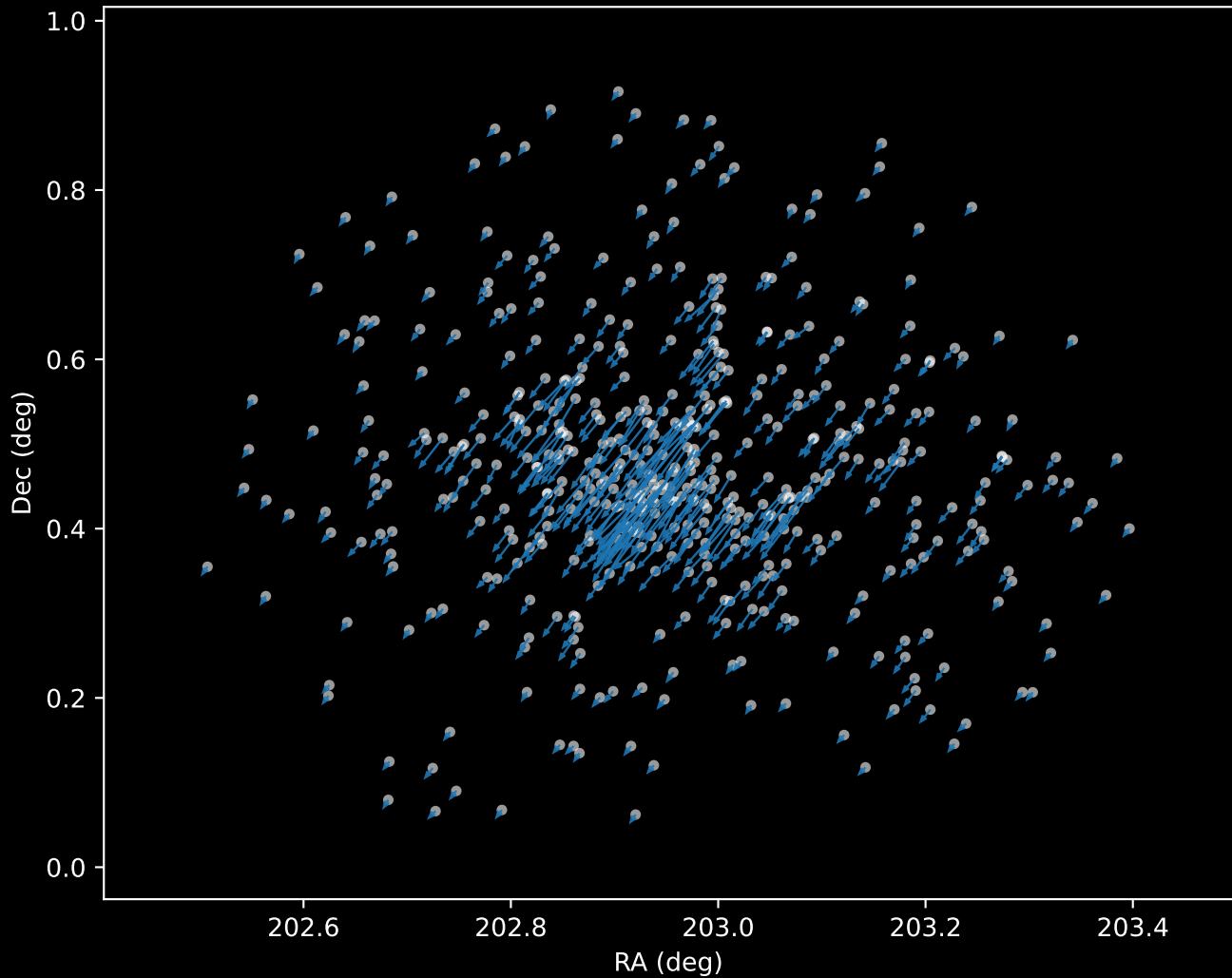
Gaia DR3 Cluster 0 Proper Motion Vectors (n=480)
