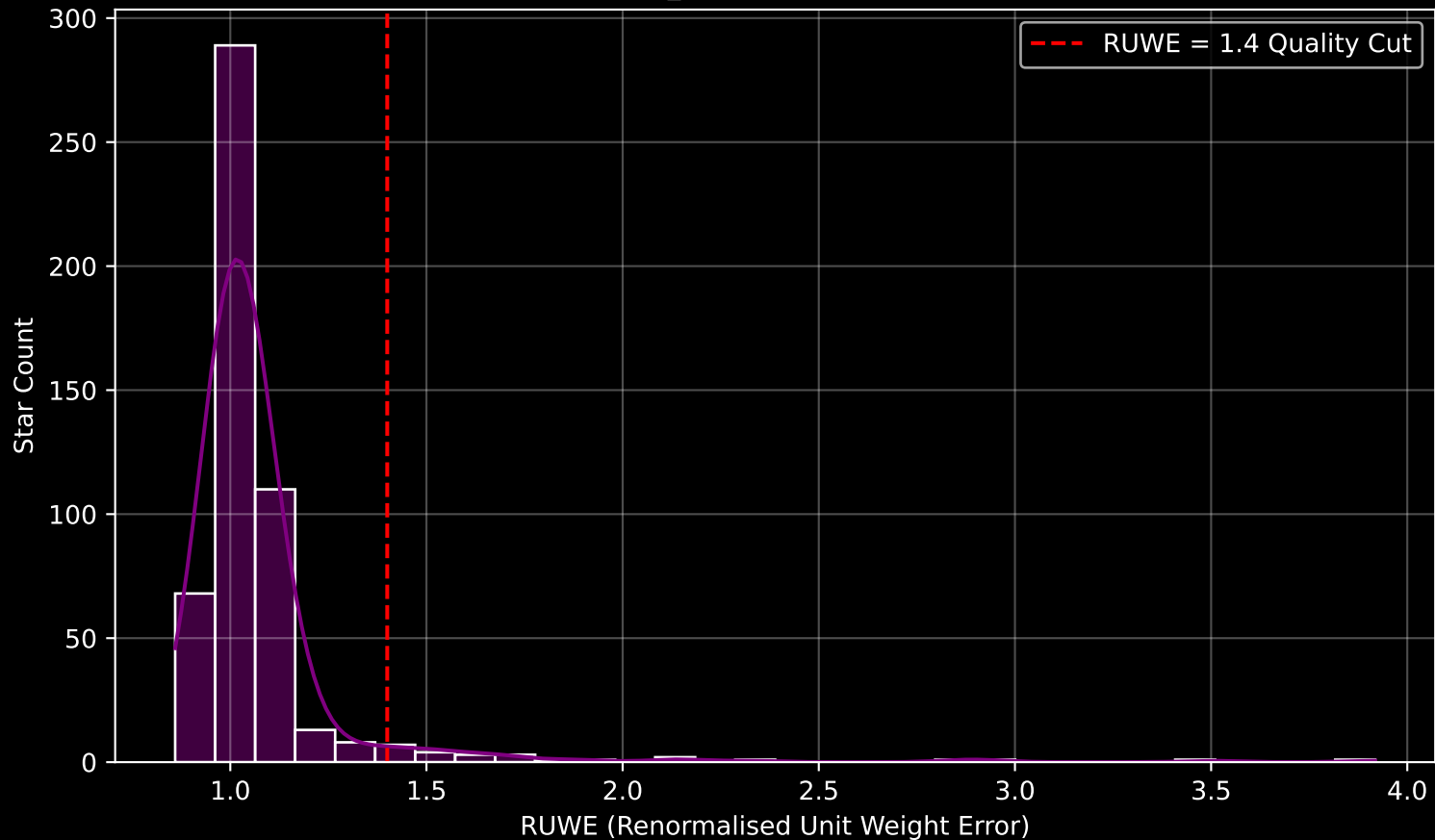
Gaia Cluster: [NGC_2301] RUWE Distribution (n= 514)
