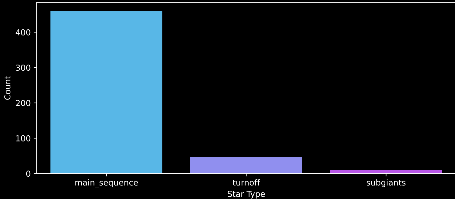
Gaia Cluster: [NGC_2301] Count plot of Star Type
