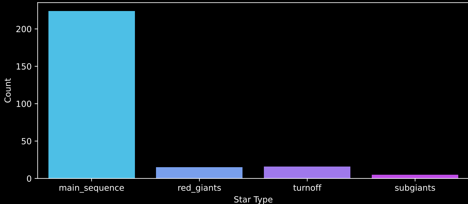
Gaia Cluster: [NGC_2304] Count plot of Star Type
