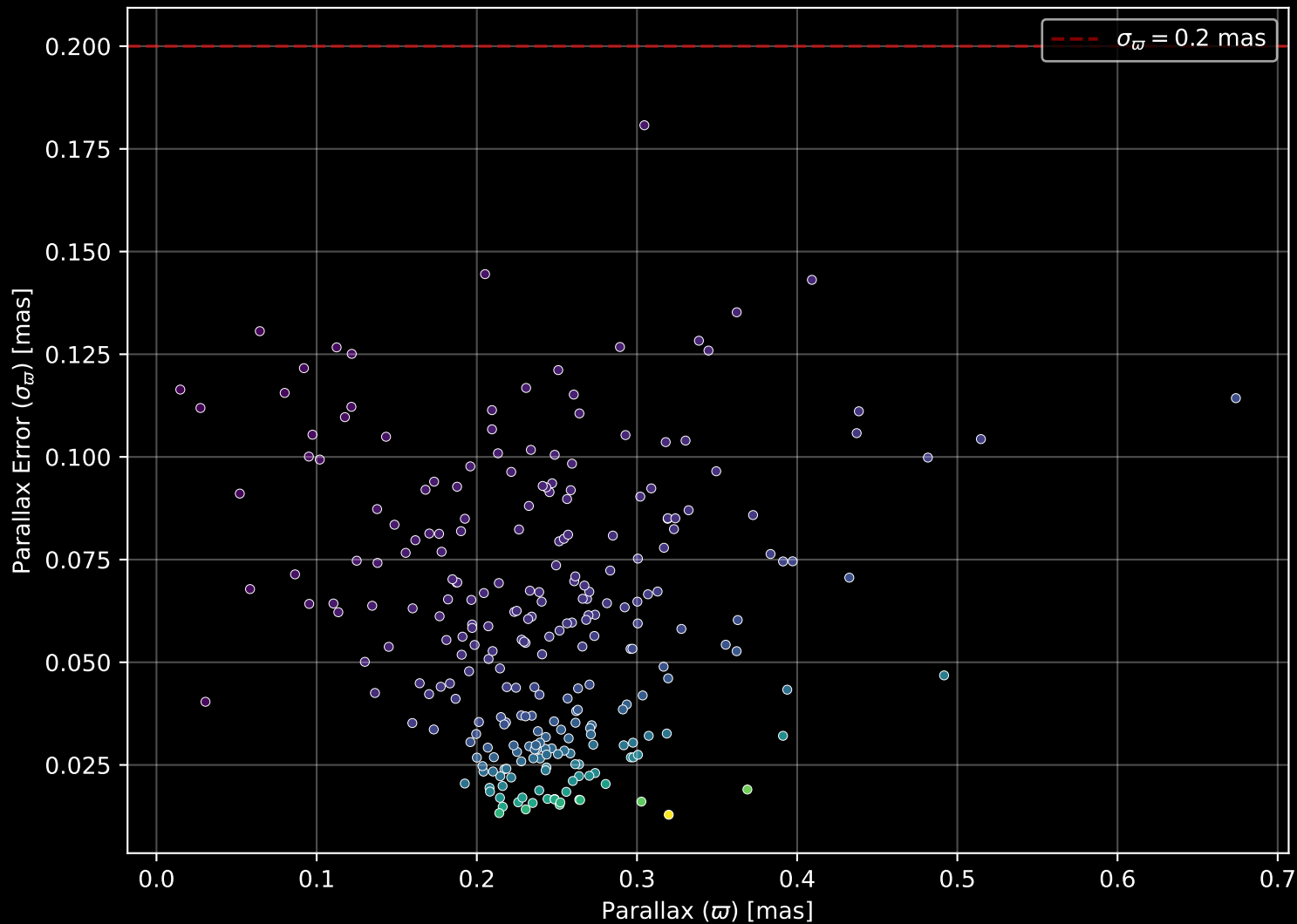
Gaia Cluster: [NGC_2304] Parallax Quality (n= 260)
