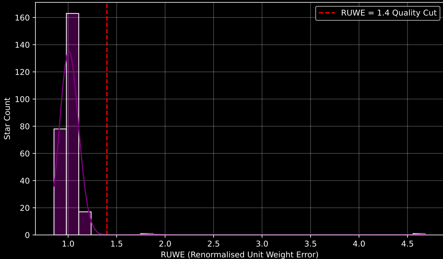
Gaia Cluster: [NGC_2304] RUWE Distribution (n= 260)
