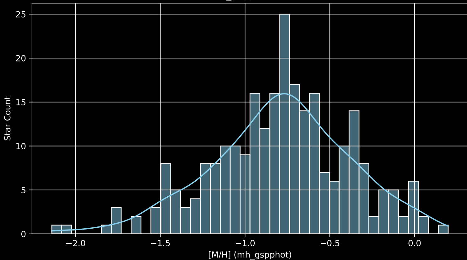
Gaia Cluster: [NGC_2304 [M/H] (mh_gspphot) (n= 260)
