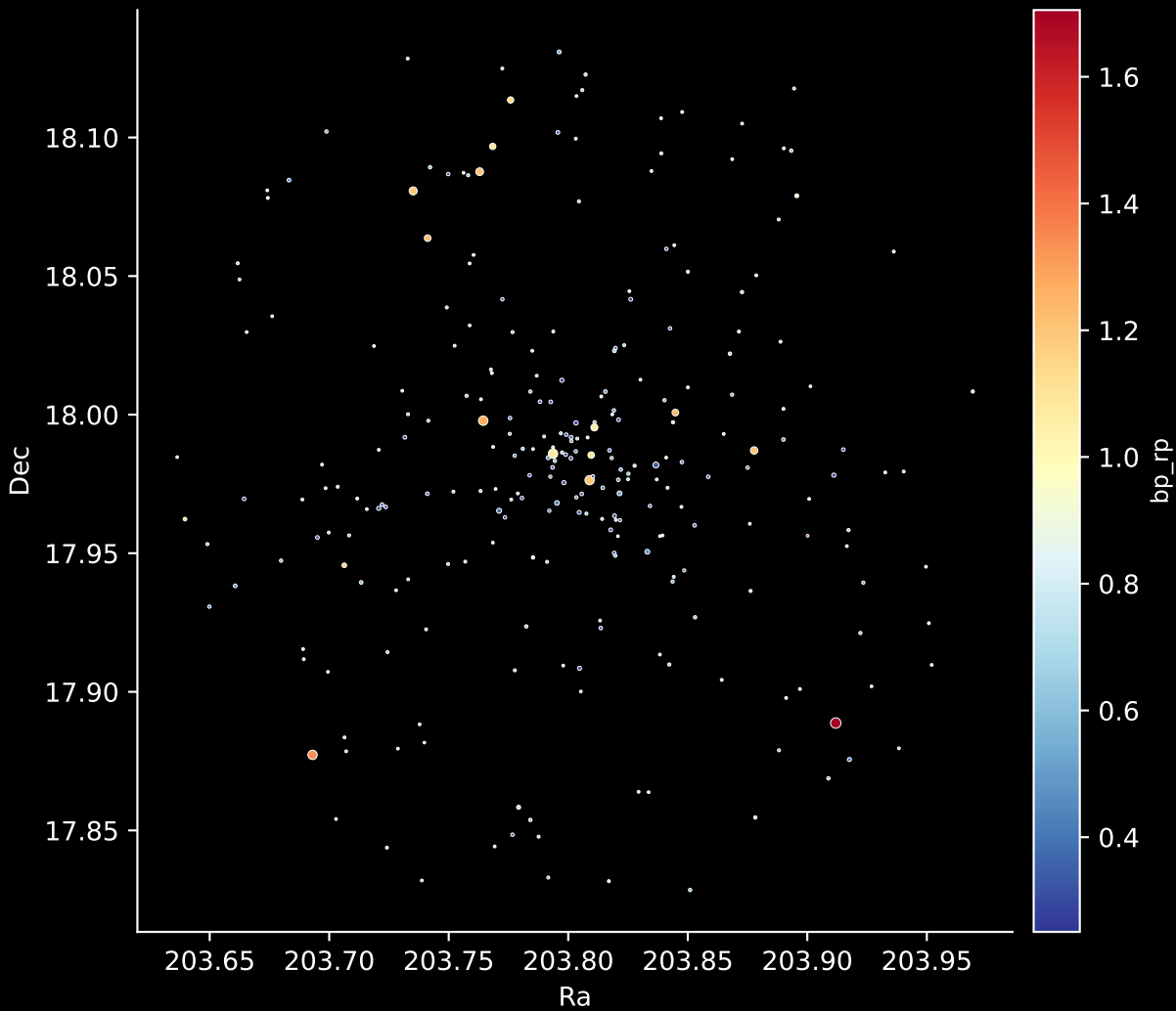
Gaia Cluster: [NGC_2304] Stars: 260
