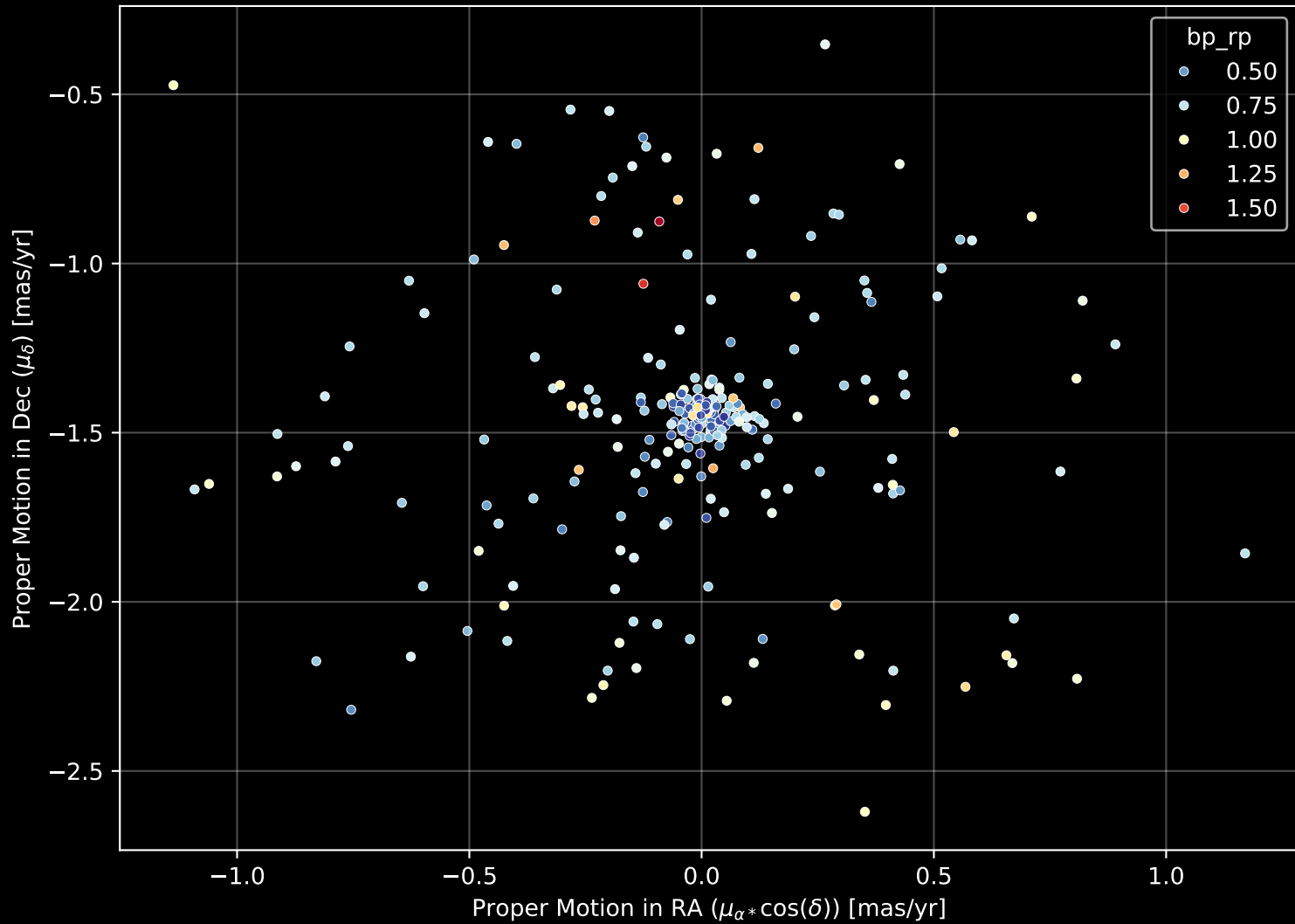
Gaia Cluster: [NGC_2304] Proper Motion Diagram (n= 260)
