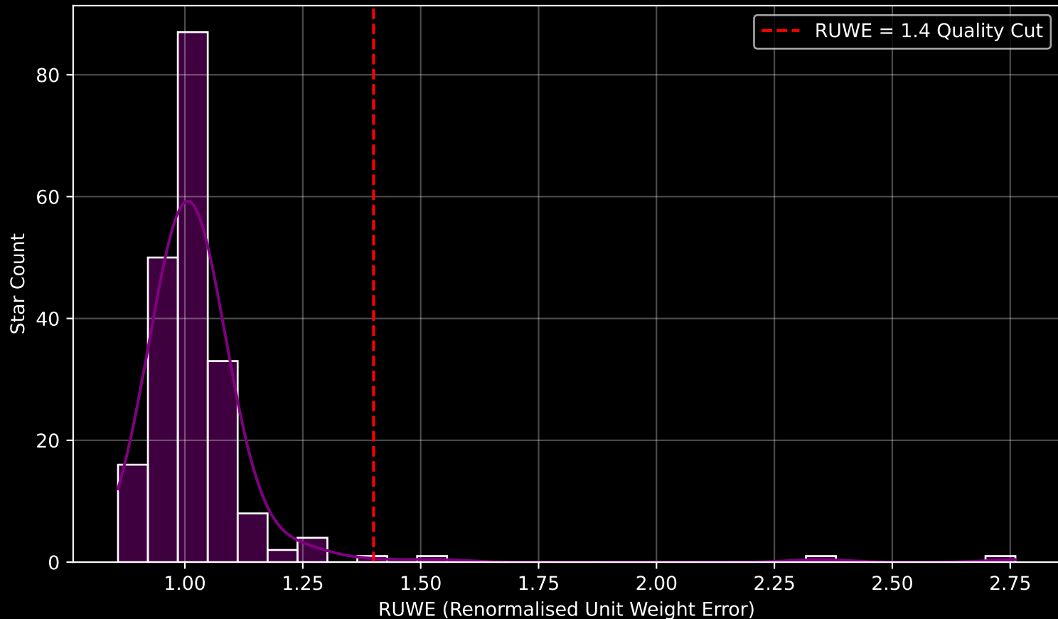
Gaia Cluster: [NGC_2311] RUWE Distribution (n= 204)
