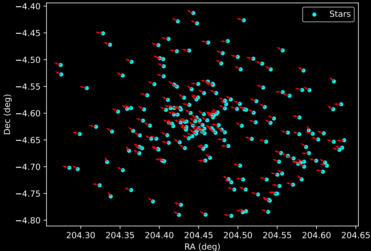
Gaia Cluster: [NGC_2311] Proper Motion Vectors for Gaia Star Field (n= 204)
