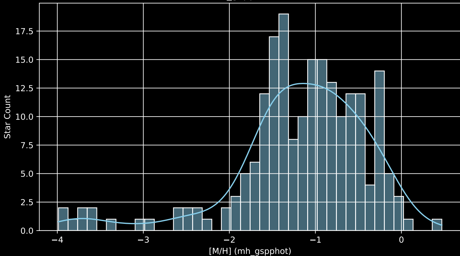
Gaia Cluster: [NGC_2311 [M/H] (mh_gspphot) (n= 204)
