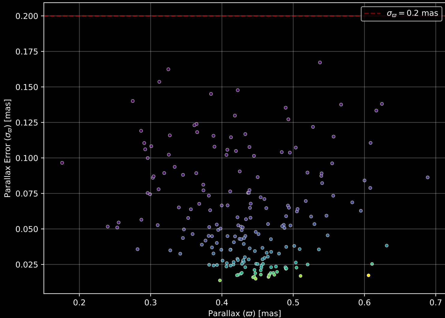
Gaia Cluster: [NGC_2311] Parallax Quality (n= 204)
