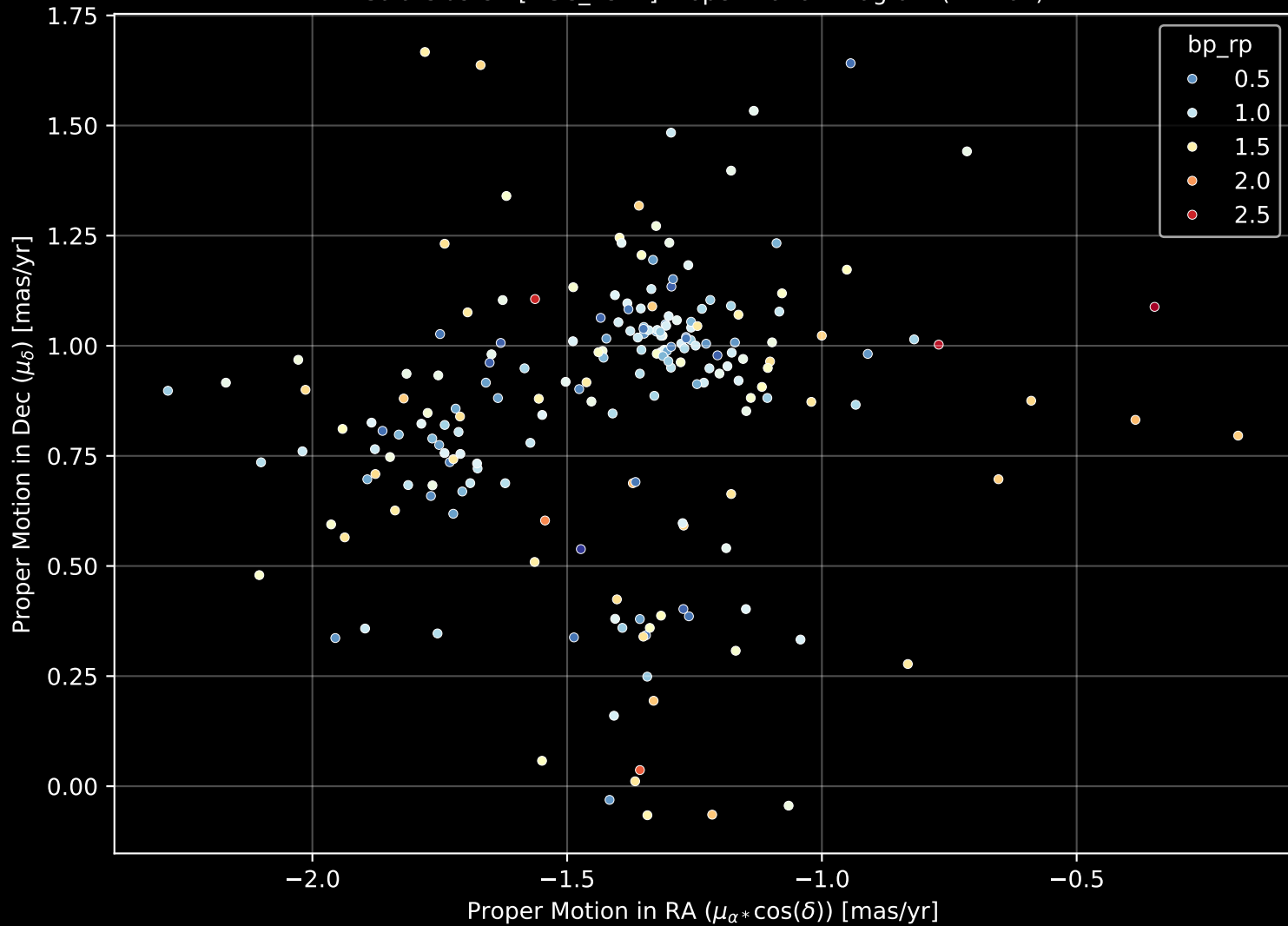
Gaia Cluster: [NGC_2311] Proper Motion Diagram (n= 204)
