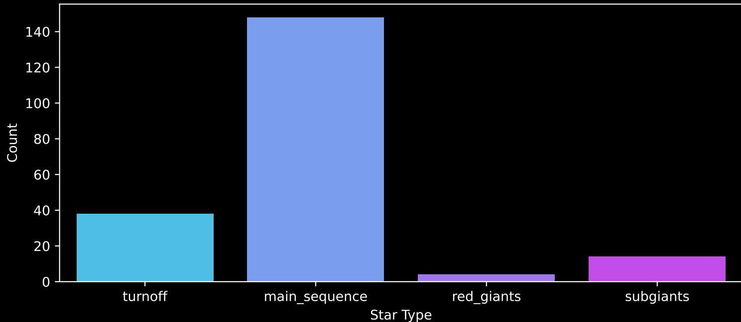
Gaia Cluster: [NGC_2311] Count plot of Star Type
