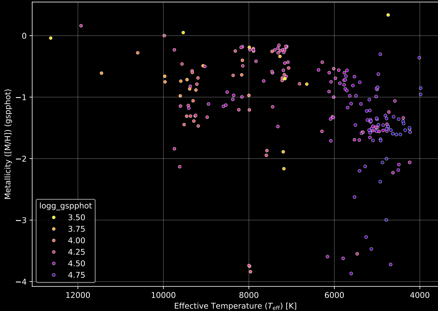
Gaia Cluster: [NGC_2335] Stellar Population Parameters (n= 209)
