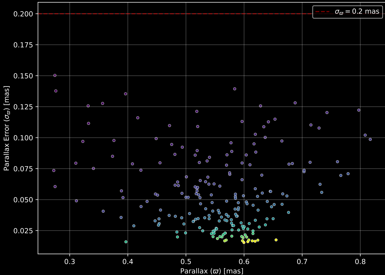
Gaia Cluster: [NGC_2335] Parallax Quality (n= 209)
