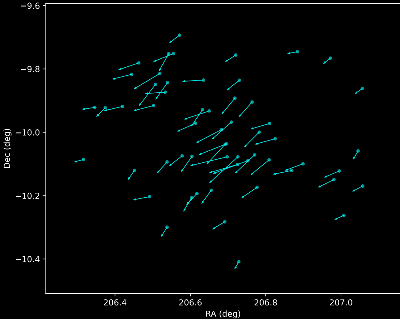
Gaia DR3 Noise Stream Proper Motion Vectors (n=57)
