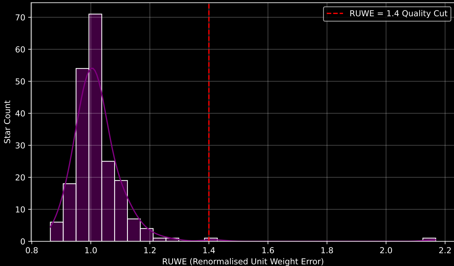
Gaia Cluster: [NGC_2335] RUWE Distribution (n= 208)
