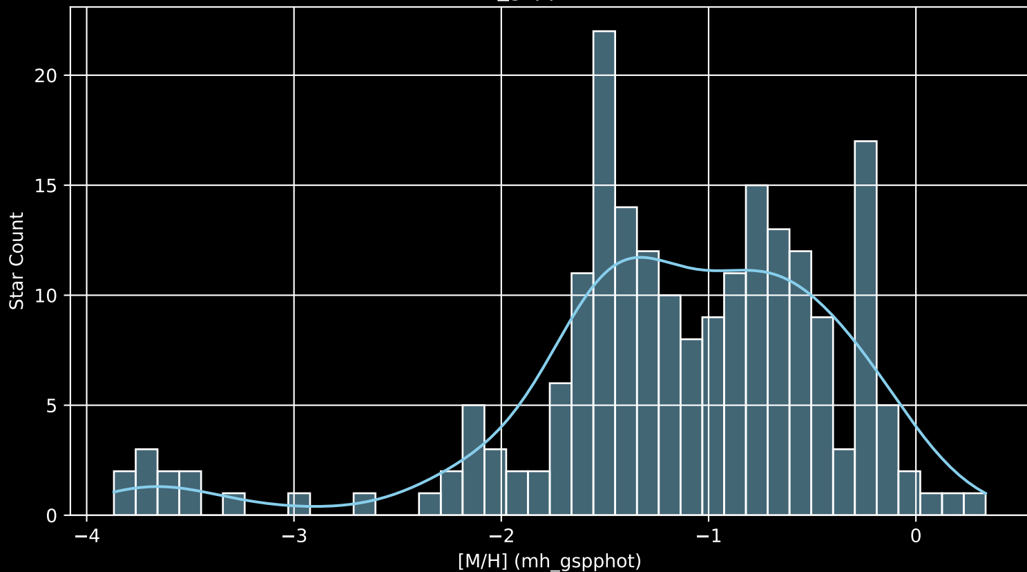
Gaia Cluster: [NGC_2335 [M/H] (mh_gspphot) (n= 209)
