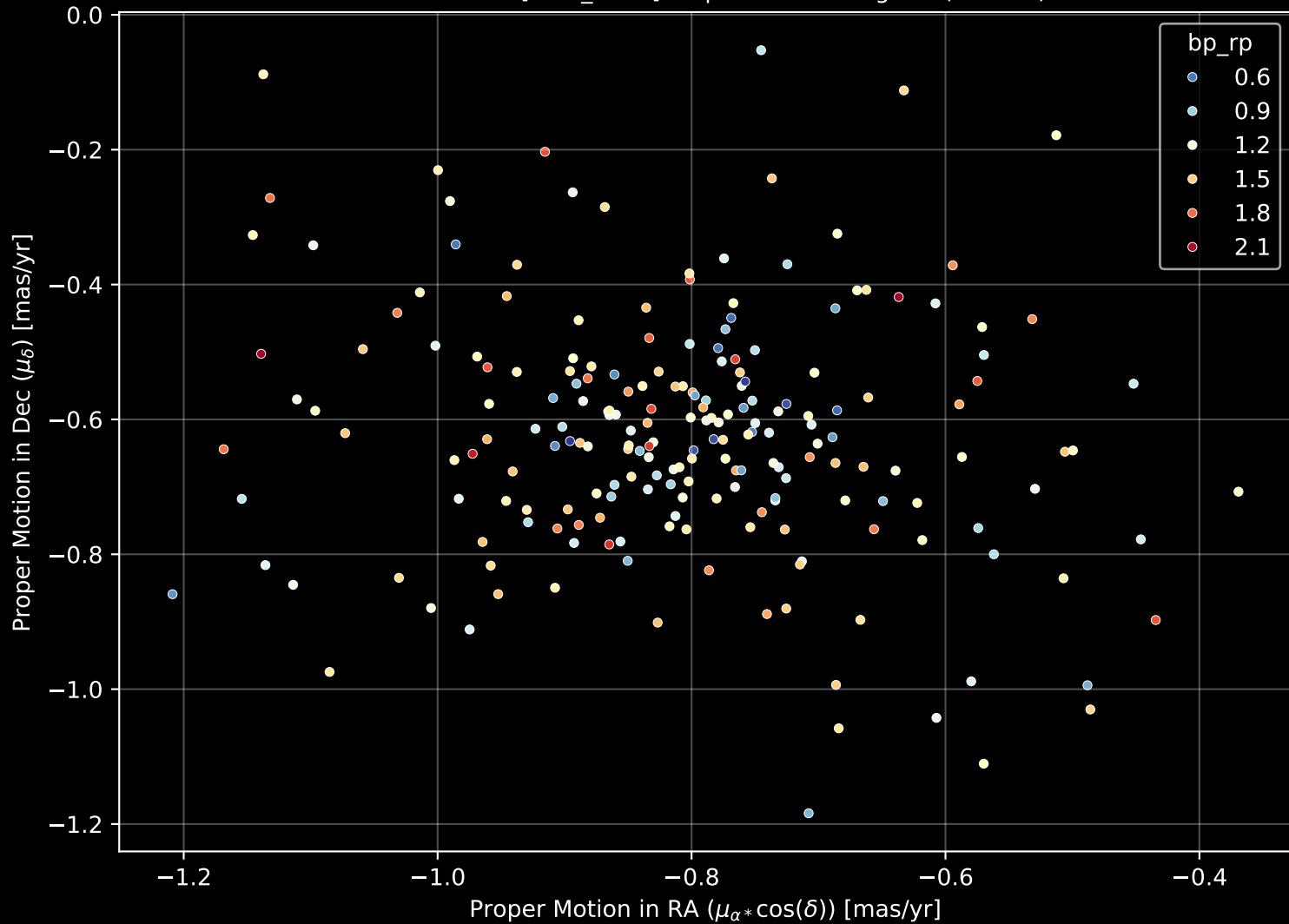
Gaia Cluster: [NGC_2335] Proper Motion Diagram (n= 209)
