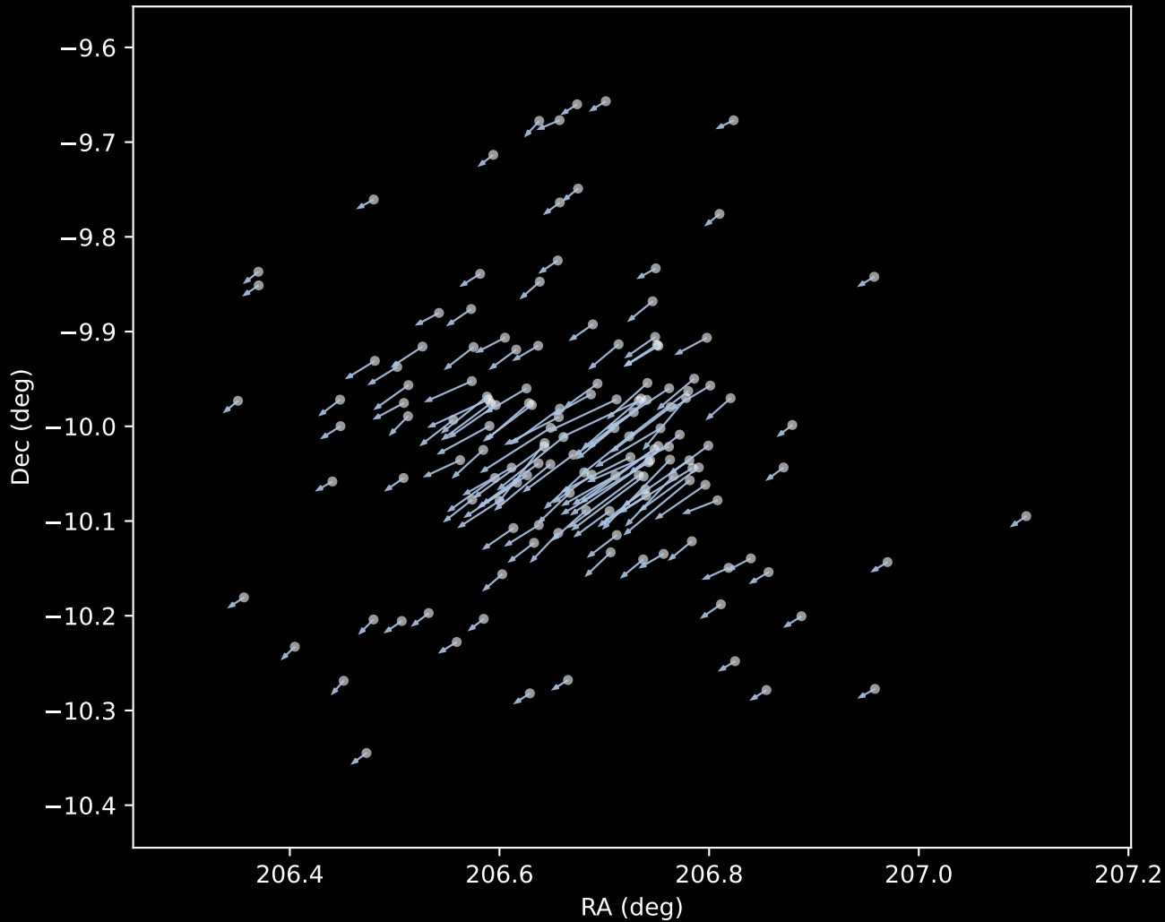
Gaia DR3 Cluster 1 Proper Motion Vectors (n=145)
