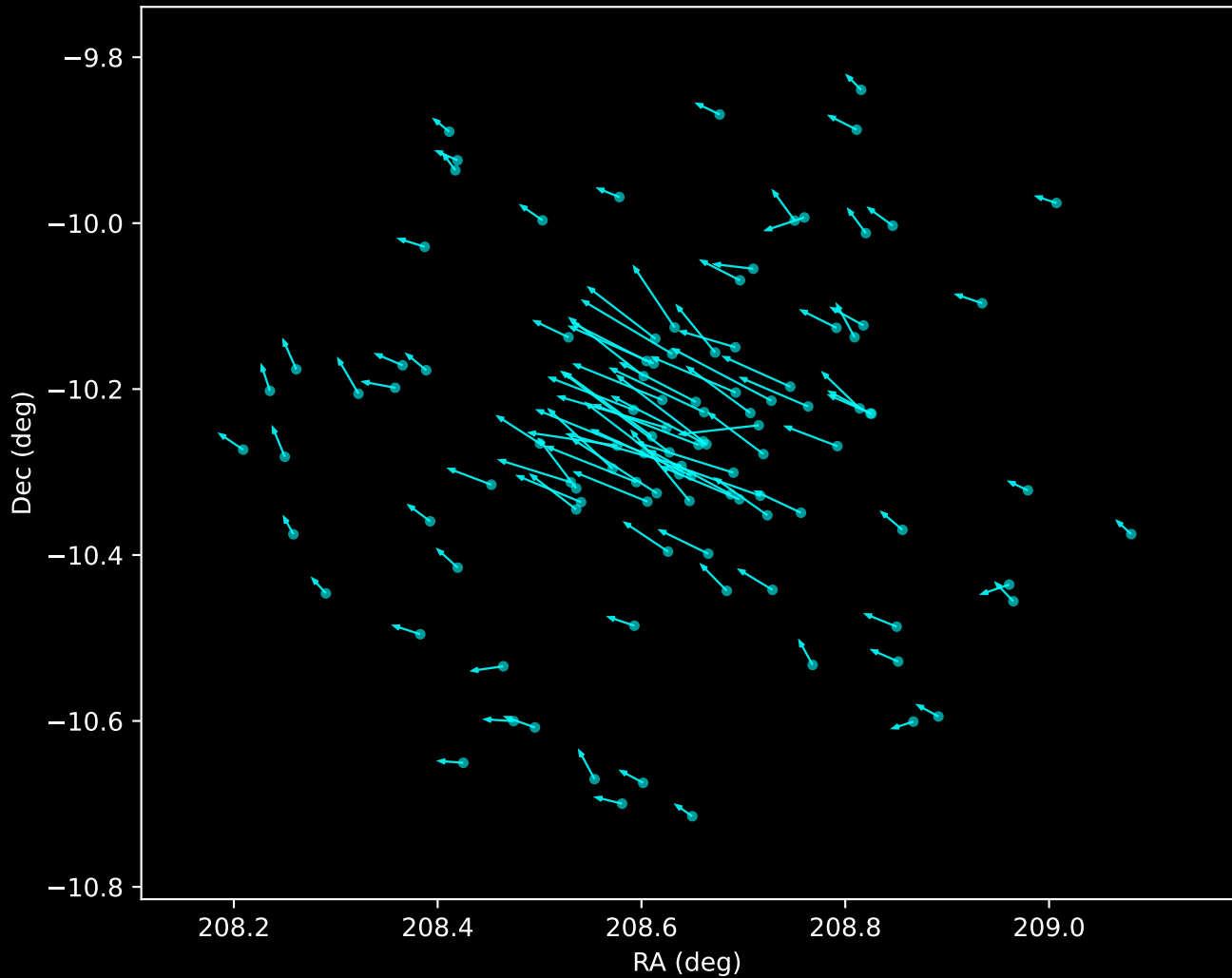
Gaia DR3 Noise Stream Proper Motion Vectors (n=108)
