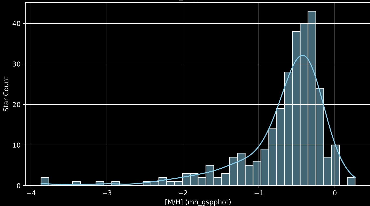
Gaia Cluster: [NGC_2353 [M/H] (mh_gspphot) (n= 289)
