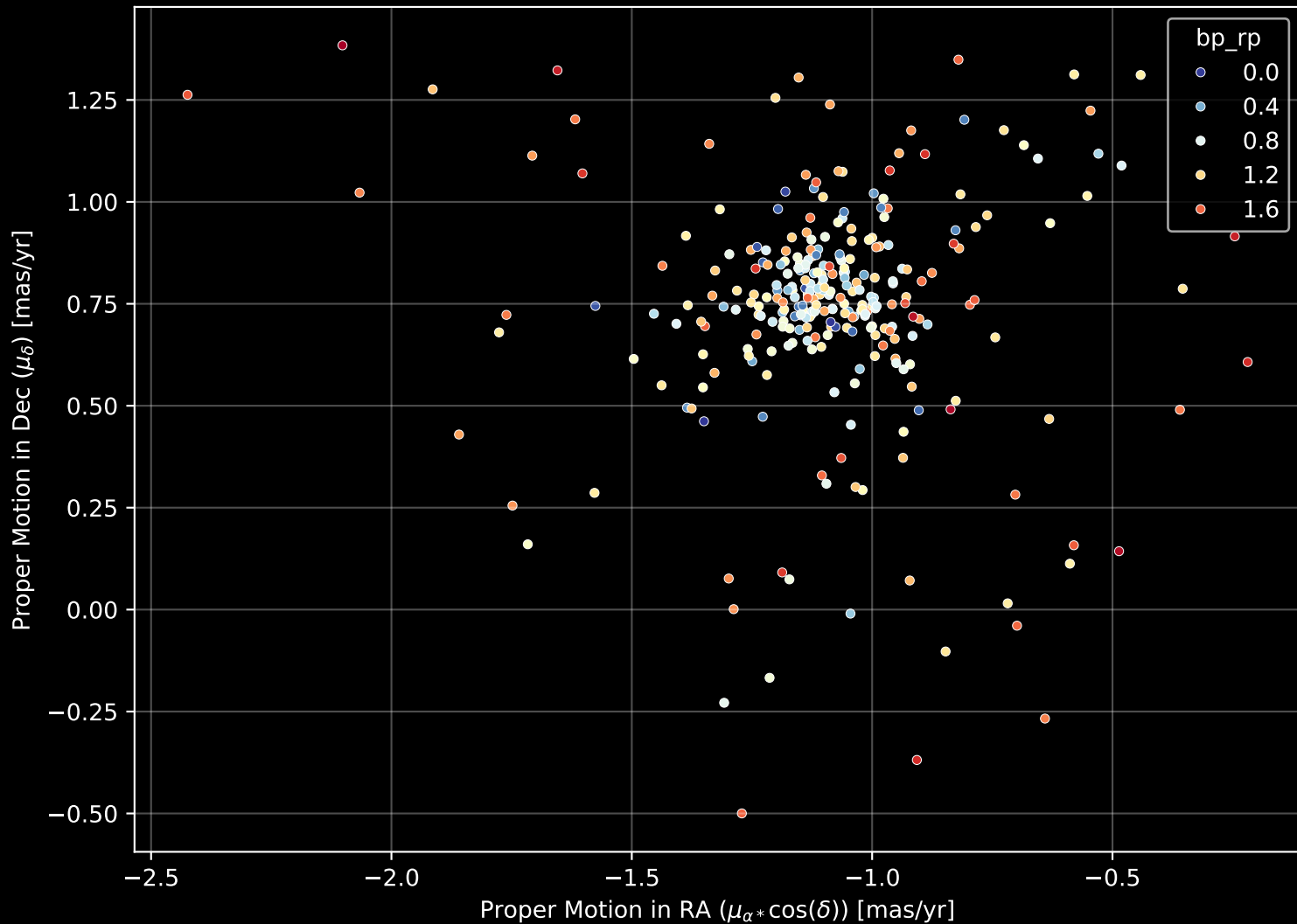
Gaia Cluster: [NGC_2353] Proper Motion Diagram (n= 289)
