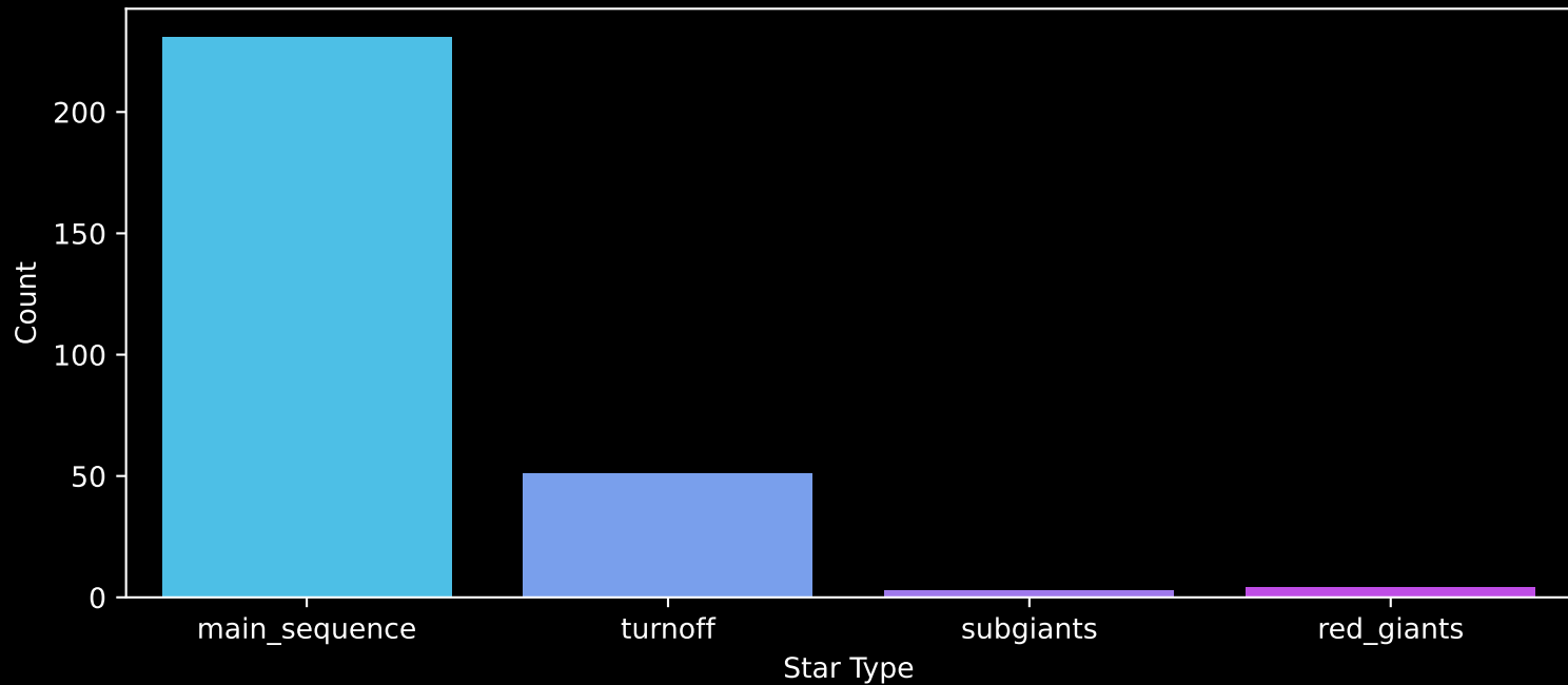
Gaia Cluster: [NGC_2353] Count plot of Star Type
