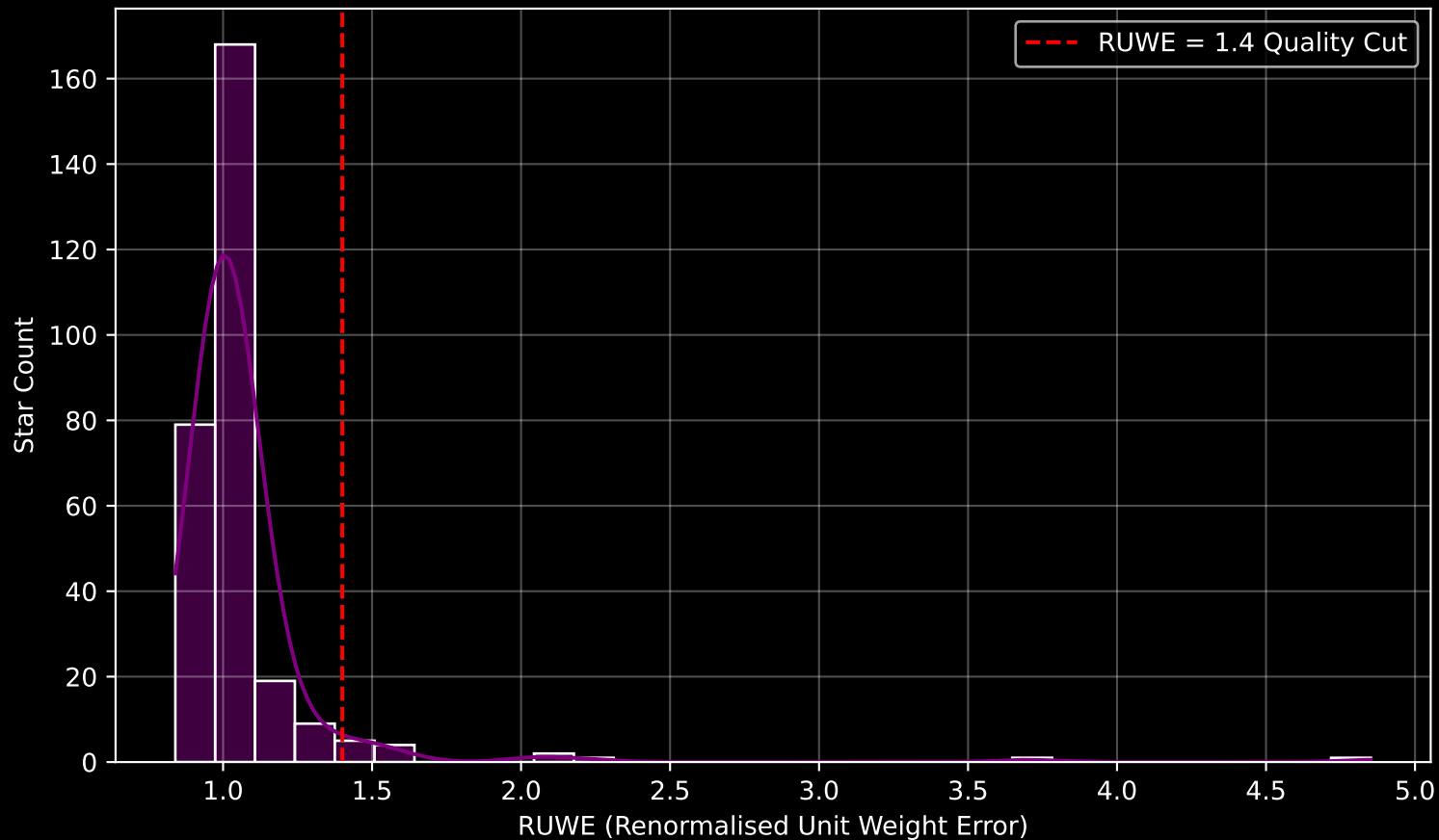
Gaia Cluster: [NGC_2353] RUWE Distribution (n= 289)
