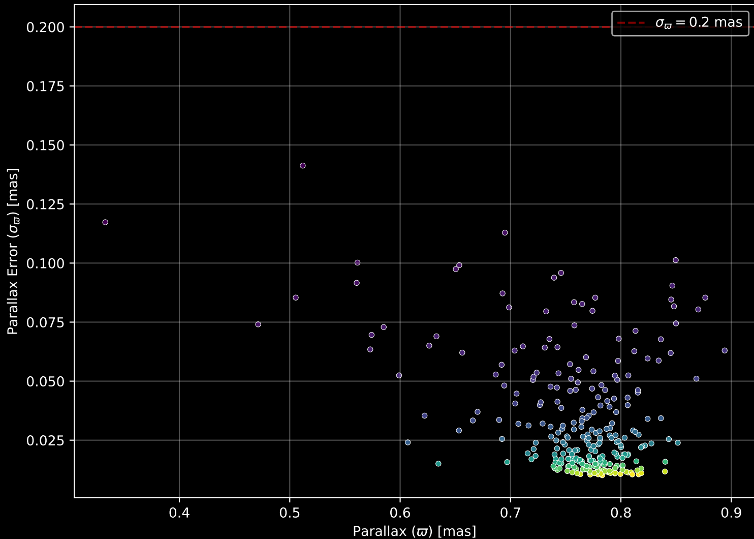
Gaia Cluster: [NGC_2354] Parallax Quality (n= 273)
