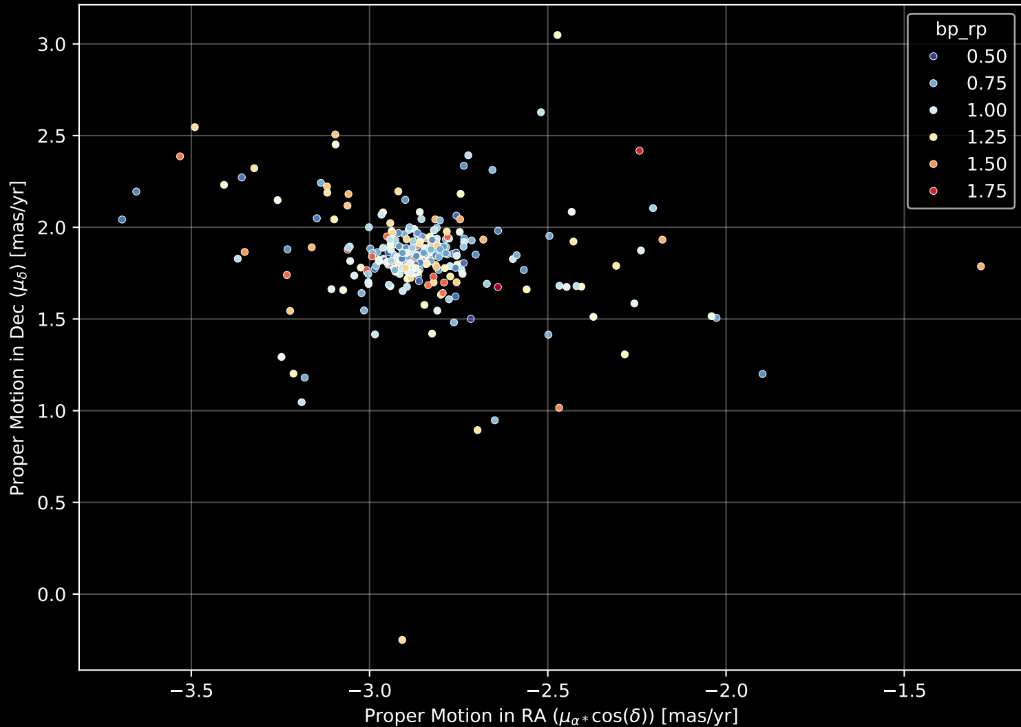
Gaia Cluster: [NGC_2354] Proper Motion Diagram (n= 273)
