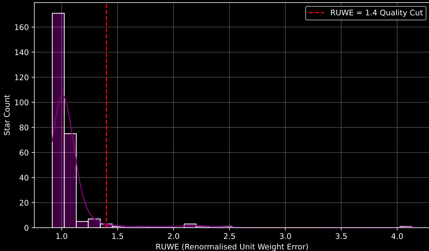
Gaia Cluster: [NGC_2354] RUWE Distribution (n= 272)
