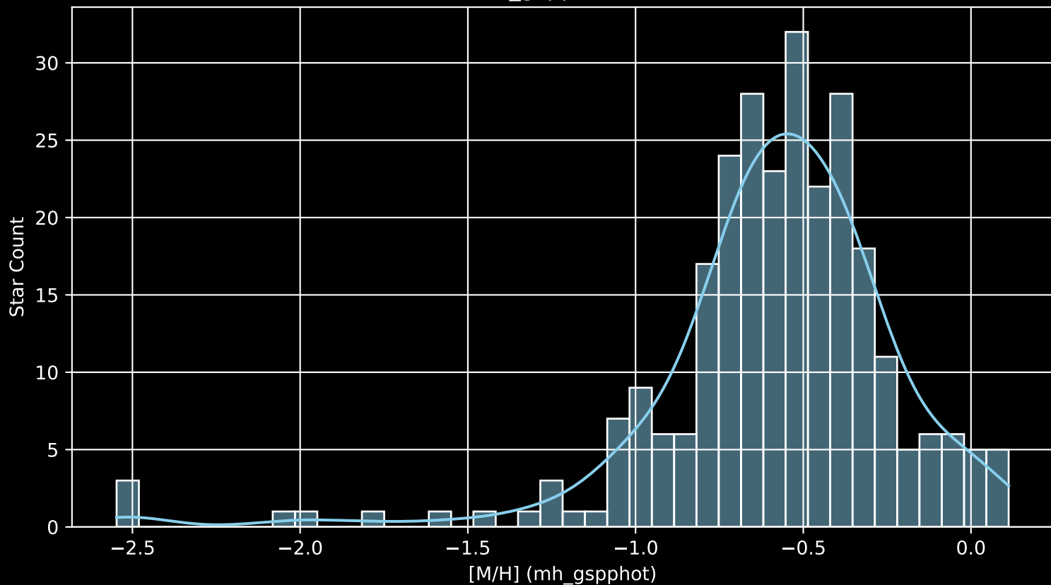
Gaia Cluster: [NGC_2354 [M/H] (mh_gspphot) (n= 272)
