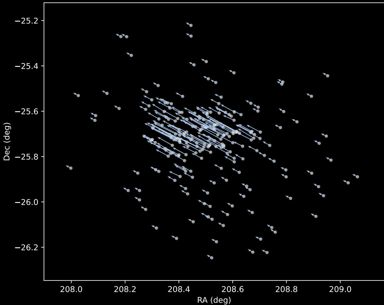
Gaia DR3 Cluster 1 Proper Motion Vectors (n=208)
