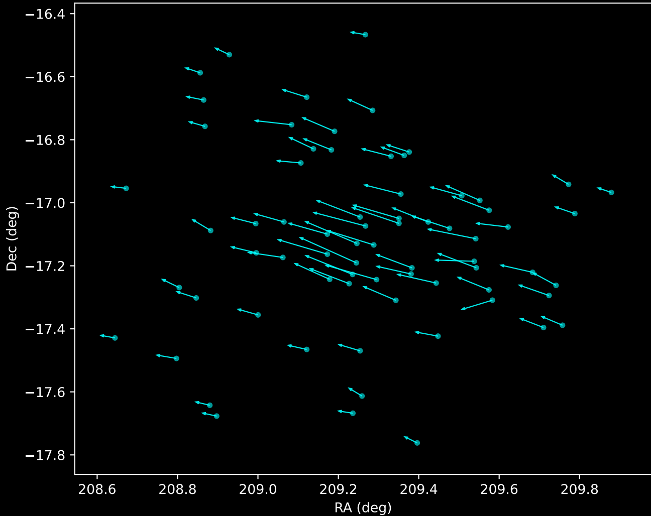
Gaia DR3 Noise Stream Proper Motion Vectors (n=71)
