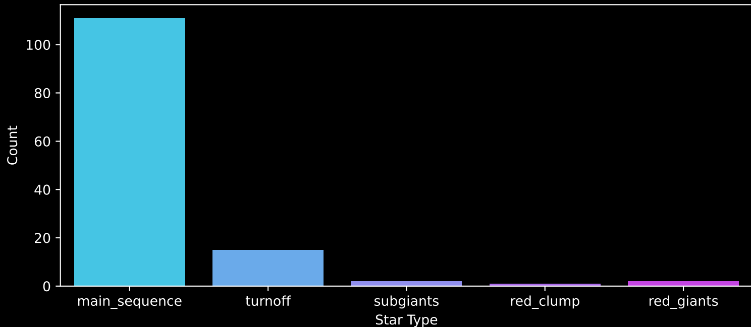
Gaia Cluster: [NGC_2358] Count plot of Star Type
