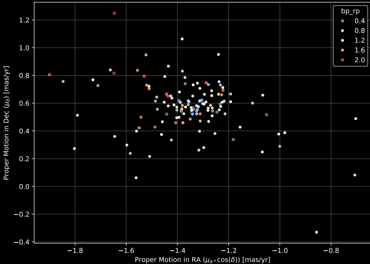
Gaia Cluster: [NGC_2358] Proper Motion Diagram (n= 131)
