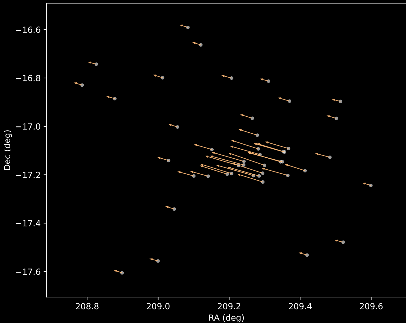
Gaia DR3 Cluster 3 Proper Motion Vectors (n=44)
