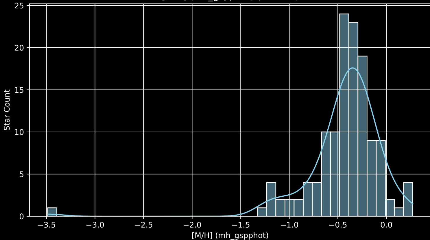
Gaia Cluster: [NGC_2358 [M/H] (mh_gspphot) (n= 131)
