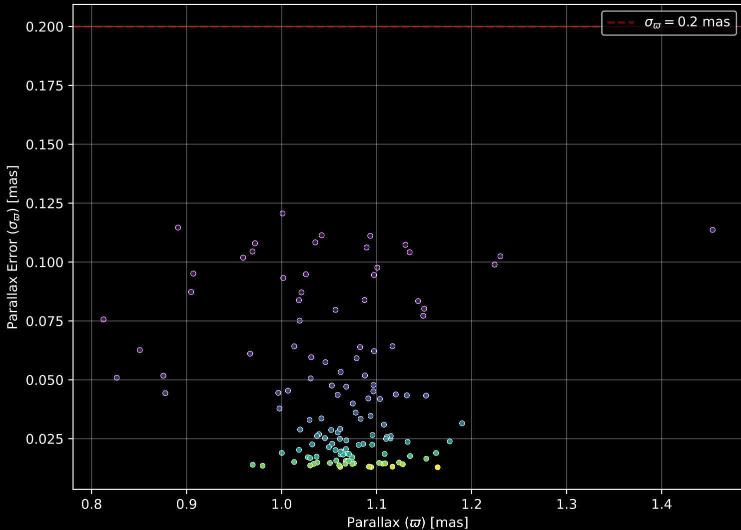
Gaia Cluster: [NGC_2358] Parallax Quality (n= 131)
