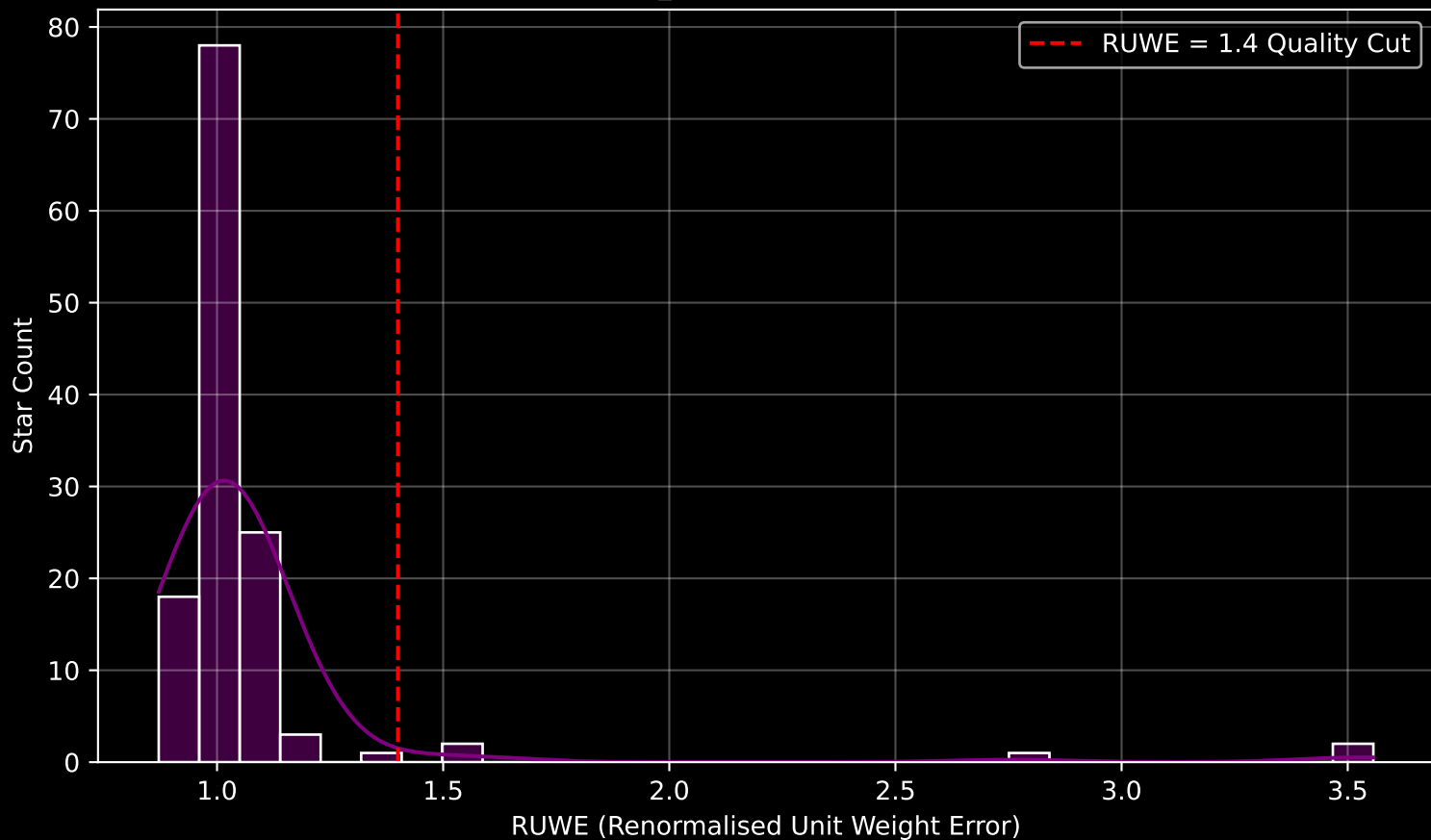
Gaia Cluster: [NGC_2358] RUWE Distribution (n= 130)
