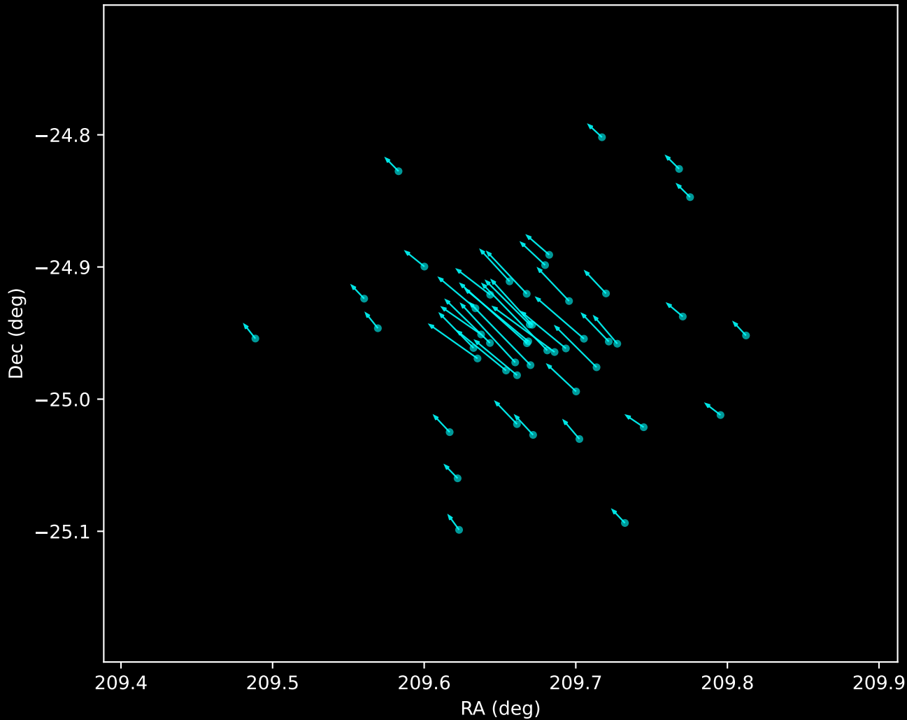
Gaia DR3 Noise Stream Proper Motion Vectors (n=47)
