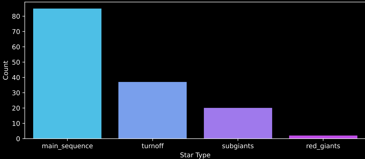
Gaia Cluster: [NGC_2362] Count plot of Star Type
