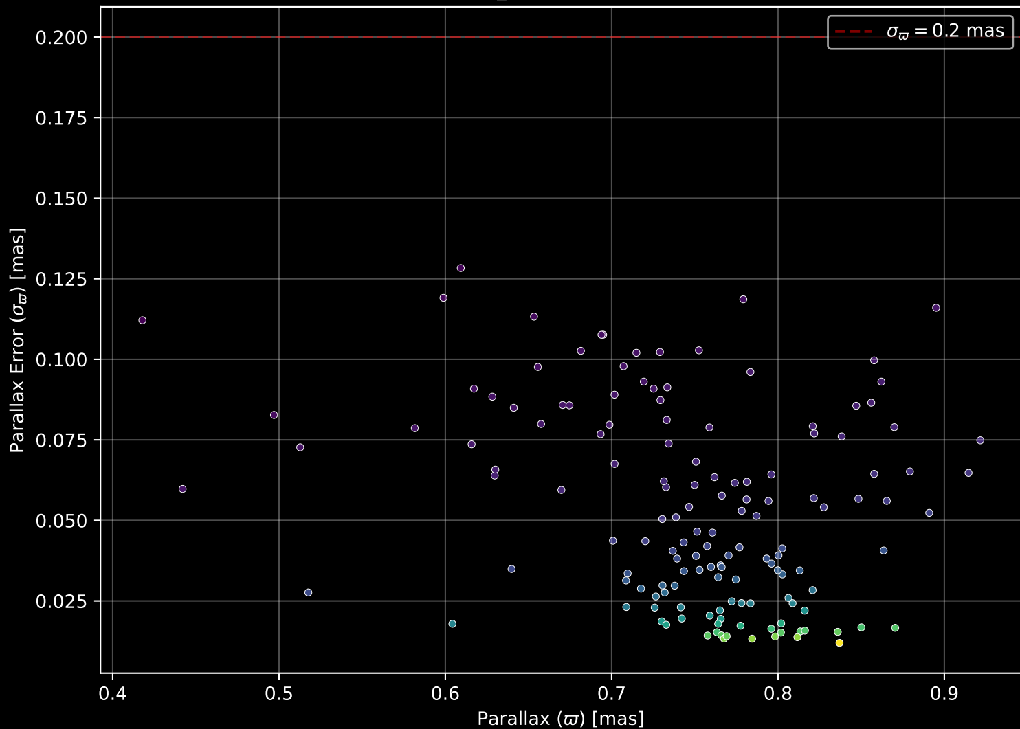
Gaia Cluster: [NGC_2362] Parallax Quality (n= 144)
