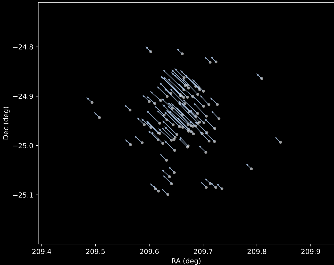
Gaia DR3 Cluster 1 Proper Motion Vectors (n=92)
