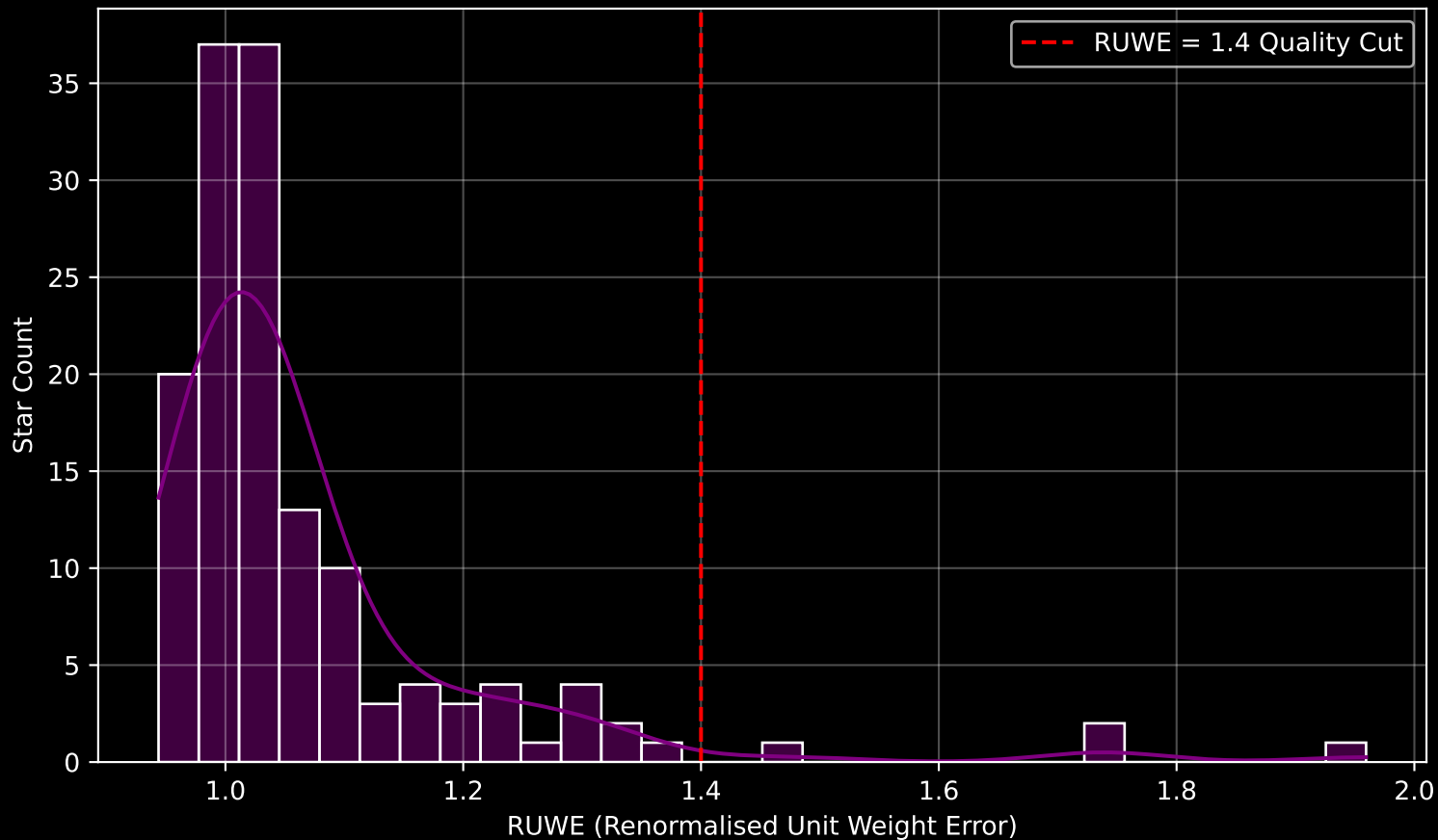
Gaia Cluster: [NGC_2362] RUWE Distribution (n= 143)
