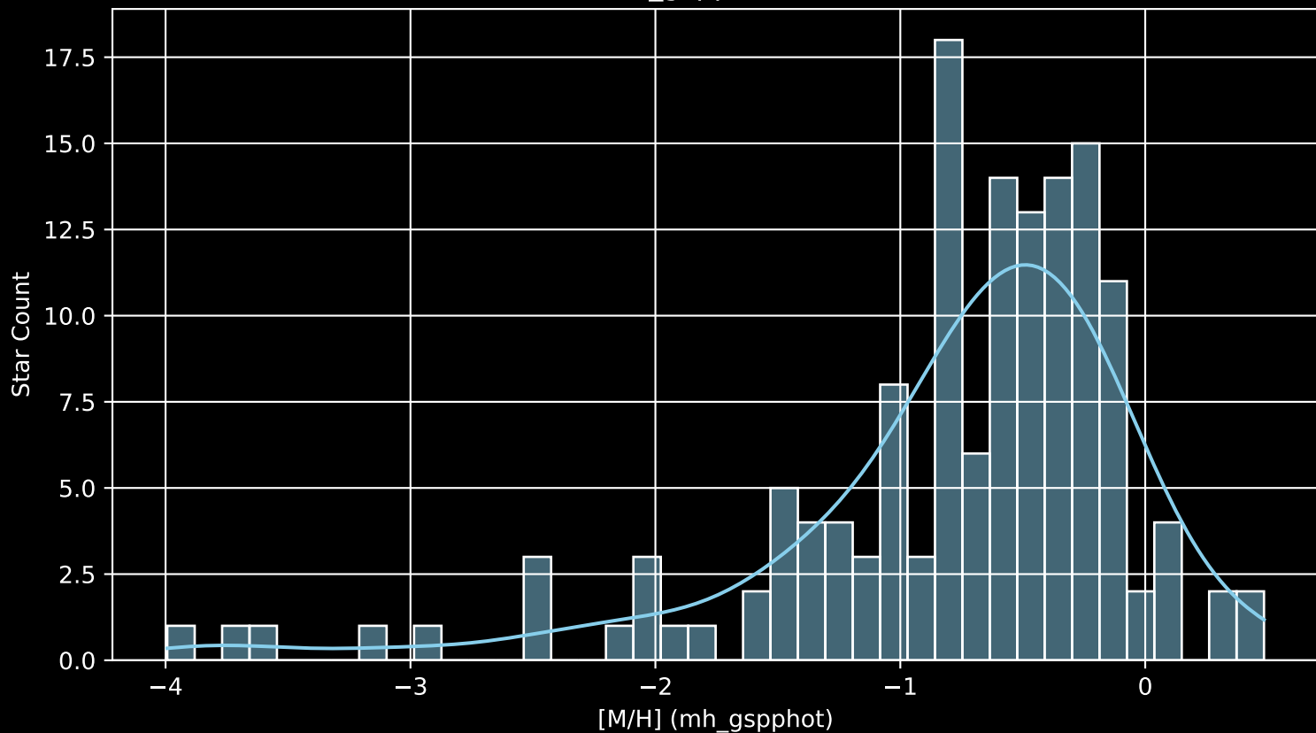
Gaia Cluster: [NGC_2362 [M/H] (mh_gspphot) (n= 144)
