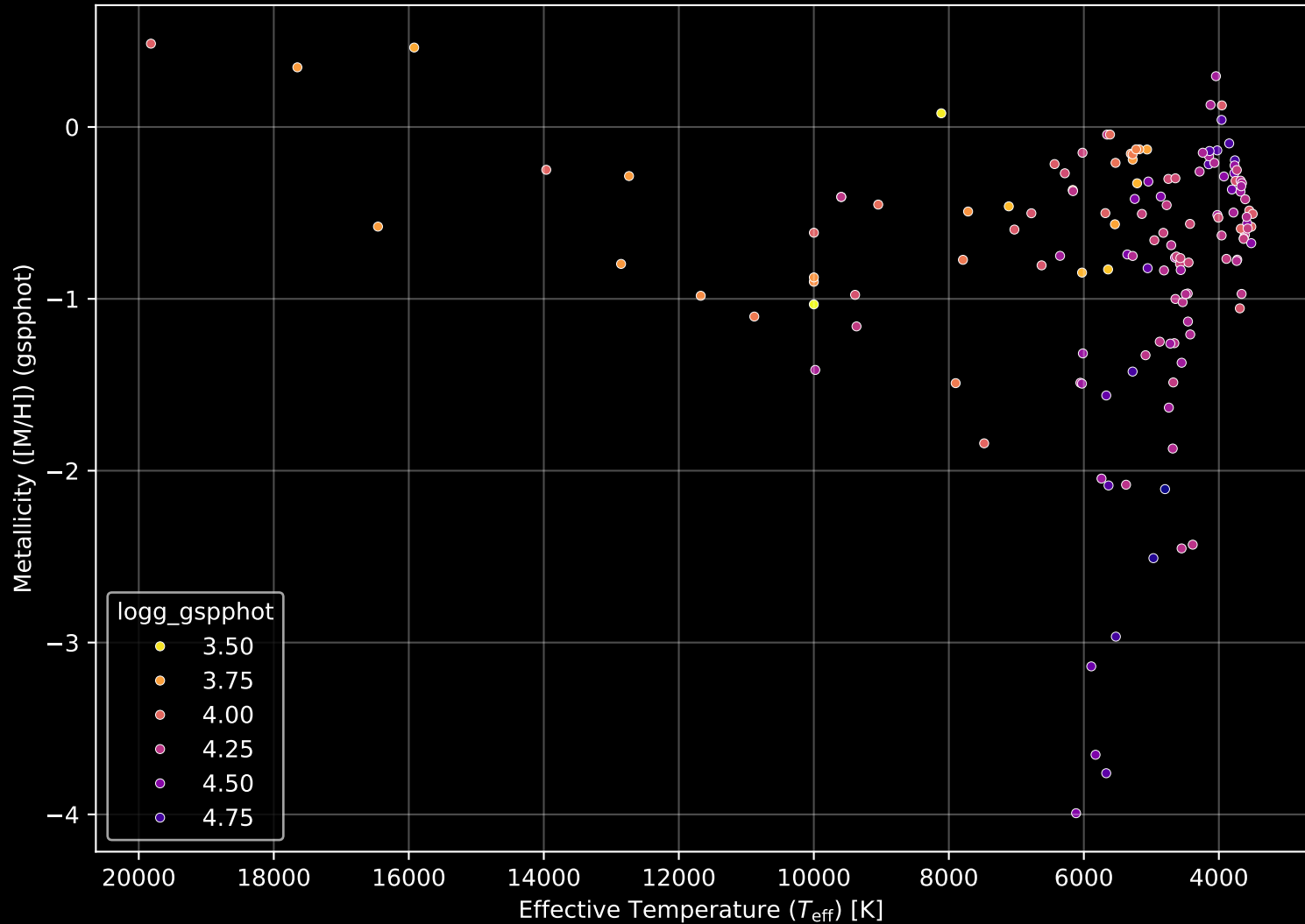
Gaia Cluster: [NGC_2362] Stellar Population Parameters (n= 144)
