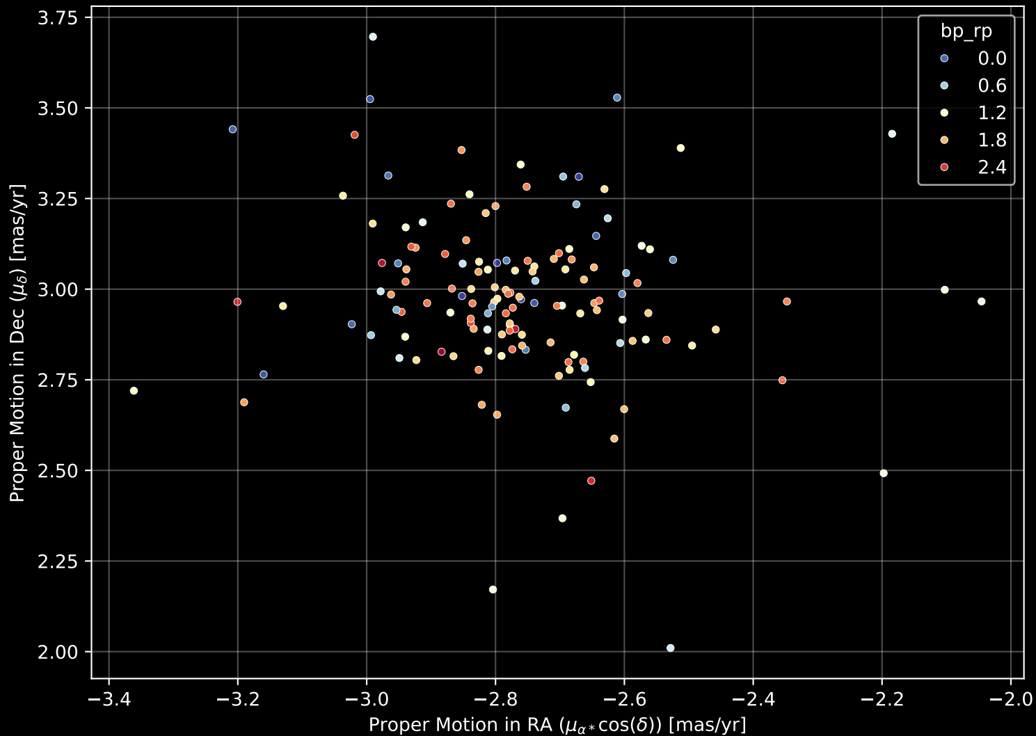
Gaia Cluster: [NGC_2362] Proper Motion Diagram (n= 144)
